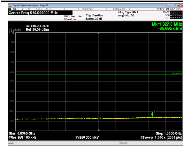
66-66-5MHz-20MHz-16QAM-16QAM-132005-132122-1RB B#0-0RB#0-30~1000MHz-PASS
