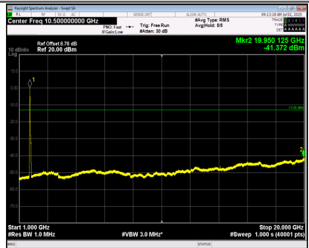
66-66-5MHz-20MHz-QPSK-QPSK-132330-132447-1RB#0- ORB#0-1000~20000MHz-PASS
