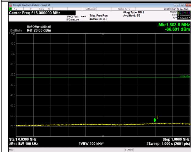
66-66-5MHz-20MHz-16QAM-16QAM-132005-132122-1RB B#0-1RB#99-30~1000MHz-PASS
