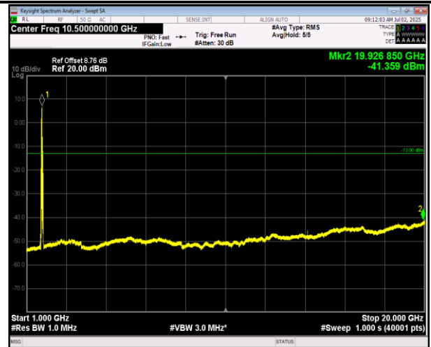
66-66-5MHz-20MHz-16QAM-16QAM-132005-132122-1RB #24-ORB#0-1000~20000MHz-PASS
