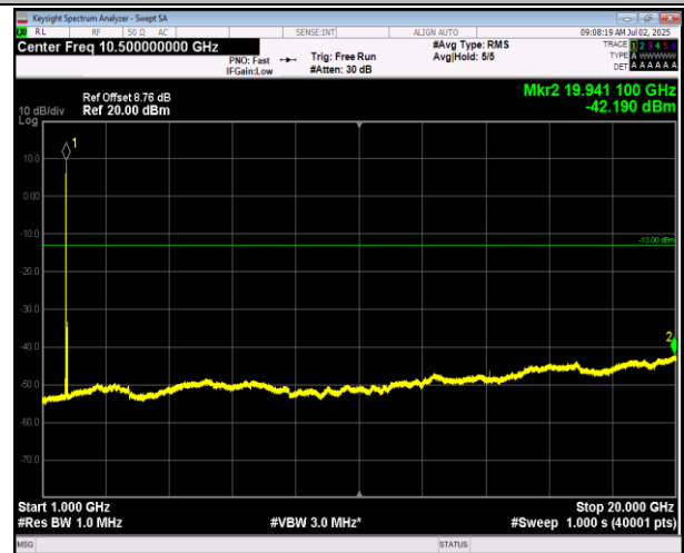
66-66-5MHz-20MHz-16QAM-16QAM-132005-132122-1RB #0-1RB#99-1000~20000MHz-PASS
