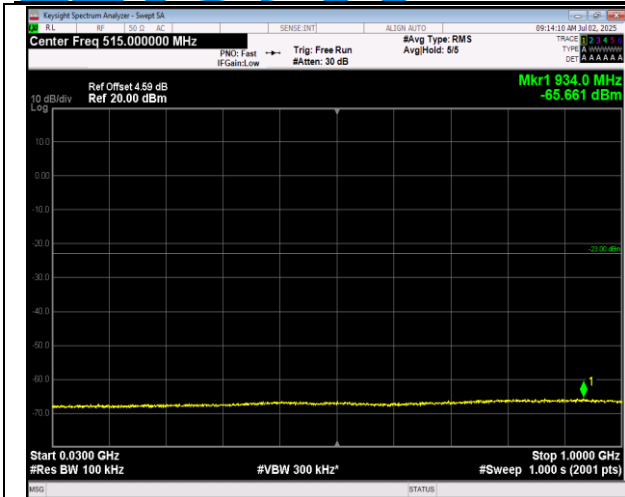
66-66-5MHz-20MHz-QPSK-QPSK-132330-132447-1RB# 0-1RB#99-30~1000MHz-PASS
