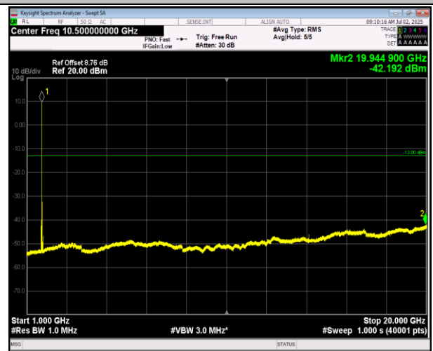
66-66-5MHz-20MHz-16QAM-16QAM-132005-132122-25R B#0-100RB#0-1000~20000MHz-PASS
