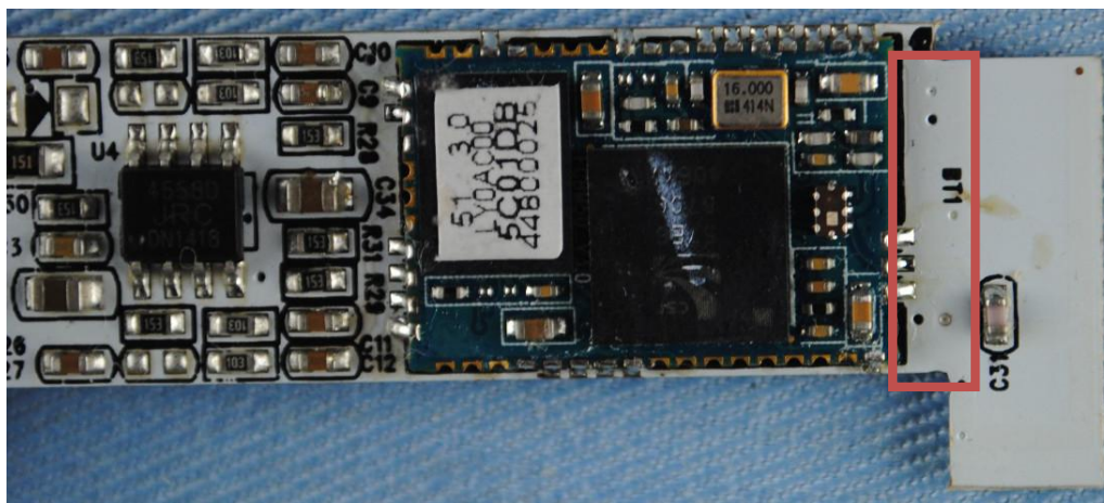
Antenna View
