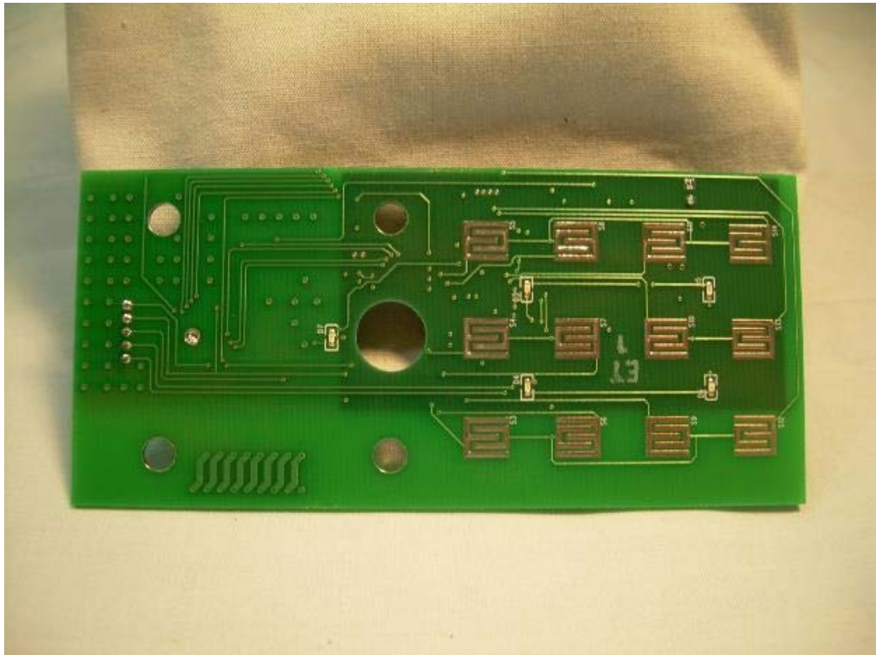
Photograph 13 – View of the Front Side of the KP001 PCB
