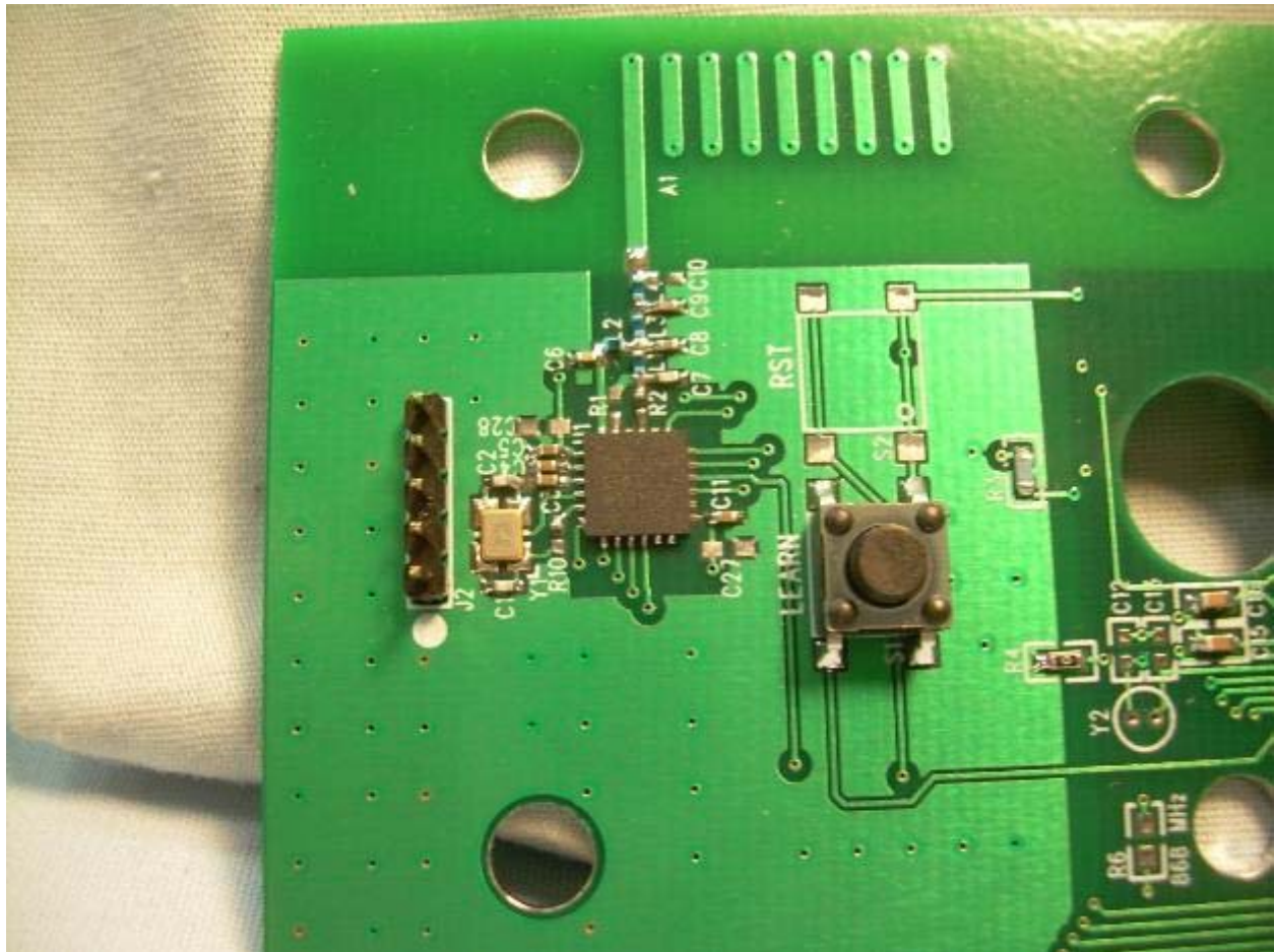
Photograph 15 – View of the RF Section of the KP001
