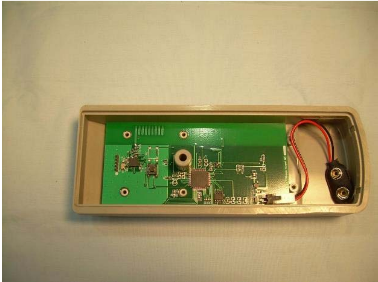
Photograph 12 – View of the PCB in the KP001 Housing
