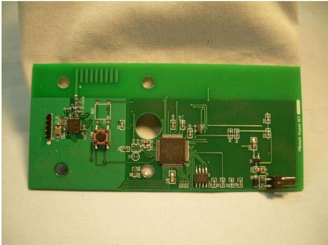
Photograph 14 – View of the Back Side of the KP001 PCB
