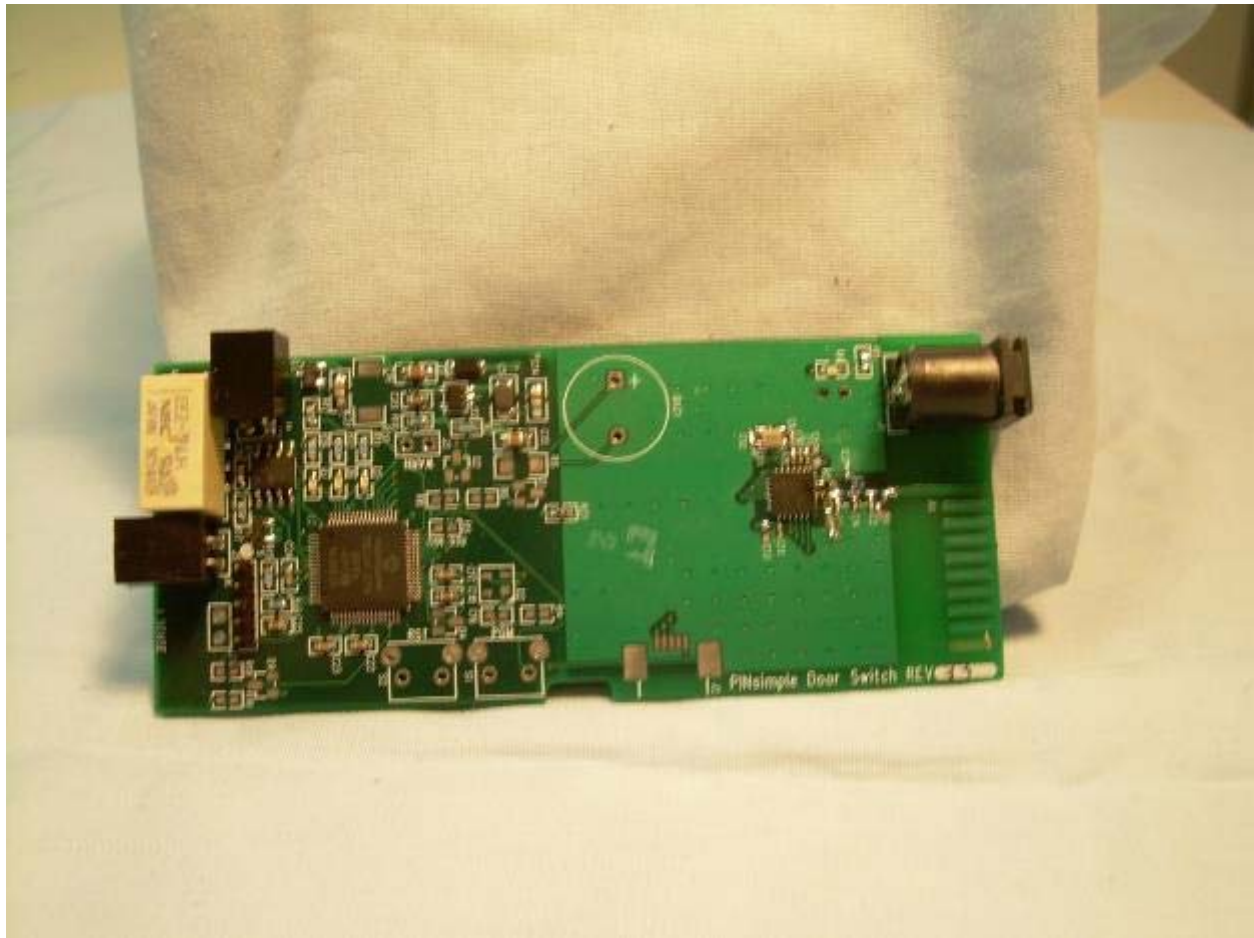
Photograph 25 – View of the Top Side of the DS001 PCB
