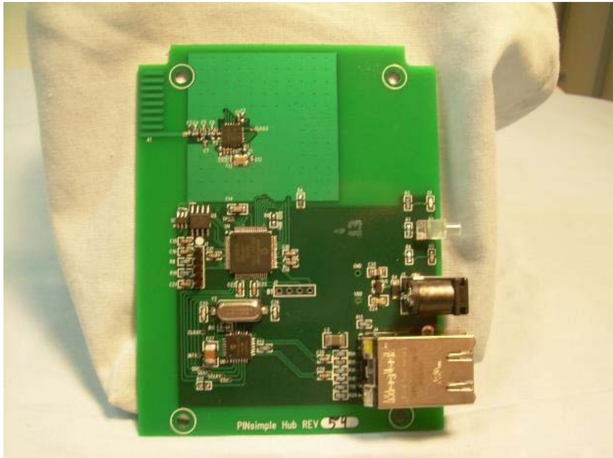
Photograph 19 – View of the Top Side of the HUB001 PCB
