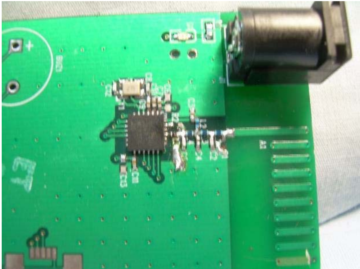
Photograph 27 – View of the RF Section of the DS001 PCB
