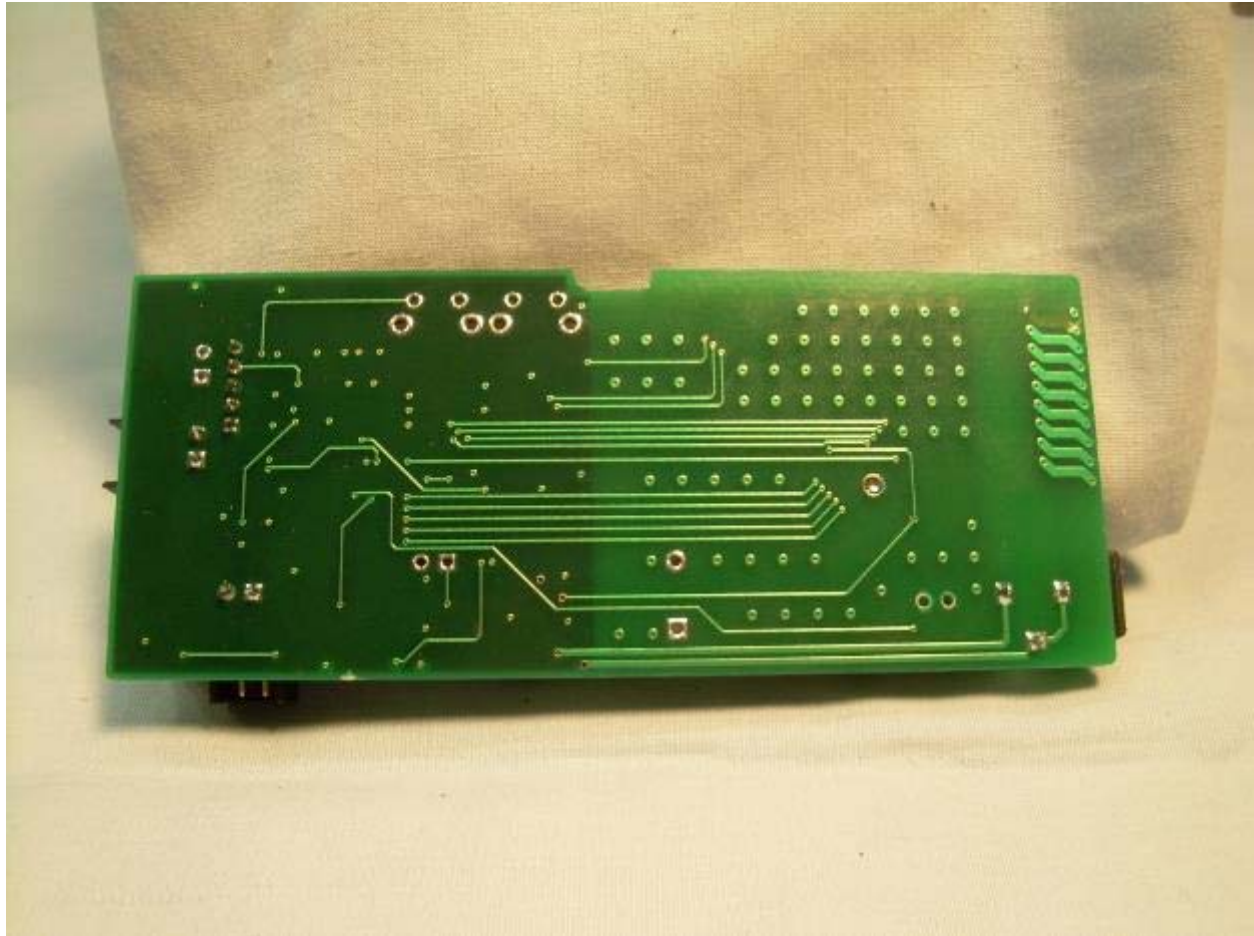
Photograph 26 – View of the Bottom Side of the DS001 PCB
