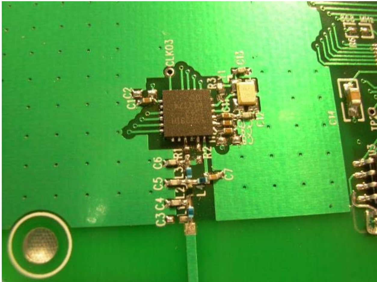
Photograph 21 – View of the RF Section of the HUB001
