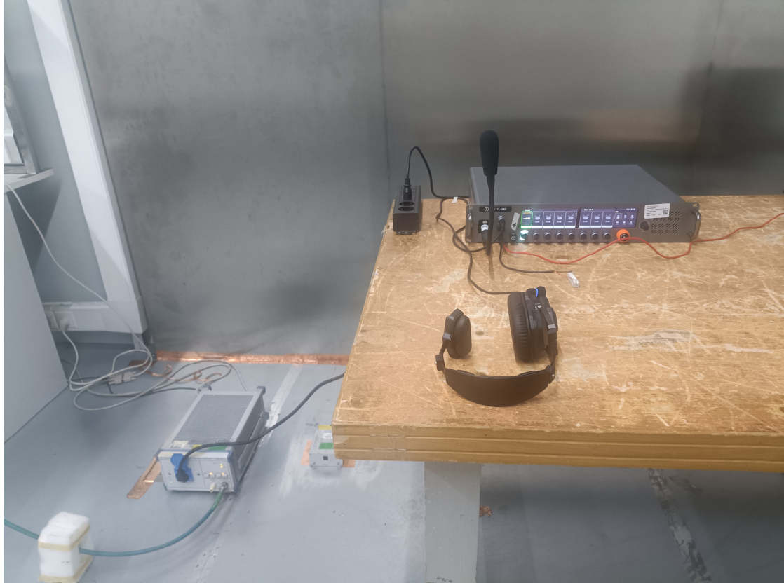
Conducted Emissions - Side View_ AC Mains
