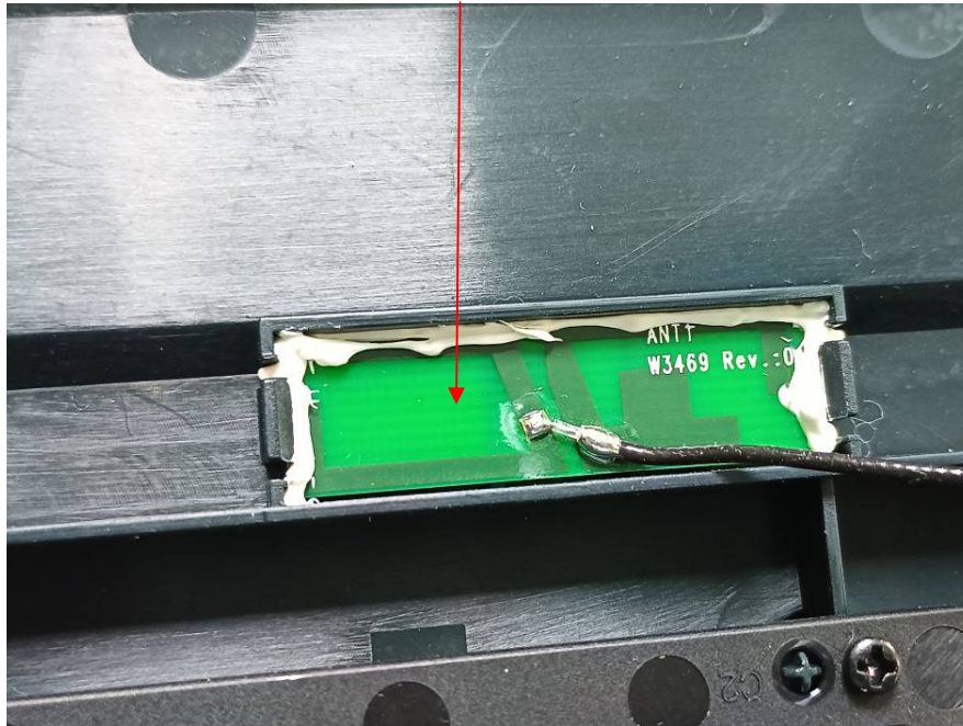
Bluetooth/Wi-Fi ANT
