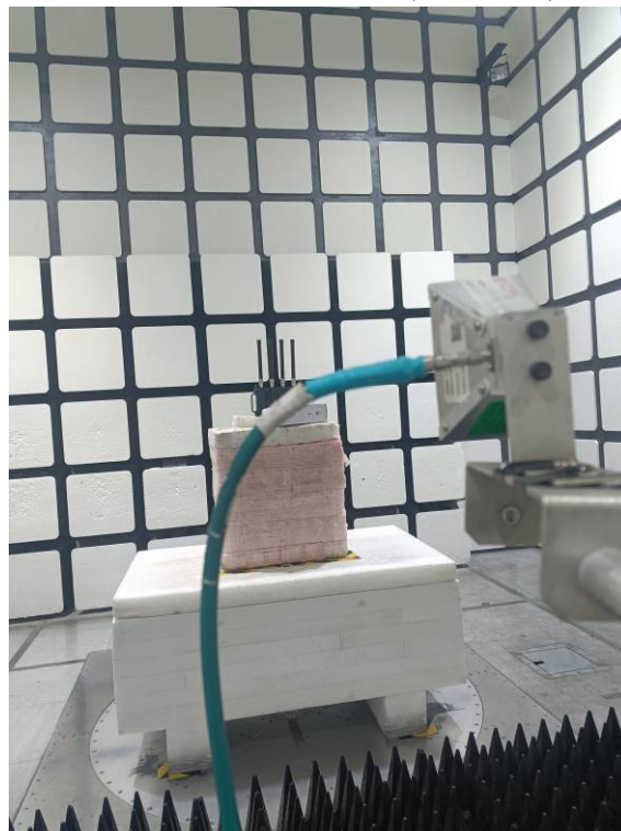
Radiated Emissions View (18-25 GHz)
