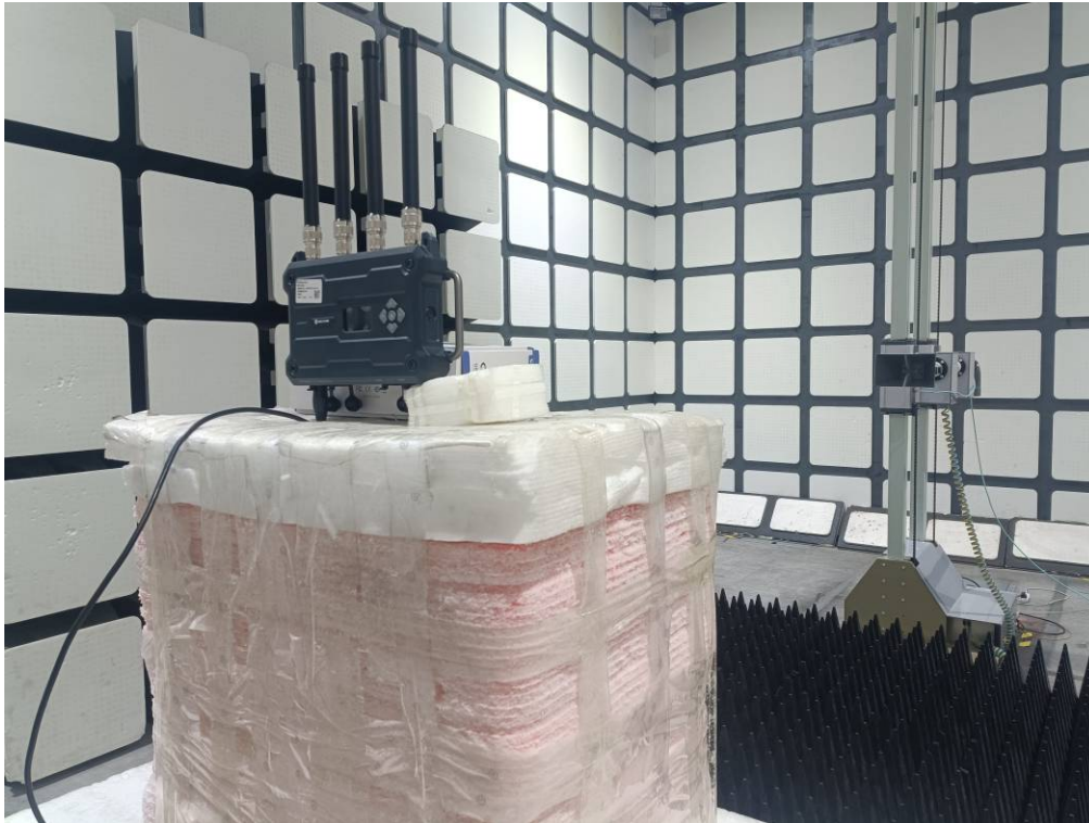
Radiated Emissions View (1-18 GHz)
