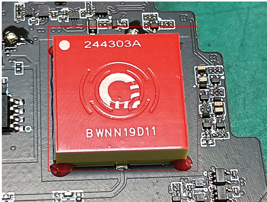
DECT ANT2
