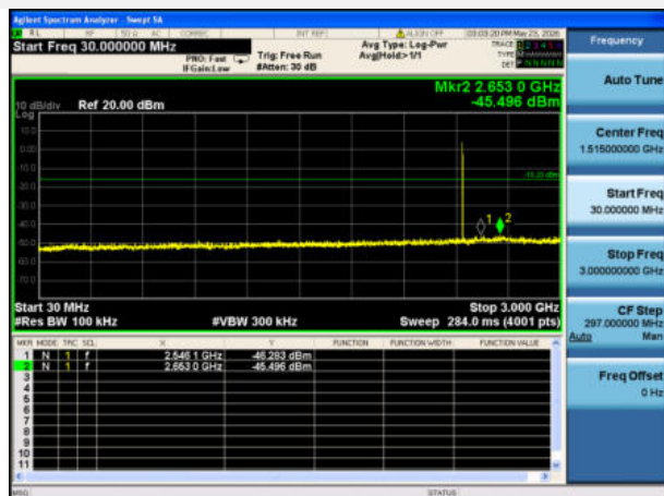
30 MHz ~ 3 GHz
