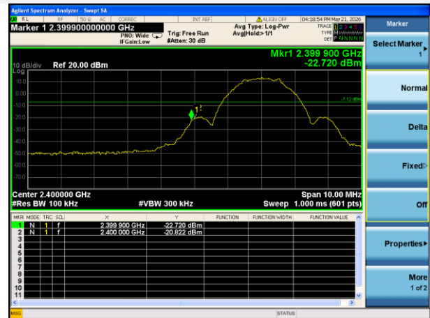
GFSK (2Mbps) LOW CHANNEL, BAND EDGE
