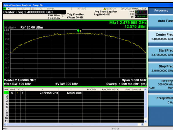
GFSK (2Mbps) HIGH CHANNEL, CARRIER LEVEL
