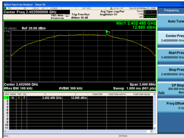
GFSK (2Mbps) LOW CHANNEL, CARRIER LEVEL
