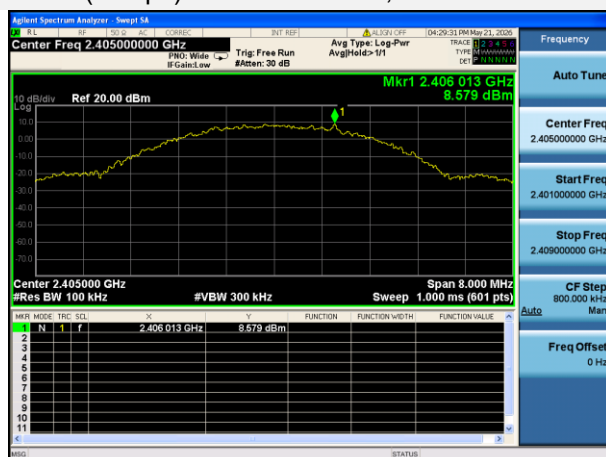
GFSK (4Mbps) LOW CHANNEL, CARRIER LEVEL
