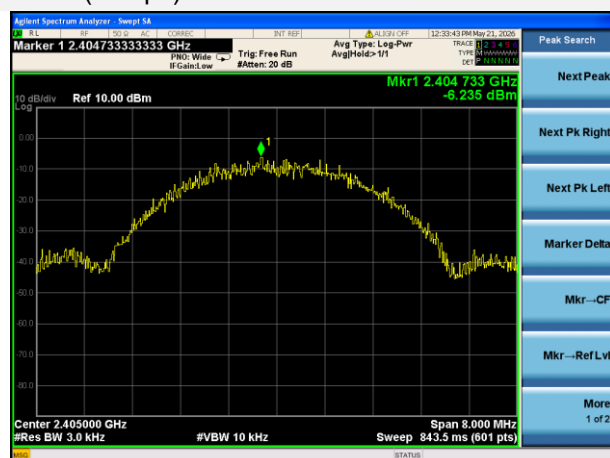
GFSK (4Mbps) LOW CHANNEL
