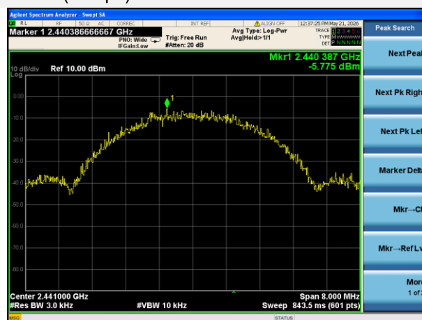
GFSK (4Mbps) MIDDLE CHANNEL
