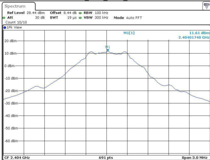
2.4G custom_Ant2_2404_0~Reference
