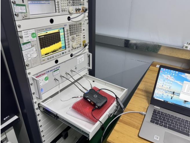
Conducted Measurement
