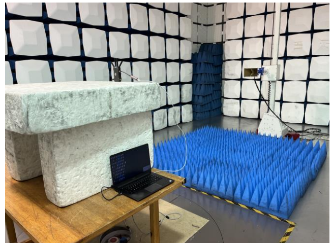
Radiated Spurious Emission Above 1GHz
