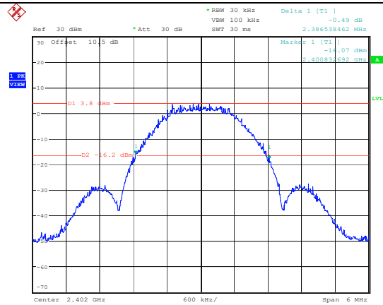
20 dB Bandwidth
