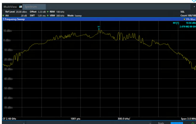
GFSK(2M) on Channel 39
