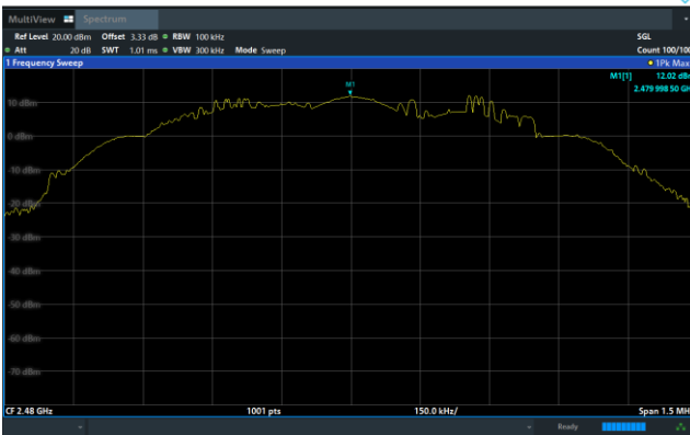
GFSK(1M) on Channel 39
