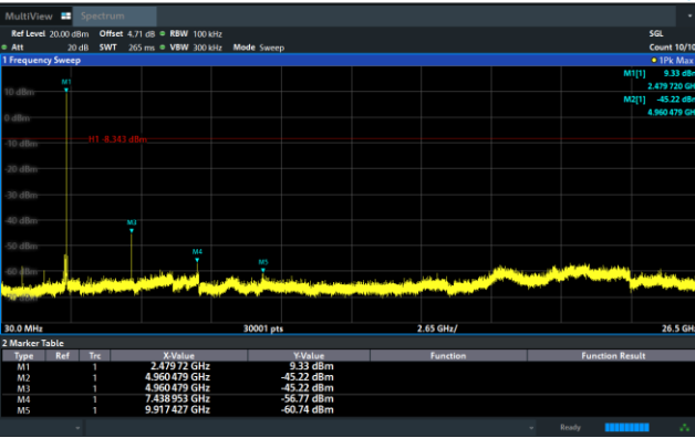
GFSK(2M) on Channel 39
