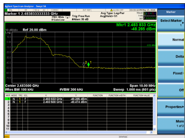
GFSK (2Mbps) HIGH CHANNEL, BAND EDGE
