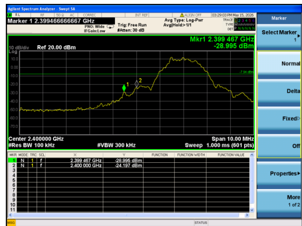
GFSK (2Mbps) LOW CHANNEL, BAND EDGE
