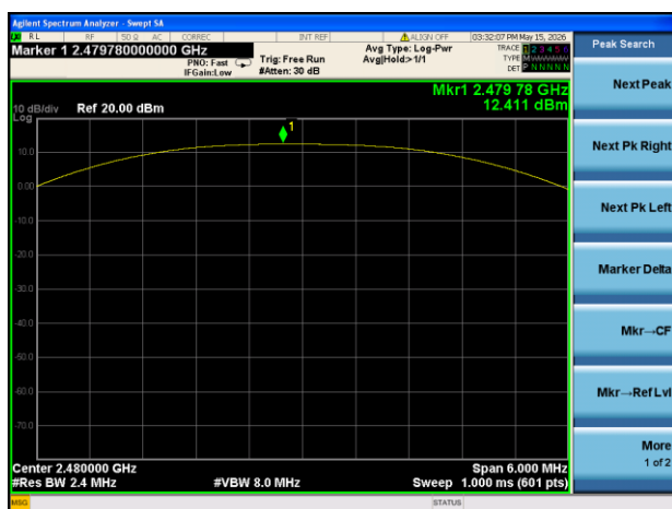
GFSK (2Mbps) HIGH CHANNEL
