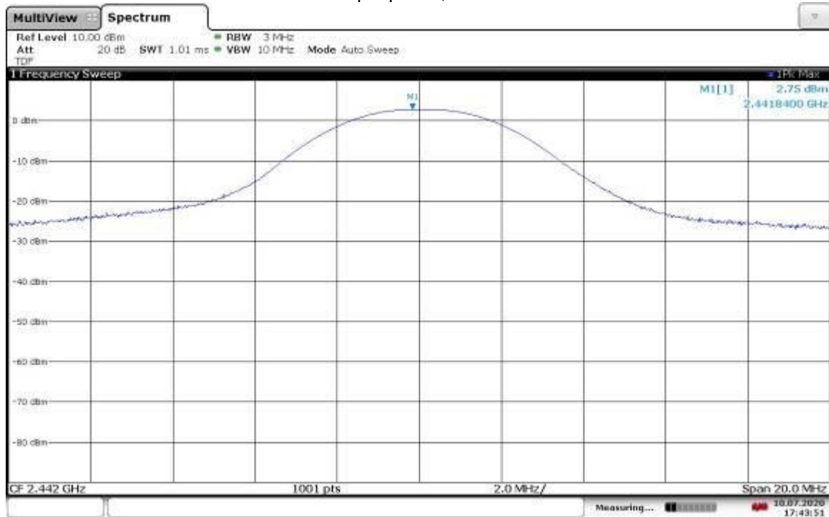
Output power, Mid Ch
