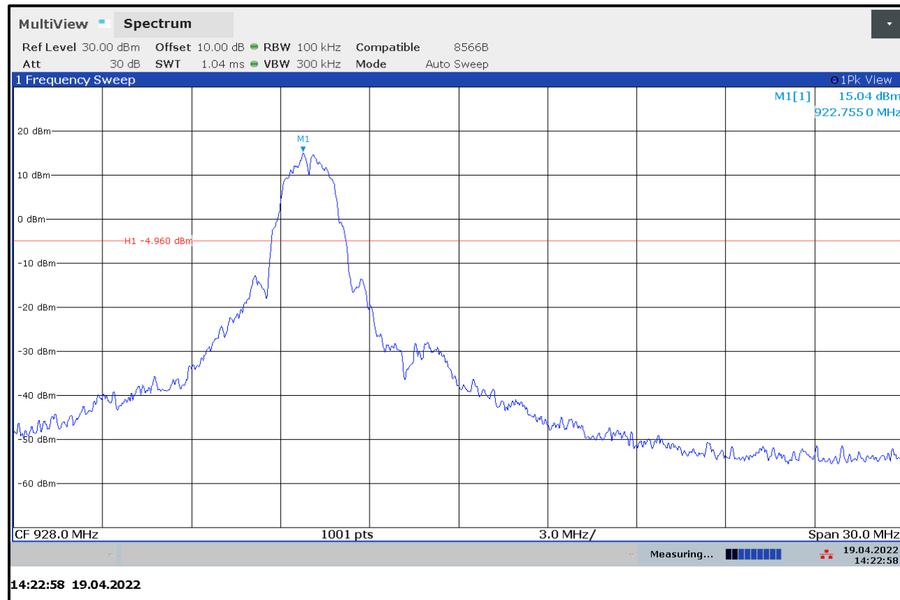
Plot 4-2: Upper Band Edge (928 MHz Band Edge, 923 MHz Carrier) – Port One
