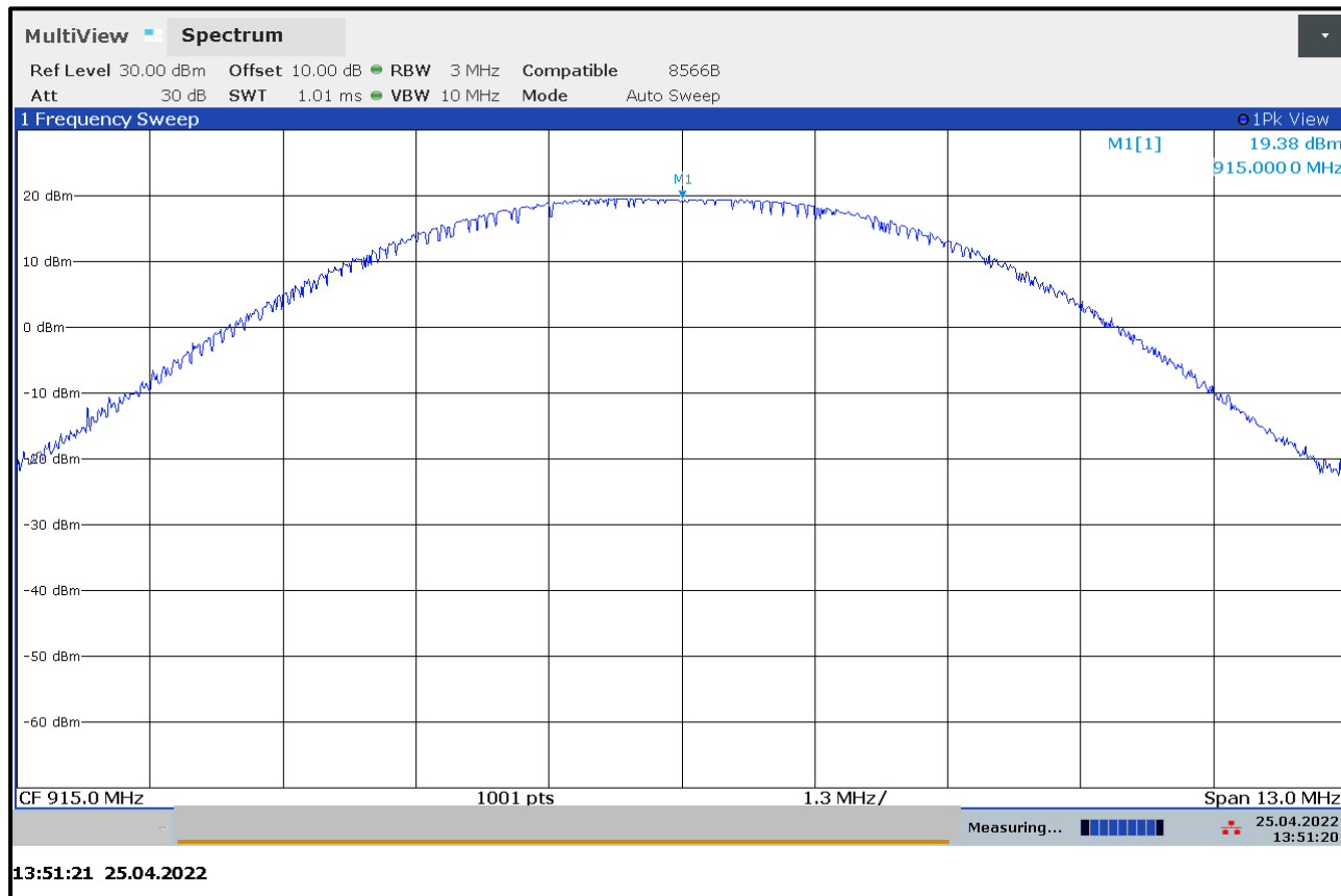
Plot 3-1: Maximum Conducted Output Power (915 MHz) – Port One
