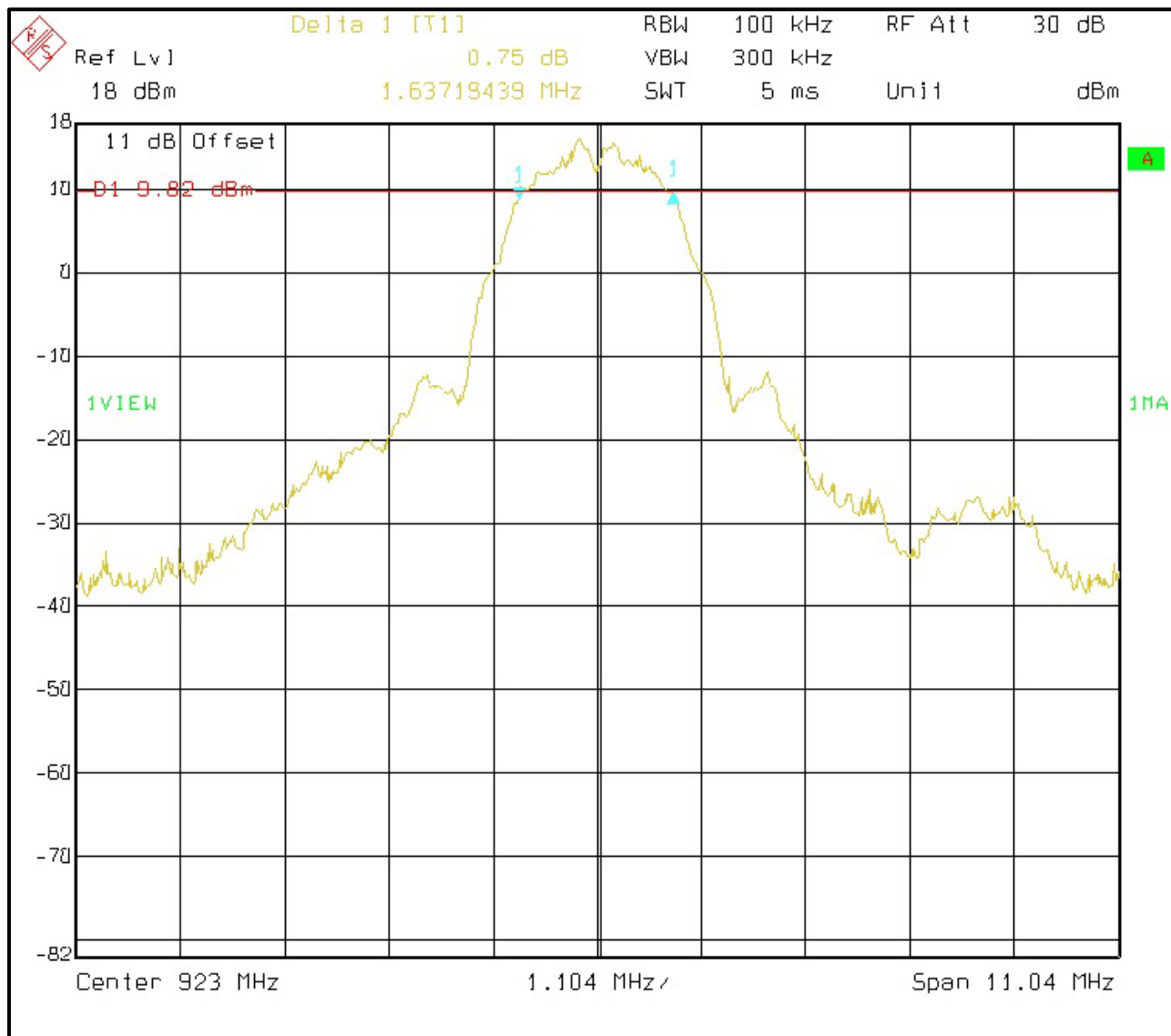
Plot 6-2: 6 dB Bandwidth – 923 MHz – Port One
