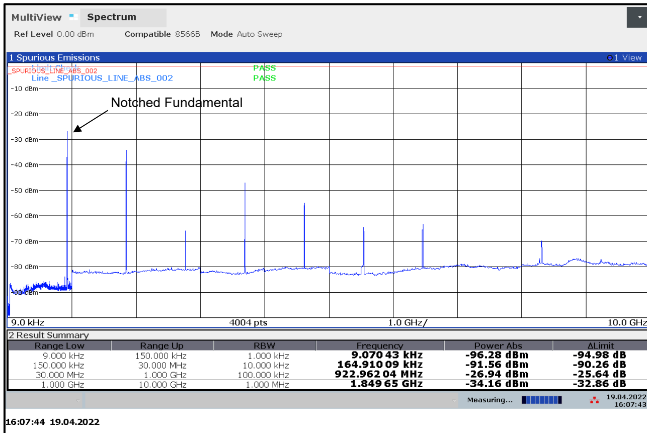
Plot 5-3: Antenna Conducted Spurious Emissions (915 MHz) Port Two
