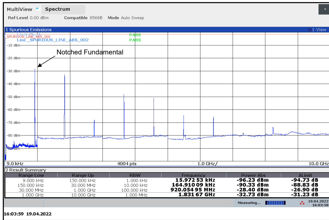
Plot 5-4: Antenna Conducted Spurious Emissions (923 MHz) Port Two
