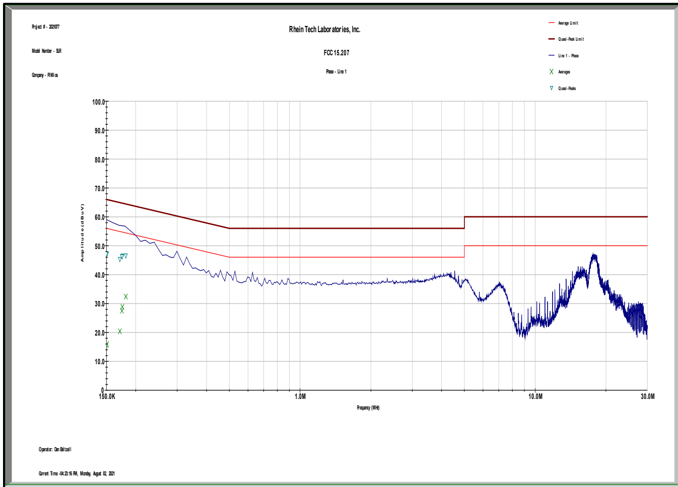
Plot 8-1: Conducted Line Emissions – Phase – Receive Mode
