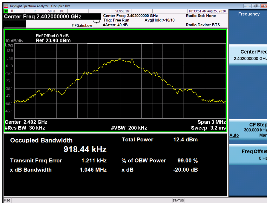
20 dB Bandwidth_DH5_2402
