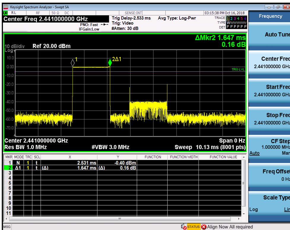
Dwell Time_2DH3_2441
