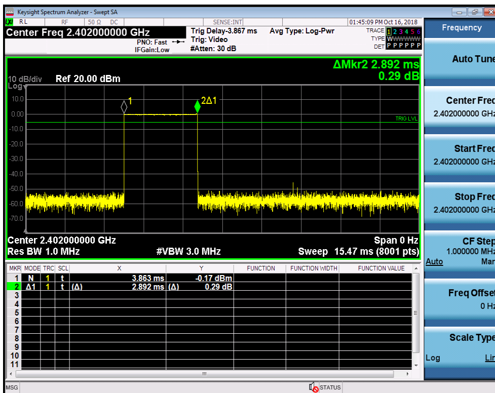
Dwell Time_DH5_2402
