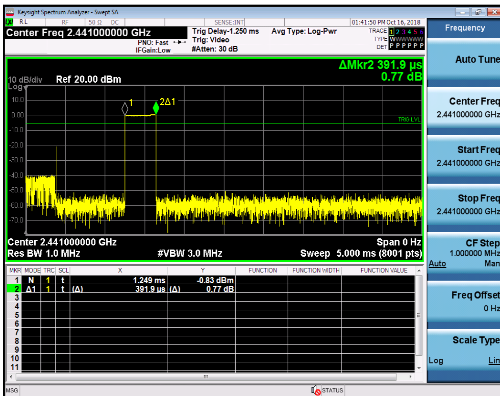
Dwell Time_DH1_2441
