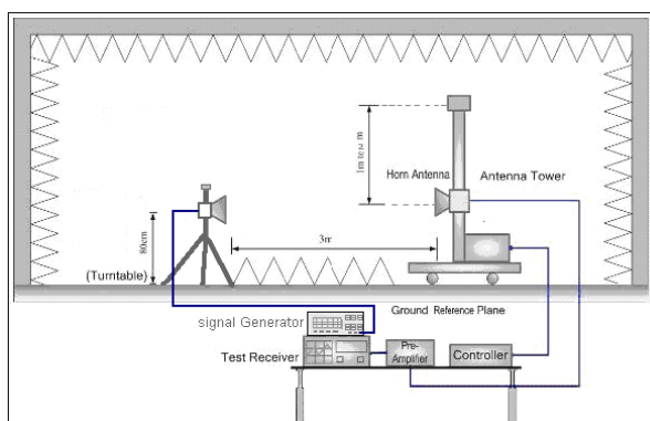
Figure 3. above 1GHz
