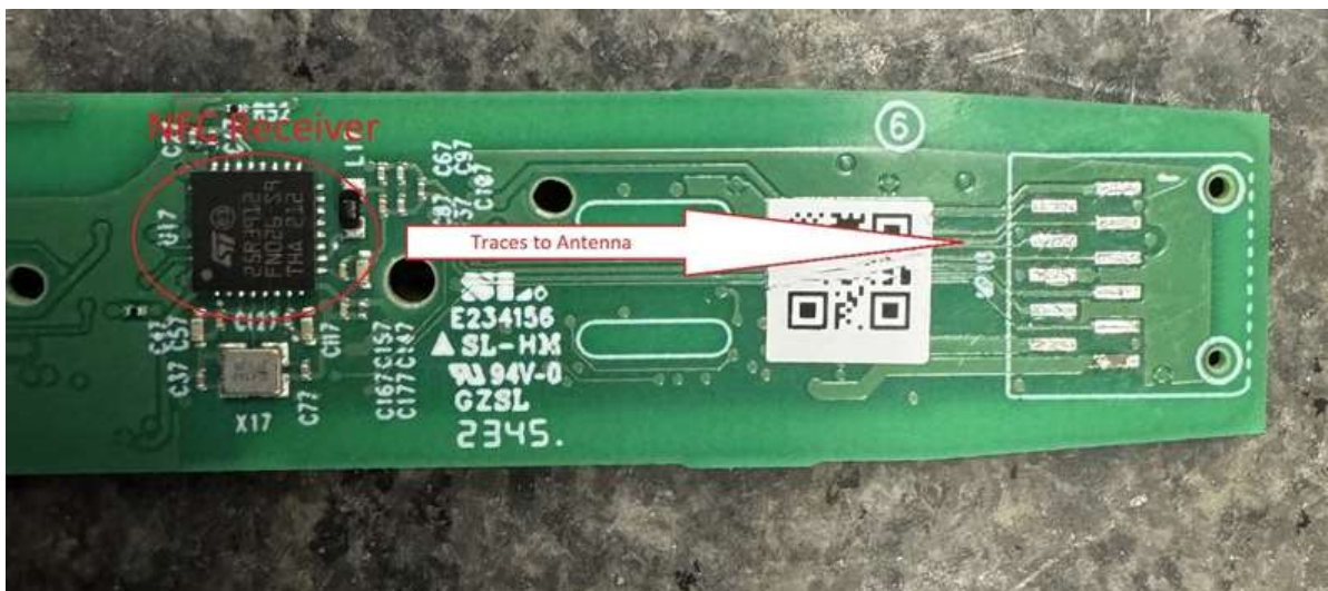
Figure 11: The MCU and BLE antenna are located on the bottom side of the PCB.
