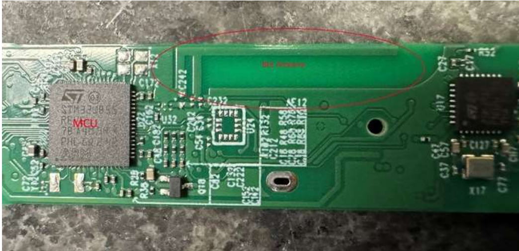
Figure 10: The MCU and BLE antenna are located on the bottom side of the PCB.
