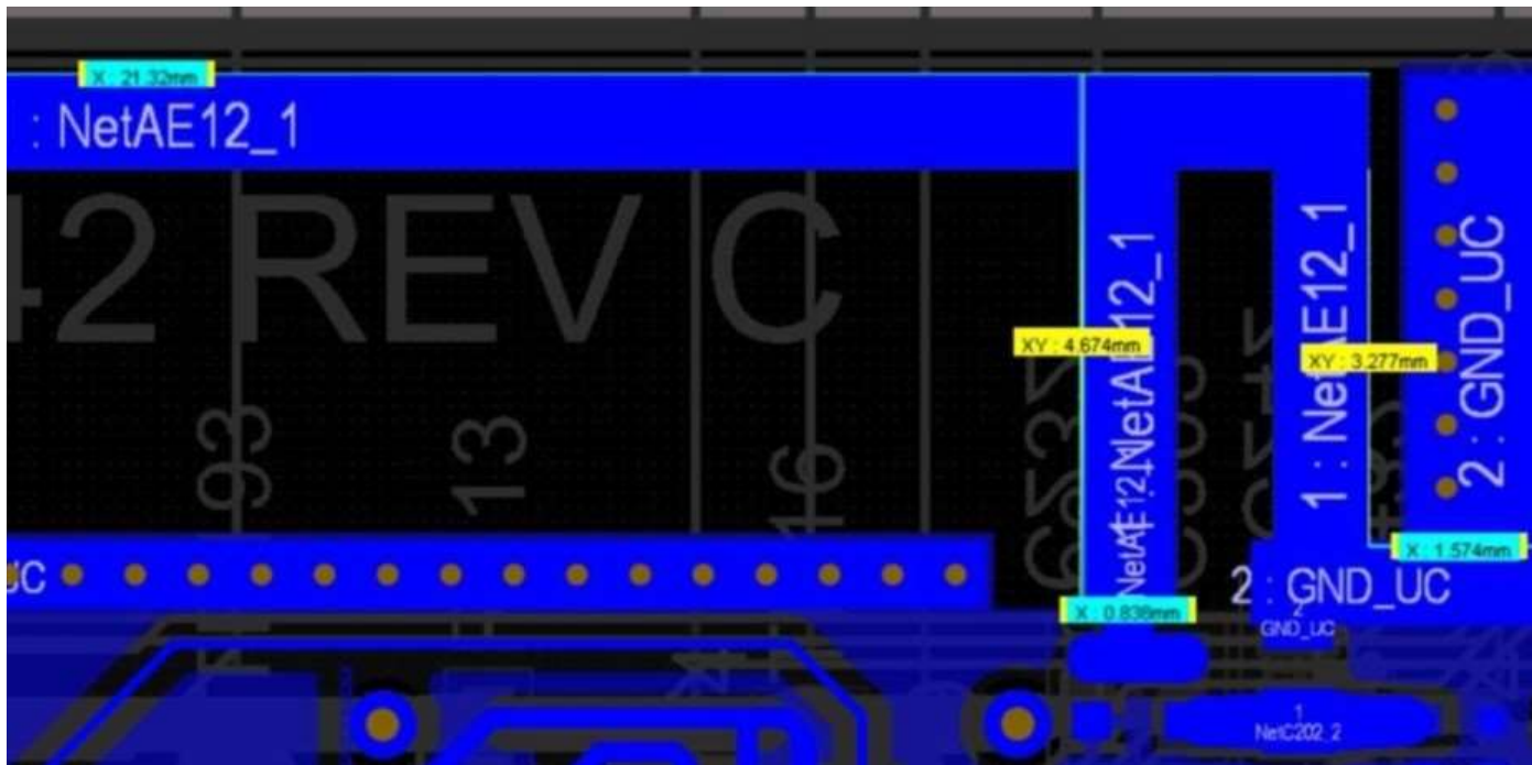
Figure 8: Layout dimensions close up.
