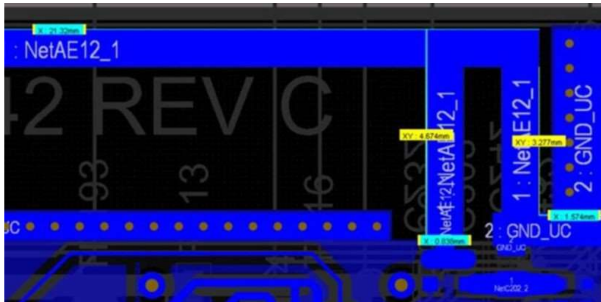
Figure 7: Layout dimensions.
