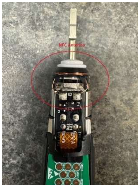
Figure 12: The flex PCB carries the NFC antenna traces from PCB1 to PCB2
