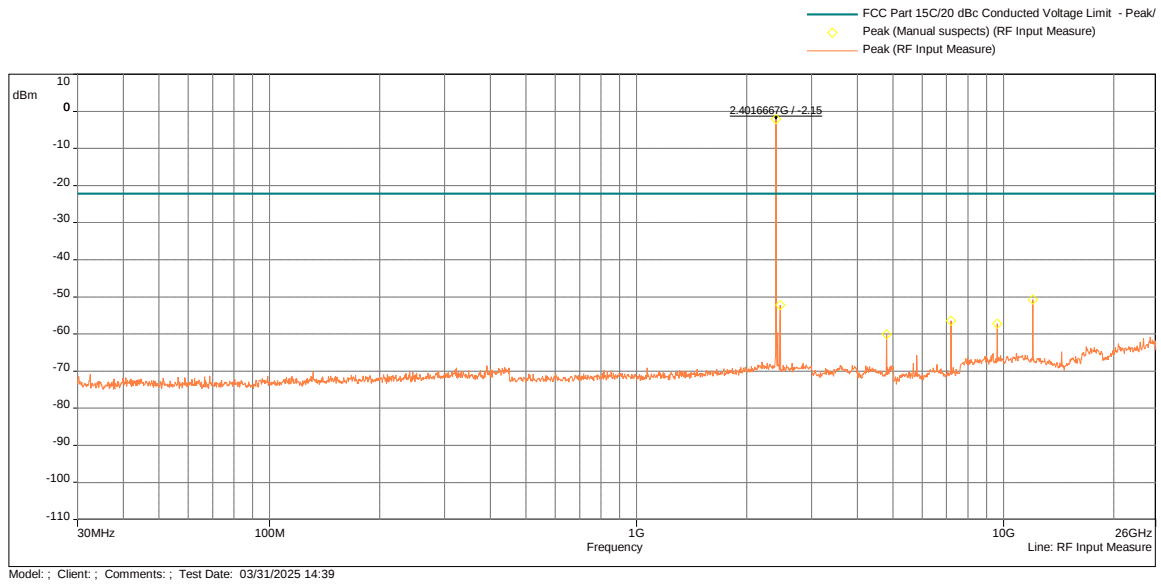
Plot 4.3
