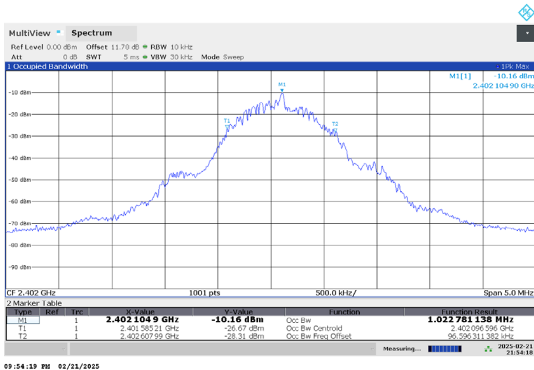
Plot 1.2 – 99% Bandwidth
