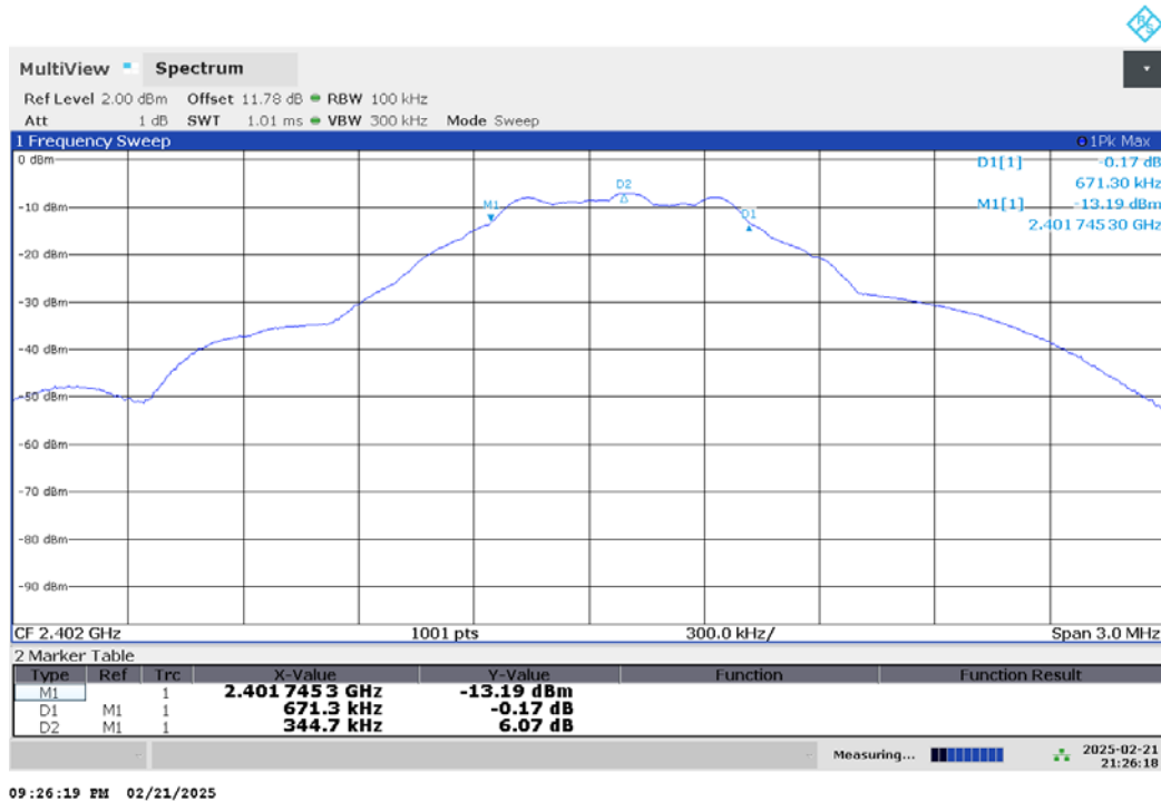
Plot 1.1 – 6dB Bandwidth (FCC)
