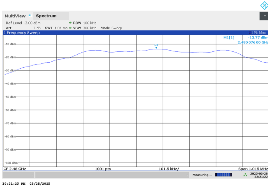
Plot 3. 3
