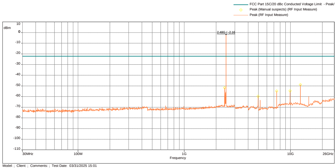
Plot 4.5
