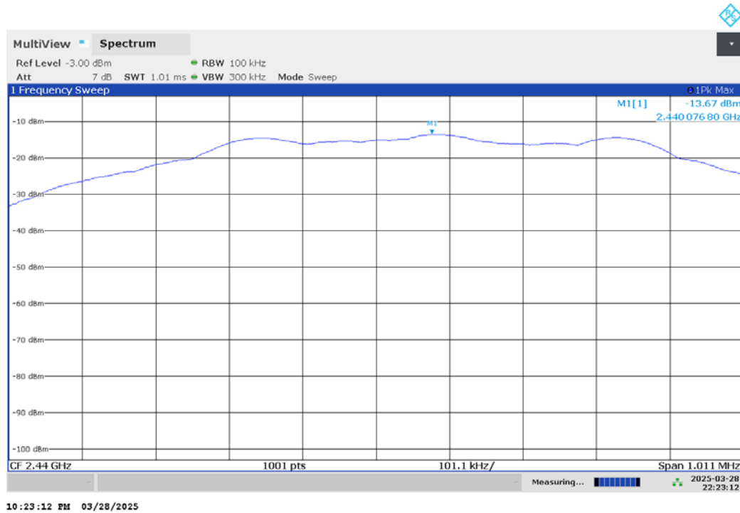
Plot 3. 2
