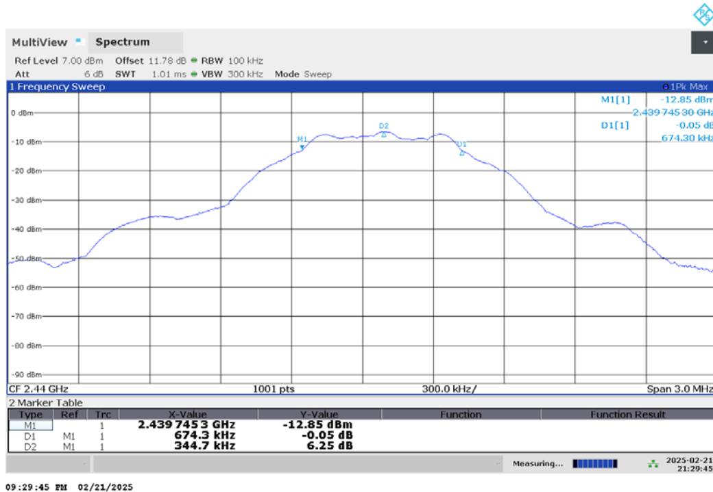
Plot 1.3 – 6dB Bandwidth (FCC)
