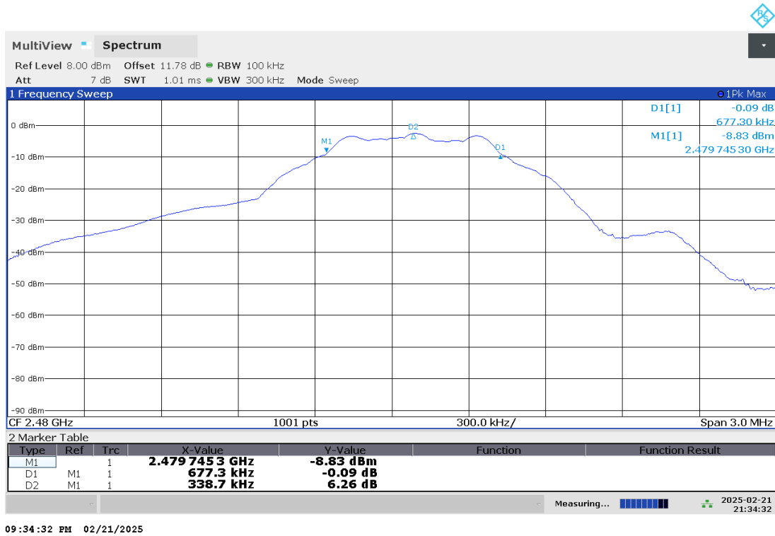
Plot 1.6 – 99% Bandwidth
