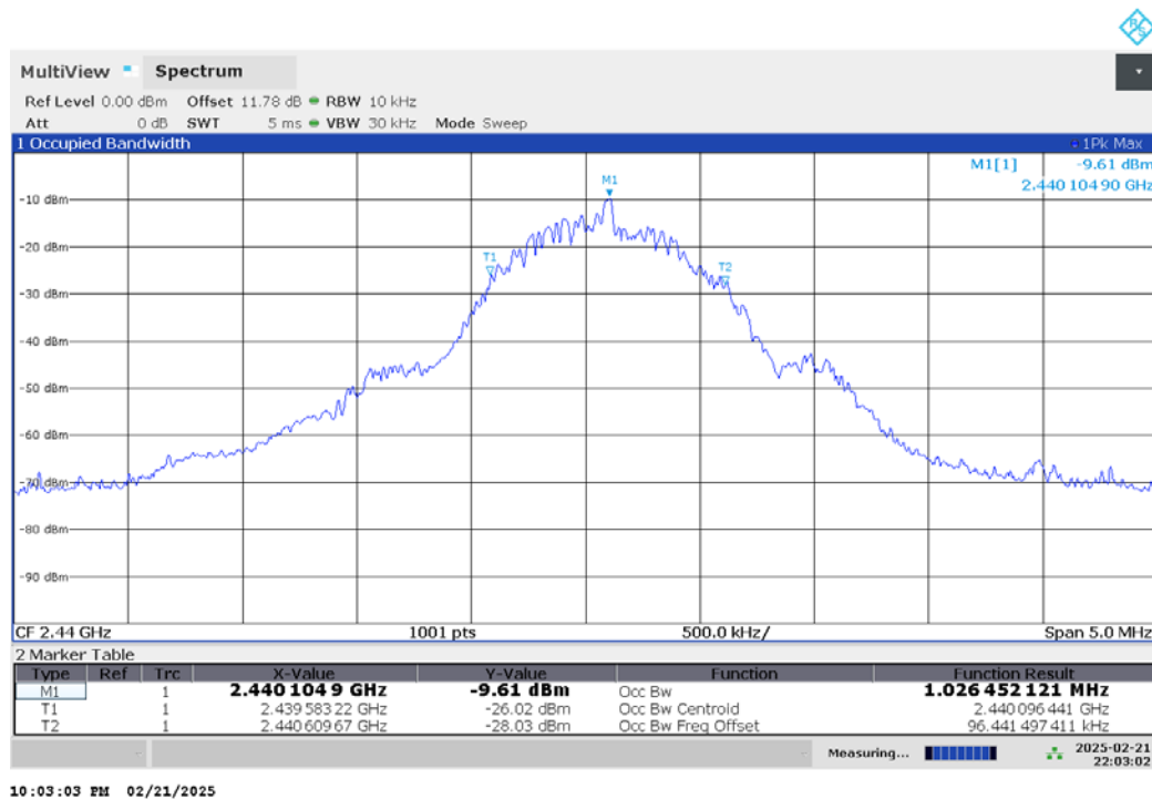
Plot 1.4 – 99% Bandwidth
