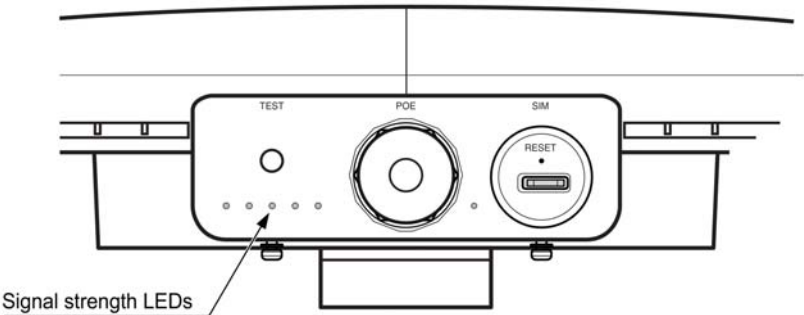
Figure 24 Location of the signal strength LEDs on the High gain CBRS model
