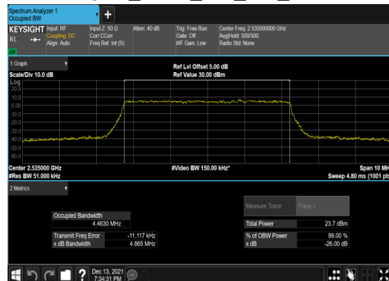
B2_N7(5M)_CP-OFDM_256 QAM_Outer_Full_Mid_CH
