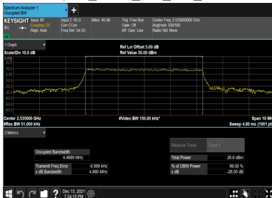
B2_N7(5M)_CP-OFDM_64 QAM_Outer_Full_Mid_CH
