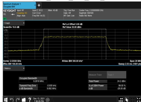
B2_N7(10M)_CP-OFDM_256 QAM_Outer_Full_Mid_CH
