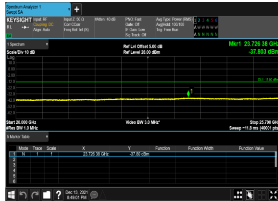
B2_N7(10M)_DFT-s-OFDM_BPSK_Edge_1RB_Left_Low_CH
