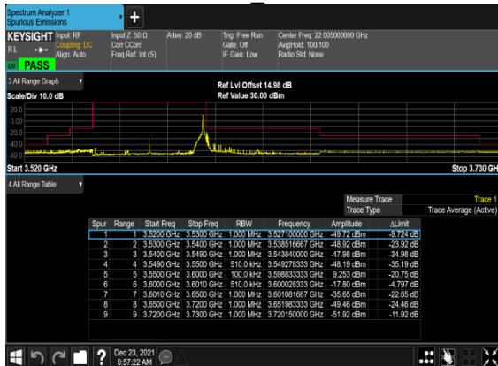
N48(50M)_CP-OFDM_QPSK_Edge_1RB_Right_ Low CH
