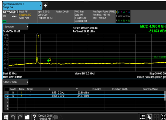
N48(100M)_CP-OFDM_QPSK_Edge_1RB_Right_
