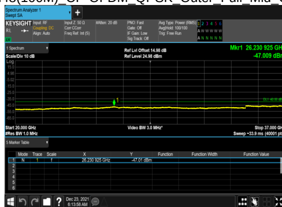
N48(100M)_CP-OFDM_QPSK_Outer_Full_Mid_CH
