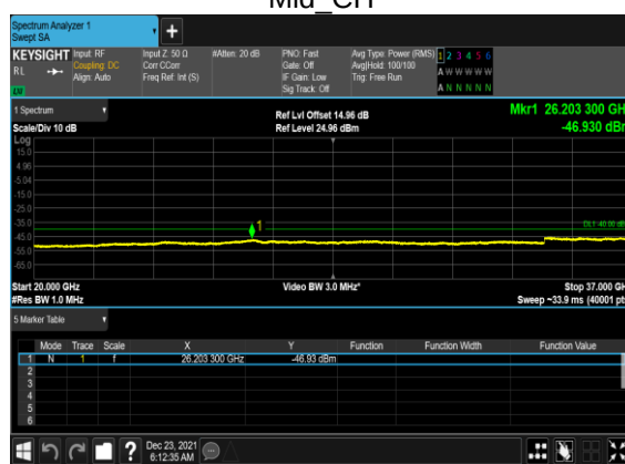
N48(100M)_CP-OFDM_QPSK_Outer_Full_Mid_CH
