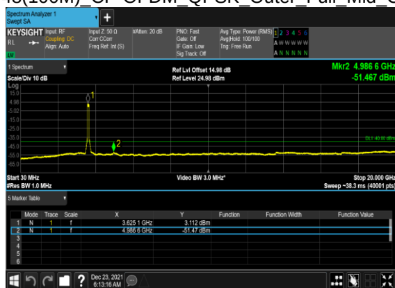
N48(100M)_CP-OFDM_QPSK_Outer_Full_Mid_CH
