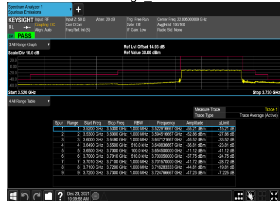
N48(50M)_CP-OFDM_QPSK_Outer_Full_ High CH
