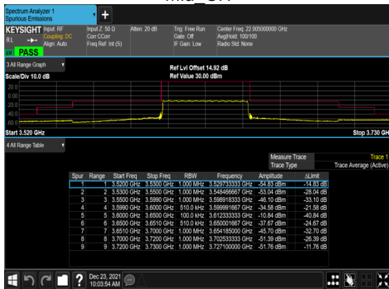
N48(50M)_CP-OFDM_QPSK_Edge_1RB_Right_ High CH
