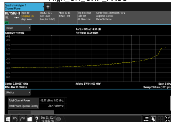
N48(100M)_CP-OFDM_QPSK_Edge_1RB_Left_ High_CH_ CHP_PASS
