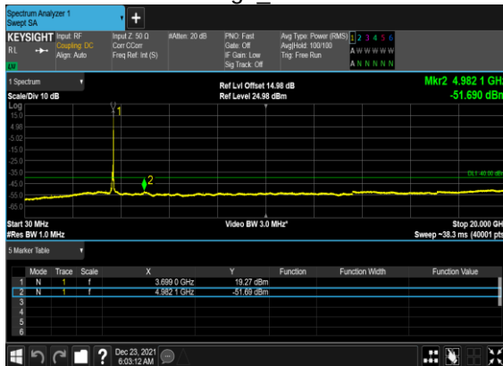
N48(50M)_CP-OFDM_QPSK_Outer_Full_High CH
