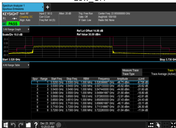
N48(100M)_CP-OFDM_QPSK_Outer_Full_
