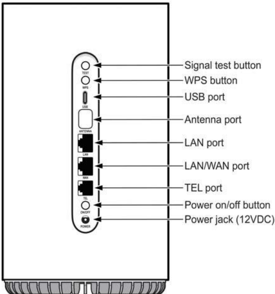
Figure 13 Location of physical interfaces on the side of the Nokia FastMile 5G Gateway 3.2
