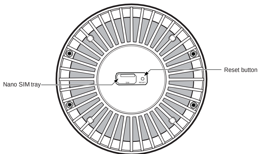
Figure 16 Inserting the SIM card in the Nokia FastMile 5G Gateway 3.2
