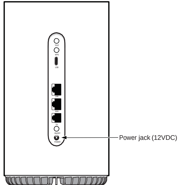
Figure 17 Connecting the power adapter to the Nokia FastMile 5G Gateway 3.2
