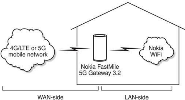
Figure 14 Typical connectivity for the Nokia FastMile 5G Gateway 3.2
