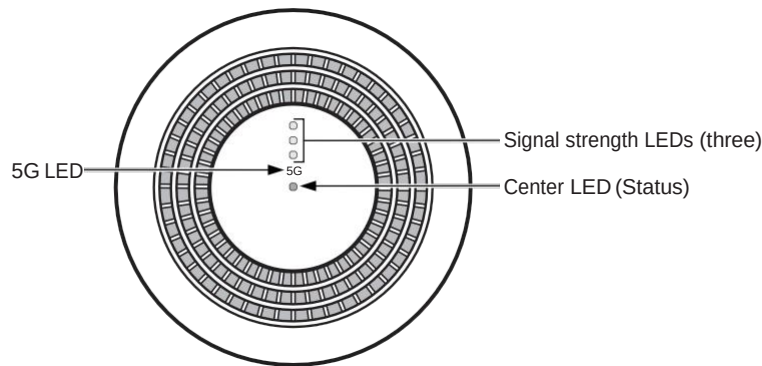
Figure 19 Location of LEDs
