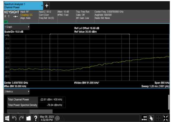
N48(40M)_DFT-s- OFDM_BPSK_Edge_1RB_Left_High_CH_CHP_PASS
