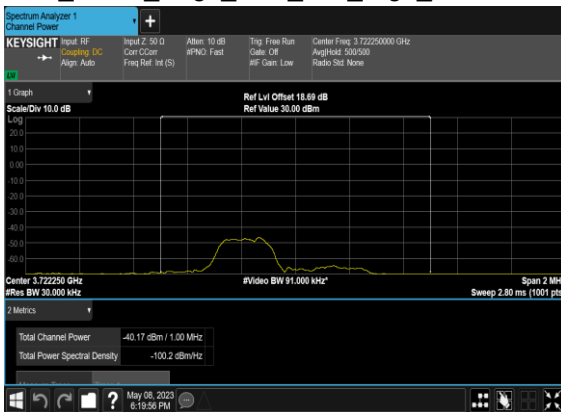
N48(40M)_DFT-s- OFDM_BPSK_Edge_1RB_Left_High_CH_CHP_Pass
