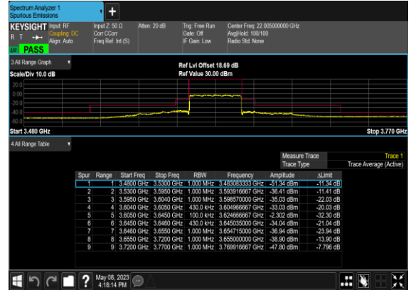
N48(40M)_DFT-s- OFDM_QPSK_Outer_Full_Mid_CH
