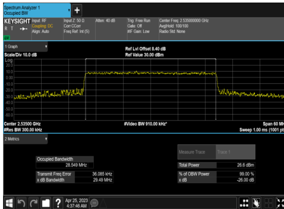
B2_N7(30M)_CP- OFDM_QPSK_Outer_Full_531000_CH
