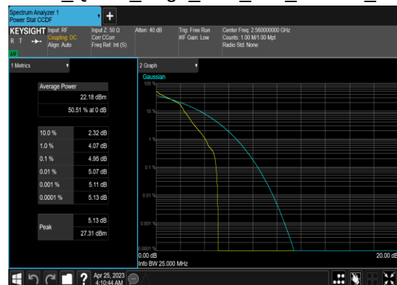
B2_N7(20M)_DFT-s-OFDM_QPSK_Edge_1RB_Left_536000_CH
