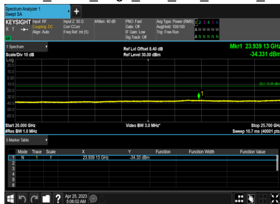
B2_N7(20M)_DFT-s- OFDM_BPSK_Edge_1RB_Left_531000_CH
