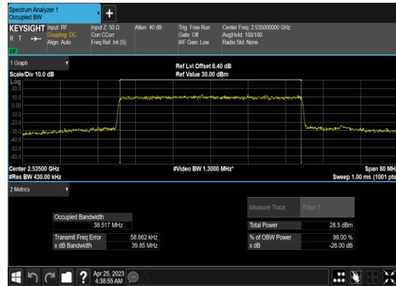
B2_N7(40M)_DFT-s- OFDM_QPSK_Outer_Full_531000_CH
