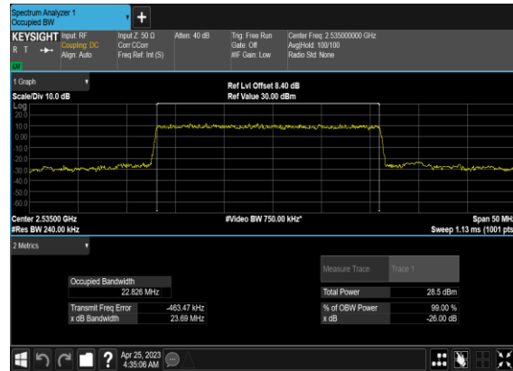
B2_N7(25M)_DFT-s- OFDM_QPSK_Outer_Full_531000_CH
