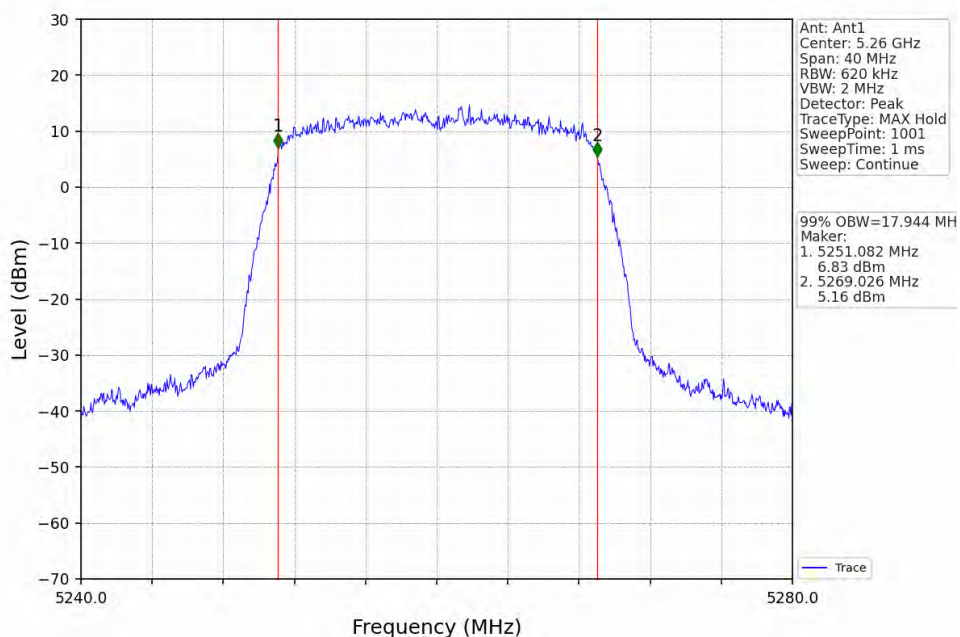
802.11ac(VHT20)_LCH_5260MHz_Ant1_NTNV
