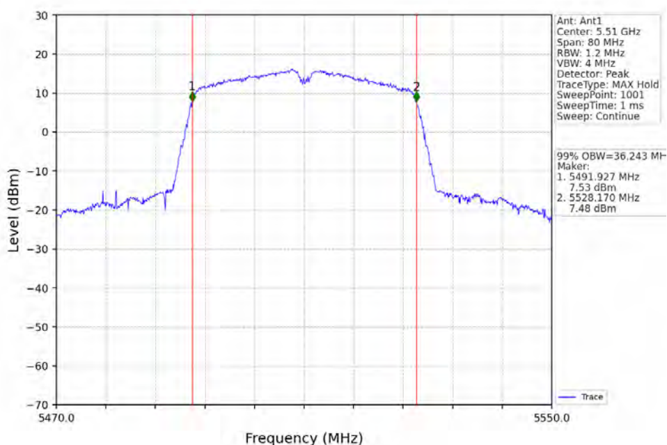
802.11ac(VHT40)_LCH_5510MHz_Ant1_NTNV
