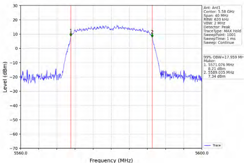
802.11ac(VHT20)_MCH_5580MHz_Ant1_NTNV
