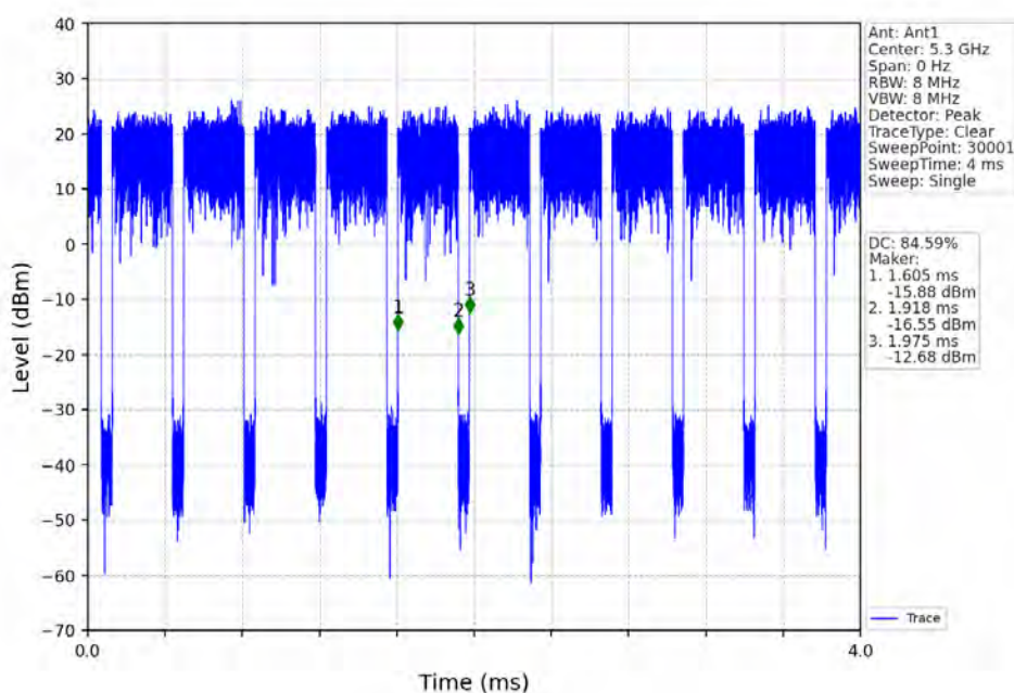
802.11ax(HEW20)_MCH_5300MHz_RU242_Left_Ant1_NTNV
