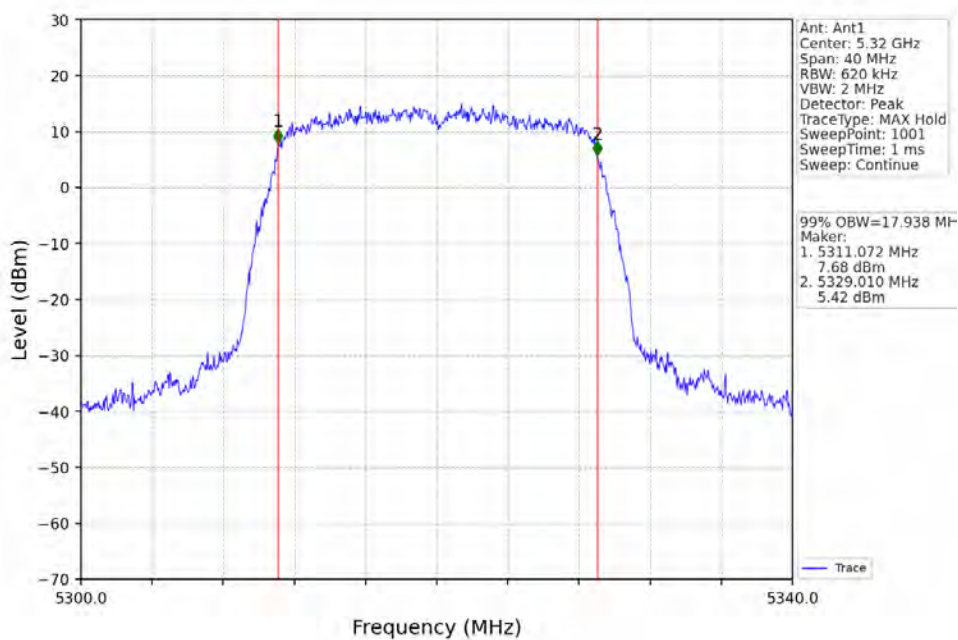
802.11ac(VHT20)_HCH_5320MHz_Ant1_NTNV
