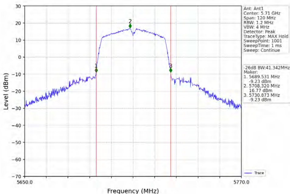
802.11ac(VHT40)_HCH_5710MHz_Ant1_NTNV
