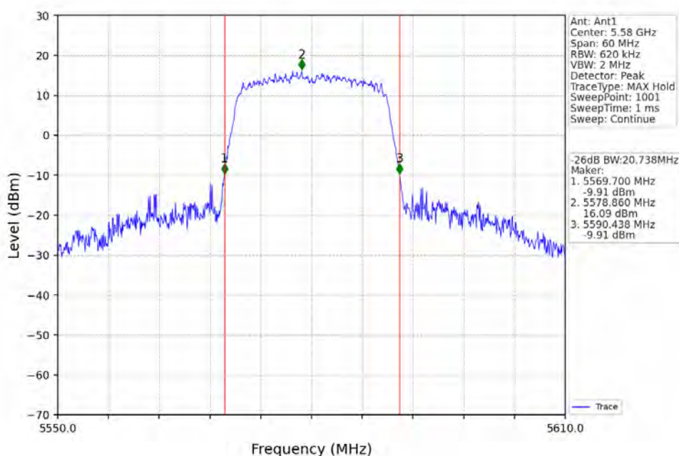
802.11ac(VHT20)_MCH_5580MHz_Ant1_NTNV
