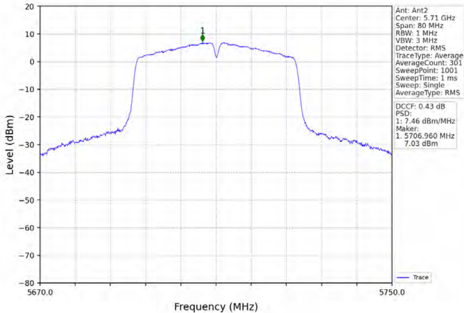
802.11n(HT40)_HCH_5710MHz_MIMO_NTNV
