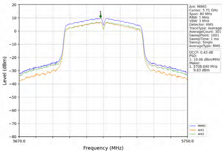
802.11n(HT40)_HCH_5710MHz_MIMO_NTNV
