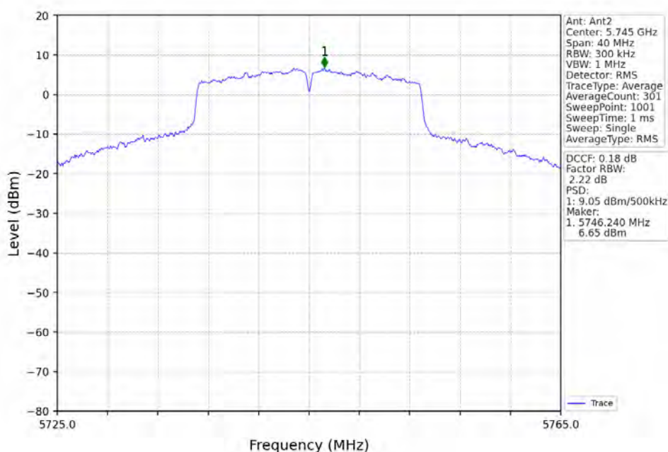
802.11ac(VHT20)_LCH_5745MHz_Ant2_NTNV
