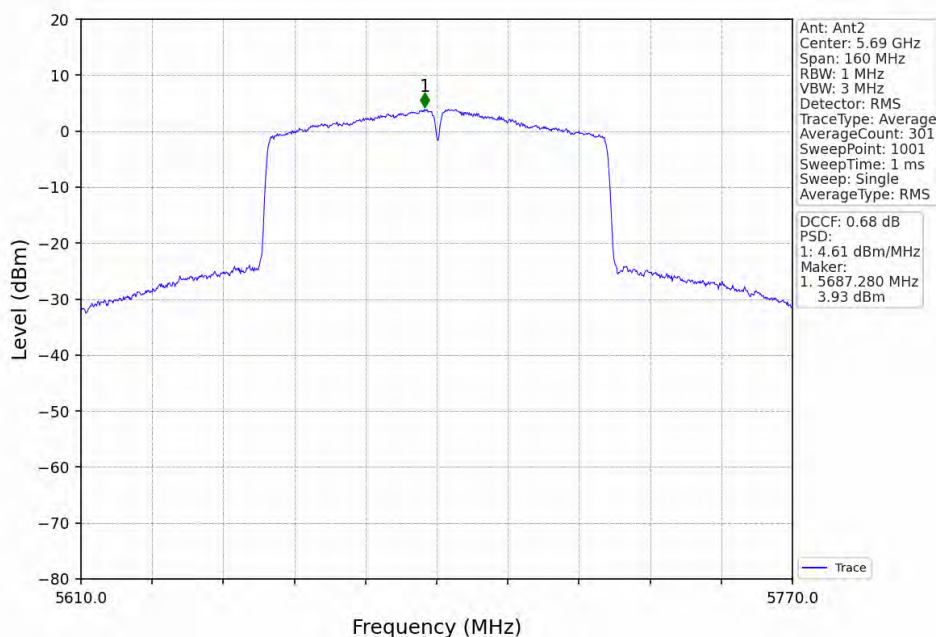
802.11ac(VHT80)_HCH_5690MHz_Ant2_NTNV
