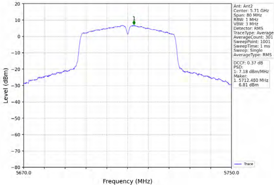
802.11ac(VHT40)_HCH_5710MHz_MIMO_NTNV
