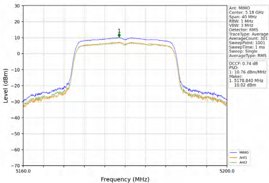
802.11ax(HEW20)_LCH_5180MHz_RU242_Left_MIMO_NTNV
