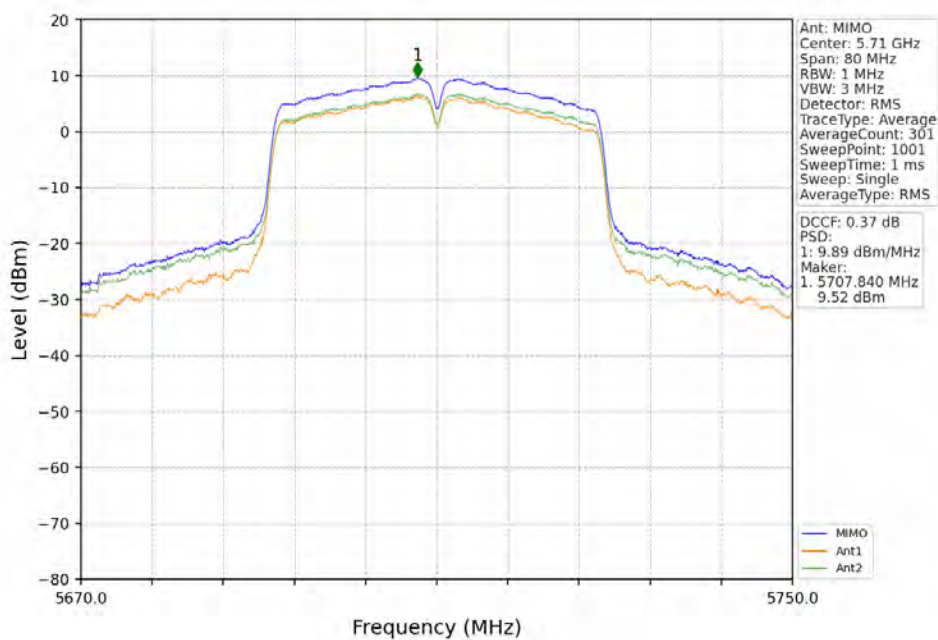
802.11ac(VHT40)_HCH_5710MHz_MIMO_NTNV
