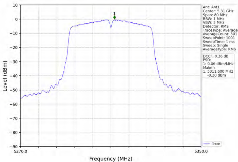
802.11ac(VHT40)_HCH_5310MHz_Ant1_NTNV
