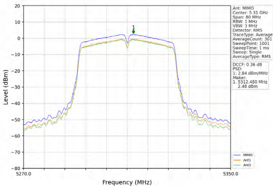
802.11ac(VHT40)_HCH_5310MHz_MIMO_NTNV
