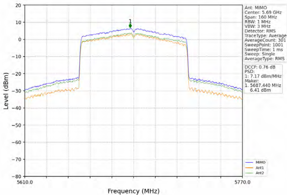
802.11ax(HEW80)_HCH_5690MHz_RU996_Left_MIMO_NTNV
