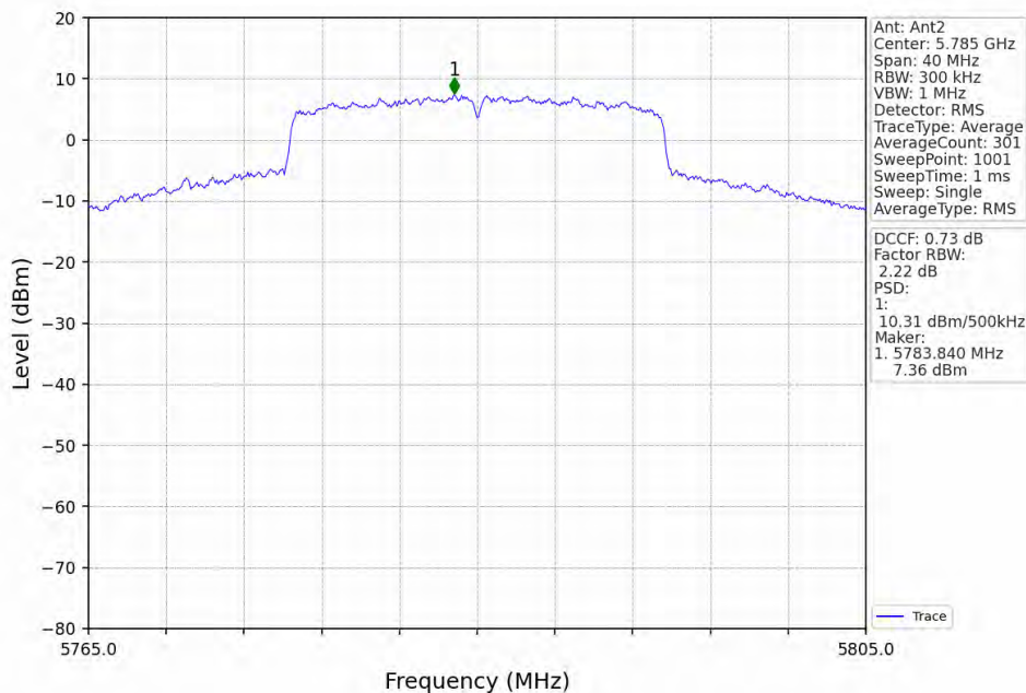
802.11ax(HEW20)_MCH_5785MHz_RU242_Left_MIMO_NTNV
