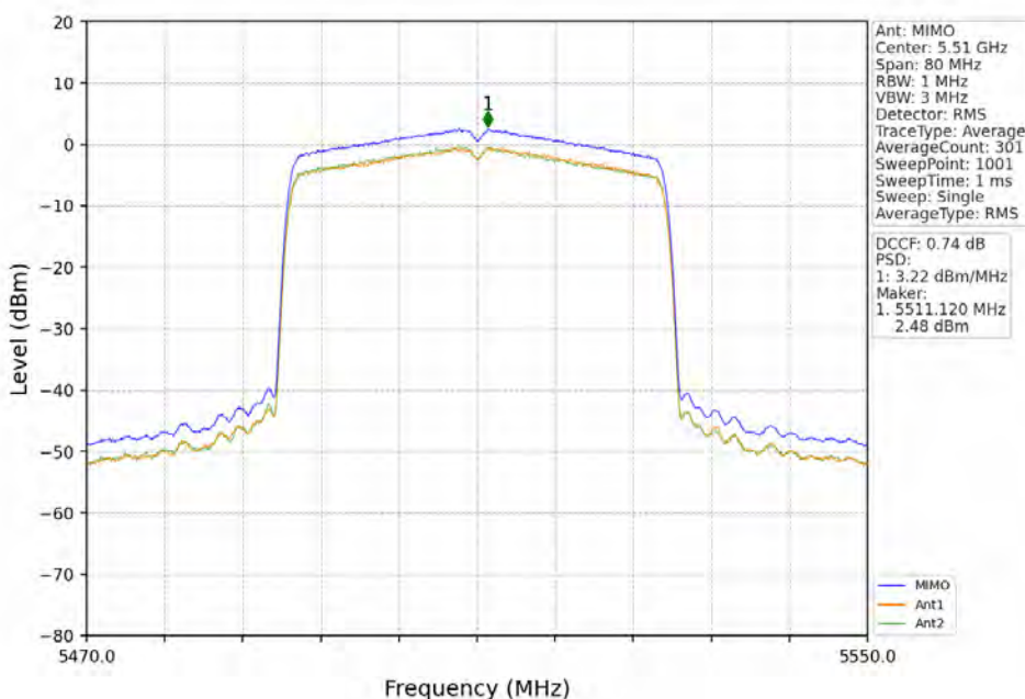
802.11ax(HEW40)_LCH_5510MHz_RU484_Left_MIMO_NTNV
