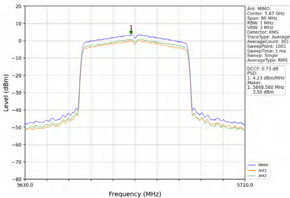
802.11ax(HEW40)_HCH_5670MHz_RU484_Left_MIMO_NTNV
