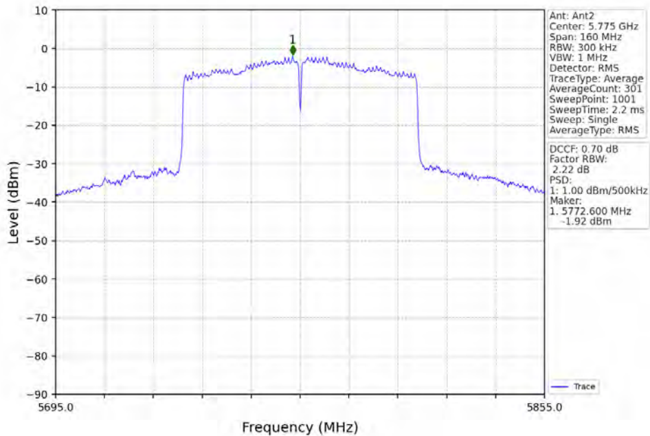
802.11ac(VHT80)_MCH_5775MHz_MIMO_NTNV
