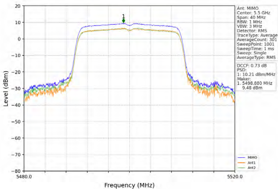
802.11ax(HEW20)_LCH_5500MHz_RU242_Left_MIMO_NTNV
