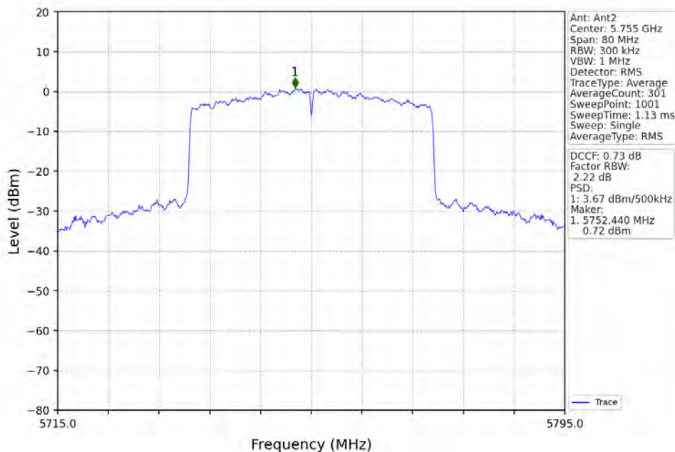
802.11ax(HEW40)_LCH_5755MHz_RU484_Left_MIMO_NTNV
