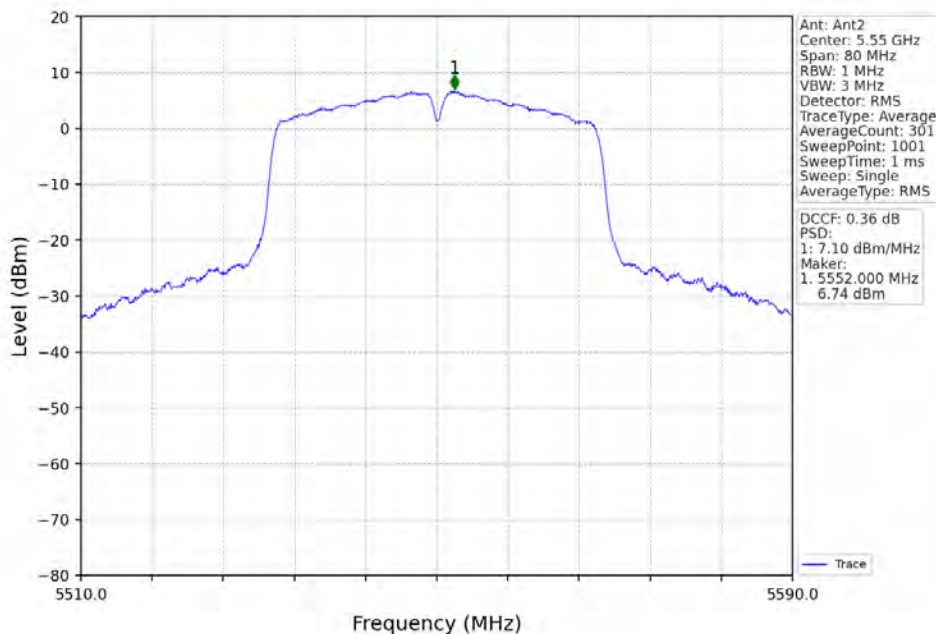
802.11ac(VHT40)_MCH_5550MHz_MIMO_NTNV
