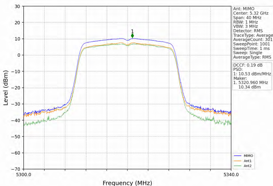
802.11ac(VHT20)_HCH_5320MHz_MIMO_NTNV
