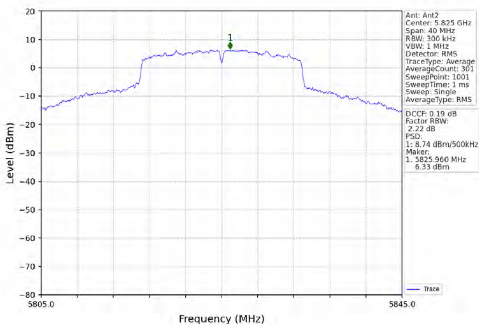
802.11ac(VHT20)_HCH_5825MHz_Ant2_NTNV
