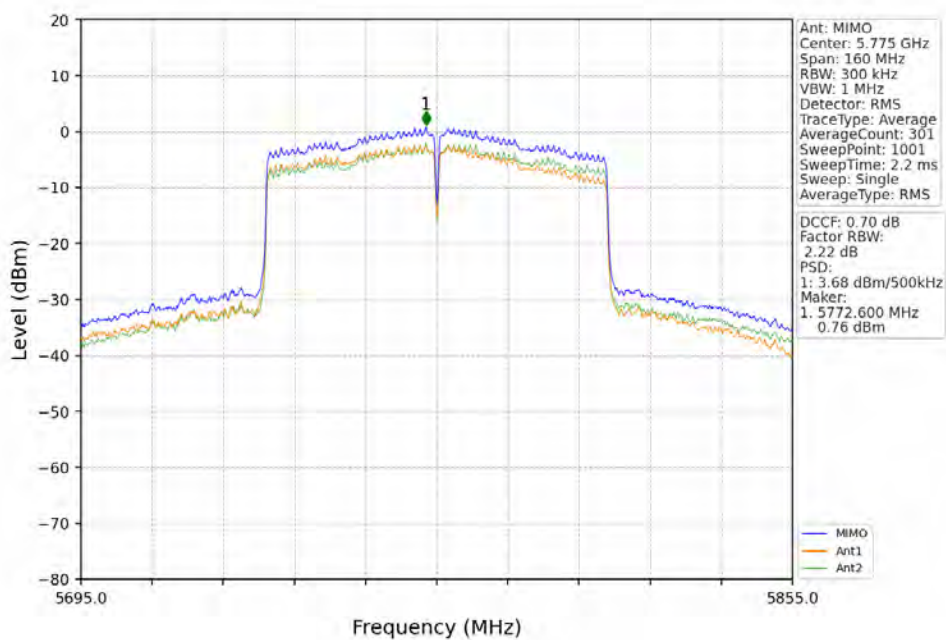
802.11ac(VHT80)_MCH_5775MHz_MIMO_NTNV
