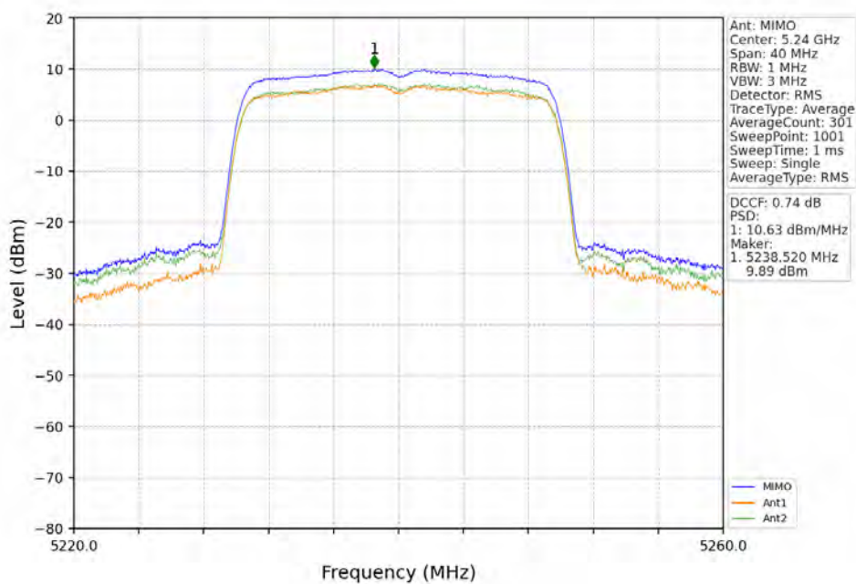
802.11ax(HEW20)_HCH_5240MHz_RU242_Left_MIMO_NTNV
