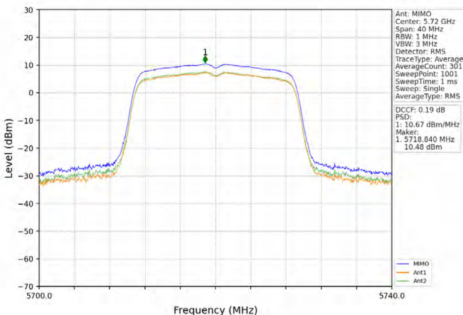
802.11ac(VHT20)_HCH_5720MHz_MIMO_NTNV
