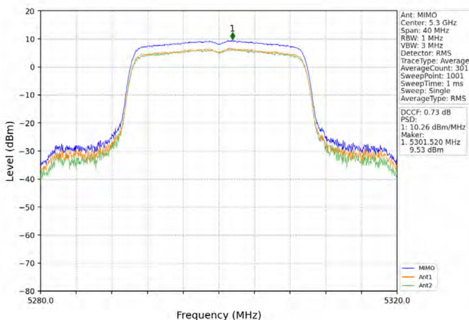
802.11ax(HEW20)_MCH_5300MHz_RU242_Left_MIMO_NTNV
