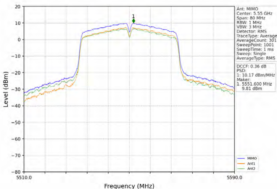
802.11ac(VHT40)_MCH_5550MHz_MIMO_NTNV
