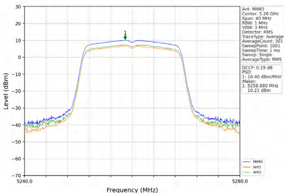
802.11ac(VHT20)_LCH_5260MHz_MIMO_NTNV
