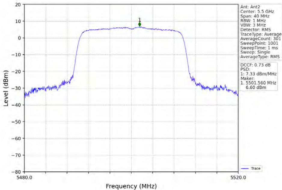
802.11ax(HEW20)_LCH_5500MHz_RU242_Left_MIMO_NTNV
