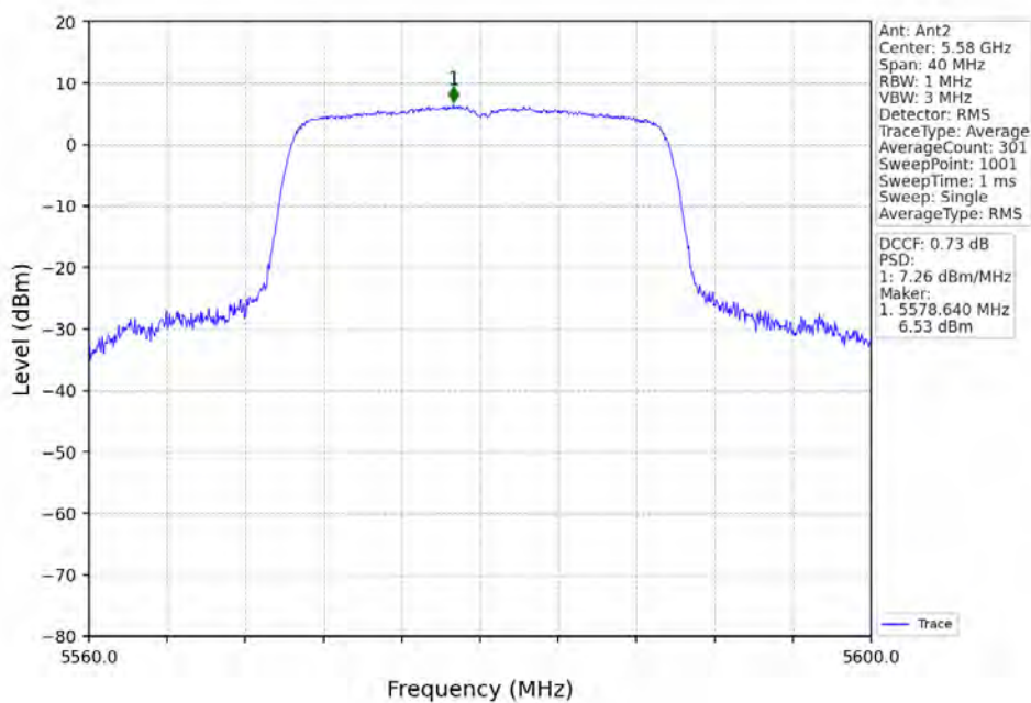
802.11ax(HEW20)_MCH_5580MHz_RU242_Left_Ant2_NTNV
