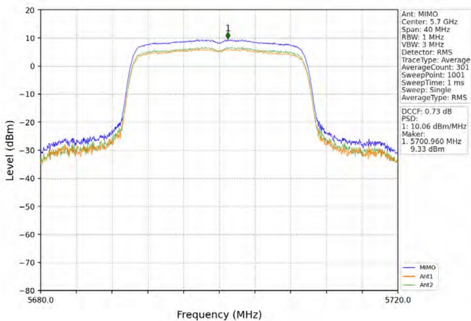
802.11ax(HEW20)_HCH_5700MHz_RU242_Left_MIMO_NTNV
