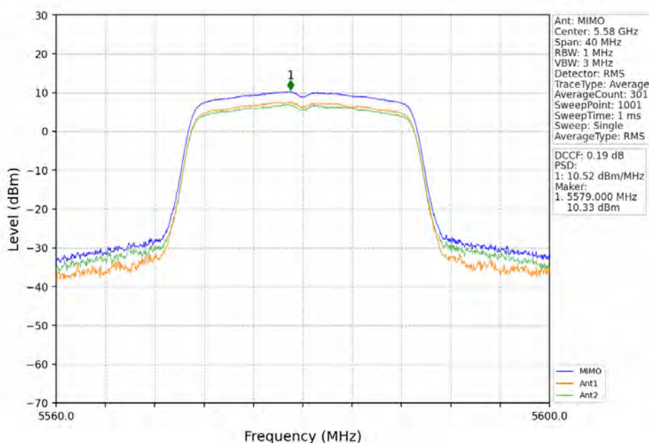
802.11ac(VHT20)_MCH_5580MHz_MIMO_NTNV
