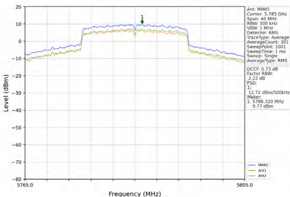
802.11ax(HEW20)_MCH_5785MHz_RU242_Left_MIMO_NTNV
