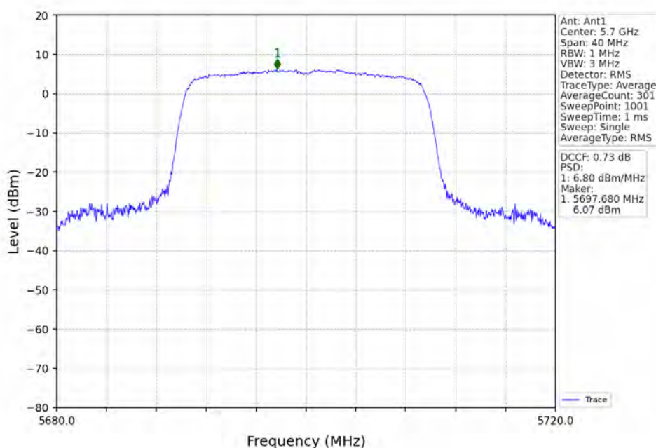
802.11ax(HEW20)_HCH_5700MHz_RU242_Left_Ant1_NTNV
