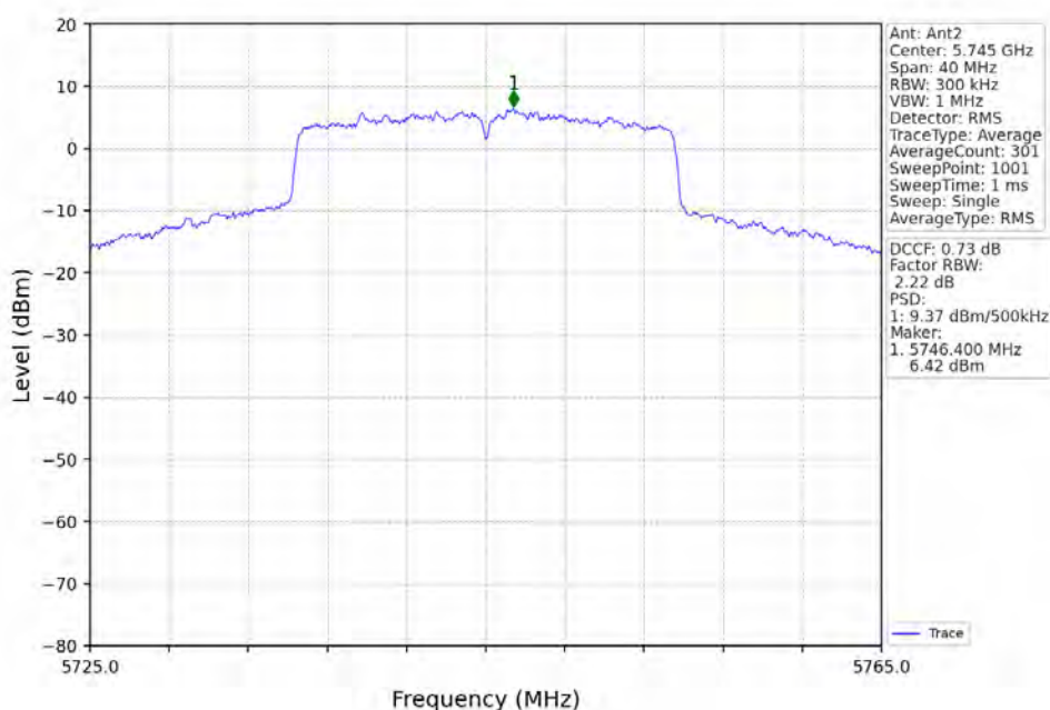
802.11ax(HEW20)_LCH_5745MHz_RU242_Left_Ant2_NTNV
