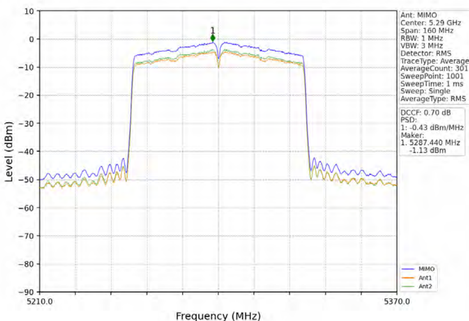
802.11ac(VHT80)_MCH_5290MHz_MIMO_NTNV
