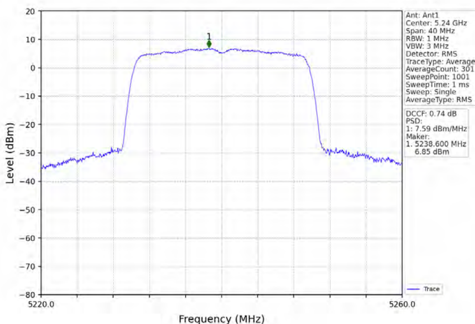
802.11ax(HEW20)_HCH_5240MHz_RU242_Left_Ant1_NTNV
