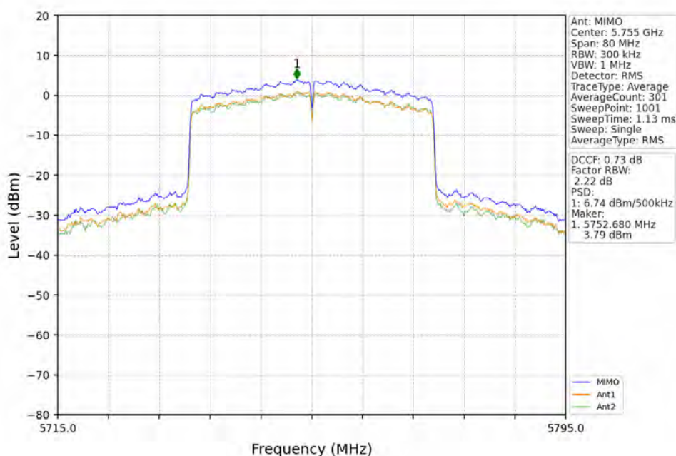
802.11ax(HEW40)_LCH_5755MHz_RU484_Left_MIMO_NTNV
