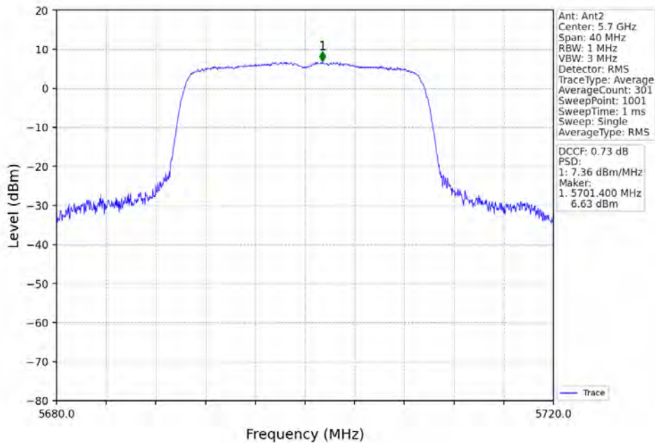
802.11ax(HEW20)_HCH_5700MHz_RU242_Left_MIMO_NTNV
