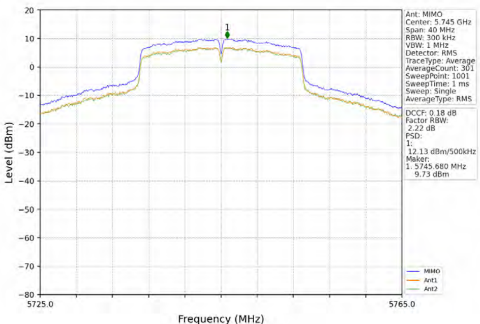
802.11n(HT20)_LCH_5745MHz_MIMO_NTNV
