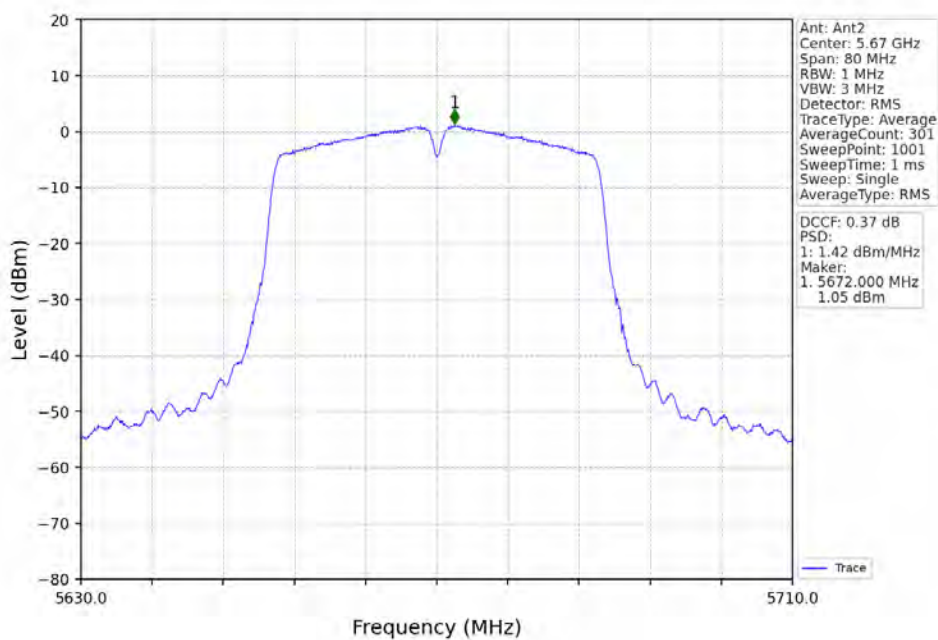
802.11ac(VHT40)_HCH_5670MHz_Ant2_NTNV
