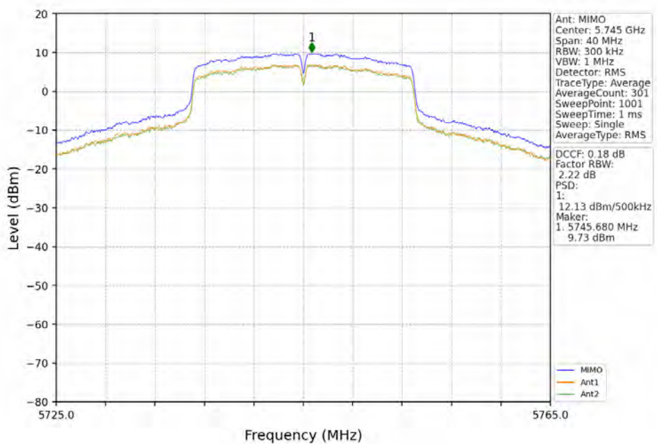
802.11n(HT20)_LCH_5745MHz_MIMO_NTNV
