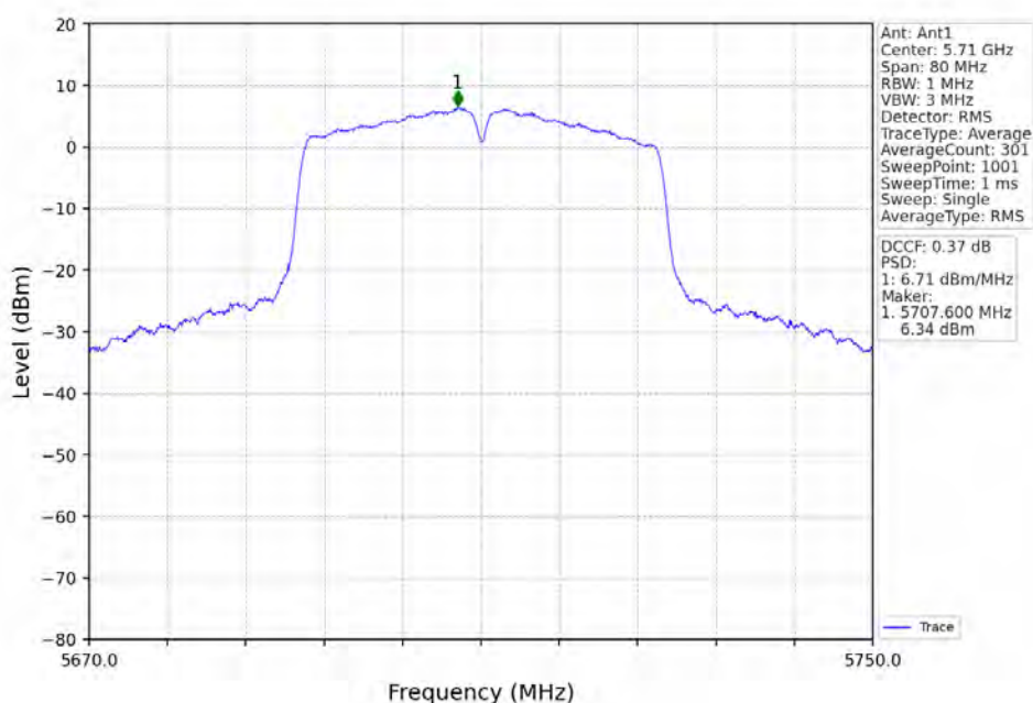
802.11ac(VHT40)_HCH_5710MHz_Ant1_NTNV
