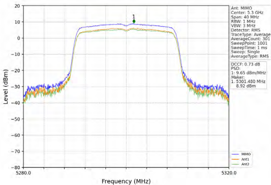
802.11ax(HEW20)_MCH_5300MHz_RU242_Left_MIMO_NTNV
