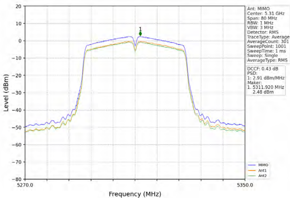
802.11n(HT40)_HCH_5310MHz_MIMO_NTNV
