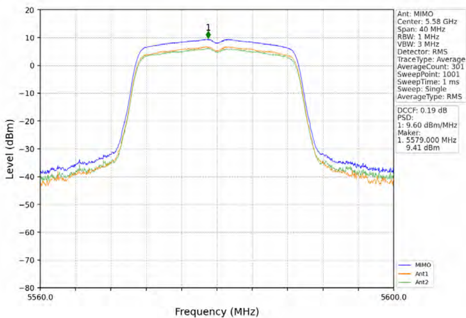
802.11ac(VHT20)_MCH_5580MHz_MIMO_NTNV
