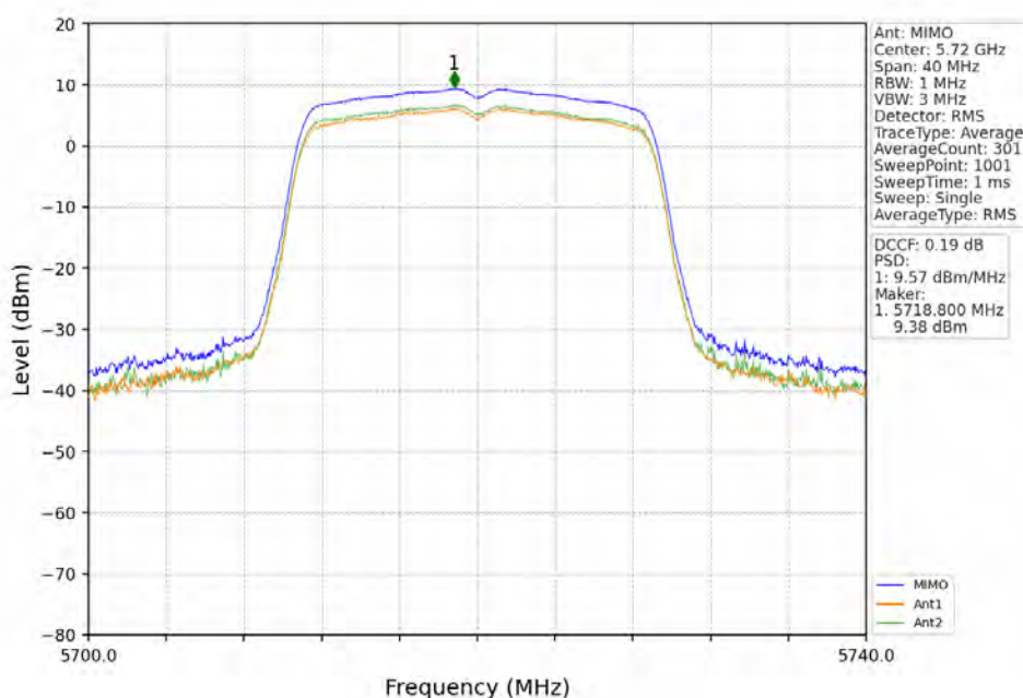
802.11ac(VHT20)_HCH_5720MHz_MIMO_NTNV
