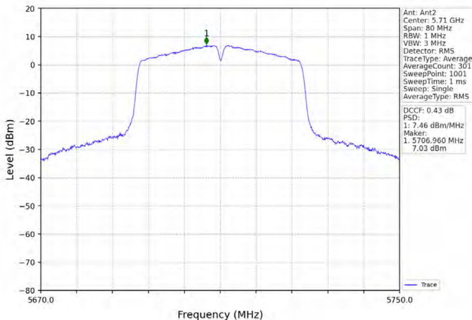
802.11n(HT40)_HCH_5710MHz_MIMO_NTNV
