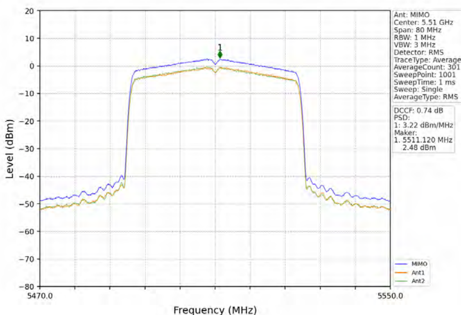
802.11ax(HEW40)_LCH_5510MHz_RU484_Left_MIMO_NTNV
