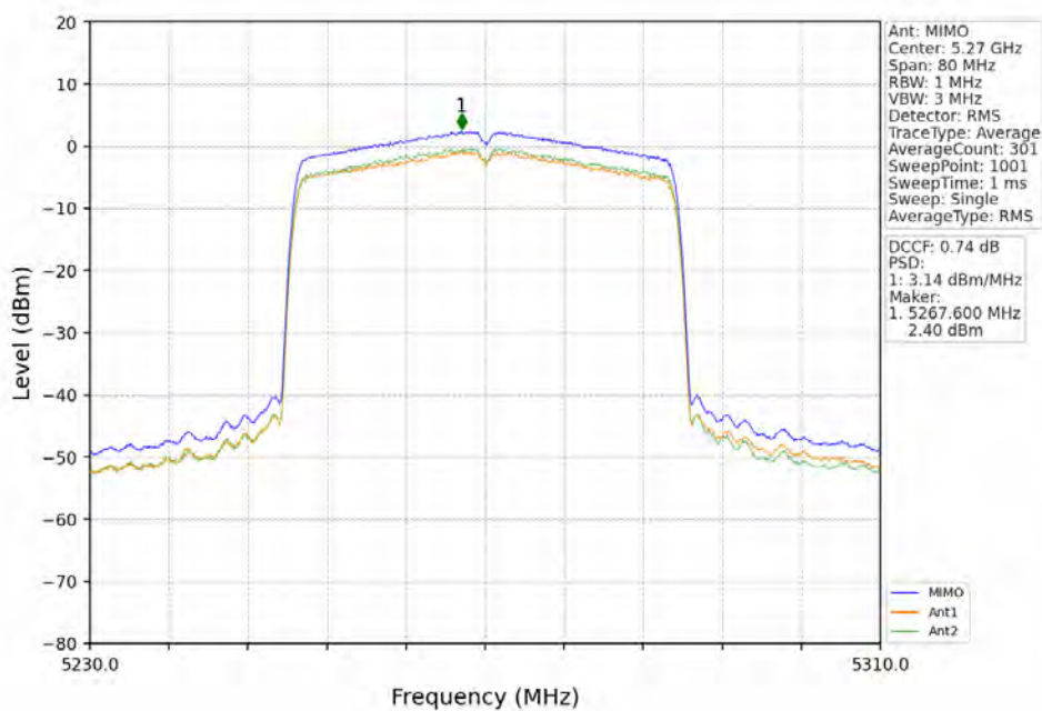
802.11ax(HEW40)_LCH_5270MHz_RU484_Left_MIMO_NTNV
