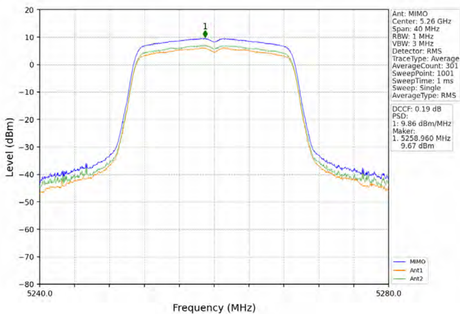
802.11n(HT20)_LCH_5260MHz_MIMO_NTNV
