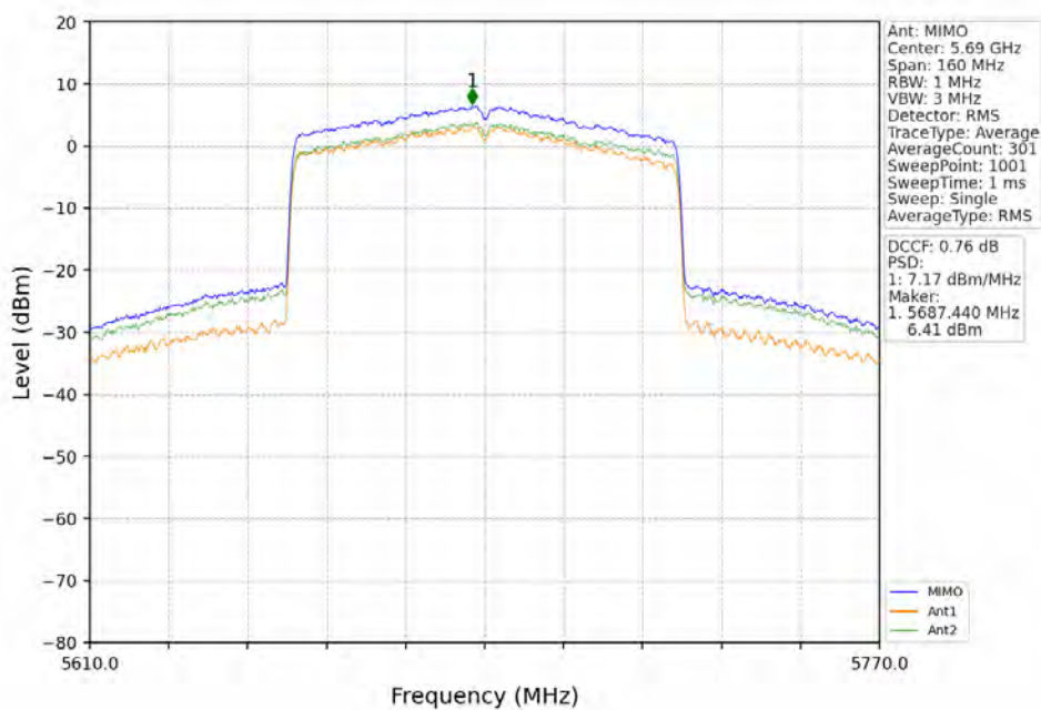
802.11ax(HEW80)_HCH_5690MHz_RU996_Left_MIMO_NTNV
