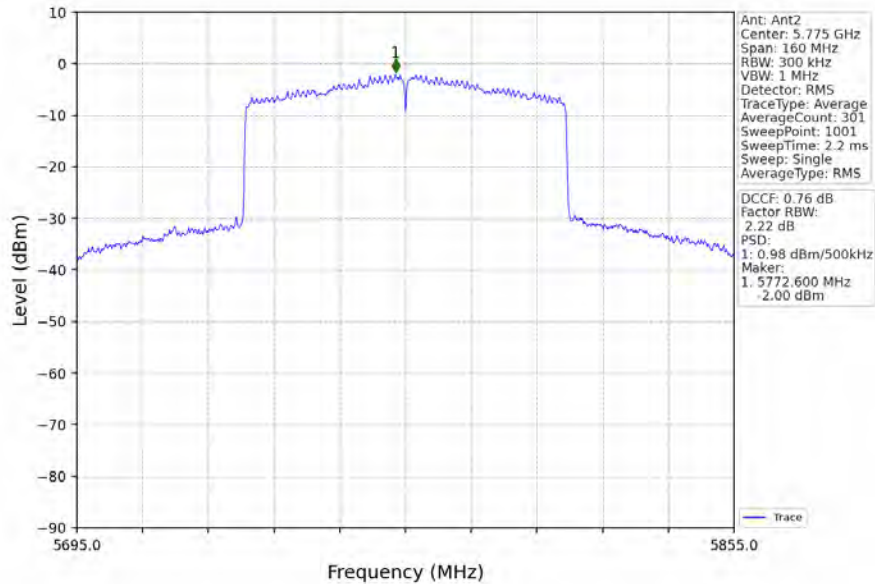
802.11ax(HEW80)_MCH_5775MHz_RU996_Left_MIMO_NTNV
