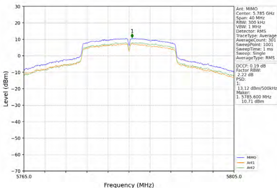
802.11ac(VHT20)_MCH_5785MHz_MIMO_NTNV
