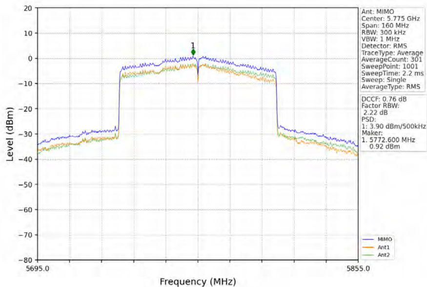
802.11ax(HEW80)_MCH_5775MHz_RU996_Left_MIMO_NTNV
