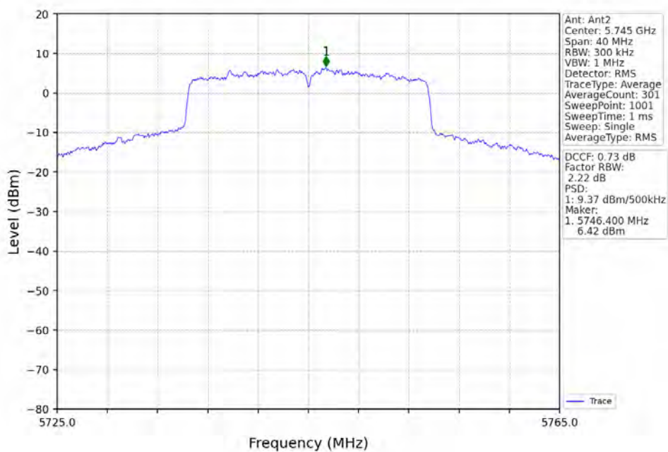
802.11ax(HEW20)_LCH_5745MHz_RU242_Left_Ant2_NTNV
