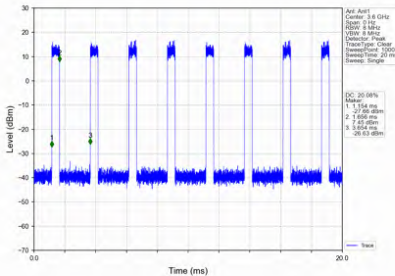
n78d_30kHz_SISO_NTNV_100MHz_CP-OFDM_256_QAM_3600MHz_Inner_Full
