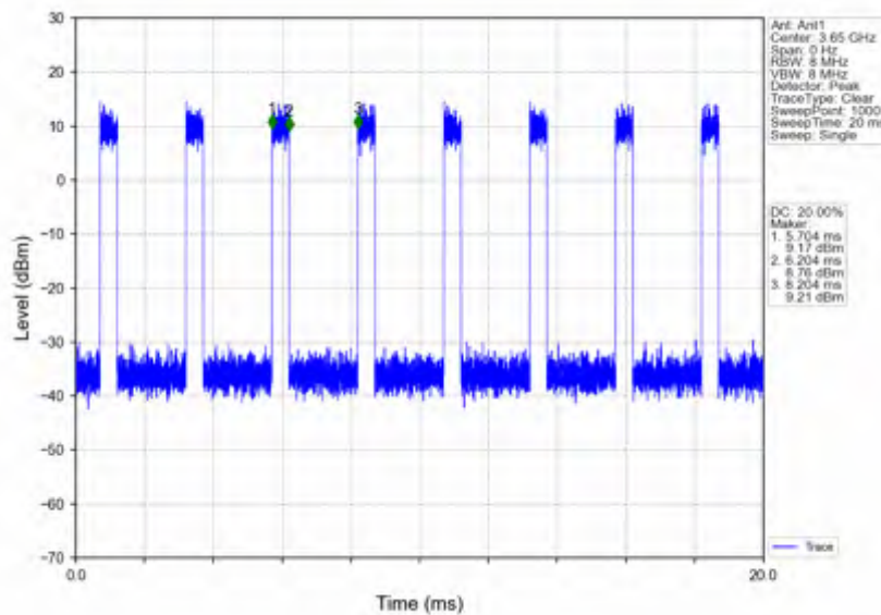
n78d_30kHz_SISO_NTNV_100MHz_CP-OFDM 256 QAM_3649.98MHz_Inner_Full
