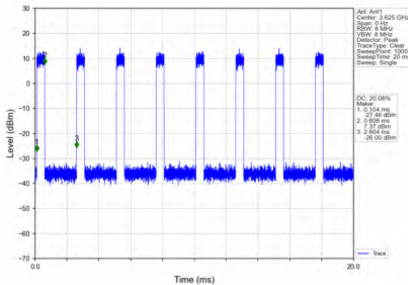
n78d_30kHz_SISO_NTNV_100MHz_CP-OFDM_256_QAM_3624.99MHz_Inner_Full
