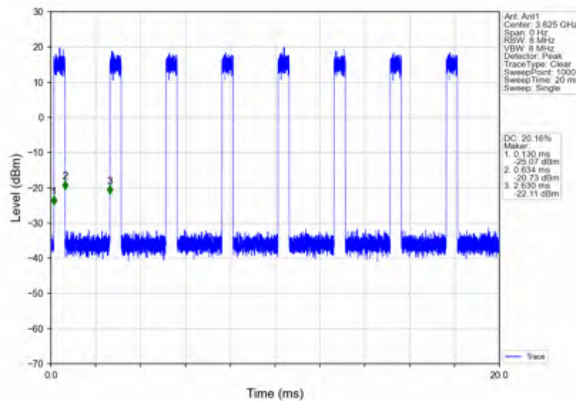
n78d_30kHz_SISO_NTNV_30MHz_CP-OFDM_QPSK_3624.99MHz_Inner_Full
