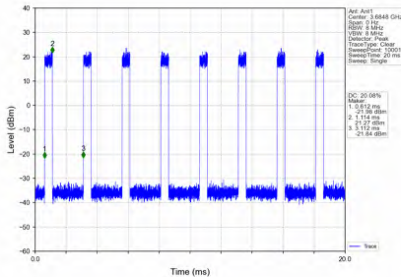
n78d_30kHz_SISO_NTNV_30MHz_CP-OFDM QPSK_3684.99MHz_Inner_Full
