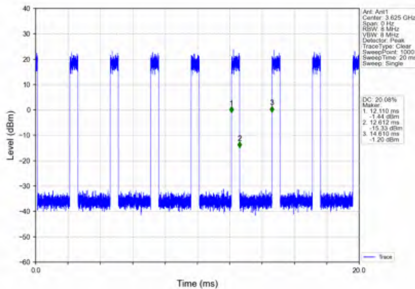
n78d_30kHz_SISO_NTNV_25MHz_CP-OFDM QPSK_3624.99MHz_Inner_Full
