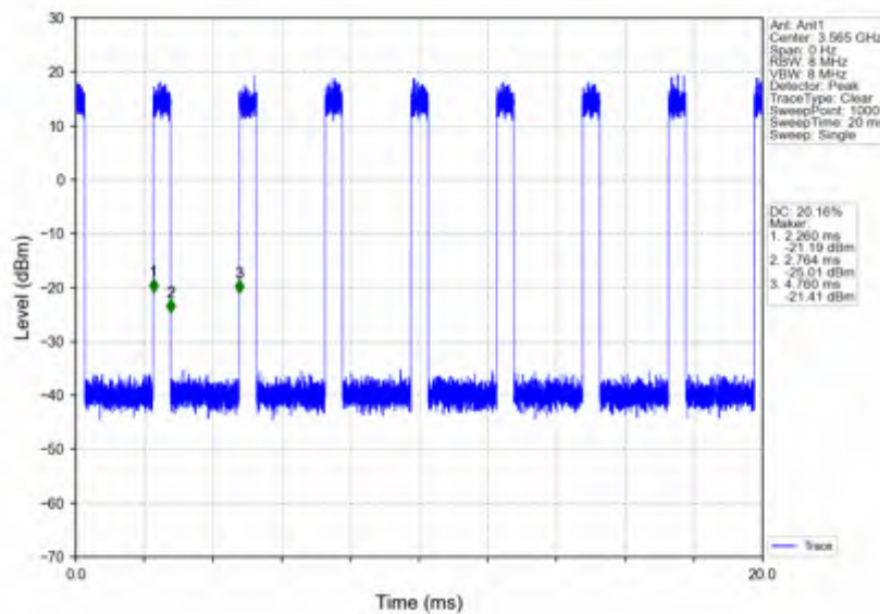
n78d_30kHz_SISO_NTNV_30MHz_CP-OFDM_256_QAM_3565.02MHz_Inner_Full
