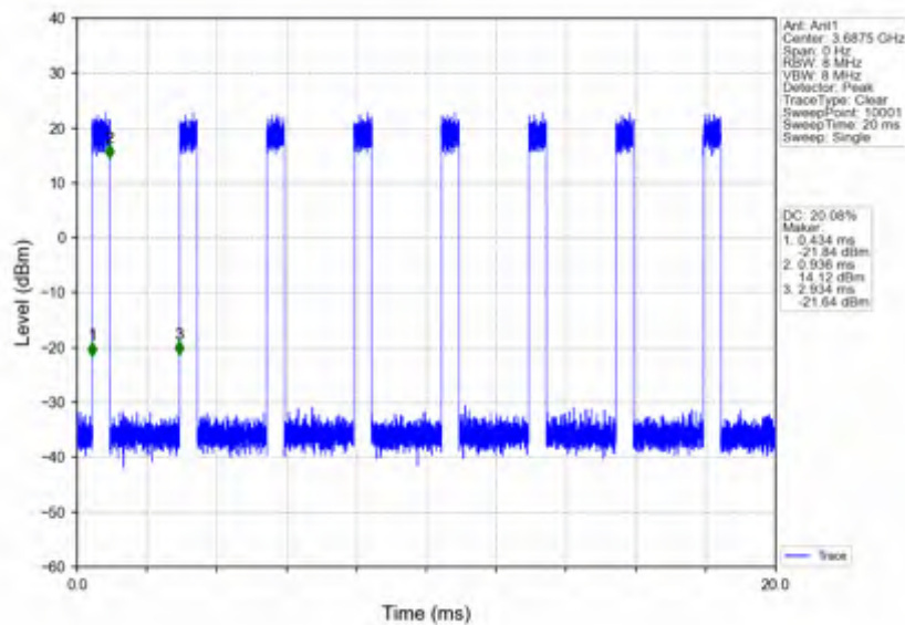
n78d_30kHz_SISO_NTNV_25MHz_CP-OFDM 64 QAM_3687.48MHz_Inner_Full
