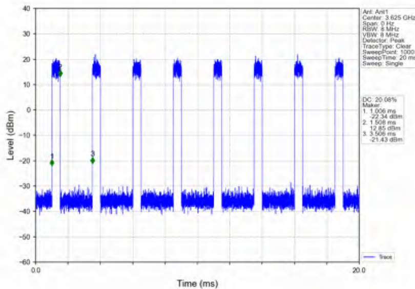
n78d_30kHz_SISO_NTNV_25MHz_CP-OFDM_256_QAM_3624.99MHz_Inner_Full
