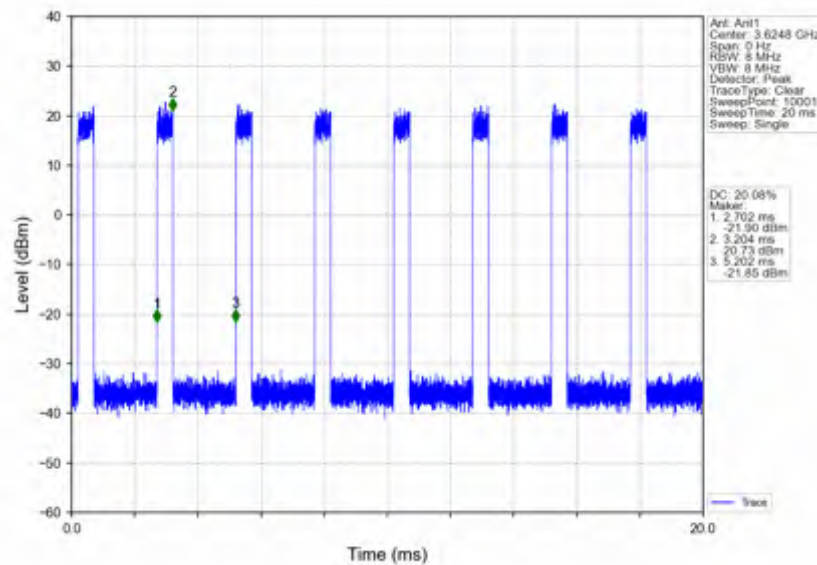
n78d_30kHz_SISO_NTNV_30MHz_CP-OFDM_QPSK_3624.99MHz_Inner_Full
