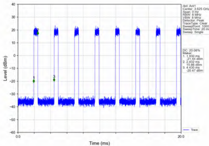
n78d_30kHz_SISO_NTNV_25MHz_CP-OFDM_16_QAM_3624.99MHz_Inner_Full
