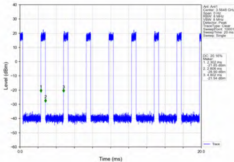
n78d_30kHz_SISO_NTNV_30MHz_CP-OFDM_QPSK_3565.02MHz_Inner_Full
