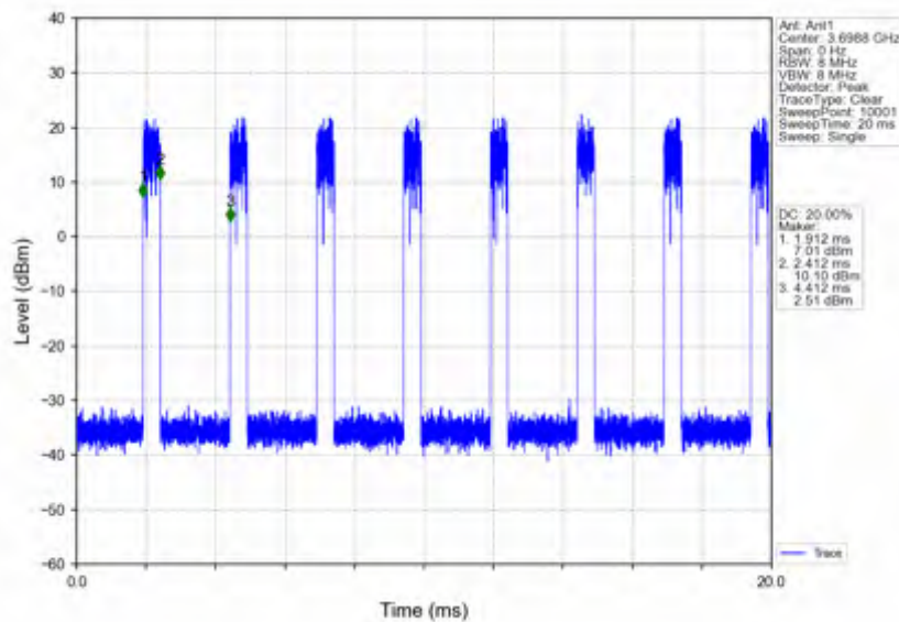
n78d_30kHz_SISO_NTNV_30MHz_CP-OFDM 16 QAM_3684.99MHz_Edge_1RB_Right
