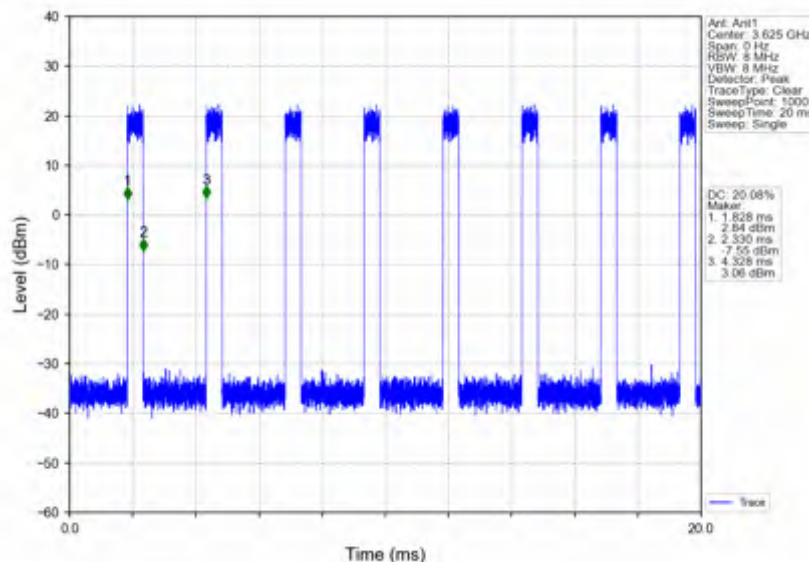
n78d_30kHz_SISO_NTNV_25MHz_CP-OFDM 64 QAM_3624.99MHz_Inner_Full
