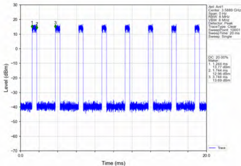
n78d_30kHz_SISO_NTNV_40MHz_DFT-s-OFDM PI/2 BPSK_3570MHz_Edge_1RB_Right
