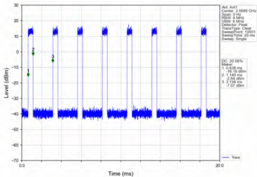
n78d_30kHz_SISO_NTNV_40MHz_DFT-s-OFDM_256_QAM_3570MHz_Inner_Full
