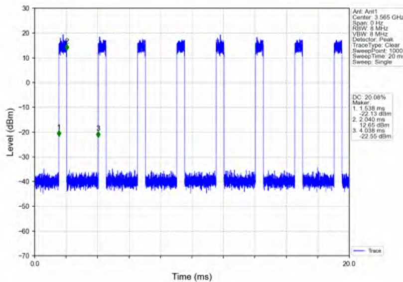
n78d_30kHz_SISO_NTNV_30MHz_CP-OFDM_QPSK_3565.02MHz_Inner_Full
