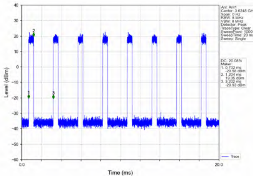
n78d_30kHz_SISO_NTNV_30MHz_CP-OFDM 64 QAM_3624.99MHz_Inner_Full
