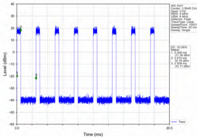
n78d_30kHz_SISO_NTNV_30MHz_CP-OFDM_256_QAM_3565.02MHz_Inner_Full
