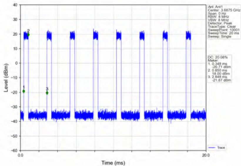
n78d_30kHz_SISO_NTNV_25MHz_CP-OFDM_256_QAM_3687.48MHz_Inner_Full
