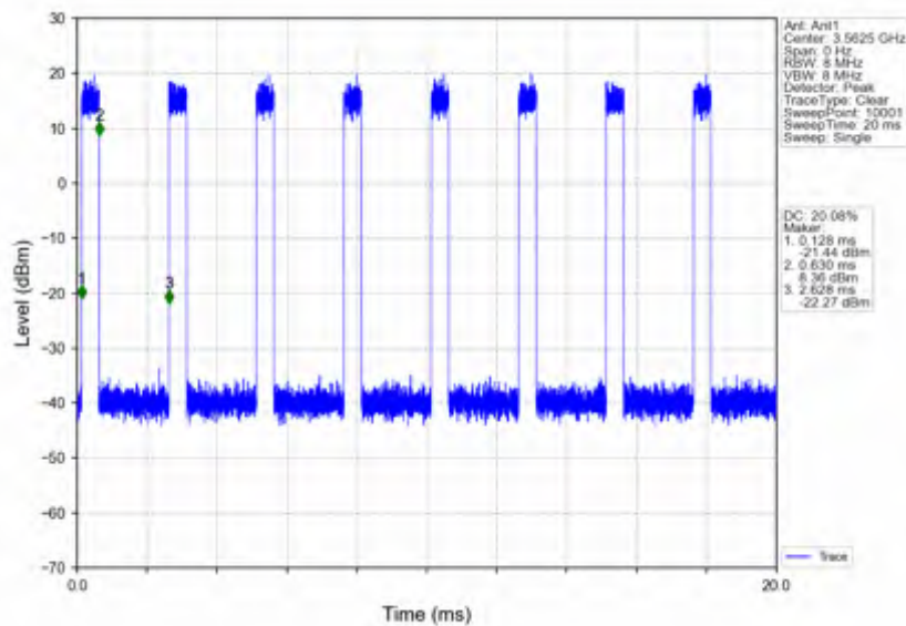
n78d_30kHz_SISO_NTNV_25MHz_CP-OFDM QPSK_3562.5MHz_Inner_Full
