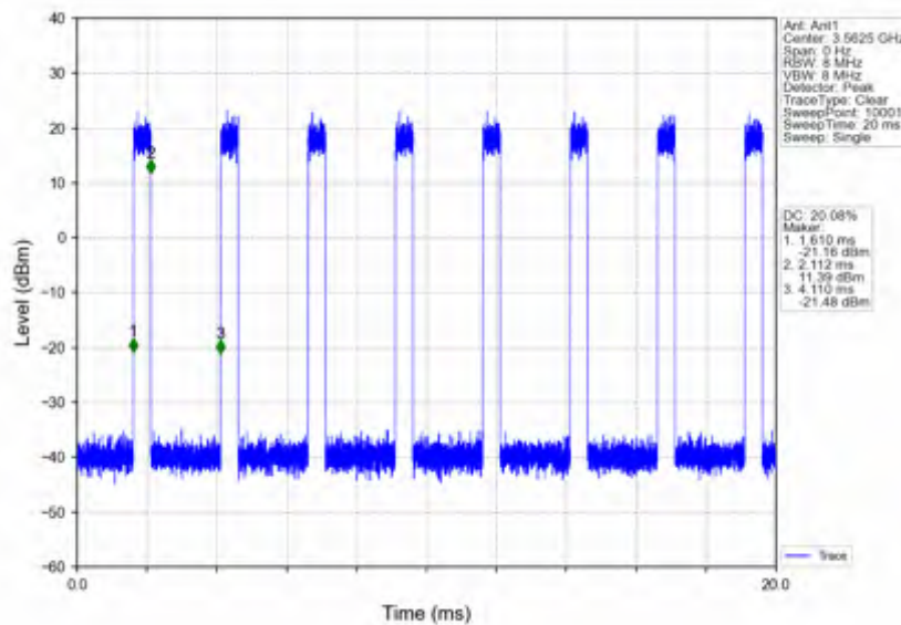
n78d_30kHz_SISO_NTNV_25MHz_CP-OFDM_16_QAM_3562.5MHz_Inner_Full
