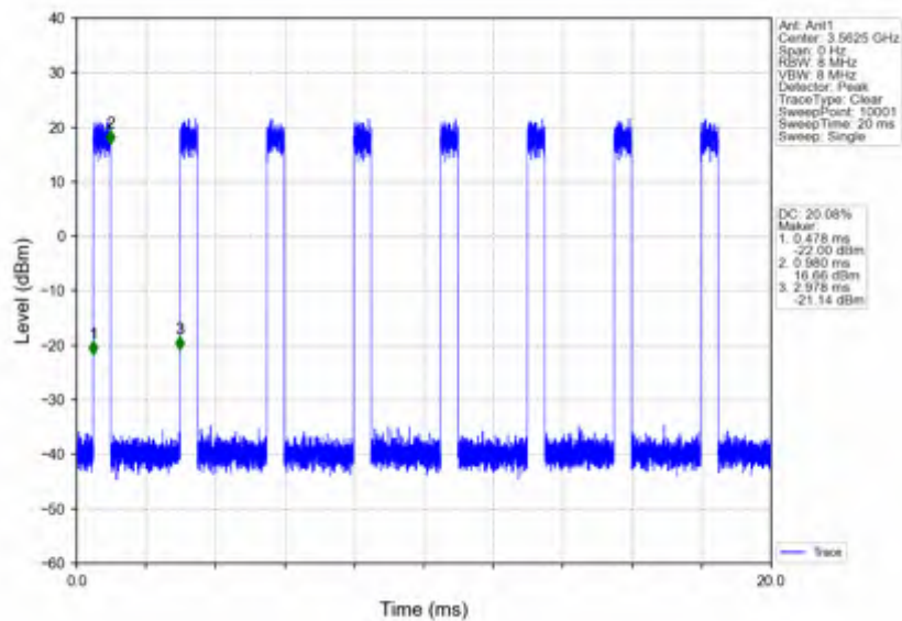
n78d_30kHz_SISO_NTNV_25MHz_CP-OFDM_256_QAM_3562.5MHz_Inner_Full
