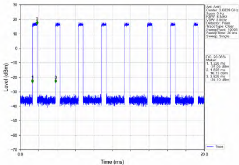
n78d_30kHz_SISO_NTNV_30MHz_DFT-s-OFDM_QPSK_3684.99MHz_Inner_Full
