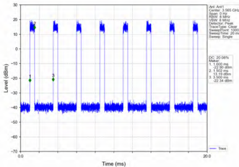
n78d_30kHz_SISO_NTNV_30MHz_CP-OFDM 64 QAM_3565.02MHz_Inner_Full
