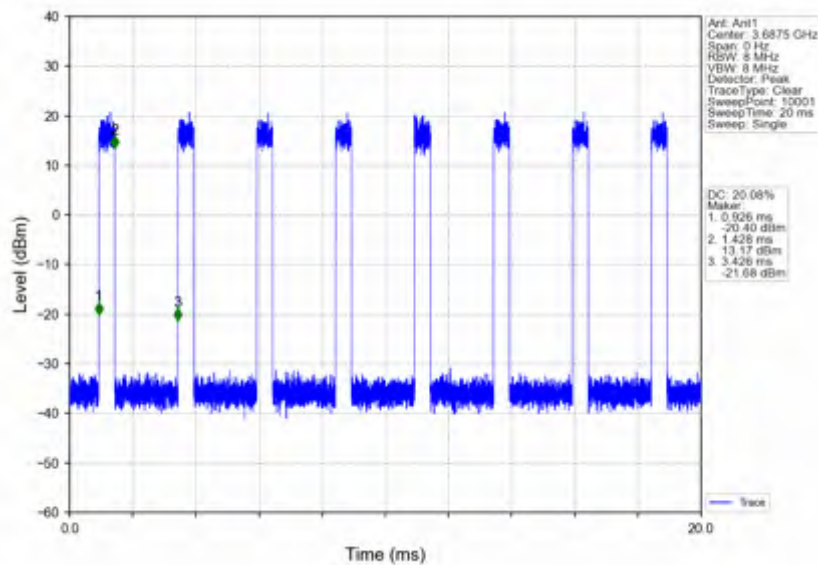
n78d_30kHz_SISO_NTNV_25MHz_CP-OFDM QPSK_3687.48MHz_Inner_Full
