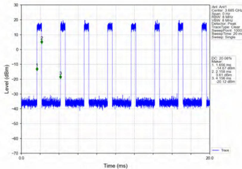
n78d_30kHz_SISO_NTNV_30MHz_CP-OFDM QPSK_3684.99MHz_Inner_Full
