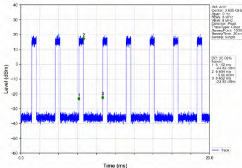
n78d_30kHz_SISO_NTNV_50MHz_CP-OFDM_256_QAM_3624.99MHz_Inner_Full
