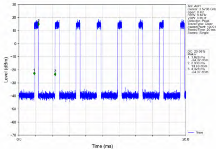
n78d_30kHz_SISO_NTNV_60MHz_CP-OFDM_QPSK_3580.02MHz_Inner_Full
