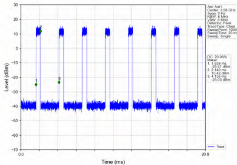
n78d_30kHz_SISO_NTNV_60MHz_CP-OFDM_QPSK_3580.02MHz_Inner_Full
