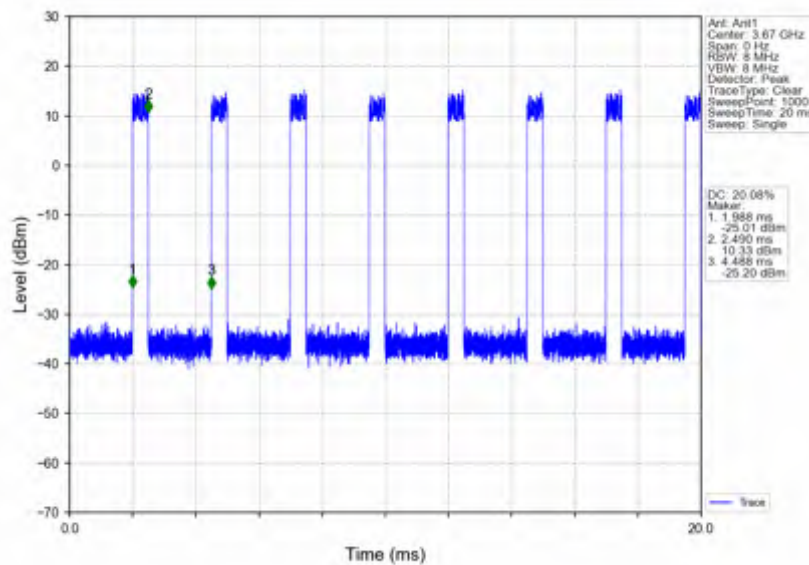
n78d_30kHz_SISO_NTNV_60MHz_DFT-s-OFDM 64 QAM_3669.99MHz_Inner_Full
