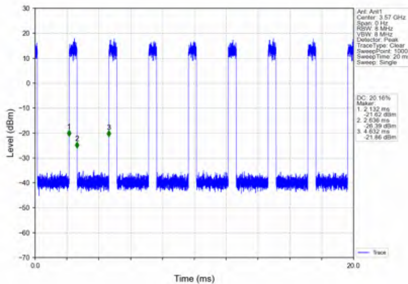
n78d_30kHz_SISO_NTV_40MHz_CP-OFDM_256_QAM_3570MHz_Inner_Full
