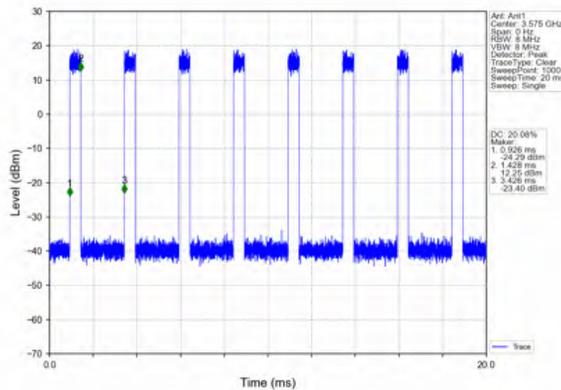
n78d_30kHz_SISO_NTNV_50MHz_CP-OFDM_256_QAM_3575.01MHz_Inner_Full
