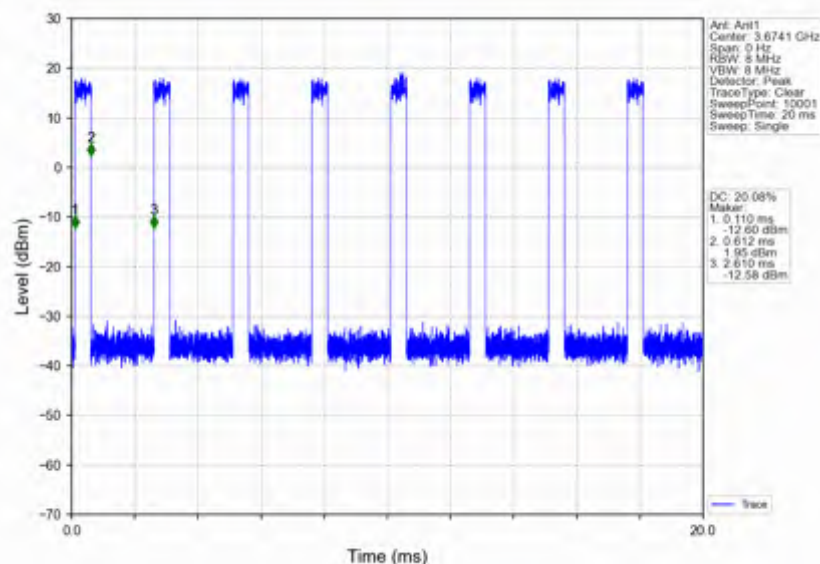
n78d_30kHz_SISO_NTNV_50MHz_DFT-s-OFDM_256_QAM_3675MHz_Inner_Full
