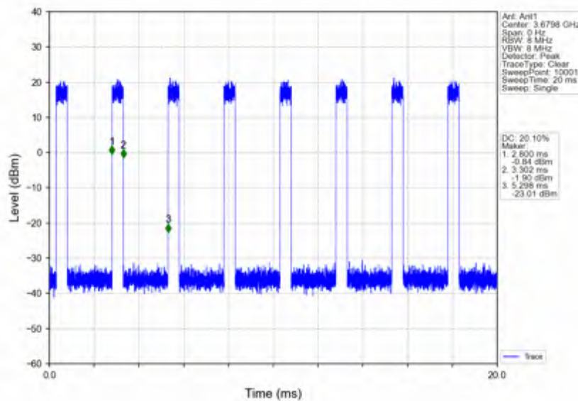
n78d_30kHz_SISO_NTNV_40MHz_CP-OFDM_256_QAM_3679.98MHz_Inner_Full
