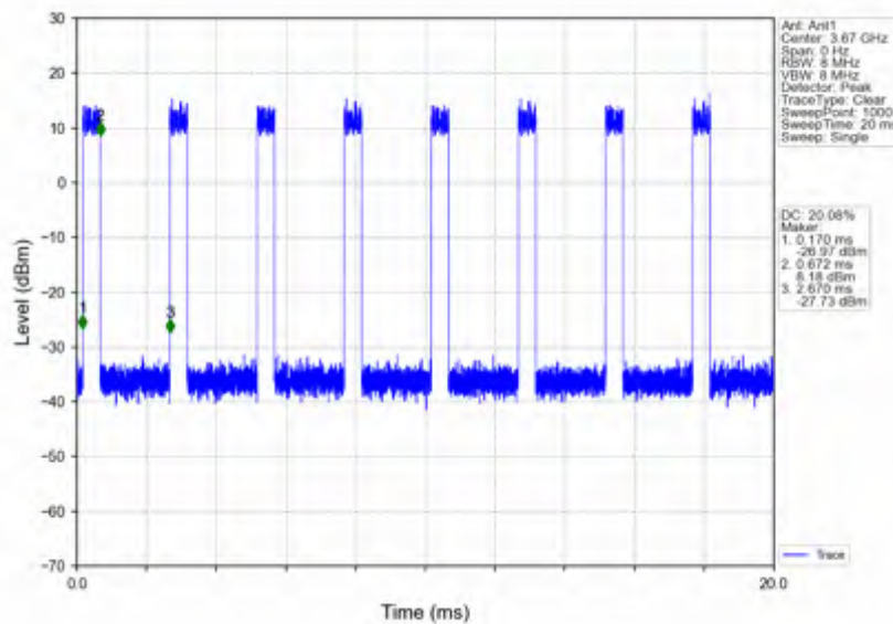
n78d_30kHz_SISO_NTNV_60MHz_DFT-s-OFDM_QPSK_3669.99MHz_Inner_Full
