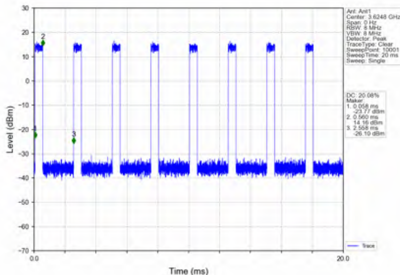
n78d 30kHz SISO NTNV 60MHz DFT-s-OFDM QPSK 3624.99MHz Inner Full
