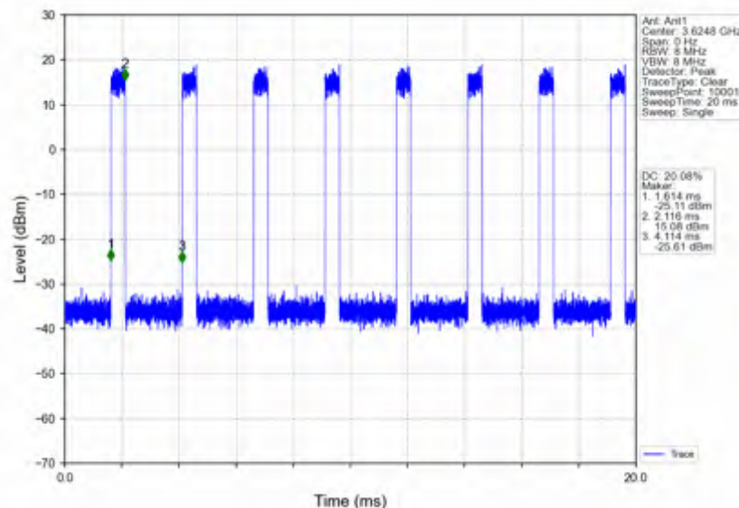
n78d_30kHz_SISO_NTNV_60MHz_CP-OFDM_QPSK_3624.99MHz_Inner_Full
