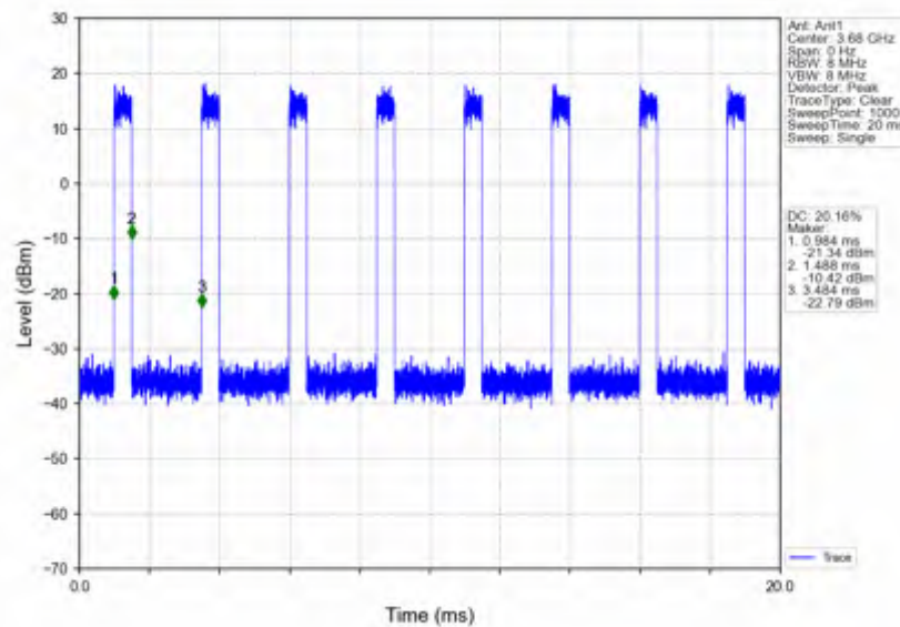
n78d_30kHz_SISO_NTNV_40MHz_CP-OFDM QPSK_3679.98MHz_Inner_Full
