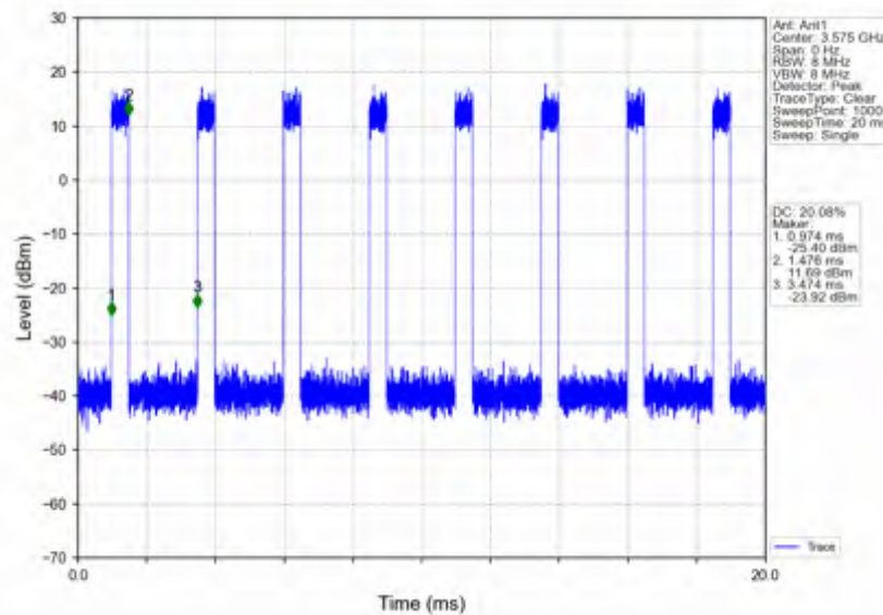
n78d_30kHz_SISO_NTNV_50MHz_CP-OFDM QPSK_3575.01MHz_Inner_Full
