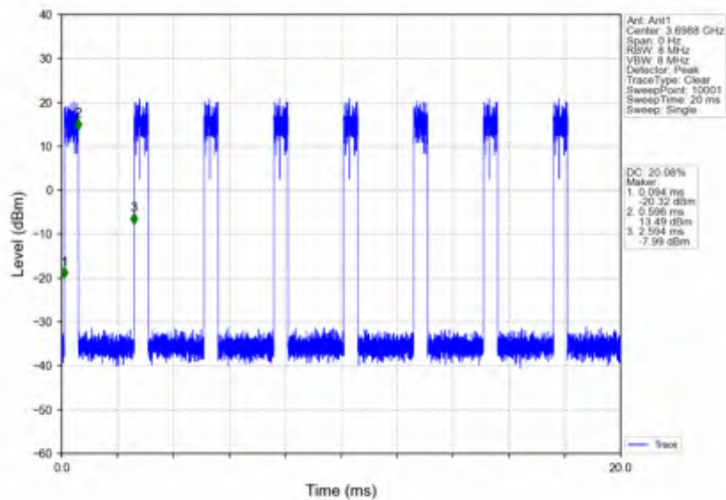
n78d_30kHz_SISO_NTNV_50MHz_DFT-s-OFDM_64_QAM_3675MHz_Edge_1RB_Right
