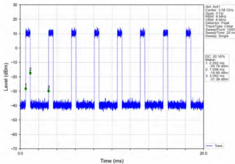
n78d_30kHz_SISO_NTNV_60MHz_DFT-s-OFDM_QPSK_3580.02MHz_Inner_Full
