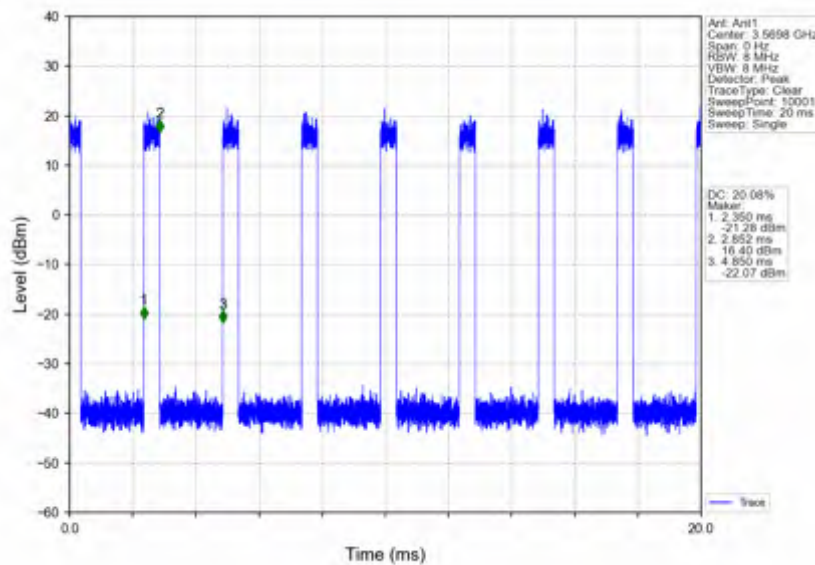
n78d_30kHz_SISO_NTNV_40MHz_CP-OFDM 64 QAM_3570MHz_Inner_Full
