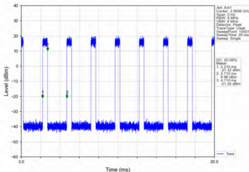
n78d 30kHz SISO NTV 40MHz CP-OFDM QPSK 3570MHz Inner Full
