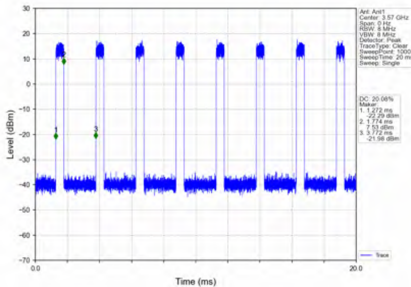
n78d_30kHz_SISO_NTNV_40MHz_CP-OFDM 64 QAM_3570MHz_Inner_Full
