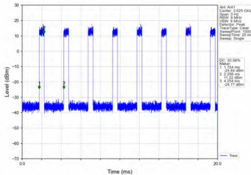
n78d_30kHz_SISO_NTNV_50MHz_CP-OFDM_QPSK_3624.99MHz_Inner_Full
