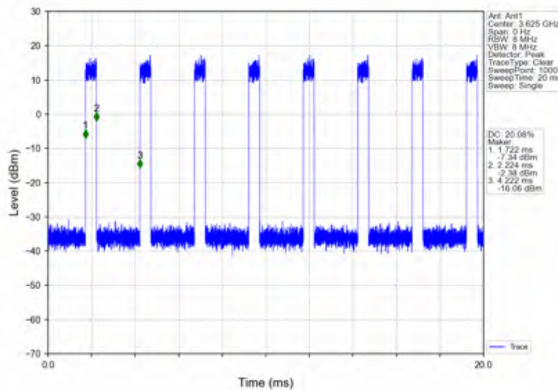
n78d_30kHz_SISO_NTNV_50MHz_CP-OFDM 16 QAM 3624.99MHz_Inner_Full
