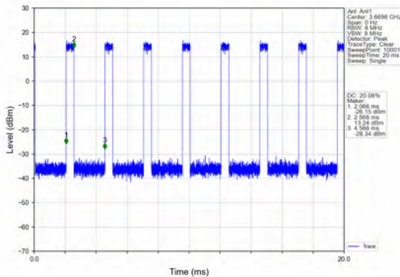
n78d_30kHz_SISO_NTNV_60MHz_DFT-s-OFDM_QPSK_3669.99MHz_Inner_Full
