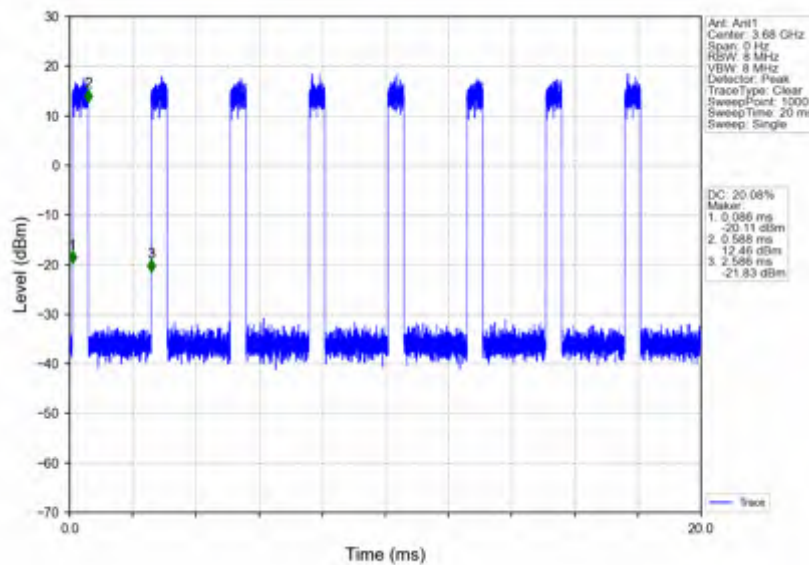
n78d_30kHz_SISO_NTNV_40MHz_CP-OFDM_256_QAM_3679.98MHz_Inner_Full
