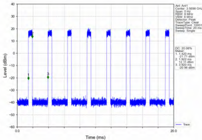
n78d_30kHz_SISO_NTV_40MHz_CP-OFDM_256_QAM_3570MHz_Inner_Full
