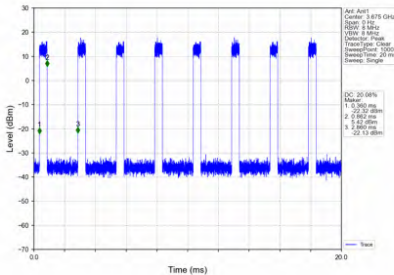
n78d_30kHz_SISO_NTNV_50MHz_CP-OFDM_64_QAM_3675MHz_Inner_Full
