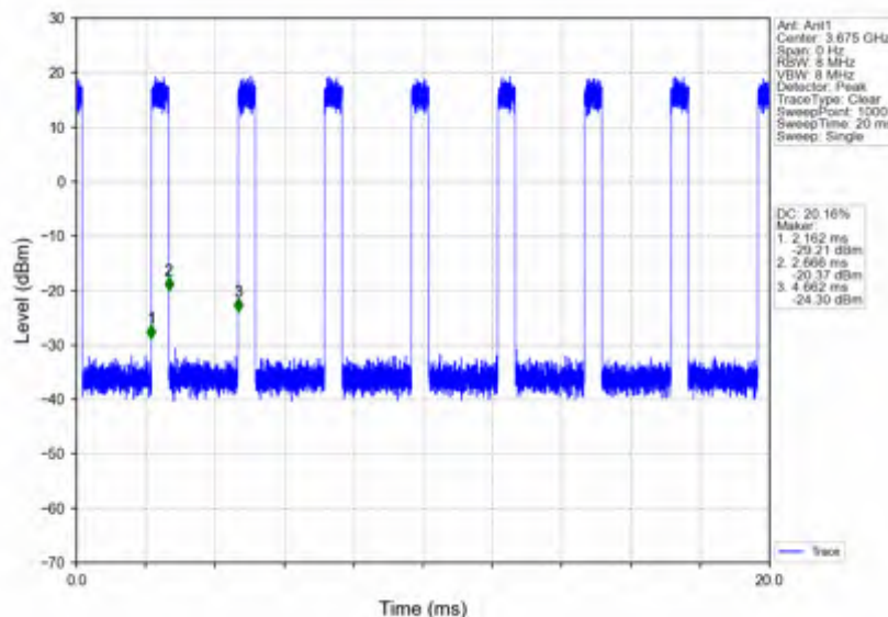
n78d_30kHz_SISO_NTNV_50MHz_CP-OFDM_QPSK_3675MHz_Inner_Full
