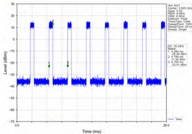
n78d_30kHz_SISO_NTNV_60MHz_CP-OFDM_QPSK_3624.99MHz_Inner_Full
