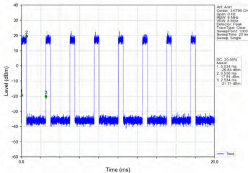
n78d_30kHz_SISO_NTNV_40MHz_CP-OFDM 64 QAM_3679.98MHz_Inner_Full
