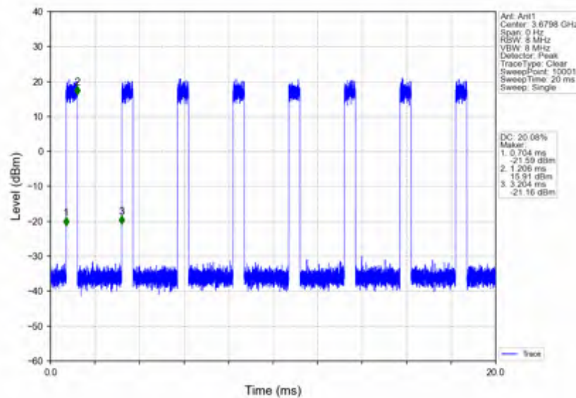
n78d_30kHz_SISO_NTNV_40MHz_CP-OFDM QPSK_3679.98MHz_Inner_Full
