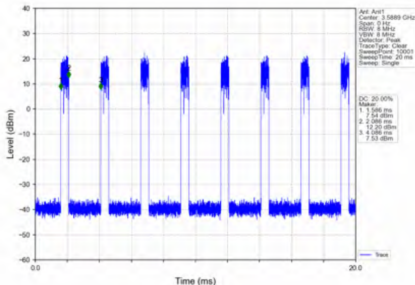
n78d_30kHz_SISO_NTNV_40MHz_CP-OFDM_16 QAM_3570MHz_Edge_1RB_Right
