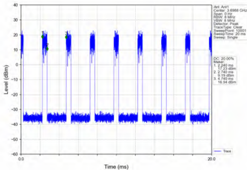
n78d_30kHz_SISO_NTNV_50MHz_CP-OFDM_QPSK_3675MHz_Edge_1RB_Right
