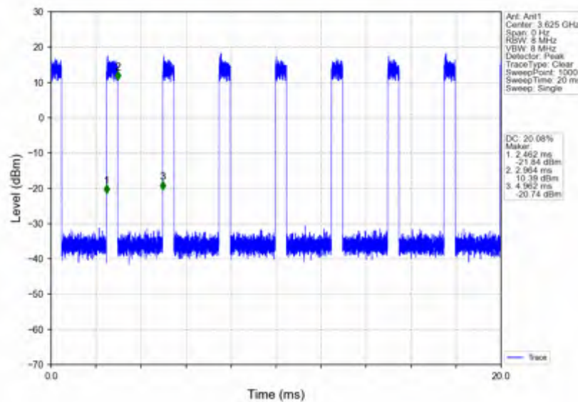
n78d_30kHz_SISO_NTNV_40MHz_CP-OFDM_QPSK_3624.99MHz_Inner_Full
