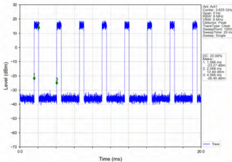
n78d_30kHz_SISO_NTNV_50MHz_CP-OFDM 64 QAM_3624.99MHz_Inner_Full
