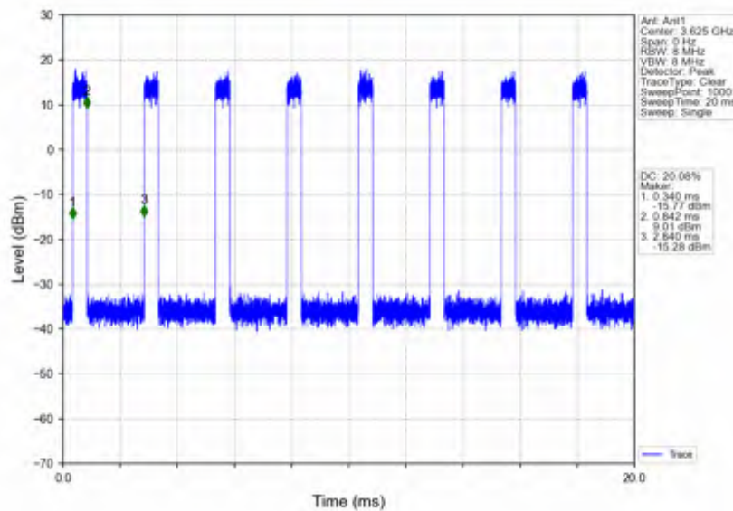
n78d 30kHz SISO NTNV 40MHz CP-OFDM 256 QAM 3624.99MHz Inner Full
