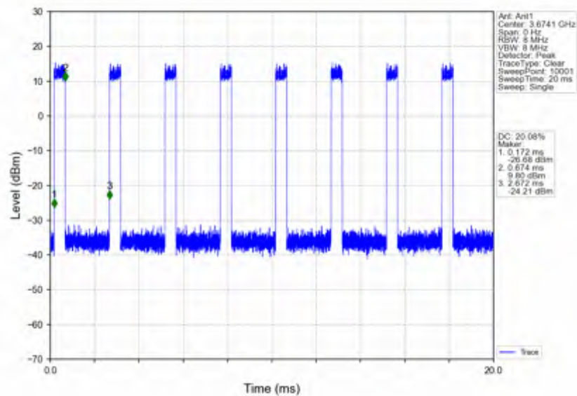
n78d_30kHz_SISO_NTNV_50MHz_DFT-s-OFDM_QPSK_3675MHz_Inner_Full
