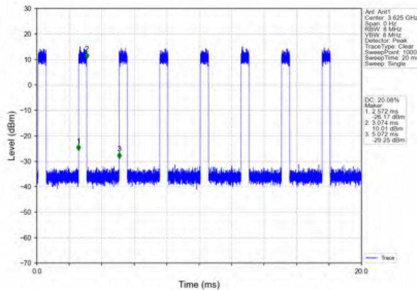
n78d_30kHz_SISO_NTNV_70MHz_CP-OFDM_QPSK_3624.99MHz_Inner_Full
