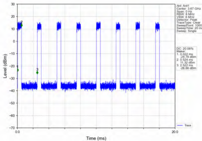
n78d_30kHz_SISO_NTNV_60MHz_CP-OFDM_QPSK_3669.99MHz_Inner_Full
