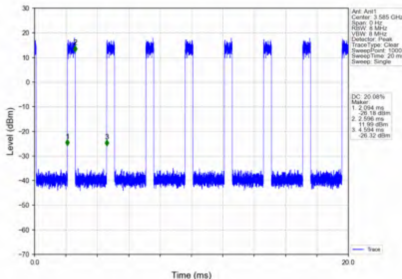
n78d_30kHz_SISO_NTNV_70MHz_CP-OFDM_16_QAM_3585MHz_Inner_Full
