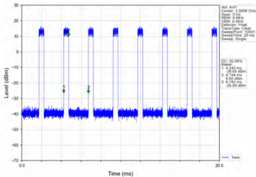
n78d_30kHz_SISO_NTNV_80MHz_DFT-s-OFDM_256_QAM_3590.01MHz_Inner_Full
