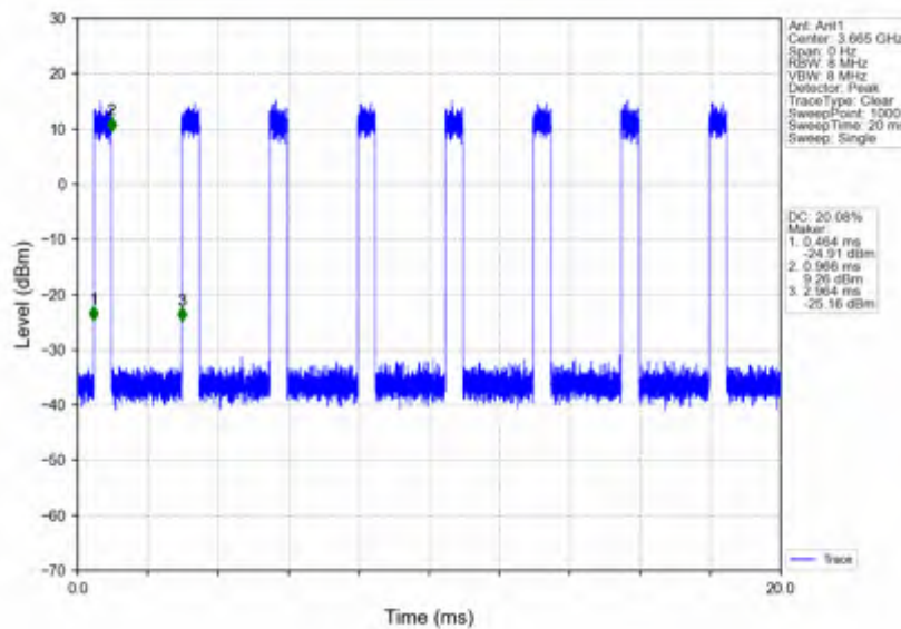
n78d_30kHz_SISO_NTNV_70MHz_CP-OFDM_16_QAM_3664.98MHz_Inner_Full
