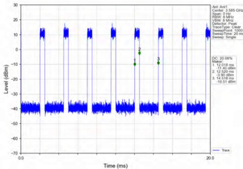
n78d_30kHz_SISO_NTNV_70MHz_CP-OFDM 64 QAM_3585MHz_Inner_Full
