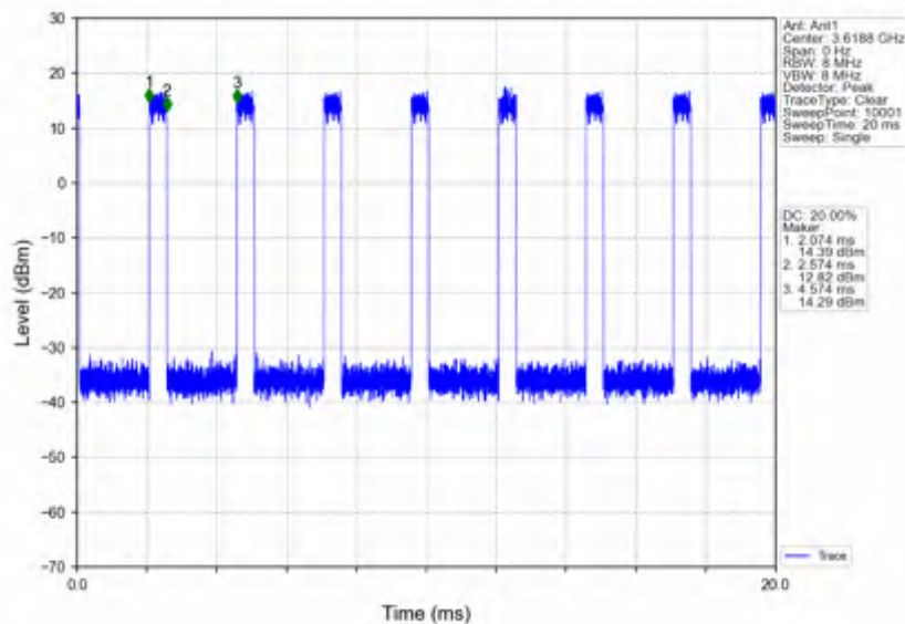
n78d_30kHz_SISO_NTNV_70MHz_DFT-s-OFDM_PI/2_BPSK_3585MHz_Edge_1RB_Right
