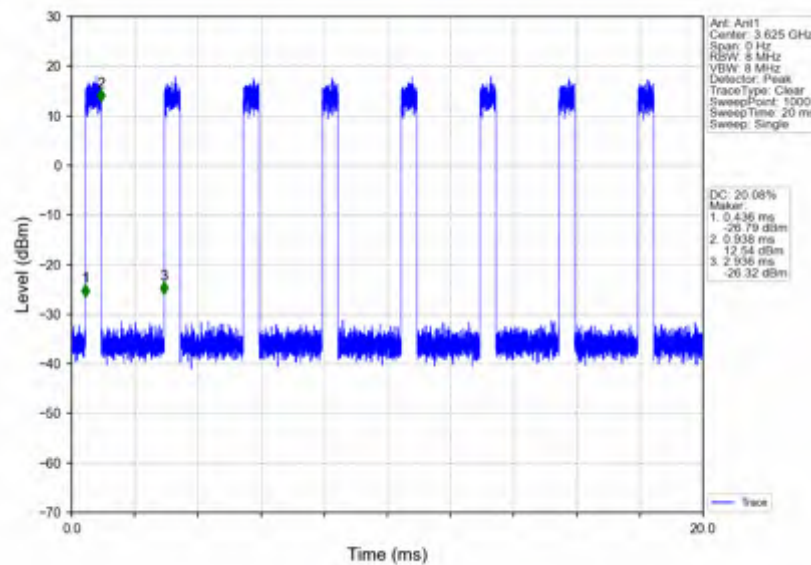
n78d_30kHz_SISO_NTNV_80MHz_CP-OFDM_QPSK_3624.99MHz_Inner_Full
