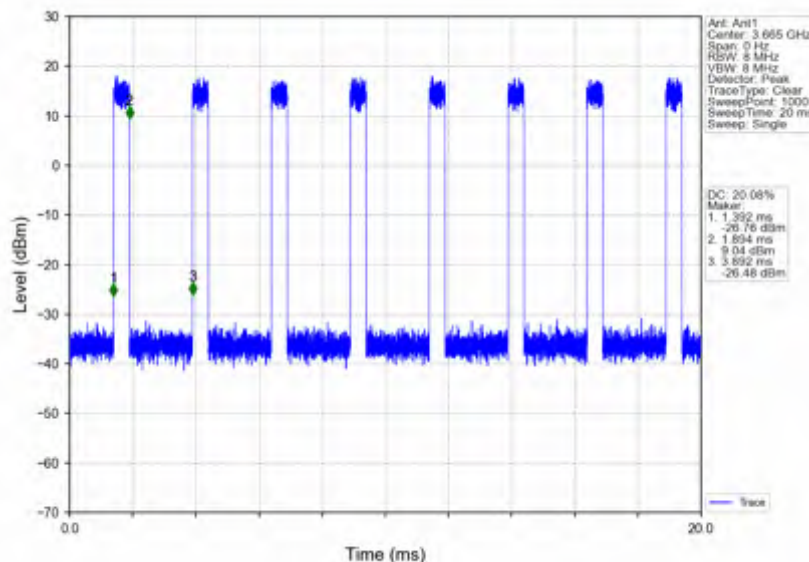
n78d_30kHz_SISO_NTNV_70MHz_CP-OFDM 64 QAM_3664.98MHz_Inner_Full
