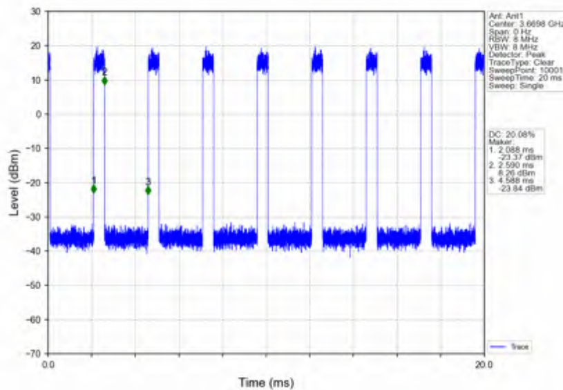
n78d_30kHz_SISO_NTNV_60MHz_CP-OFDM_16_QAM_3669.99MHz_Inner_Full
