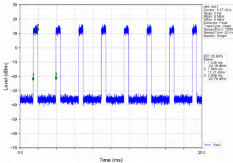
n78d_30kHz_SISO_NTNV_60MHz_CP-OFDM 64 QAM_3669.99MHz_Inner_Full
