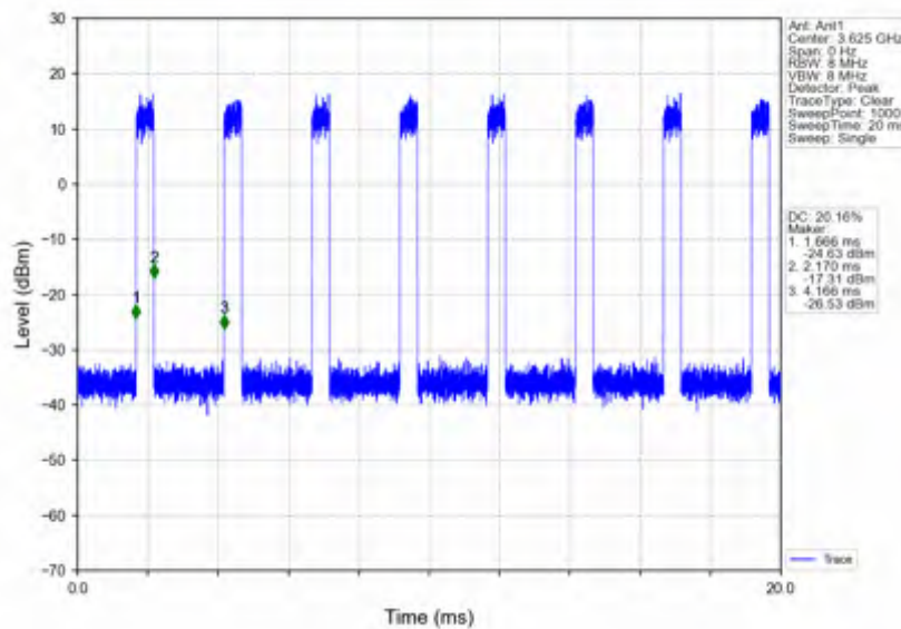
n78d_30kHz_SISO_NTNV_60MHz_CP-OFDM 64 QAM_3624.99MHz_Inner_Full
