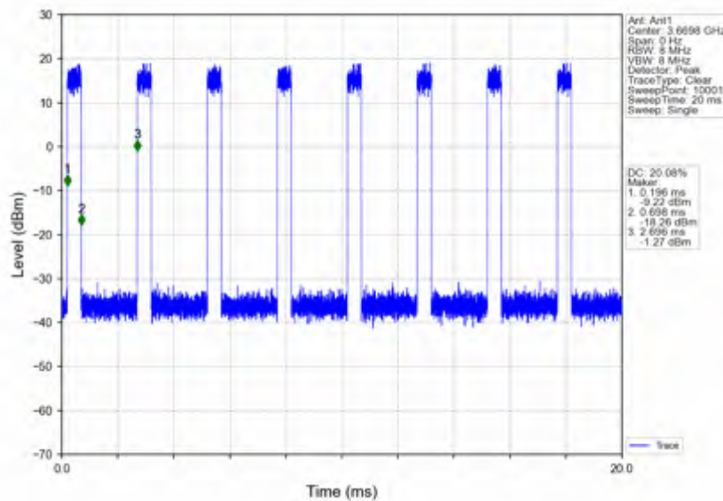
n78d_30kHz_SISO_NTNV_60MHz_CP-OFDM_256_QAM_3669.99MHz_Inner_Full
