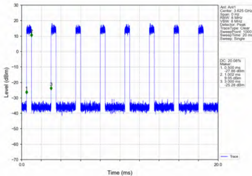
n78d_30kHz_SISO_NTNV_70MHz_CP-OFDM 64 QAM_3624.99MHz_Inner_Full
