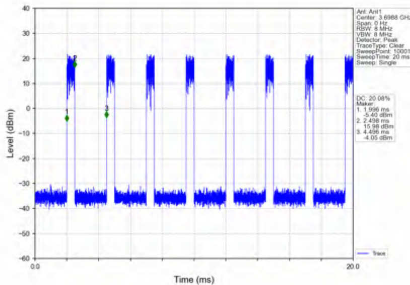
n78d_30kHz_SISO_NTNV_70MHz_CP-OFDM 64 QAM_3664.98MHz_Edge_1RB_Right
