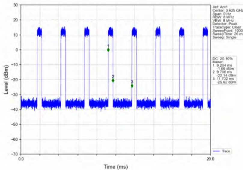
n78d_30kHz_SISO_NTNV_60MHz_CP-OFDM_256_QAM_3624.99MHz_Inner_Full
