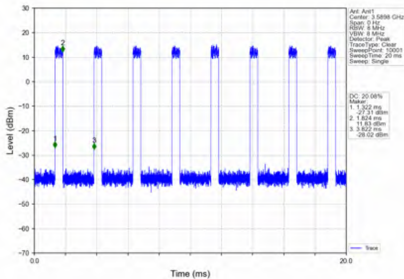
n78d_30kHz_SISO_NTNV_80MHz_DFT-s-OFDM_QPSK_3590.01MHz_Inner_Full
