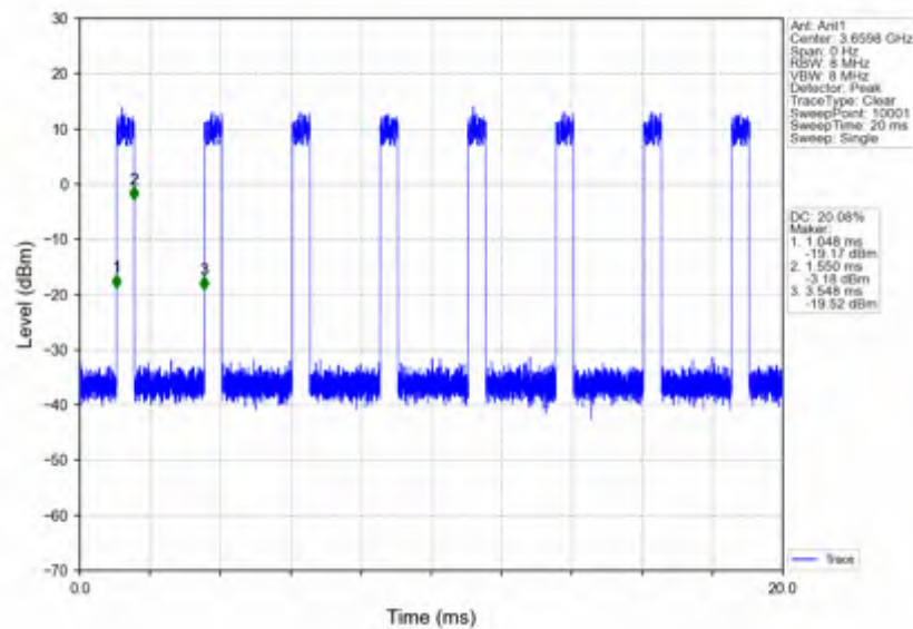
n78d_30kHz_SISO_NTNV_80MHz_DFT-s-OFDM_QPSK_3660MHz_Inner_Full
