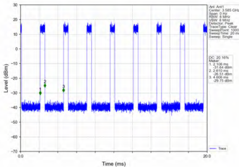
n78d_30kHz_SISO_NTNV_70MHz_CP-OFDM_QPSK_3585MHz_Inner_Full
