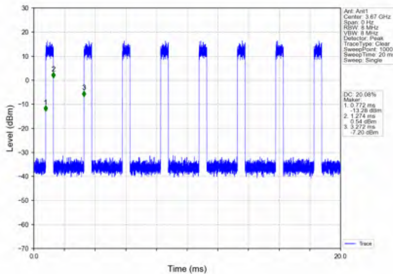
n78d_30kHz_SISO_NTNV_60MHz_CP-OFDM_16_QAM_3669.99MHz_Inner_Full
