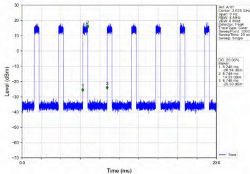
n78d_30kHz_SISO_NTNV_70MHz_CP-OFDM_256_QAM_3624.99MHz_Inner_Full
