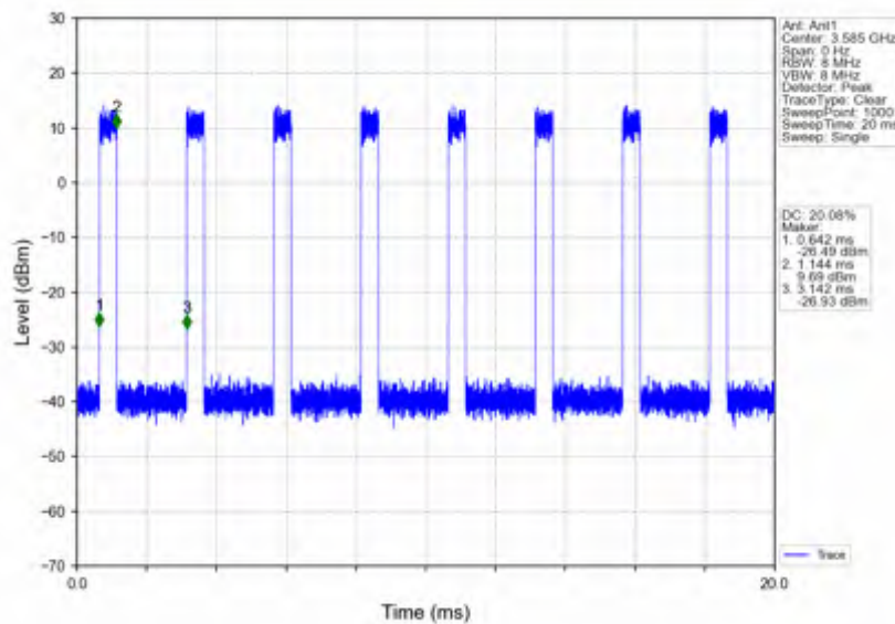
n78d_30kHz_SISO_NTNV_70MHz_CP-OFDM_256_QAM_3585MHz_Inner_Full
