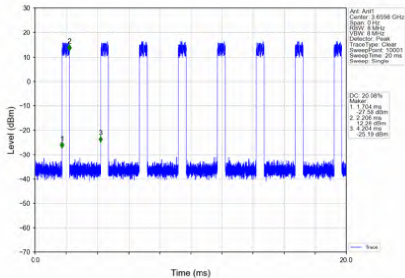
n78d_30kHz_SISO_NTNV_80MHz_DFT-s-OFDM_256_QAM_3660MHz_Inner_Full
