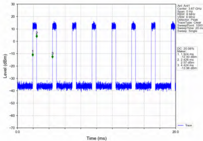
n78d_30kHz_SISO_NTNV_60MHz_CP-OFDM_256_QAM_3669.99MHz_Inner_Full
