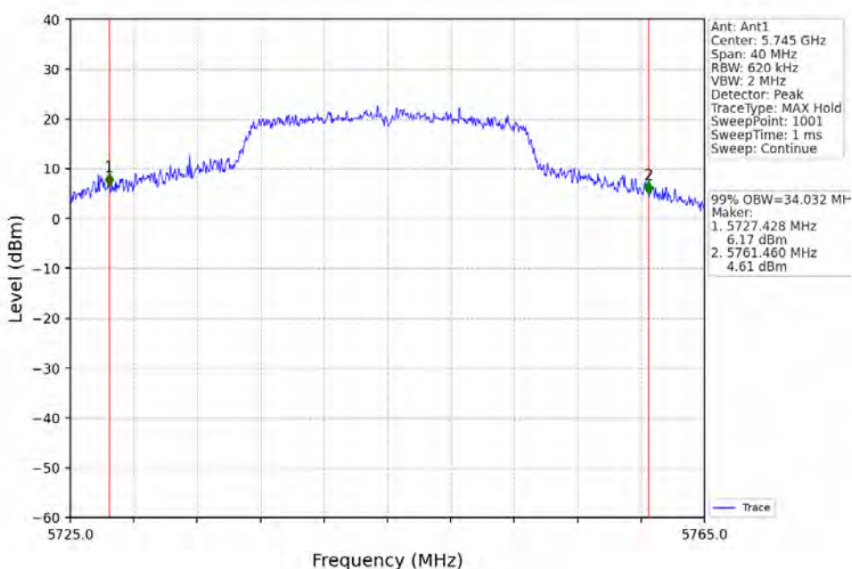
802.11ac(VHT20)_LCH_5745MHz_Ant1_NTNV
