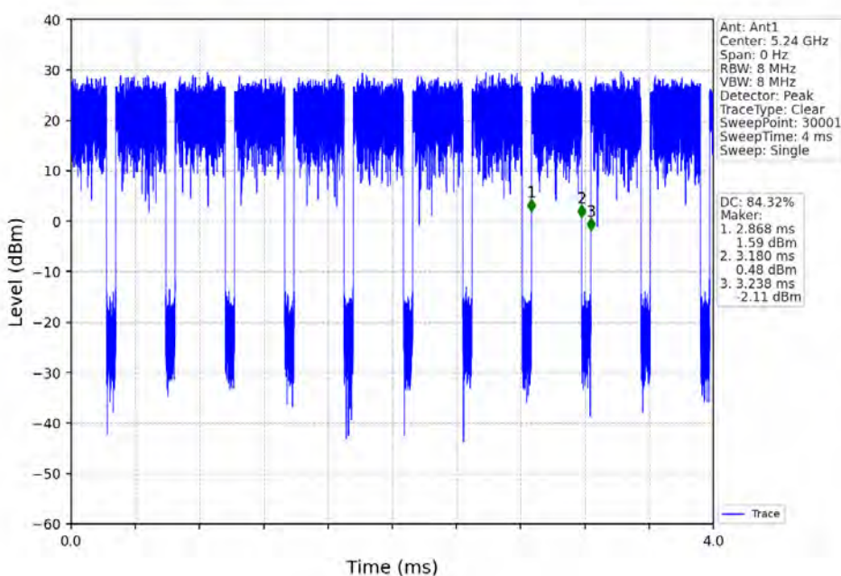
802.11ax(HEW20)_HCH_5240MHz_RU242_Left_Ant1_NTNV
