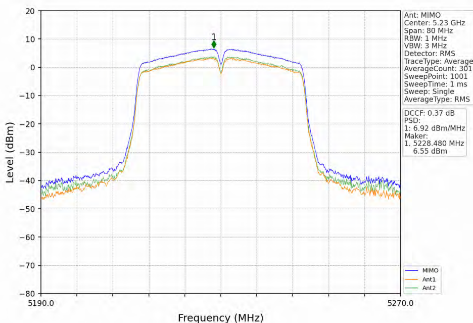
802.11ac(VHT40)_HCH_5230MHz_MIMO_NTNV
