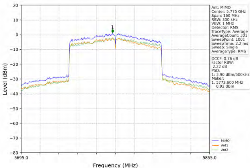
802.11ax(HEW80)_MCH_5775MHz_RU996_Left_MIMO_NTNV
