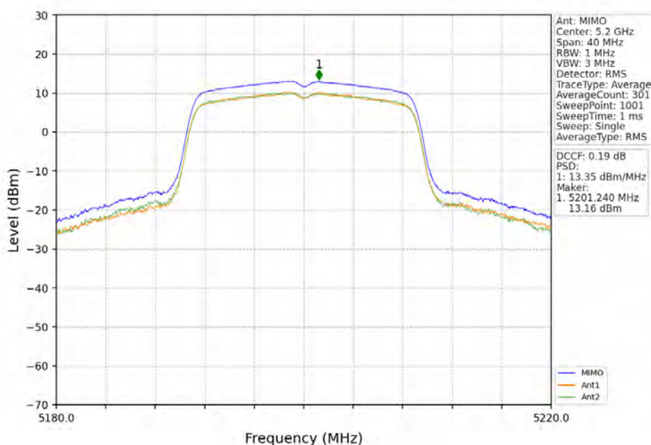
802.11ac(VHT20)_MCH_5200MHz_MIMO_NTNV
