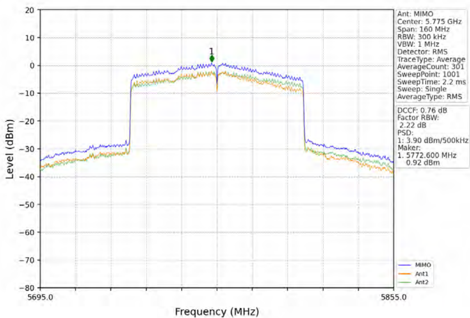
802.11ax(HEW80)_MCH_5775MHz_RU996_Left_MIMO_NTNV
