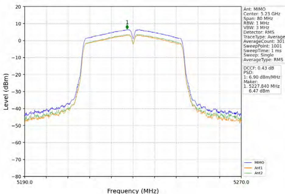
802.11n(HT40)_HCH_5230MHz_MIMO_NTNV
