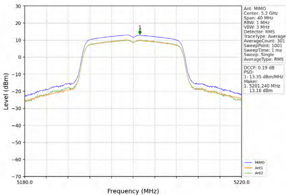
802.11ac(VHT20)_MCH_5200MHz_MIMO_NTNV
