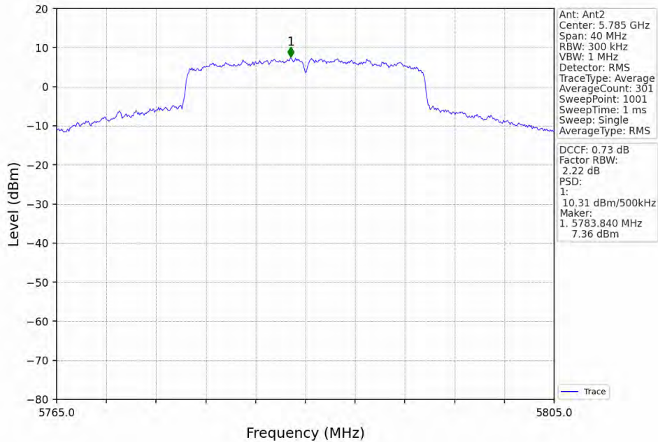
802.11ax(HEW20)_MCH_5785MHz_RU242_Left_MIMO_NTNV
