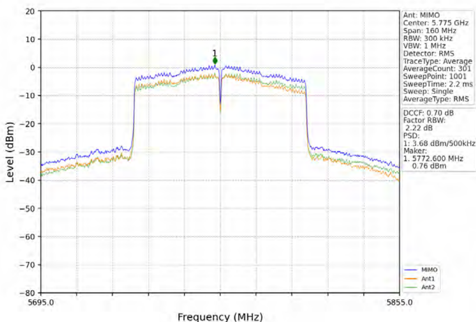
802.11ac(VHT80)_MCH_5775MHz_MIMO_NTNV
