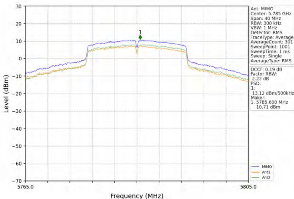
802.11ac(VHT20)_MCH_5785MHz_MIMO_NTNV
