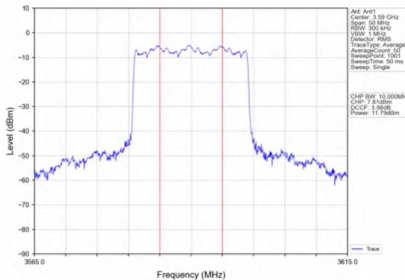
Band42c_20MHz_16QAM_HCH_3590MHz_RB_100_0_NTNV
