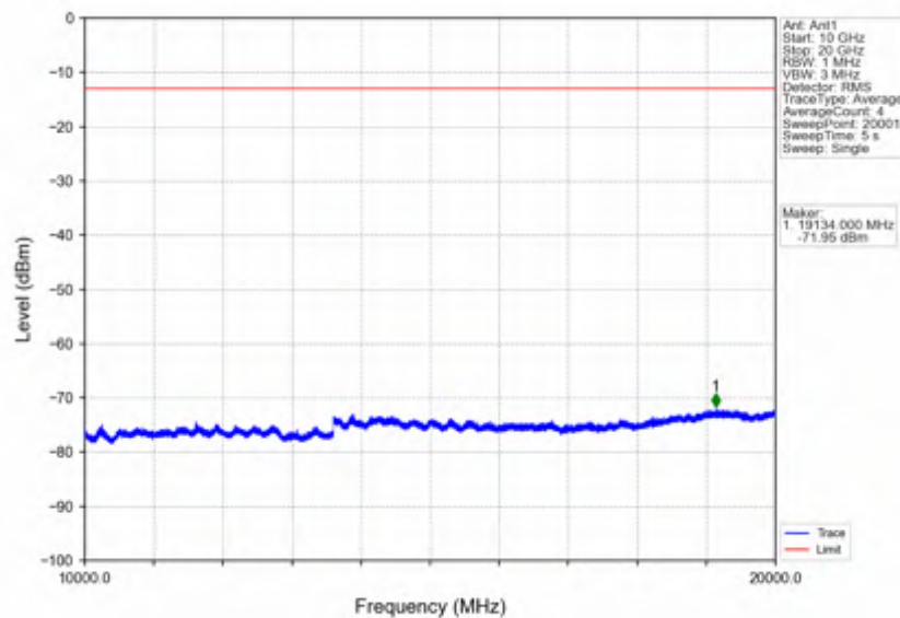
Band66_10MHz_QPSK_LCH_1715MHz_RB_50_0_NTNV
