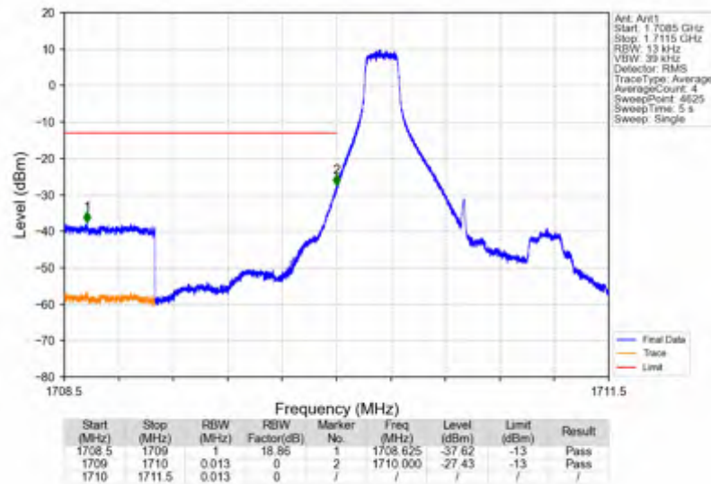
Band66_1.4MHz_256QAM_LCH_1710.7MHz_RB_6_0_NTNV
