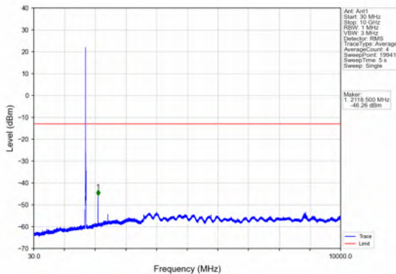
Band66_10MHz_64QAM_LCH_1715MHz_RB_1_0_NTNV
