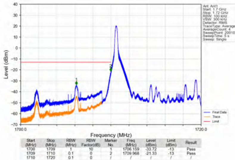
Band66_10MHz_QPSK_LCH_1715MHz_RB_50_0_NTNV
