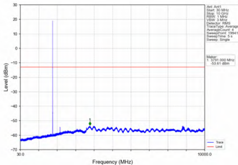
Band66_3MHz_256QAM_HCH_1778.5MHz_RB_1_0_NTNV
