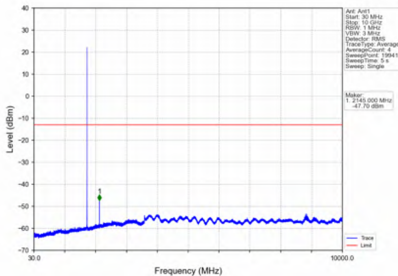
Band66_1.4MHz_64QAM_MCH_1745MHz_RB_1_0_NTNV
