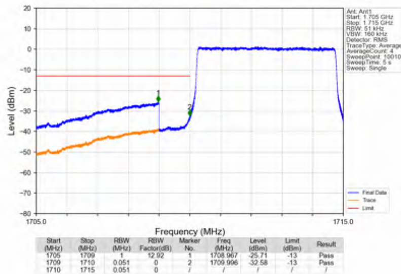
Band66_5MHz_256QAM_LCH_1712.5MHz_RB_25_0_NTNV
