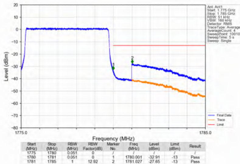
Band66_5MHz_256QAM_HCH_1777.5MHz_RB_25_0_NTNV
