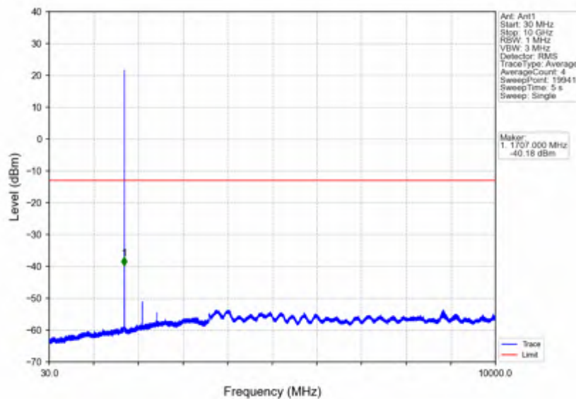
Band66 1.4MHz 64QAM LCH 1710.7MHz RB 1 0 NTNV
