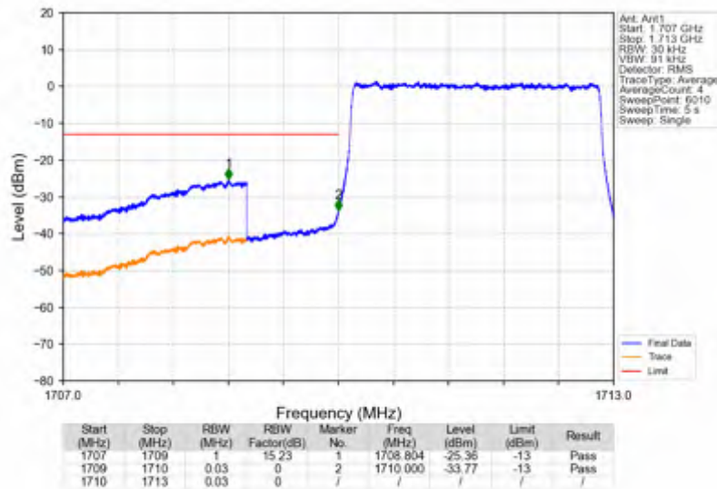
Band66_3MHz_256QAM_LCH_1711.5MHz_RB_15_0_NTNV
