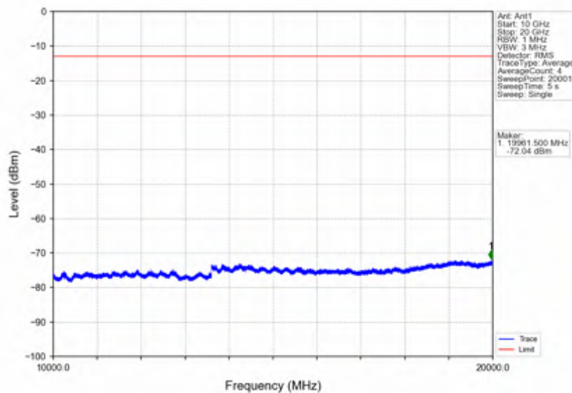
Band66_10MHz_16QAM_MCH_1745MHz_RB_1_0_NTNV
