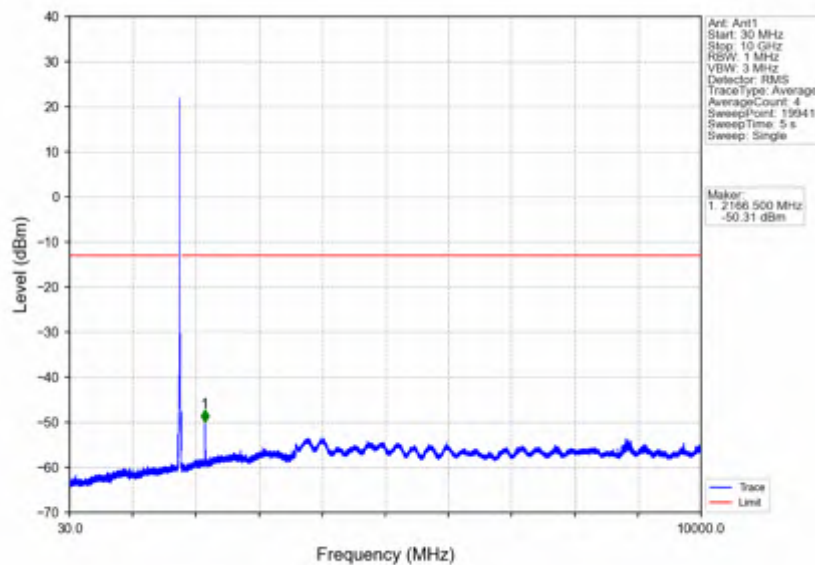
Band66_15MHz_16QAM_HCH_1772.5MHz_RB_1_0_NTNV
