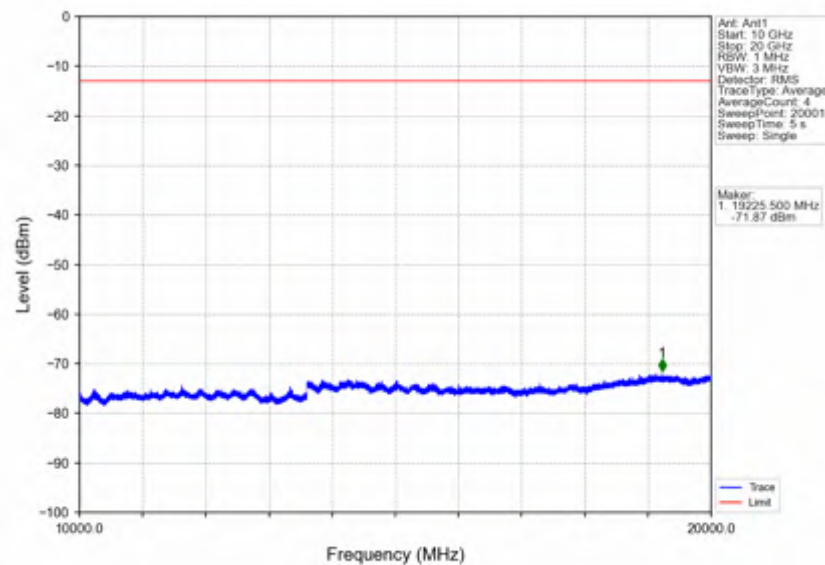
Band66_15MHz_16QAM_LCH_1717.5MHz_RB_75_0_NTNV
