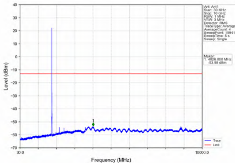
Band66_10MHz_QPSK_HCH_1775MHz_RB_1_0_NTNV
