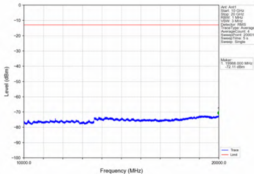
Band66_10MHz_256QAM_LCH_1715MHz_RB_50_0_NTNV
