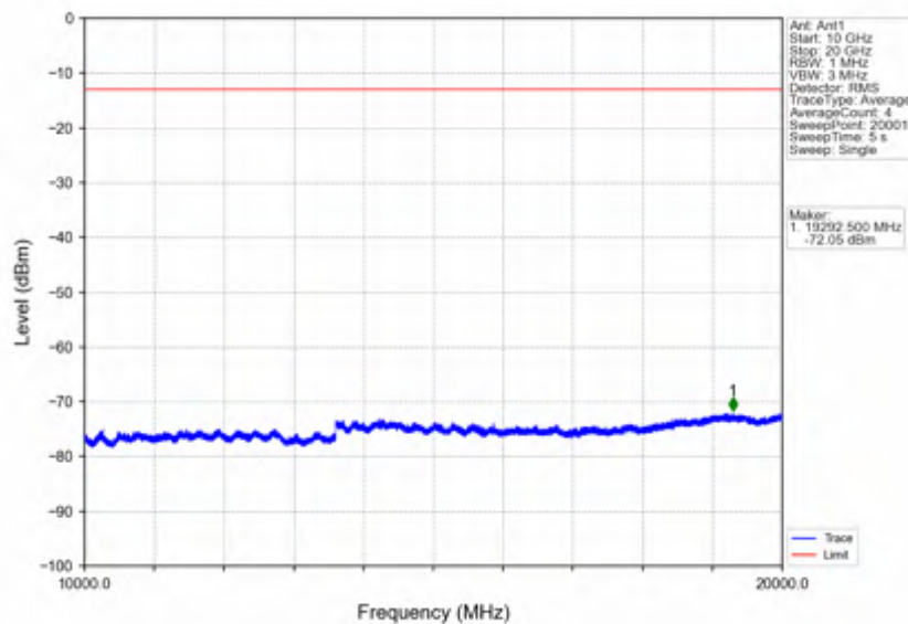
Band66_3MHz_QPSK_MCH_1745MHz_RB_1_0_NTNV
