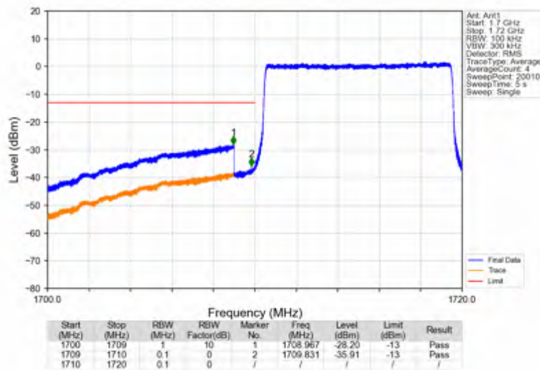
Band66_10MHz_256QAM_LCH_1715MHz_RB_50_0_NTNV
