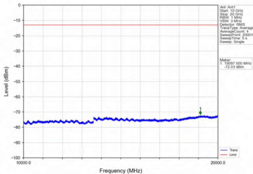
Band66_3MHz_256QAM_MCH_1745MHz_RB_1_0_NTNV
