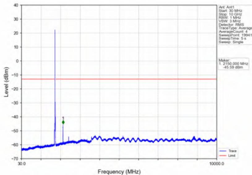
Band66_15MHz_16QAM_MCH_1745MHz_RB_1_0_NTNV
