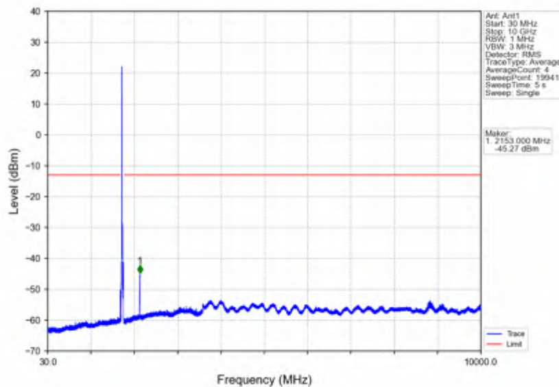
Band66_20MHz_64QAM_MCH_1745MHz_RB_1_0_NTNV
