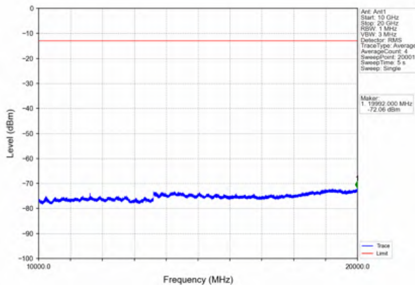
Band66_3MHz_256QAM_HCH_1778.5MHz_RB_1_0_NTNV
