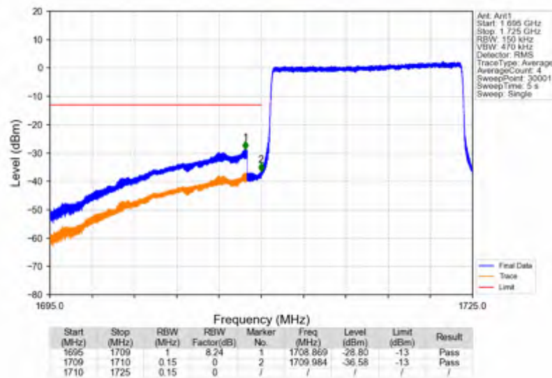
Band66_15MHz_256QAM_LCH_1717.5MHz_RB_75_0_NTNV
