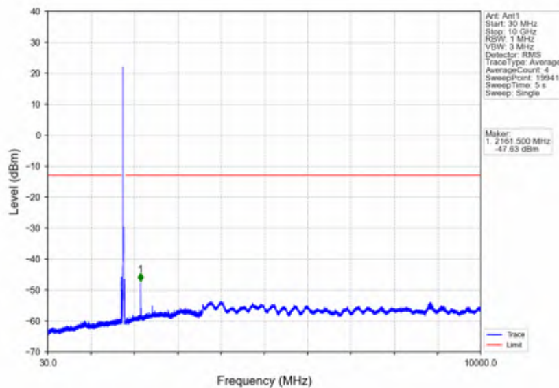
Band66_20MHz_64QAM_HCH_1770MHz_RB_1_0_NTNV
