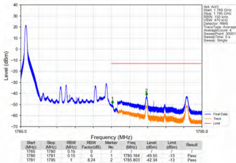
Band66_15MHz_QPSK_HCH_1772.5MHz_RB_75_0_NTNV
