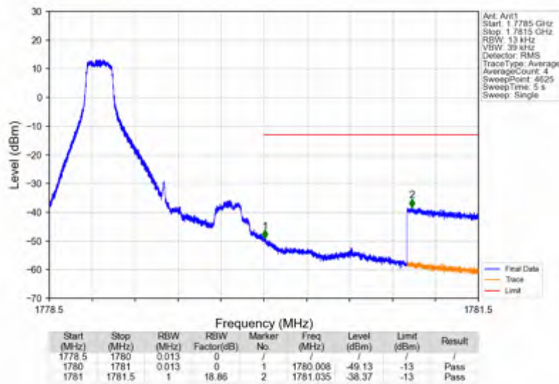
Band66_1.4MHz_16QAM_HCH_1779.3MHz_RB_6_0_NTNV
