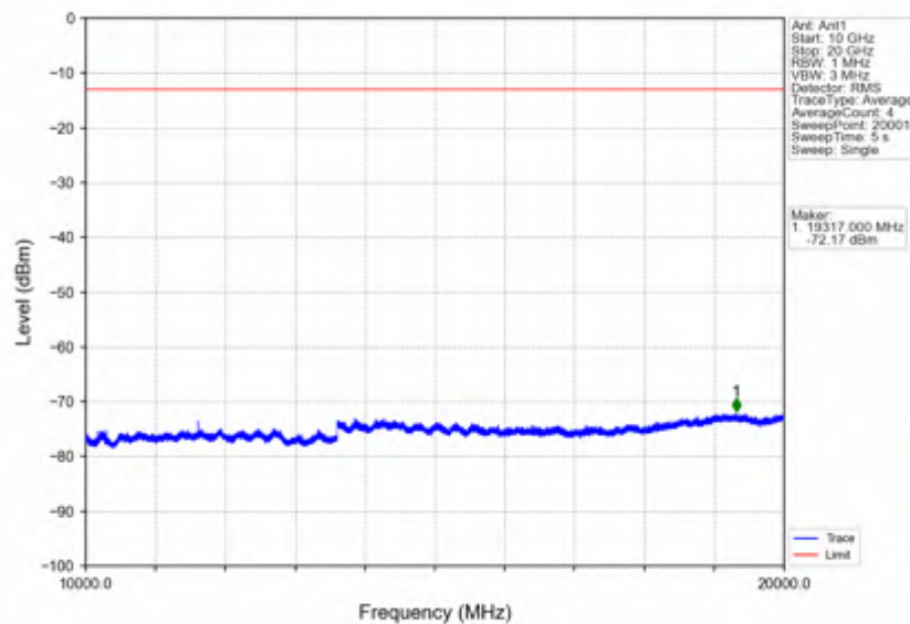
Band66_15MHz_QPSK_LCH_1717.5MHz_RB_75_0_NTNV
