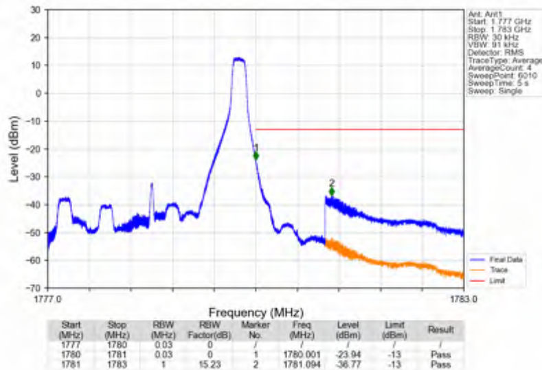
Band66_3MHz_256QAM_HCH_1778.5MHz_RB_1_14_NTNV
