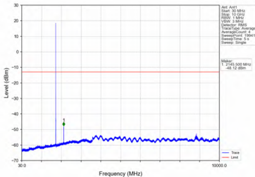
Band66_3MHz_256QAM_MCH_1745MHz_RB_1_0_NTNV
