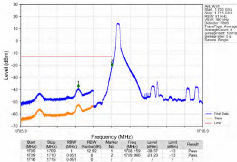
Band66_5MHz_256QAM_LCH_1712.5MHz_RB_1_0_NTNV
