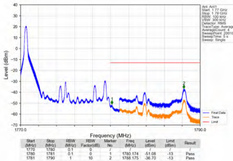
Band66_10MHz_64QAM_HCH_1775MHz_RB_50_0_NTNV
