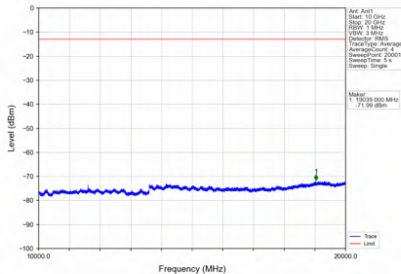
Band66 10MHz 16QAM LCH 1715MHz RB 50 0 NTNV
