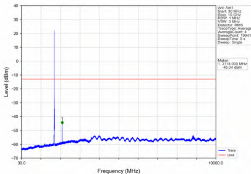
Band66 10MHz QPSK LCH 1715MHz RB 1 0 NTNV
