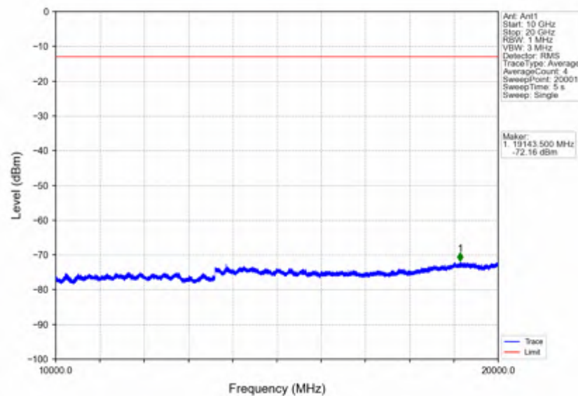
Band66_5MHz_256QAM_LCH_1712.5MHz_RB_25_0_NTNV
