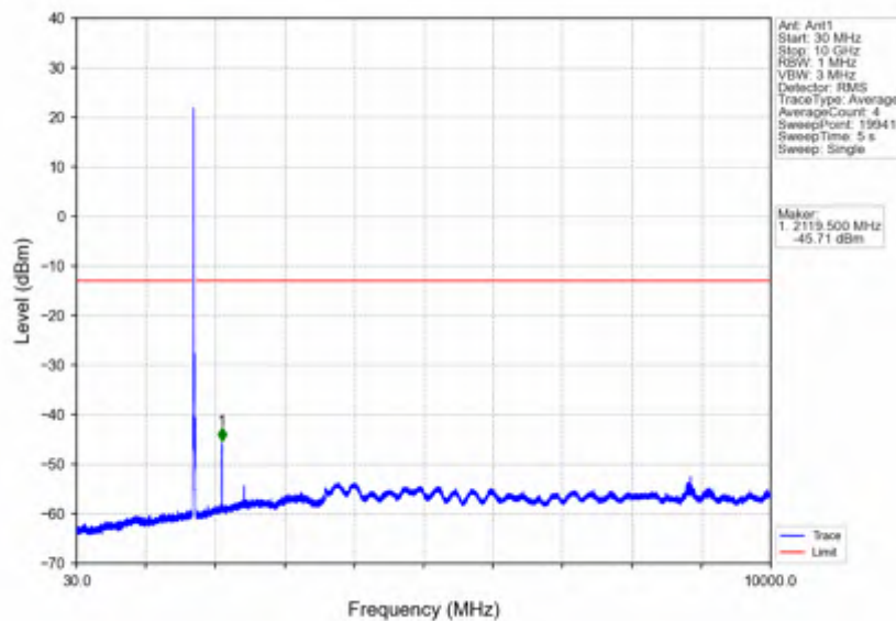
Band66_15MHz_64QAM_LCH_1717.5MHz_RB_1_0_NTNV
