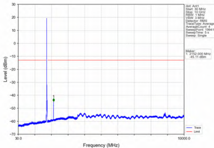
Band66_20MHz_256QAM_MCH_1745MHz_RB_1_0_NTNV
