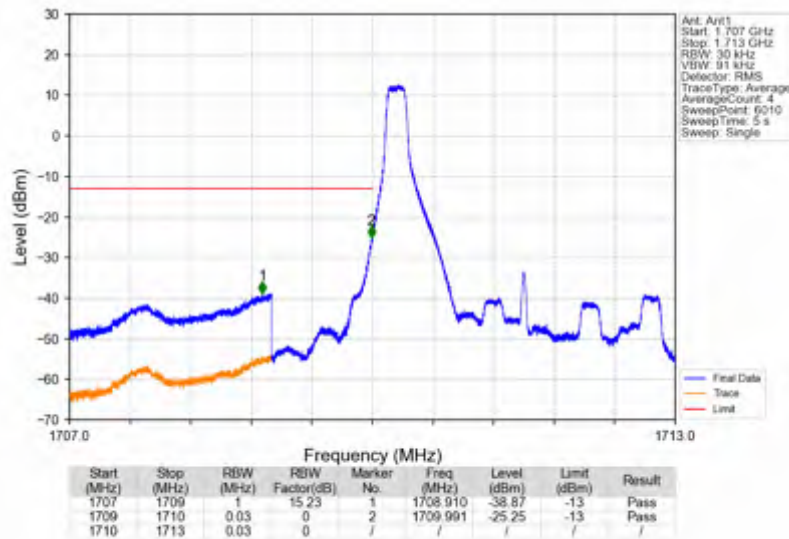
Band66 3MHz 256QAM LCH 1711.5MHz RB 1 0 NTNV
