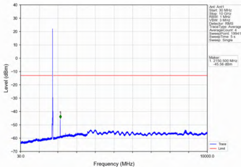
Band66_15MHz_64QAM_MCH_1745MHz_RB_1_0_NTNV
