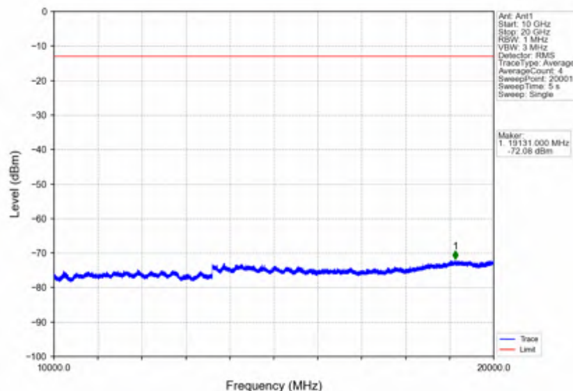
Band66 1.4MHz 256QAM HCH 1779.3MHz RB 1 0 NTNV
