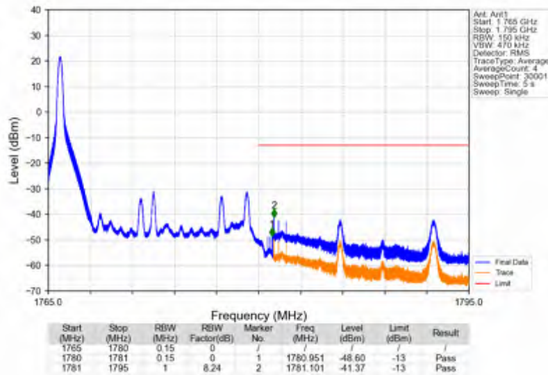
Band66_15MHz_16QAM_HCH_1772.5MHz_RB_1_74_NTNV
