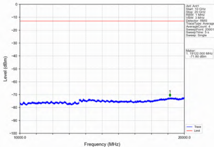
Band66_15MHz_QPSK_MCH_1745MHz_RB_1_0_NTNV
