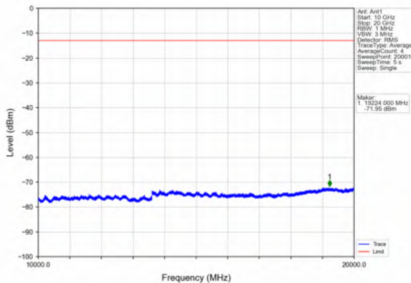
Band66_20MHz_64QAM_MCH_1745MHz_RB_1_0_NTNV
