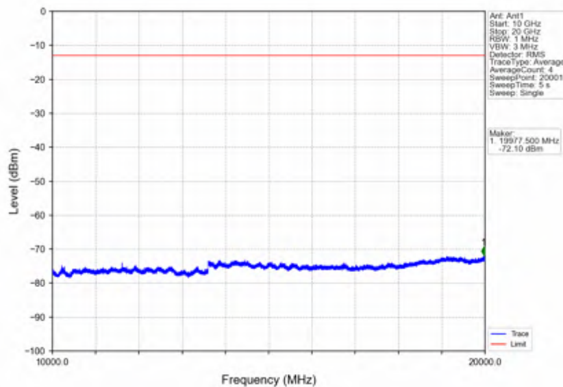
Band66_15MHz_64QAM_MCH_1745MHz_RB_1_0_NTNV
