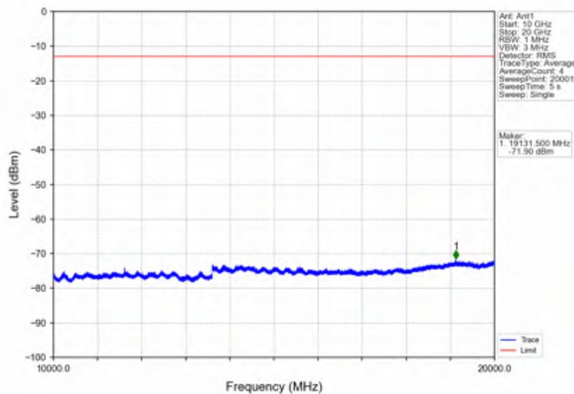
Band66_10MHz_16QAM_HCH_1775MHz_RB_1_0_NTV
