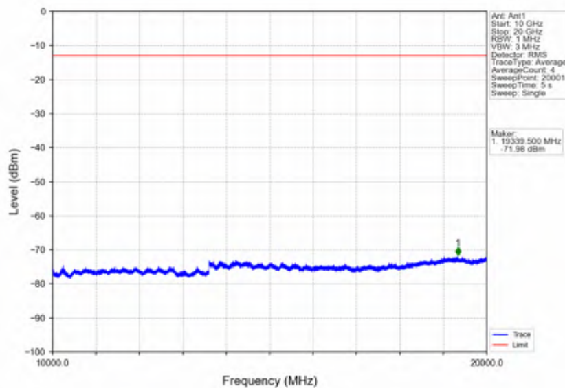
Band66_5MHz_256QAM_HCH_1777.5MHz_RB_1_0_NTNV
