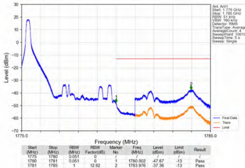
Band66_5MHz_16QAM_HCH_1777.5MHz_RB_1_24_NTNV
