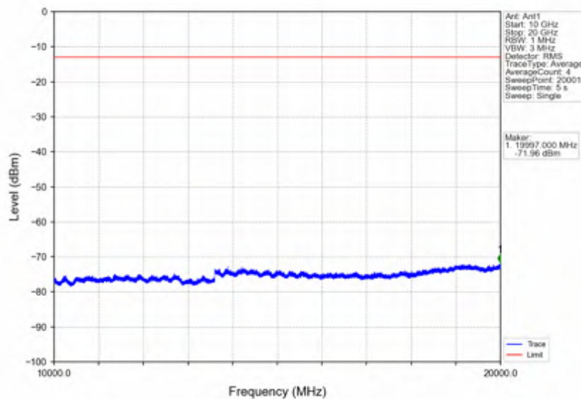
Band66_5MHz_256QAM_MCH_1745MHz_RB_1_0_NTNV
