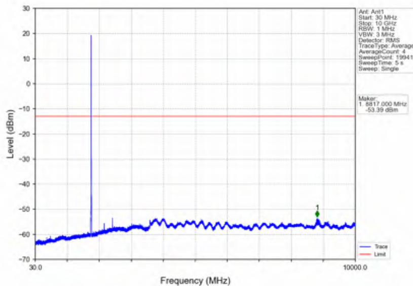
Band66_10MHz_256QAM_HCH_1775MHz_RB_1_0_NTNV
