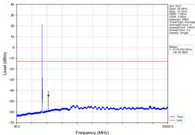
Band66_15MHz_QPSK_LCH_1717.5MHz_RB_1_0_NTNV
