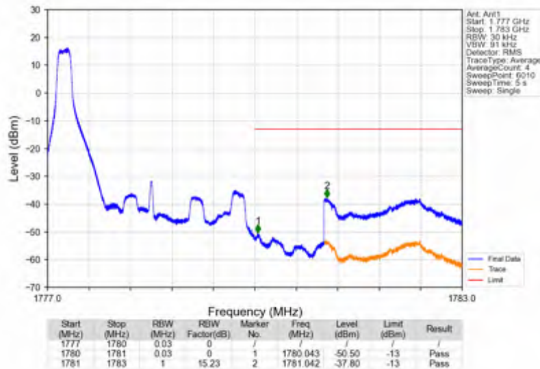
Band66_3MHz_64QAM_HCH_1778.5MHz_RB_1_14_NTNV
