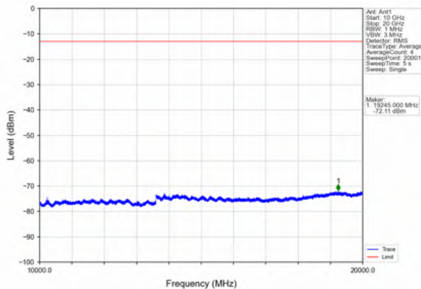
Band66_10MHz_64QAM_LCH_1715MHz_RB_50_0_NTNV
