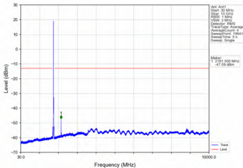
Band66_20MHz_256QAM_HCH_1770MHz_RB_1_0_NTNV
