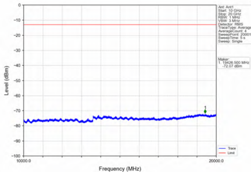
Band66_3MHz_16QAM_LCH_1711.5MHz_RB_15_0_NTNV
