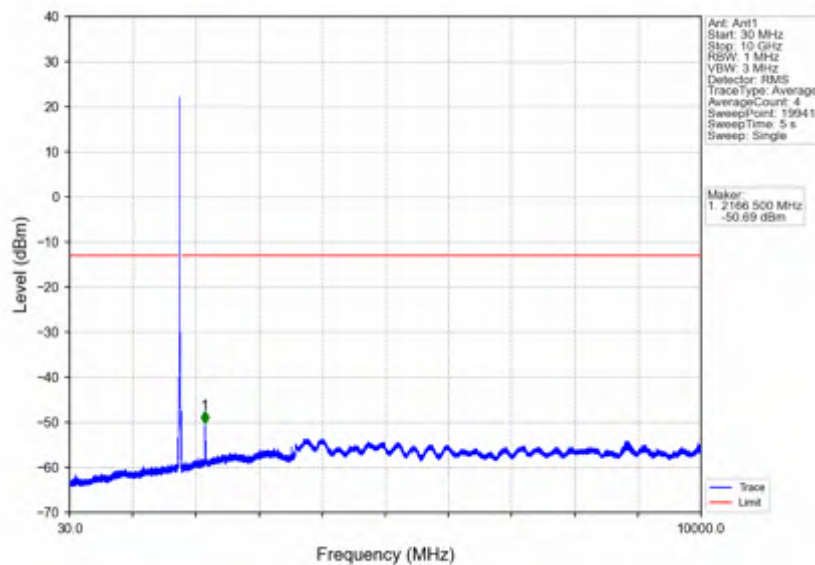
Band66_15MHz_64QAM_HCH_1772.5MHz_RB_1_0_NTNV
