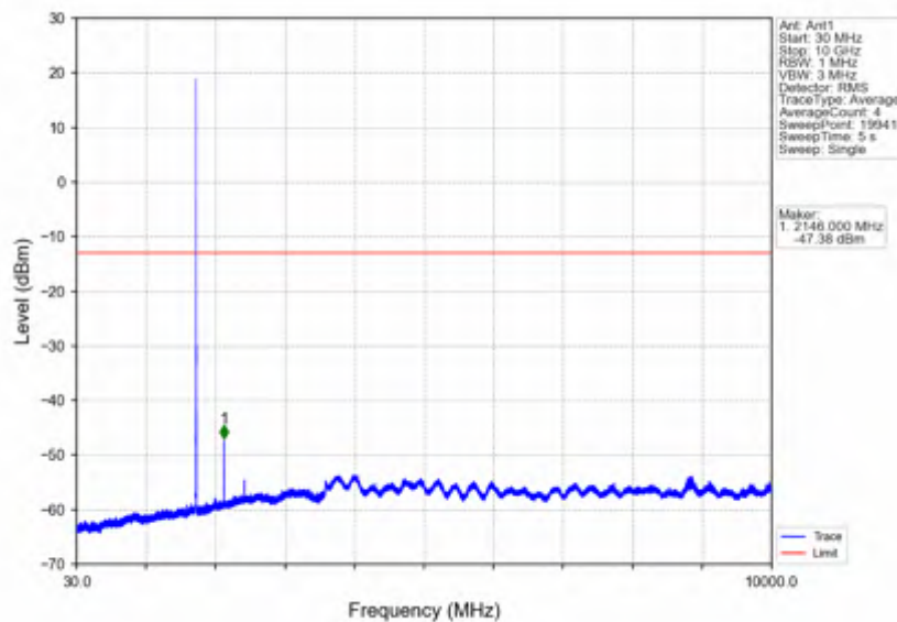
Band66_5MHz_256QAM_MCH_1745MHz_RB_1_0_NTNV
