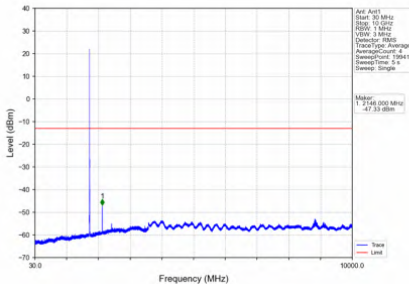
Band66_5MHz_QPSK_MCH_1745MHz_RB_1_0_NTNV
