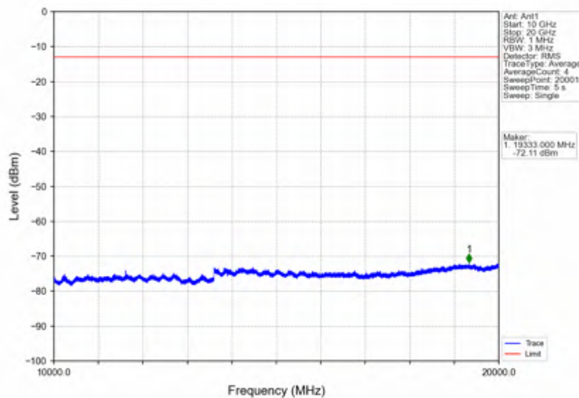
Band66 20MHz 16QAM MCH 1745MHz RB 1 0 NTNV
