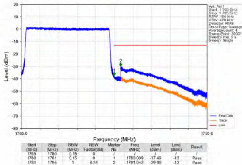
Band66_15MHz_256QAM_HCH_1772.5MHz_RB_75_0_NTNV
