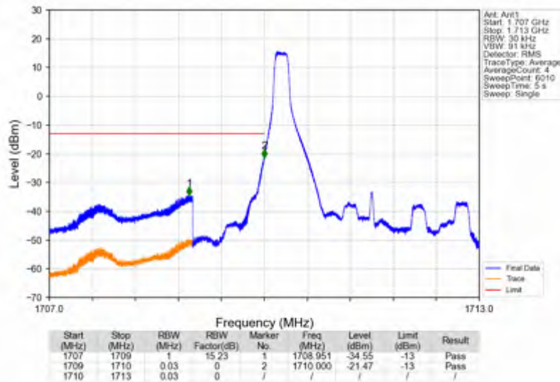
Band66_3MHz_16QAM_LCH_1711.5MHz_RB_15_0_NTNV
