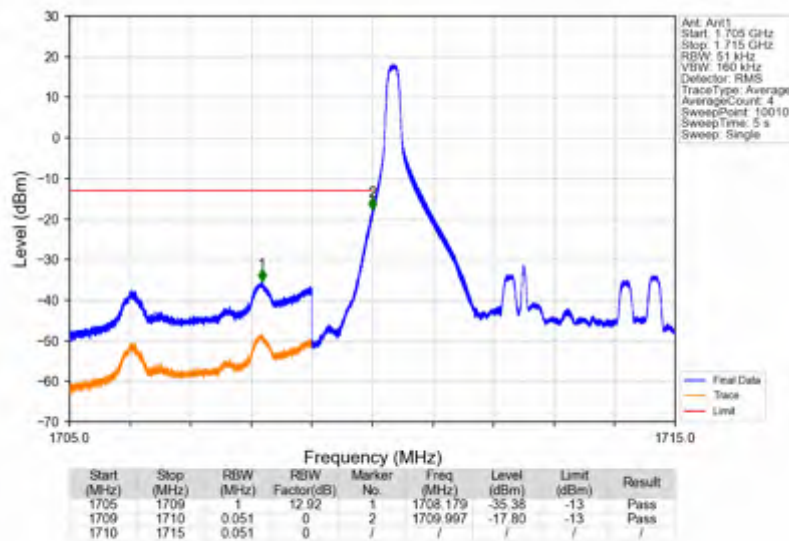
Band66_5MHz_64QAM_LCH_1712.5MHz_RB_25_0_NTNV
