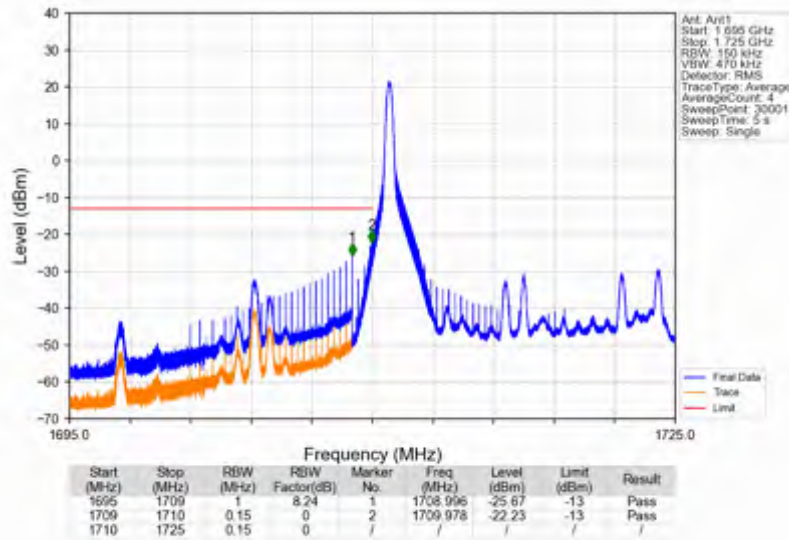
Band66_15MHz_QPSK_LCH_1717.5MHz_RB_1_0_NTNV
