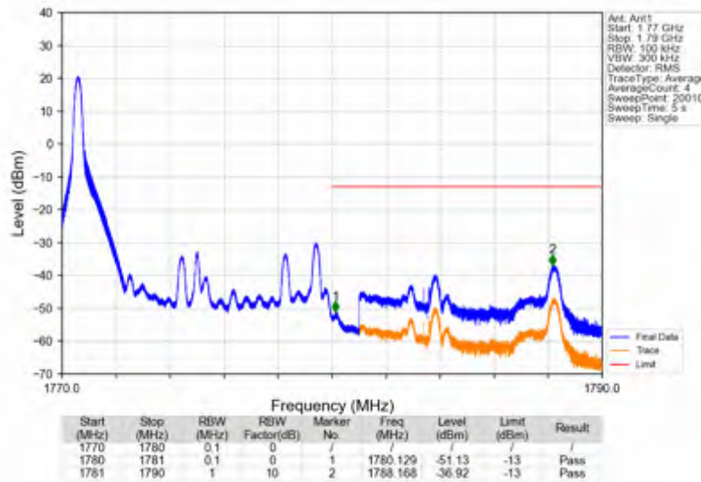
Band66_10MHz_16QAM_HCH_1775MHz_RB_50_0_NTNV
