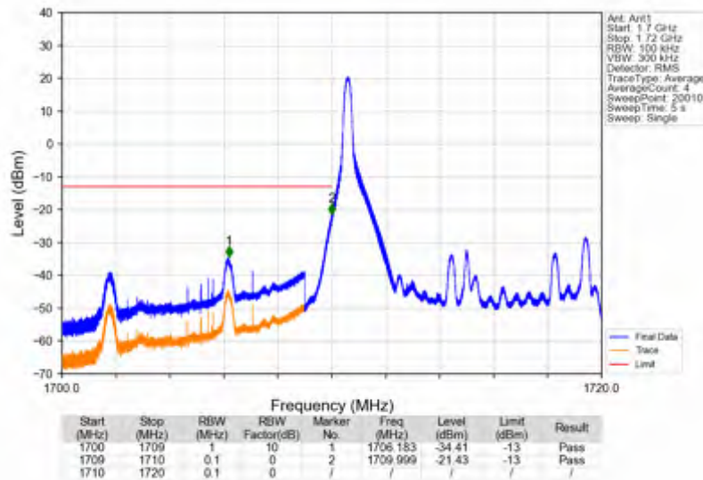
Band66_10MHz_64QAM_LCH_1715MHz_RB_50_0_NTNV
