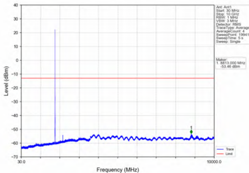
Band66_5MHz_64QAM_HCH_1777.5MHz_RB_1_0_NTNV
