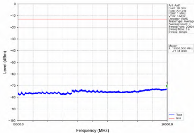
Band66_15MHz_16QAM_MCH_1745MHz_RB_1_0_NTNV
