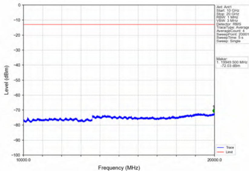
Band66_1.4MHz_64QAM_LCH_1710.7MHz_RB_6_0_NTNV
