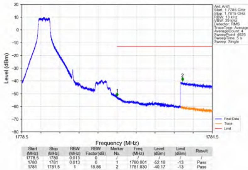
Band66_1.4MHz_256QAM_HCH_1779.3MHz_RB_1_5_NTNV
