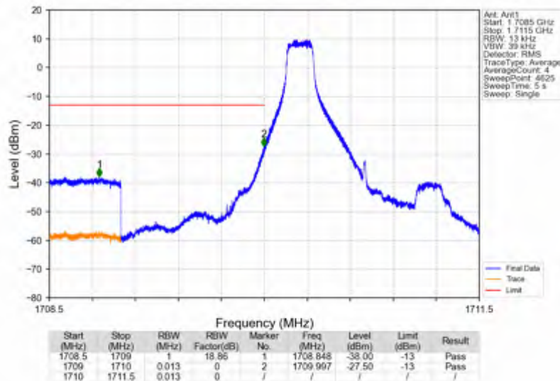
Band66_1.4MHz_256QAM_LCH_1710.7MHz_RB_1_0_NTNV
