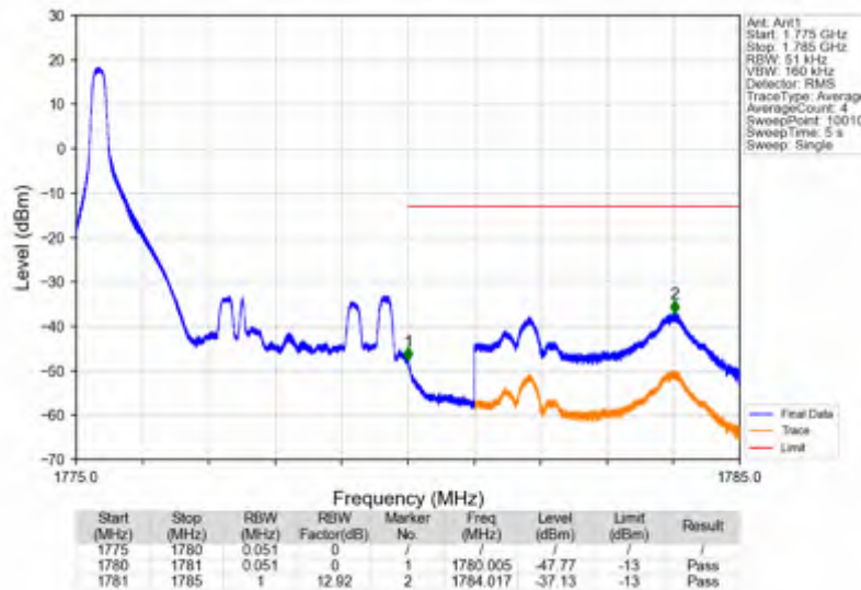
Band66_5MHz_16QAM_HCH_1777.5MHz_RB_25_0_NTNV
