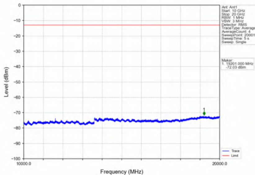
Band66_15MHz_16QAM_HCH_1772.5MHz_RB_1_0_NTNV
