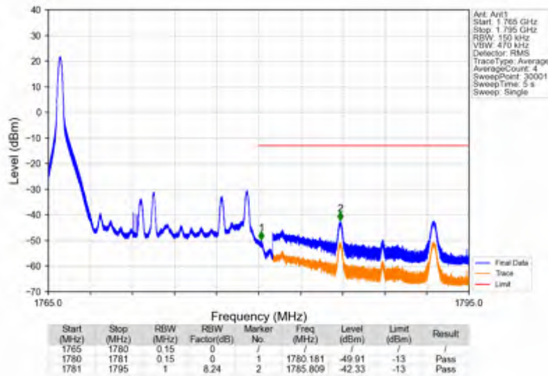
Band66_15MHz_QPSK_HCH_1772.5MHz_RB_1_74_NTNV
