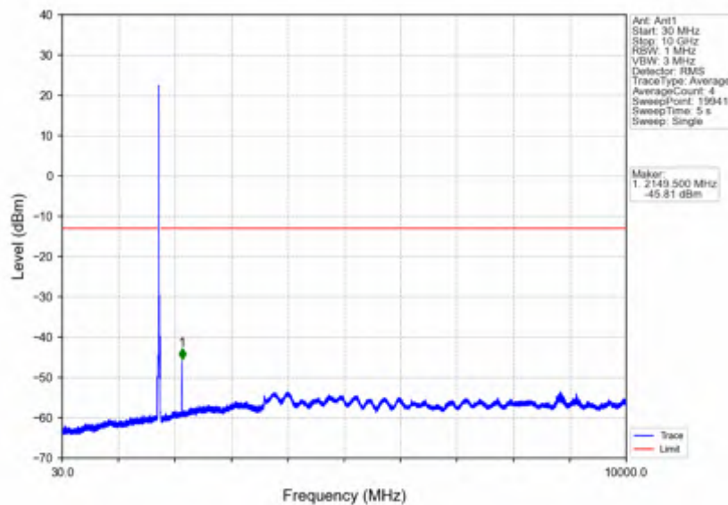
Band66_15MHz_QPSK_MCH_1745MHz_RB_1_0_NTNV
