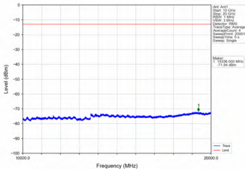
Band66_1.4MHz_64QAM_HCH_1779.3MHz_RB_1_0_NTNV
