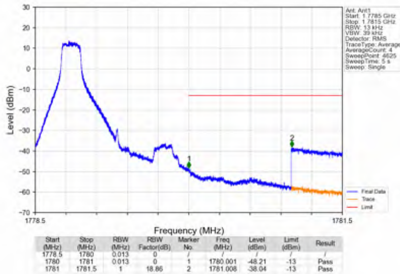
Band66_1.4MHz_64QAM_HCH_1779.3MHz_RB_1_5_NTNV
