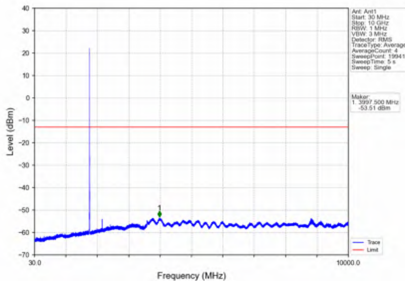
Band66_5MHz_QPSK_HCH_1777.5MHz_RB_1_0_NTNV
