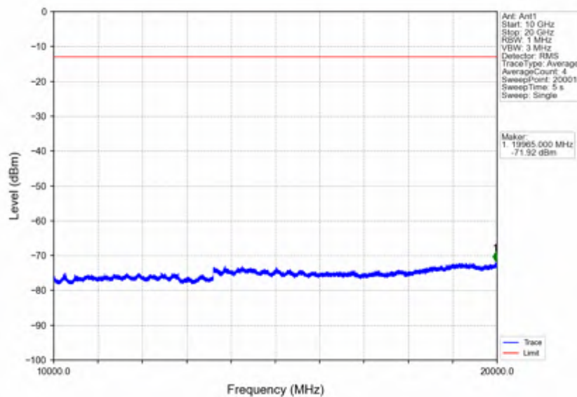
Band66_10MHz_QPSK_MCH_1745MHz_RB_1_0_NTNV
