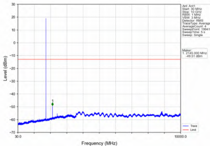
Band66_1.4MHz_256QAM_MCH_1745MHz_RB_1_0_NTNV
