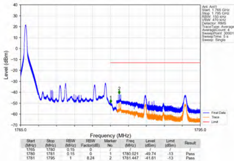
Band66_15MHz_16QAM_HCH_1772.5MHz_RB_75_0_NTNV
