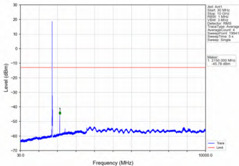
Band66_15MHz_256QAM_MCH_1745MHz_RB_1_0_NTNV
