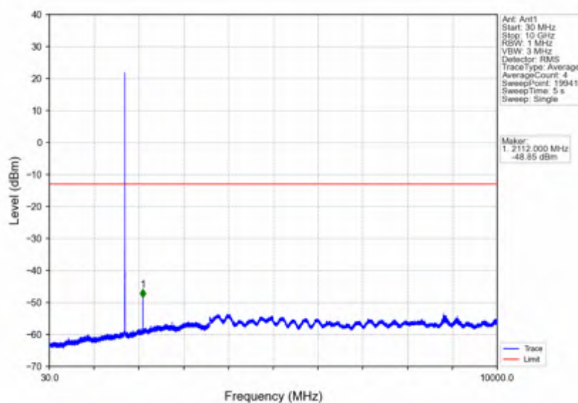
Band66_3MHz_QPSK_LCH_1711.5MHz_RB_1_0_NTNV
