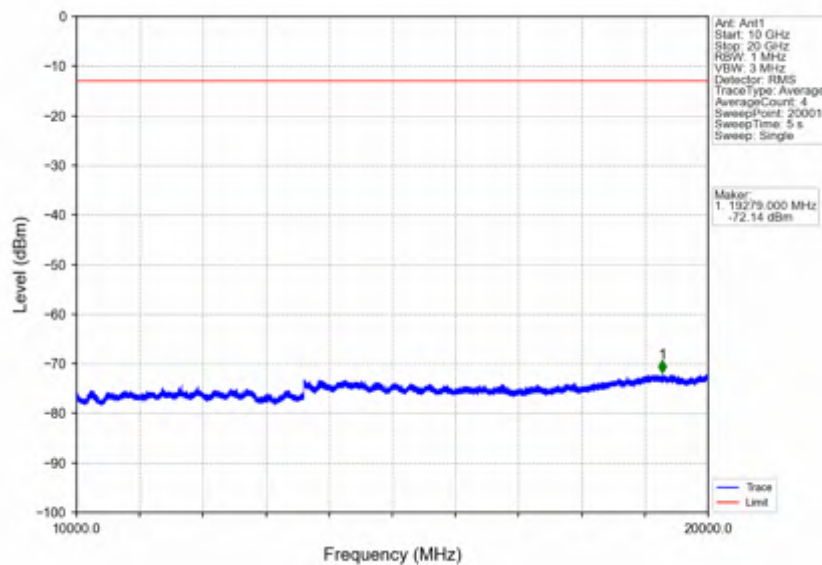
Band66_10MHz_64QAM_HCH_1775MHz_RB_1_0_NTNV
