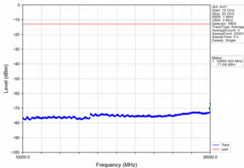
Band66_5MHz_64QAM_MCH_1745MHz_RB_1_0_NTNV
