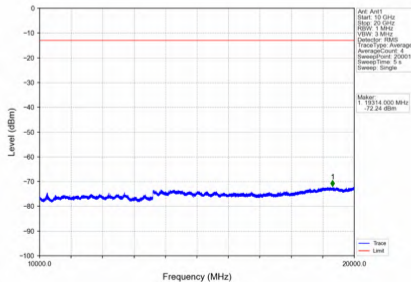
Band66_20MHz_64QAM_LCH_1720MHz_RB_100_0_NTNV
