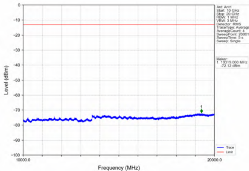
Band66_20MHz_256QAM_HCH_1770MHz_RB_1_0_NTNV
