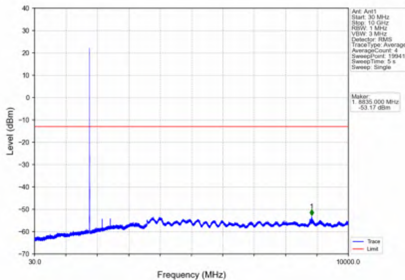
Band66_5MHz_16QAM_HCH_1777.5MHz_RB_1_0_NTNV
