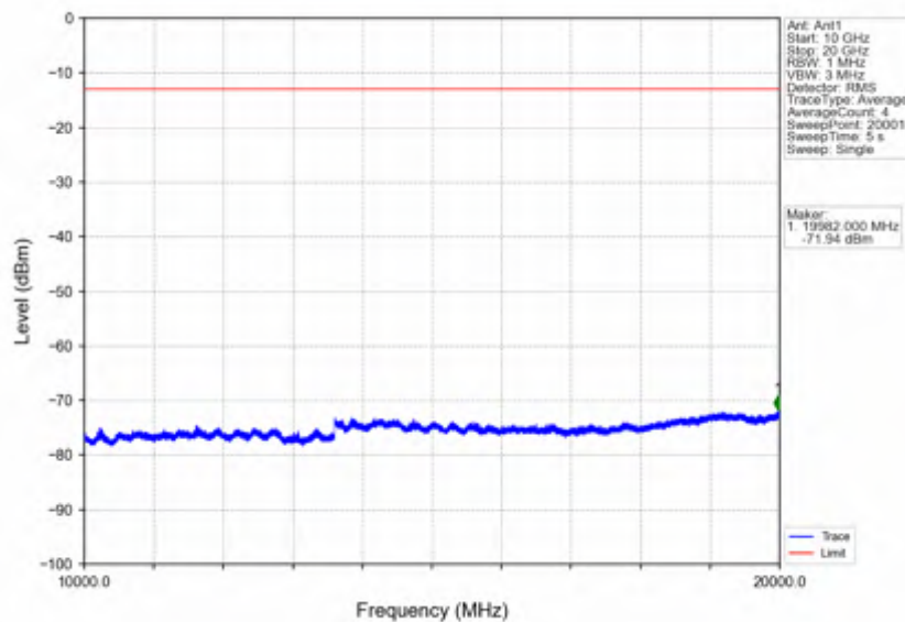
Band66_10MHz_QPSK_HCH_1775MHz_RB_1_0_NTNV
