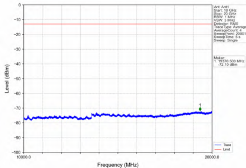
Band66_3MHz_64QAM_LCH_1711.5MHz_RB_15_0_NTNV
