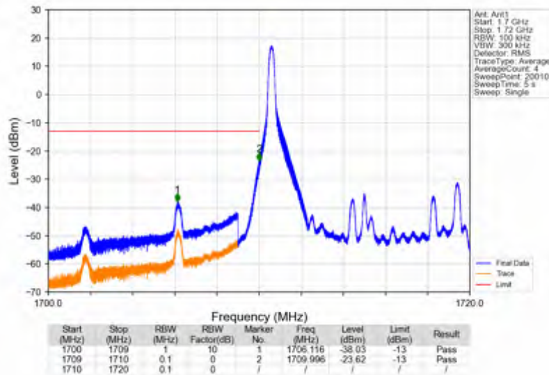
Band66 10MHz 256QAM LCH 1715MHz RB 1 0 NTNV
