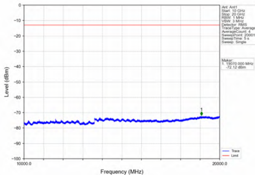
Band66_5MHz_64QAM_LCH_1712.5MHz_RB_25_0_NTNV
