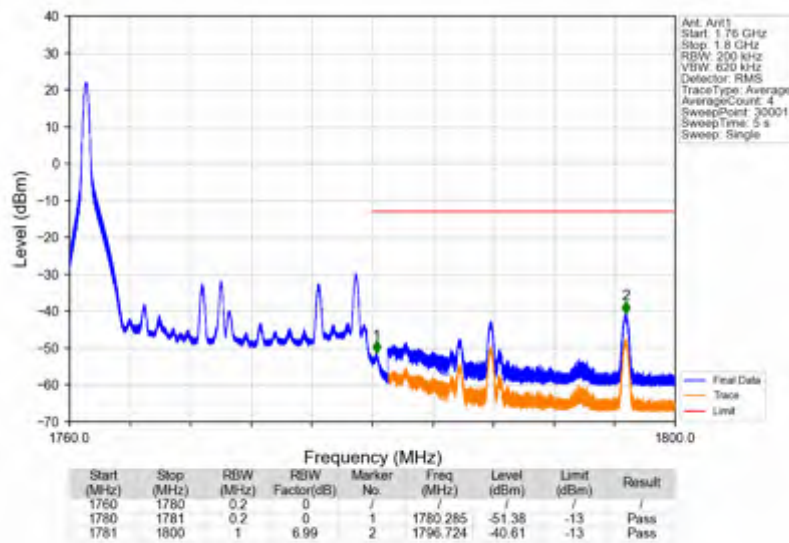
Band66_20MHz_64QAM_HCH_1770MHz_RB_100_0_NTNV
