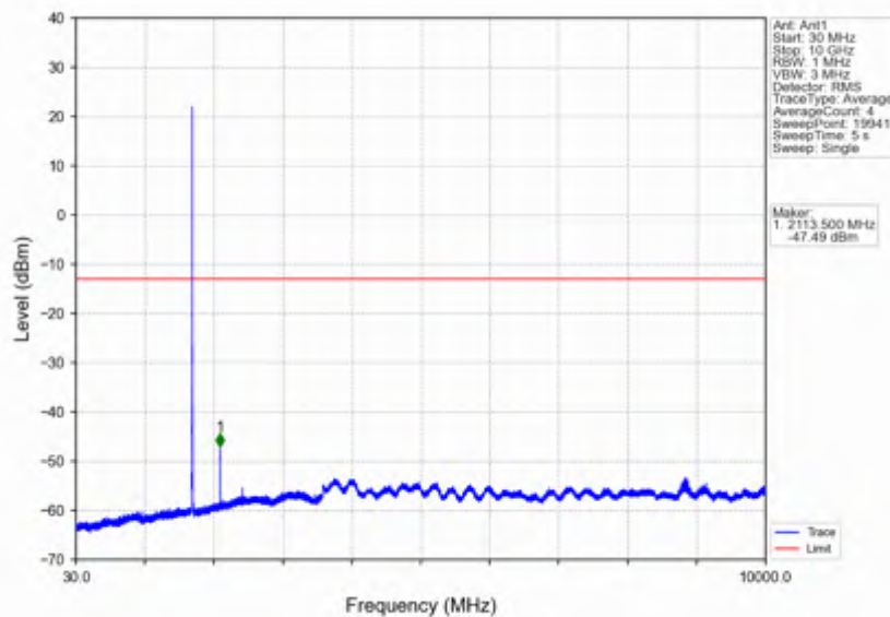
Band66_5MHz_64QAM_LCH_1712.5MHz_RB_1_0_NTNV
