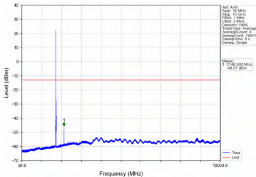
Band66_10MHz_QPSK_MCH_1745MHz_RB_1_0_NTNV
