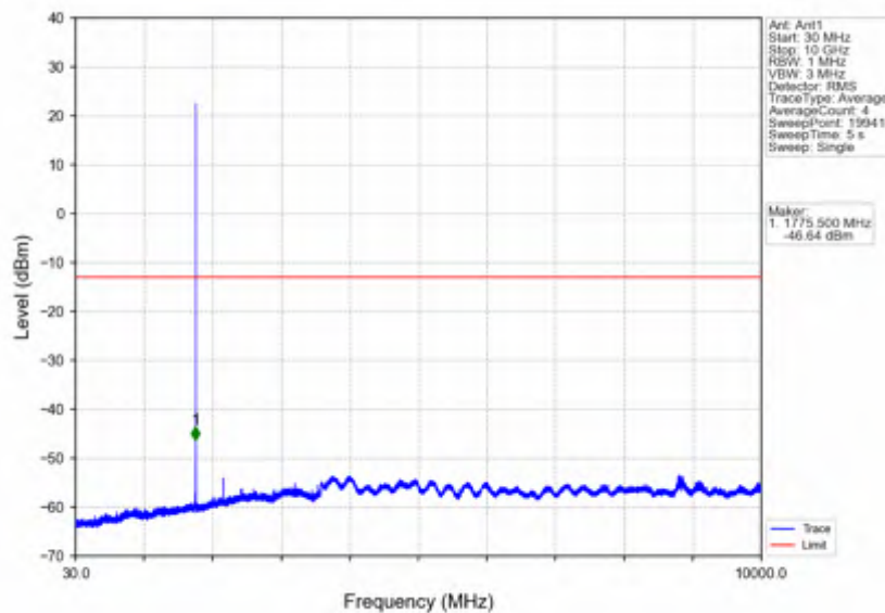
Band66_1.4MHz_64QAM_HCH_1779.3MHz_RB_1_0_NTNV
