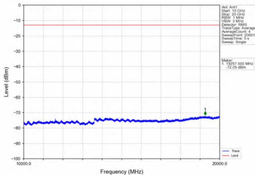
Band66_5MHz_64QAM_HCH_1777.5MHz_RB_1_0_NTNV
