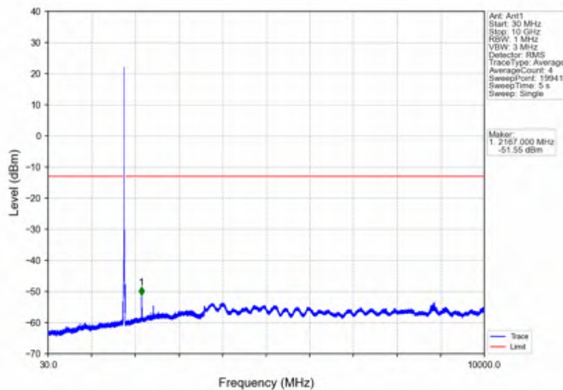
Band66_15MHz_QPSK_HCH_1772.5MHz_RB_1_0_NTNV
