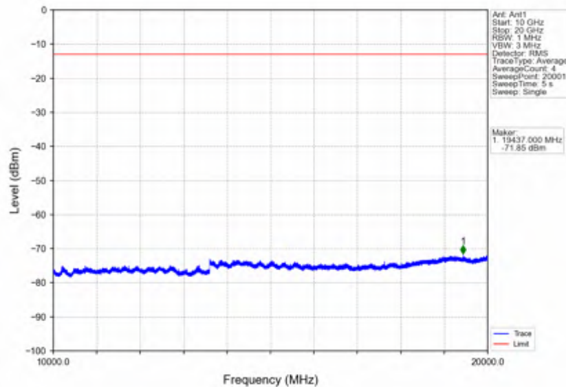
Band66_3MHz_QPSK_LCH_1711.5MHz_RB_15_0_NTNV
