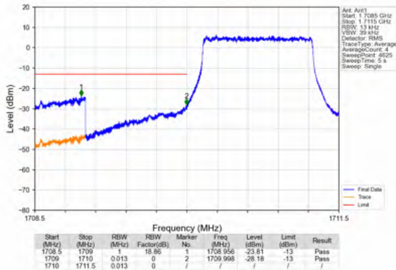
Band66 1.4MHz 64QAM LCH 1710.7MHz RB 1 0 NTNv
