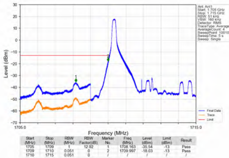
Band66_5MHz_16QAM_LCH_1712.5MHz_RB_25_0_NTNV
