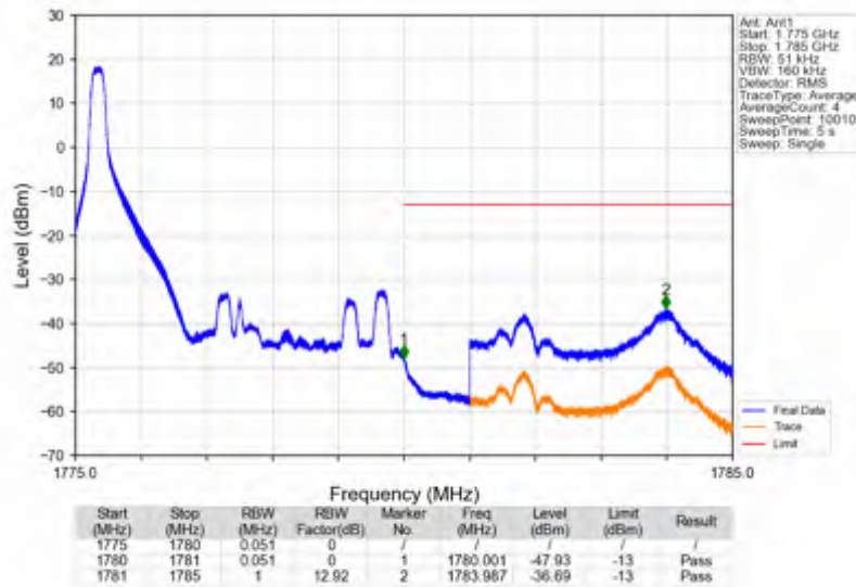
Band66_5MHz_64QAM_HCH_1777.5MHz_RB_1_24_NTNV
