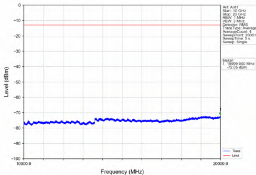
Band66_10MHz_256QAM_HCH_1775MHz_RB_1_0_NTNV
