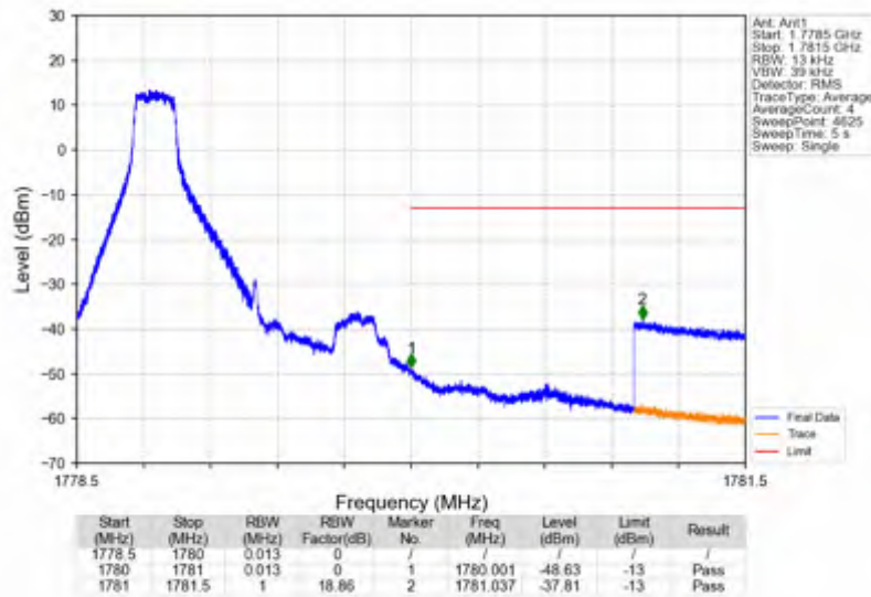
Band66_1.4MHz_64QAM_HCH_1779.3MHz_RB_6_0_NTNV
