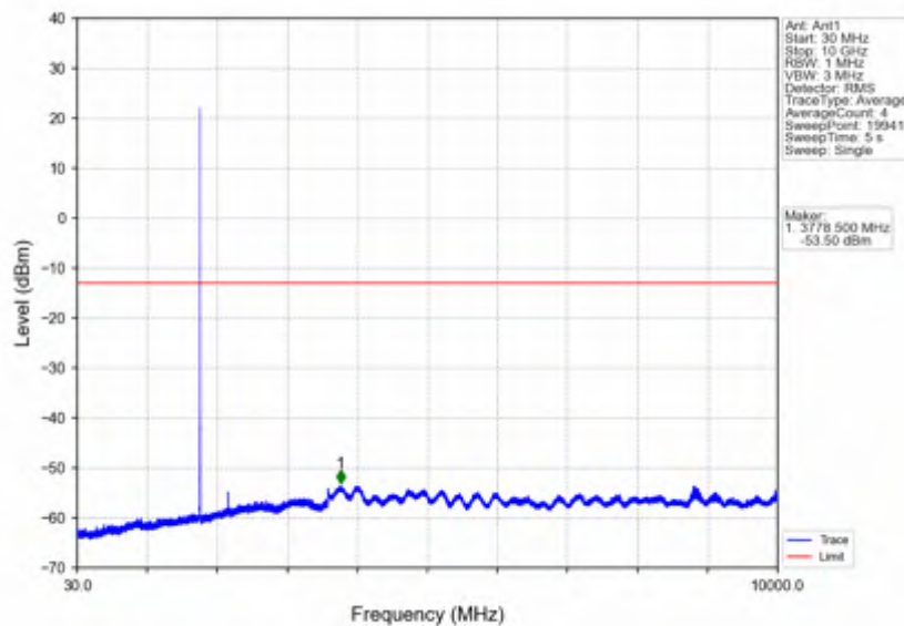
Band66_3MHz_64QAM_HCH_1778.5MHz_RB_1_0_NTNV
