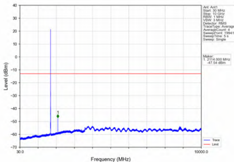
Band66_5MHz_QPSK_LCH_1712.5MHz_RB_1_0_NTNV
