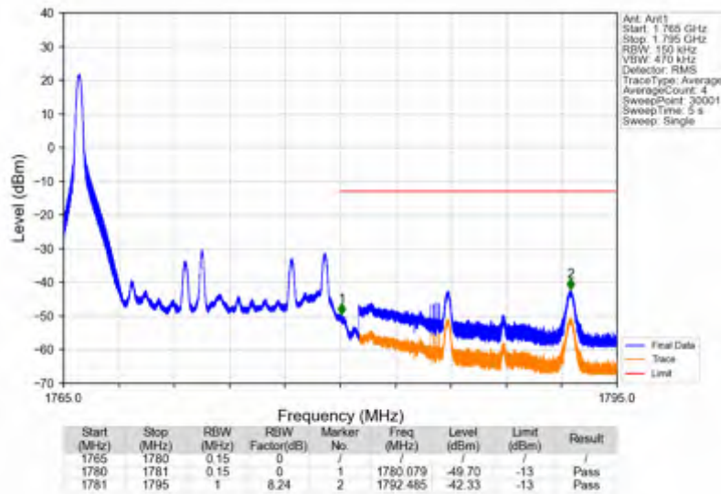
Band66_15MHz_64QAM_HCH_1772.5MHz_RB_1_74_NTNV
