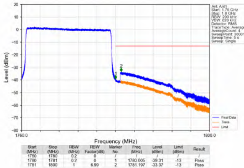
Band66_20MHz_256QAM_HCH_1770MHz_RB_100_0_NTNV
