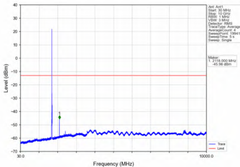
Band66_10MHz_16QAM_LCH_1715MHz_RB_1_0_NTNV
