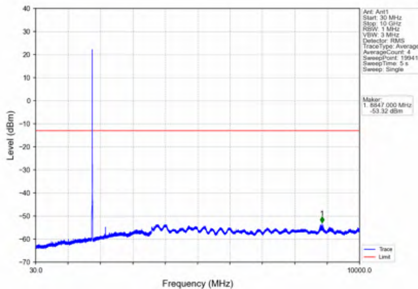
Band66_10MHz_16QAM_HCH_1775MHz_RB_1_0_NTV
