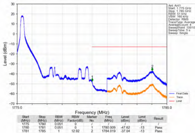
Band66_5MHz_64QAM_HCH_1777.5MHz_RB_25_0_NTNV
