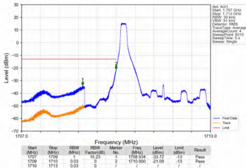
Band66_3MHz_QPSK_LCH_1711.5MHz_RB_1_0_NTNV
