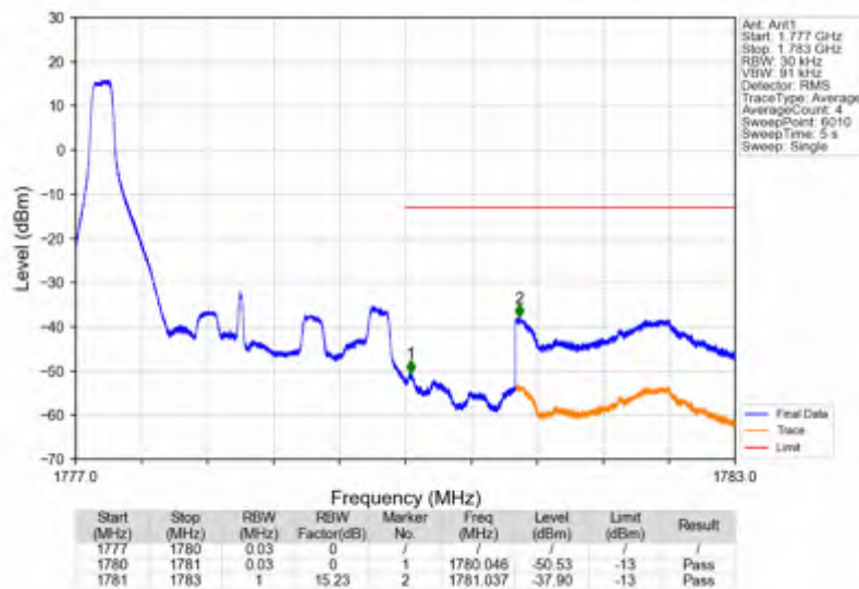
Band66_3MHz_64QAM_HCH_1778.5MHz_RB_15_0_NTNV
