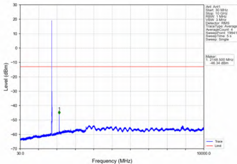
Band66_10MHz_256QAM_MCH_1745MHz_RB_1_0_NTNV
