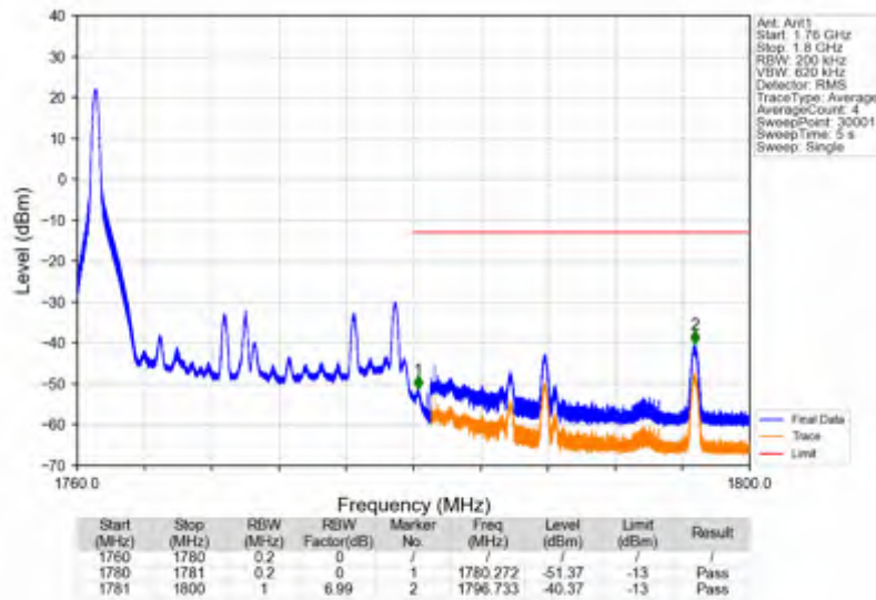
Band66_20MHz_64QAM_HCH_1770MHz_RB_1_99_NTNV
