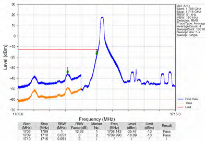
Band66_5MHz_QPSK_LCH_1712.5MHz_RB_25_0_NTNV
