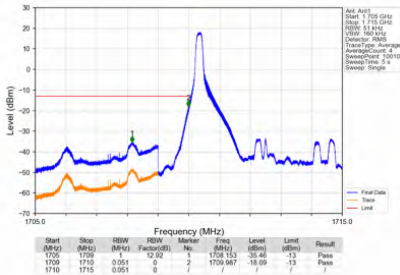
Band66_5MHz_QPSK_LCH_1712.5MHz_RB_1_0_NTNV
