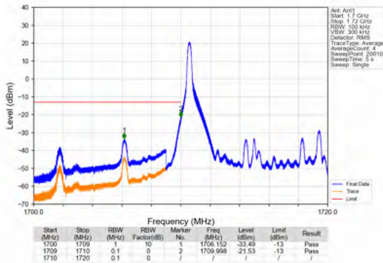
Band66 10MHz QPSK LCH 1715MHz RB 1 0 NTNV
