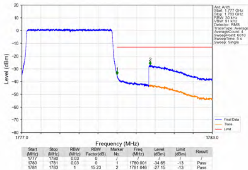
Band66_3MHz_256QAM_HCH_1778.5MHz_RB_15_0_NTNV
