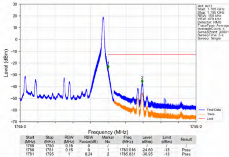
Band66_15MHz_256QAM_HCH_1772.5MHz_RB_1_74_NTNV
