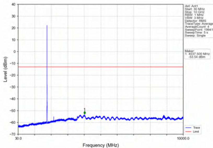
Band66_10MHz_64QAM_HCH_1775MHz_RB_1_0_NTNV
