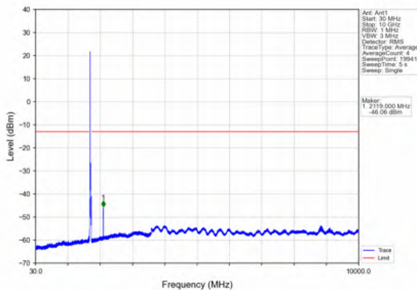
Band66_20MHz_16QAM_LCH_1720MHz_RB_1_0_NTV
