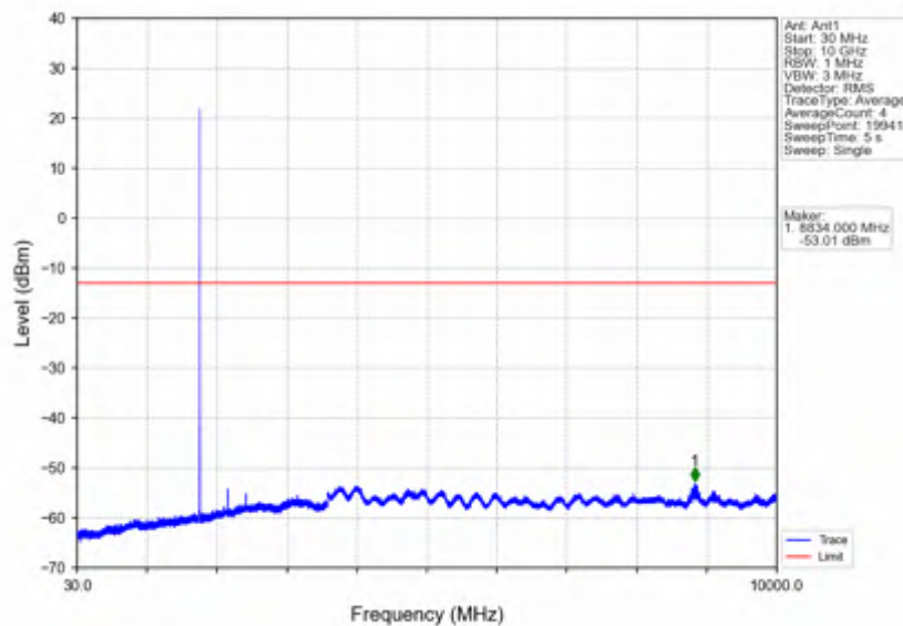
Band66_3MHz_QPSK_HCH_1778.5MHz_RB_1_0_NTNV
