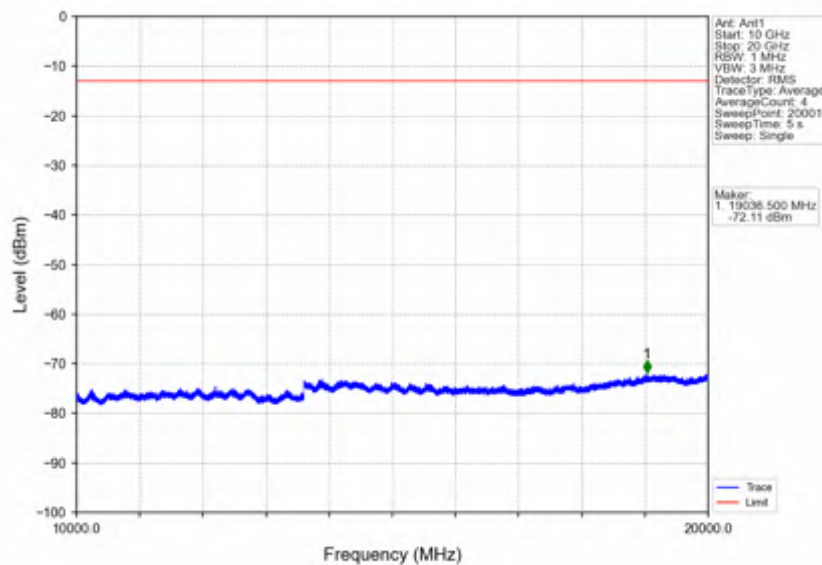
Band66_15MHz_256QAM_MCH_1745MHz_RB_1_0_NTNV
