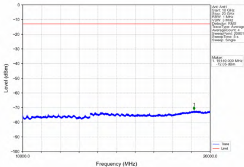
Band66_5MHz_16QAM_HCH_1777.5MHz_RB_1_0_NTNV
