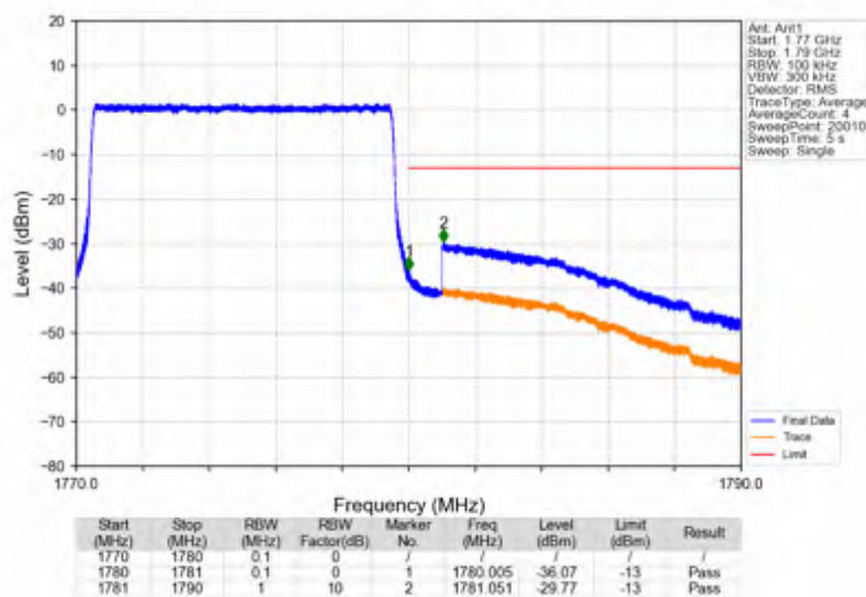
Band66_10MHz_256QAM_HCH_1775MHz_RB_50_0_NTNV
