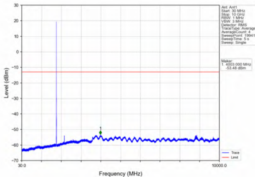
Band66_5MHz_256QAM_HCH_1777.5MHz_RB_1_0_NTNV
