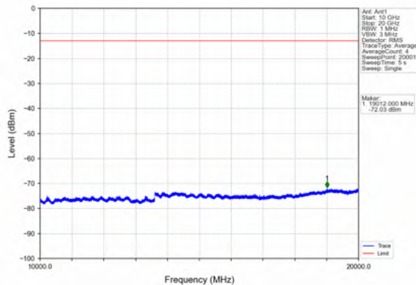
Band66_15MHz_256QAM_LCH_1717.5MHz_RB_75_0_NTNV
