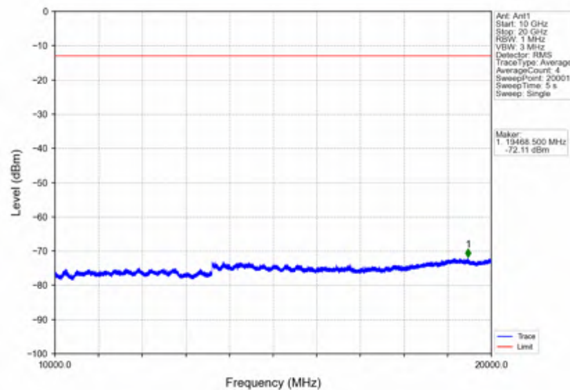
Band66_1.4MHz_256QAM_LCH_1710.7MHz_RB_6_0_NTNV
