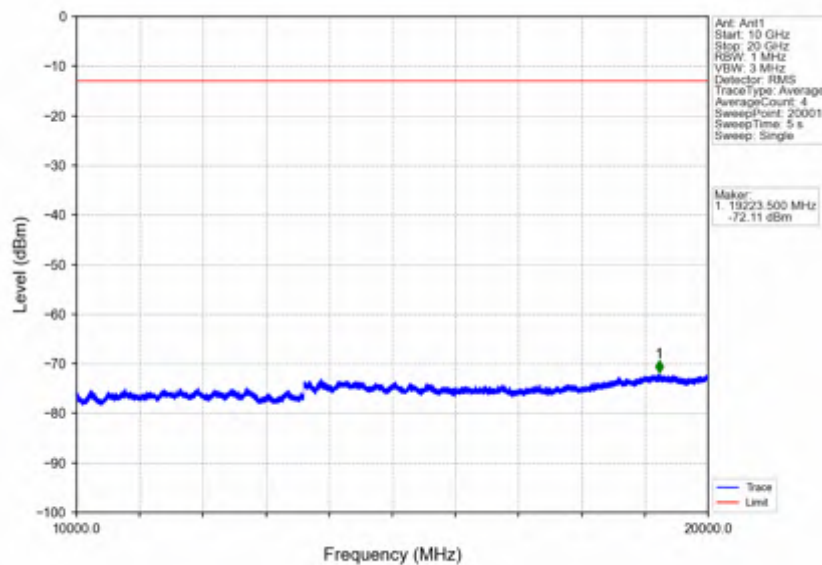
Band66_20MHz_16QAM_HCH_1770MHz_RB_1_0_NTNV
