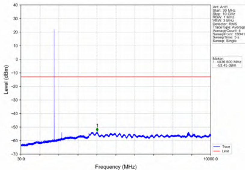
Band66_3MHz_16QAM_HCH_1778.5MHz_RB_1_0_NTNV
