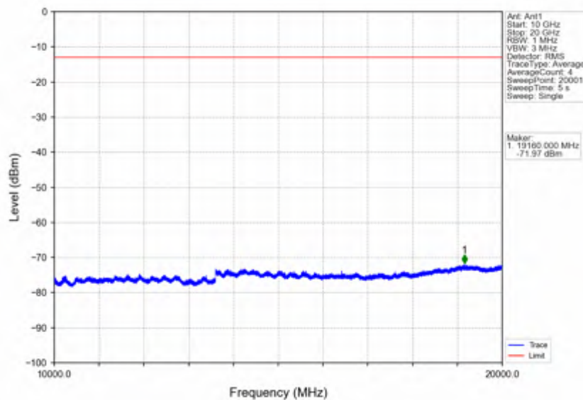
Band66_3MHz_16QAM_HCH_1778.5MHz_RB_1_0_NTNV
