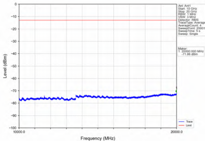
Band66_3MHz_QPSK_HCH_1778.5MHz_RB_1_0_NTNV
