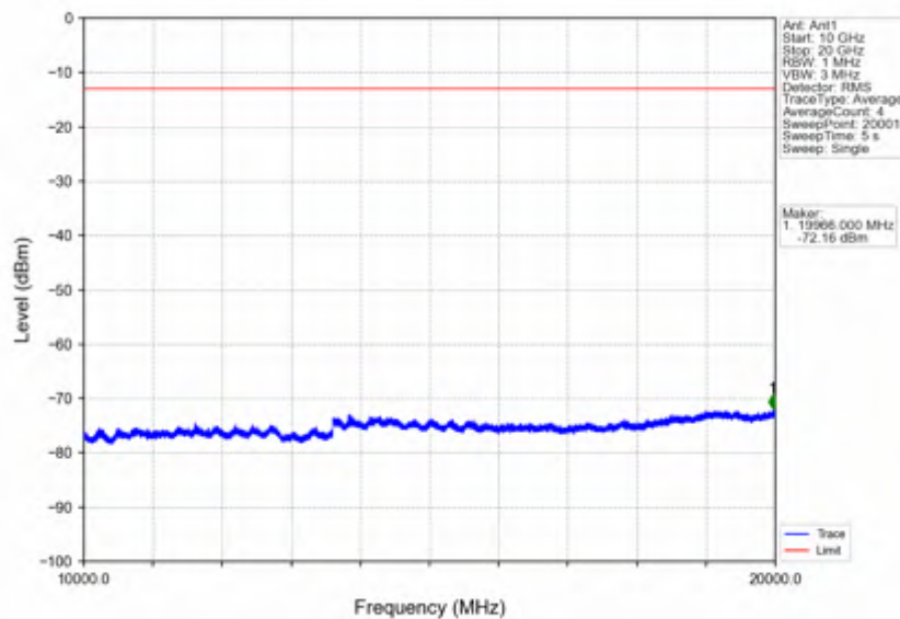
Band66_15MHz_256QAM_HCH_1772.5MHz_RB_1_0_NTNV
