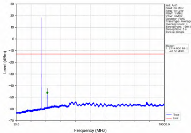
Band66_5MHz_256QAM_LCH_1712.5MHz_RB_1_0_NTNV
