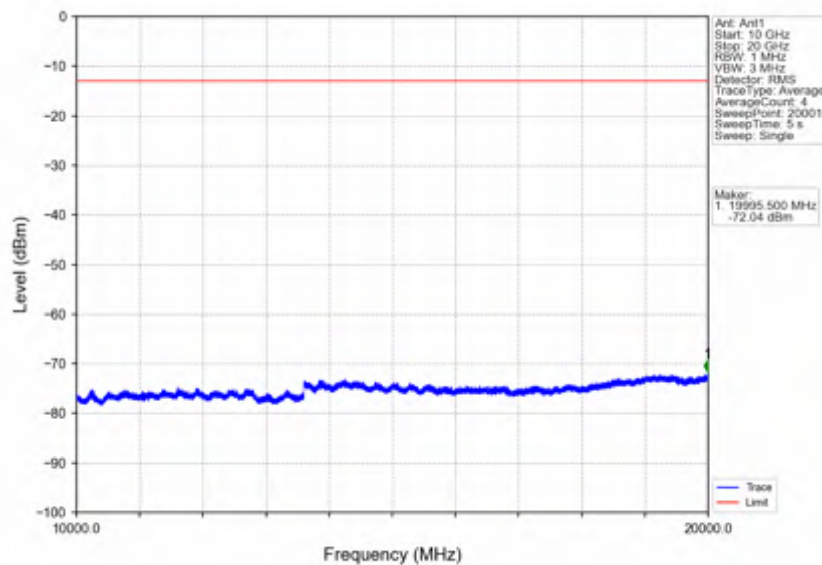
Band66_1.4MHz_256QAM_MCH_1745MHz_RB_1_0_NTNV
