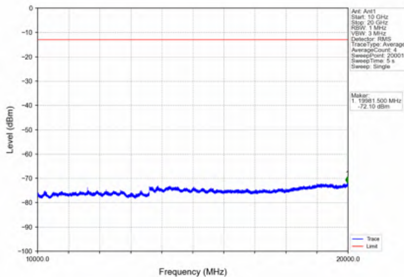
Band66_3MHz_64QAM_MCH_1745MHz_RB_1_0_NTNV
