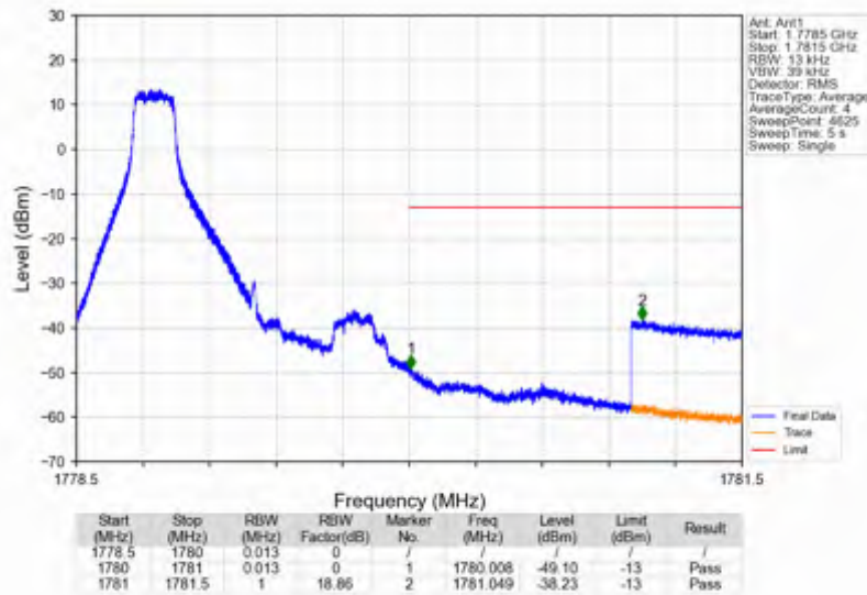
Band66_1.4MHz_16QAM_HCH_1779.3MHz_RB_1_5_NTNV
