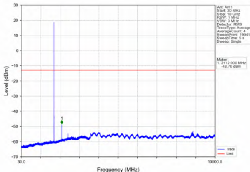
Band66 3MHz 256QAM LCH 1711.5MHz RB 1 0 NTNV
