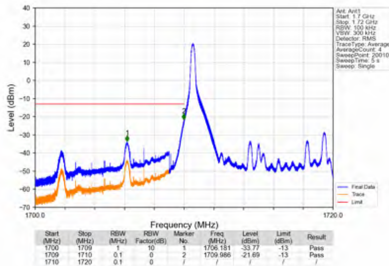
Band66 10MHz 16QAM LCH 1715MHz RB 50 0 NTNV
