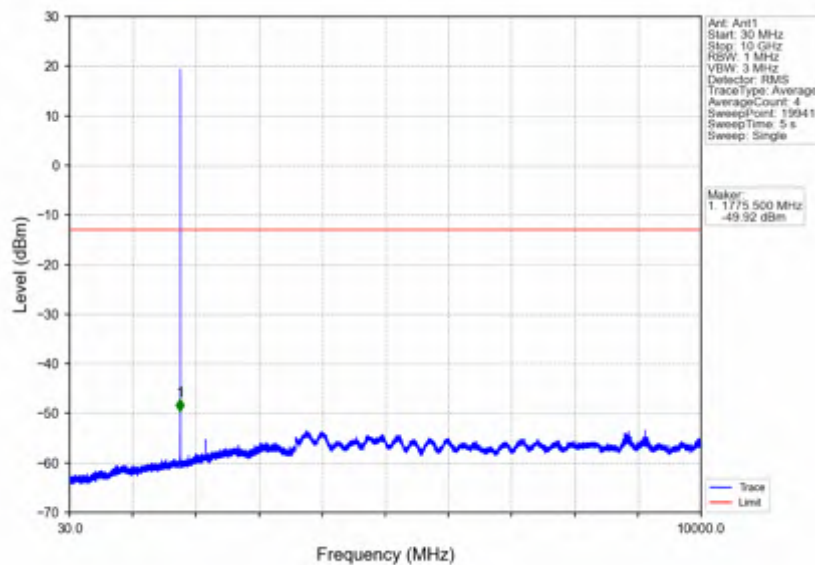
Band66 1.4MHz 256QAM HCH 1779.3MHz RB 1 0 NTNV
