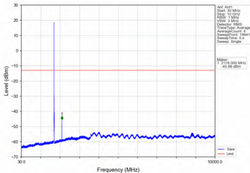
Band66 10MHz 256QAM LCH 1715MHz RB 1 0 NTV
