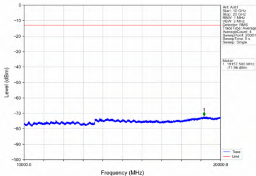
Band66_15MHz_64QAM_LCH_1717.5MHz_RB_75_0_NTNV
