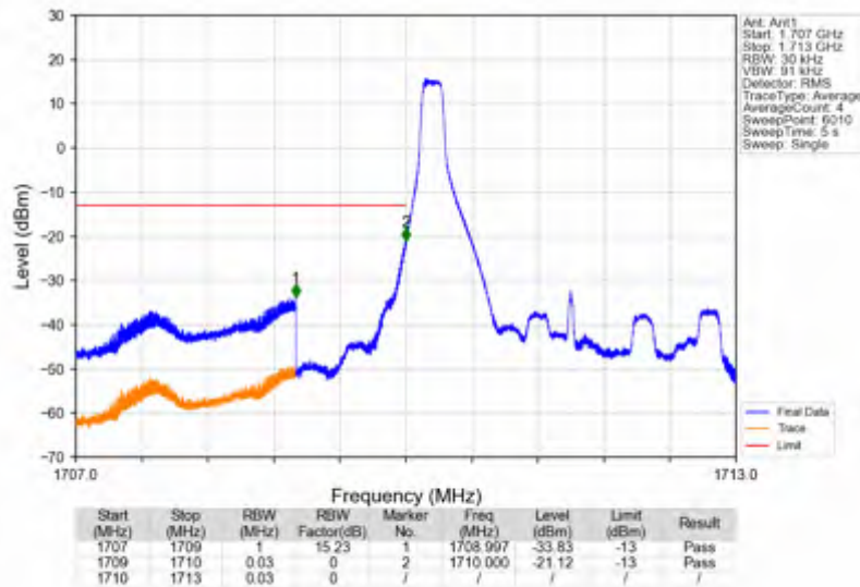
Band66_3MHz_QPSK_LCH_1711.5MHz_RB_15_0_NTNV
