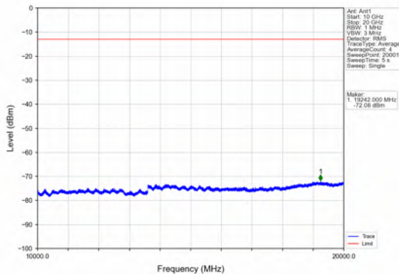
Band66_5MHz_QPSK_LCH_1712.5MHz_RB_25_0_NTNV
