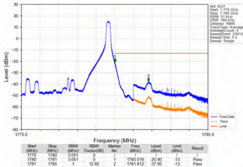
Band66_5MHz_256QAM_HCH_1777.5MHz_RB_1_24_NTNV
