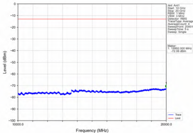
Band66_10MHz_64QAM_MCH_1745MHz_RB_1_0_NTNV
