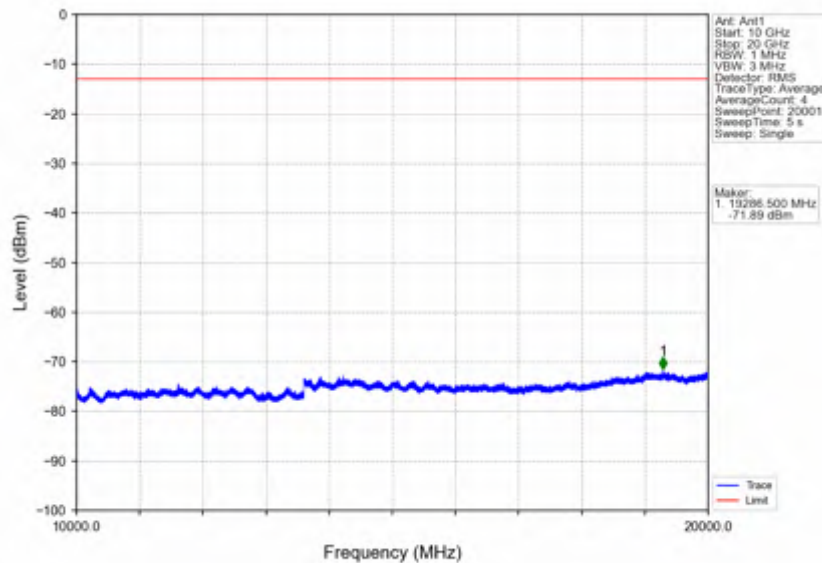
Band66_5MHz_16QAM_MCH_1745MHz_RB_1_0_NTNV
