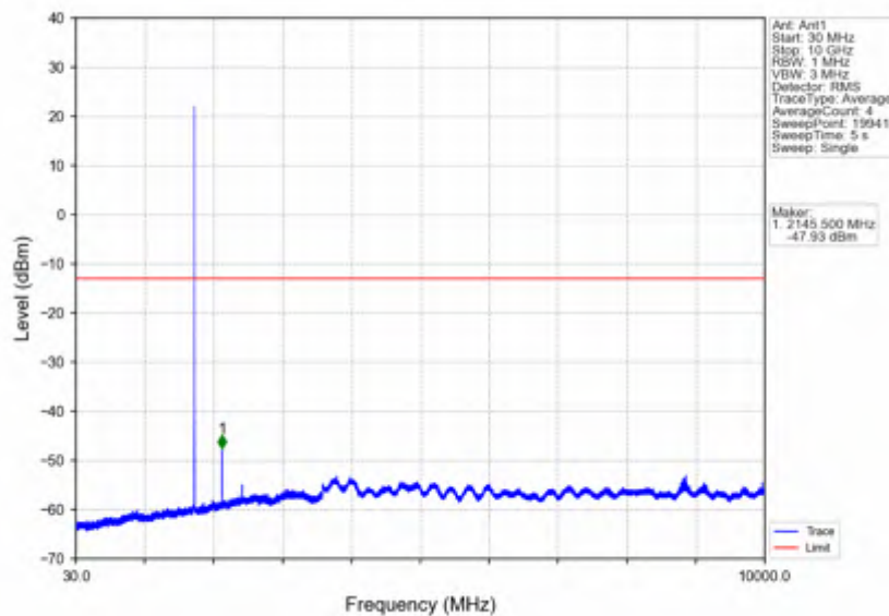
Band66_3MHz_64QAM_MCH_1745MHz_RB_1_0_NTNV
