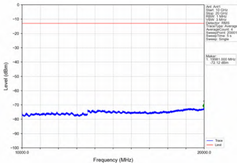
Band66_10MHz_256QAM_MCH_1745MHz_RB_1_0_NTNV
