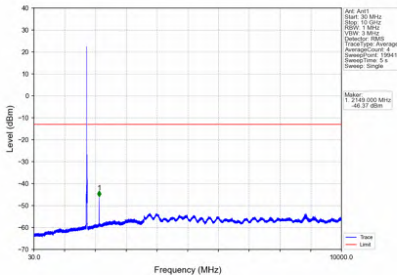
Band66_10MHz_64QAM_MCH_1745MHz_RB_1_0_NTNV
