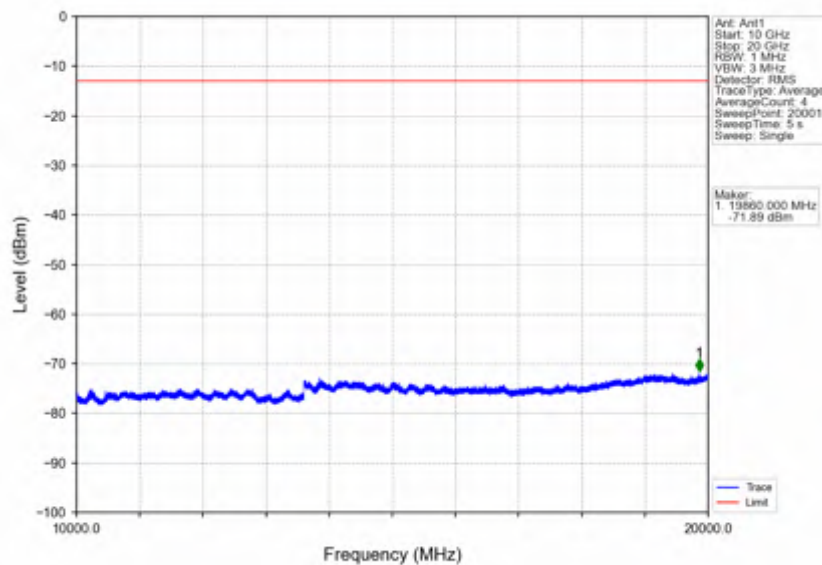
Band66_15MHz_QPSK_HCH_1772.5MHz_RB_1_0_NTNV
