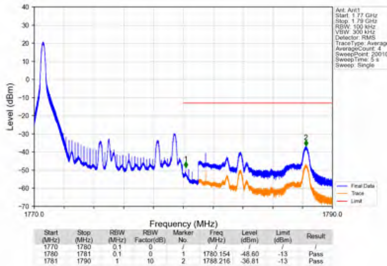
Band66_10MHz_16QAM_HCH_1775MHz_RB_1_49_NTNV
