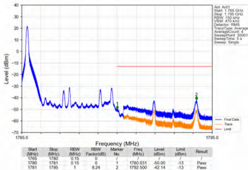
Band66_15MHz_64QAM_HCH_1772.5MHz_RB_75_0_NTNV
