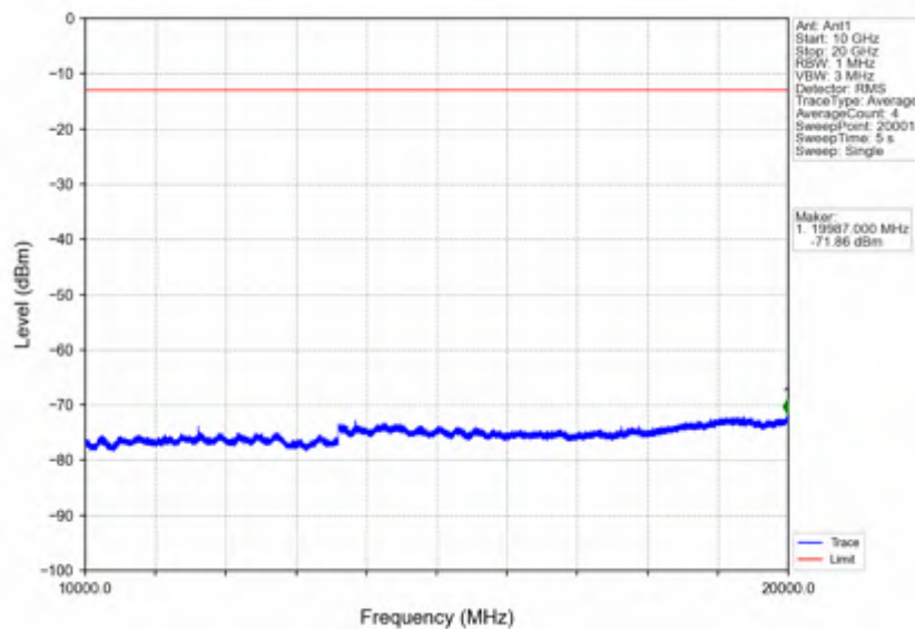
Band66_3MHz_64QAM_HCH_1778.5MHz_RB_1_0_NTNV
