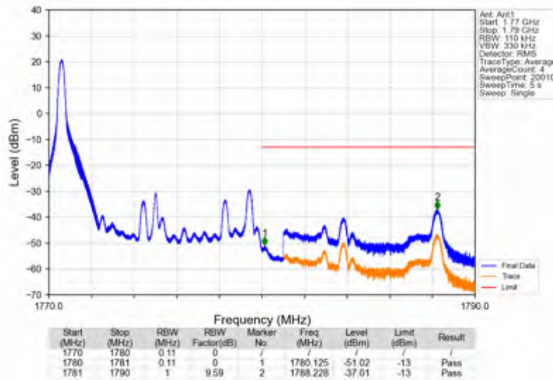
Band66_10MHz_64QAM_HCH_1775MHz_RB_1_49_NTNV
