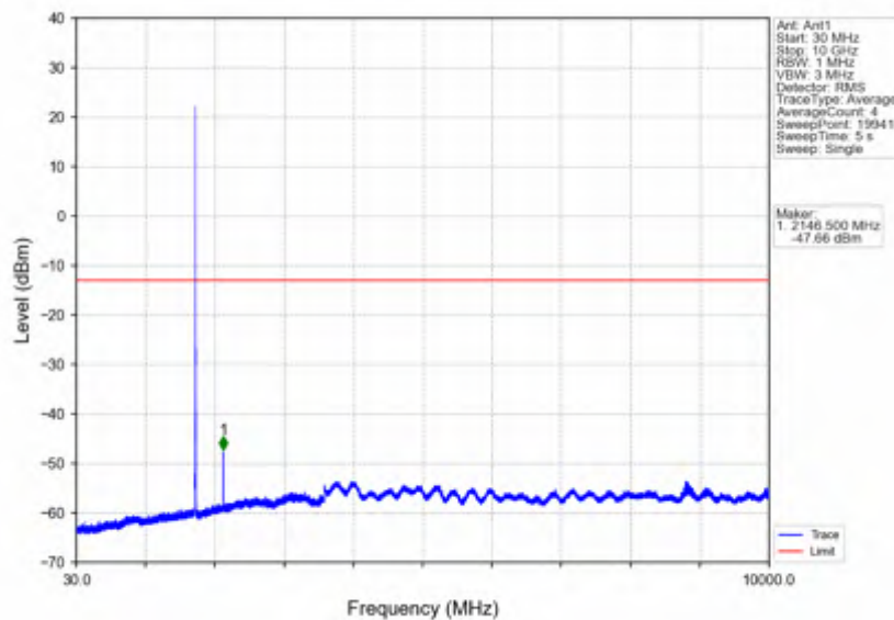
Band66_5MHz_64QAM_MCH_1745MHz_RB_1_0_NTNV
