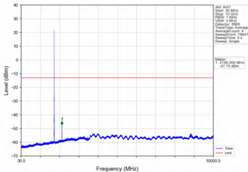
Band66_5MHz_16QAM_MCH_1745MHz_RB_1_0_NTNV
