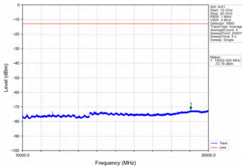
Band66_1.4MHz_64QAM_MCH_1745MHz_RB_1_0_NTNV
