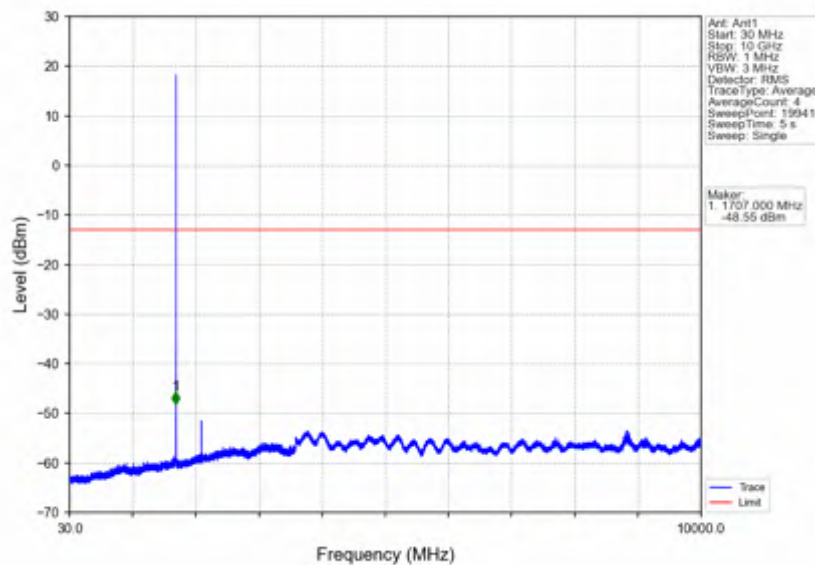
Band66_1.4MHz_256QAM_LCH_1710.7MHz_RB_1_0_NTNV
