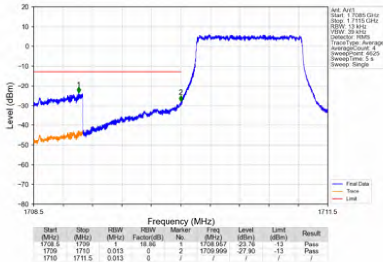
Band66_1.4MHz_64QAM_LCH_1710.7MHz_RB_6_0_NTNV
