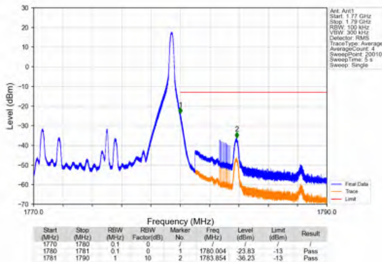
Band66_10MHz_256QAM_HCH_1775MHz_RB_1_49_NTNV
