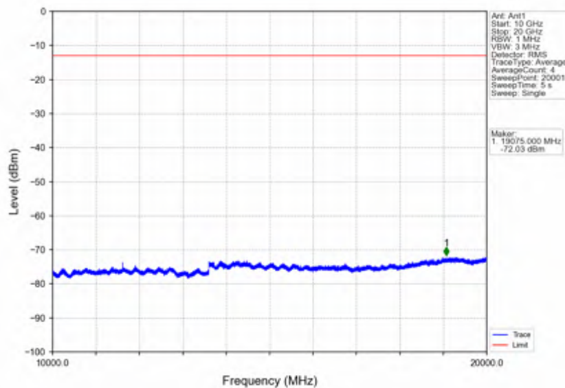
Band66_20MHz_256QAM_MCH_1745MHz_RB_1_0_NTNV
