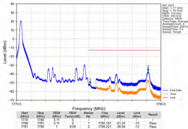
Band66_10MHz_QPSK_HCH_1775MHz_RB_50_0_NTV
