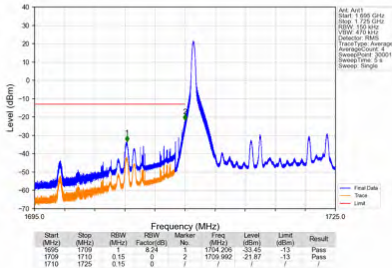
Band66_15MHz_64QAM_LCH_1717.5MHz_RB_75_0_NTNV
