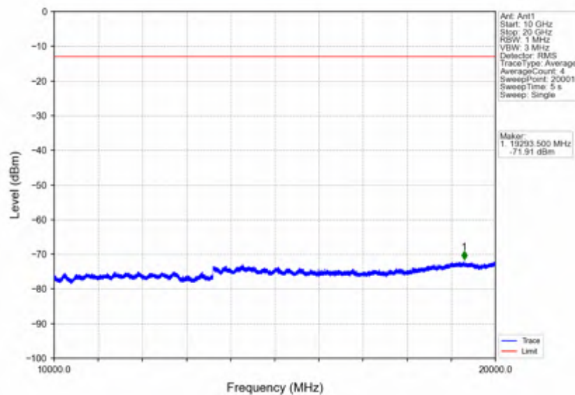
Band66_3MHz_256QAM_LCH_1711.5MHz_RB_15_0_NTNV
