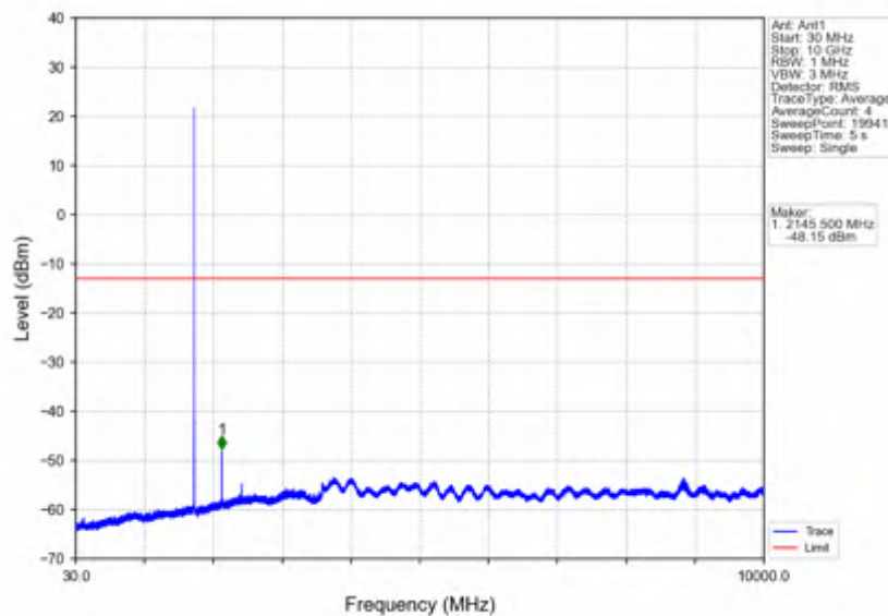
Band66_3MHz_QPSK_MCH_1745MHz_RB_1_0_NTNV
