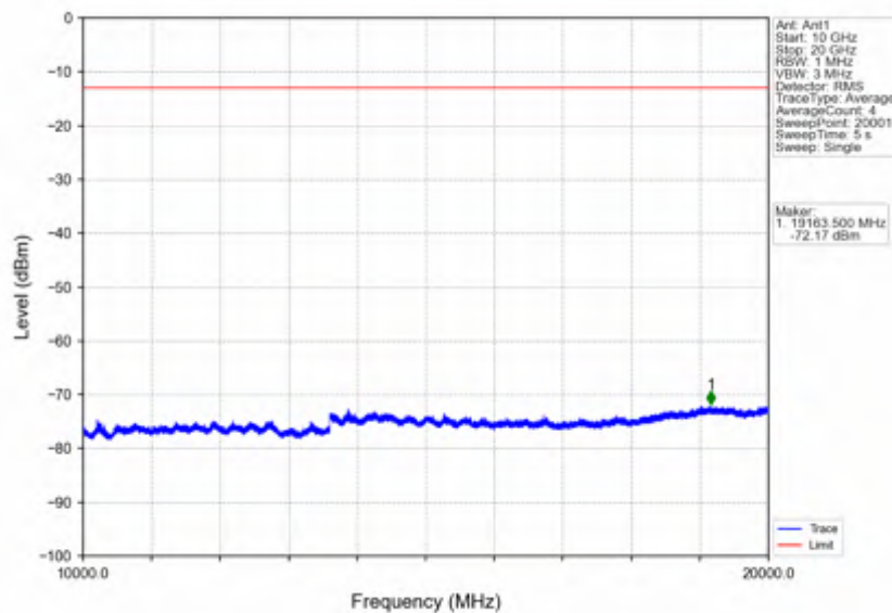
Band66_5MHz_QPSK_HCH_1777.5MHz_RB_1_0_NTNV
