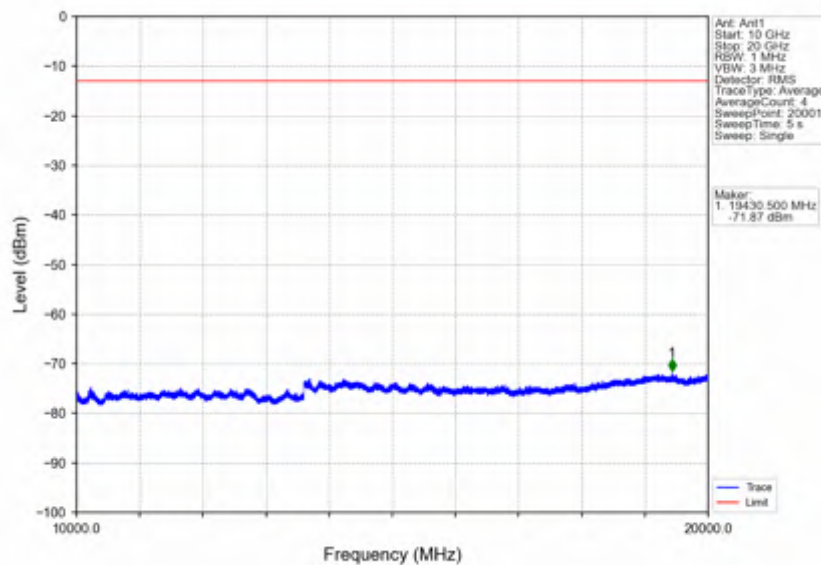
Band66_5MHz_QPSK_MCH_1745MHz_RB_1_0_NTNV
