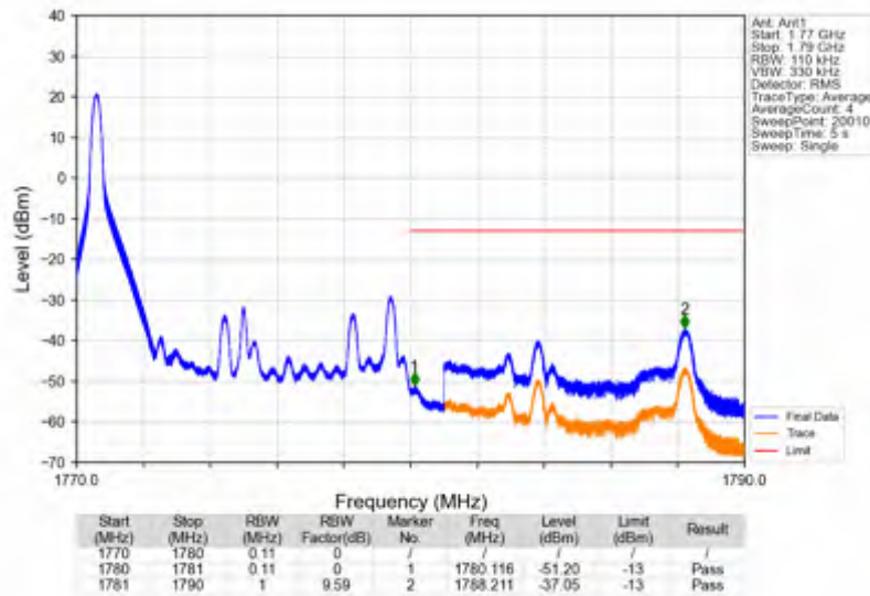
Band66_10MHz_QPSK_HCH_1775MHz_RB_1_49_NTV
