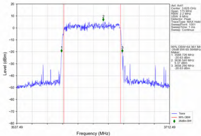
n78d_30kHz_SISO_NTNV_70MHz_DFT-s-OFDM_256_QAM_3624.99MHz_Outer_Full
