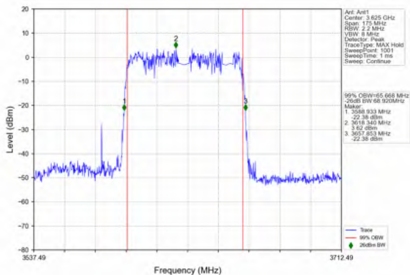
n78d_30kHz_SISO_NTNV_70MHz_DFT-s-OFDM_PI/2_BPSK_3624.99MHz_Outer_Full
