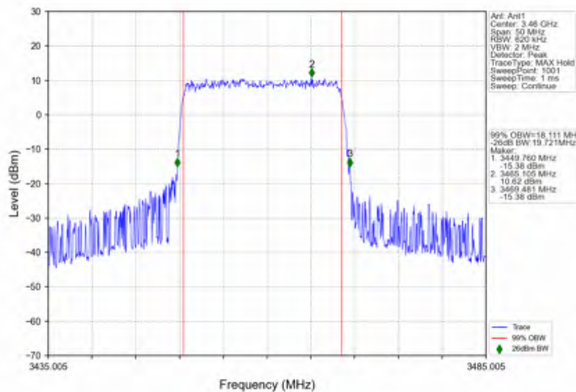
n78e_15kHz_SISO_NTNV_20MHz_DFT-s-OFDM QPSK_3460.005MHz_Outer_Full
