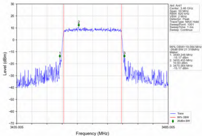
n78e_15kHz_SISO_NTNV_20MHz_CP-OFDM_64_QAM_3460.005MHz_Outer_Full
