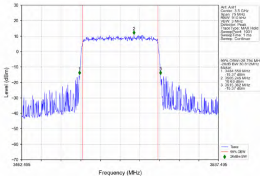
n78e_15kHz_SISO_NTNV_30MHz_DFT-s-OFDM_16_QAM_3499.995MHz_Outer_Full
