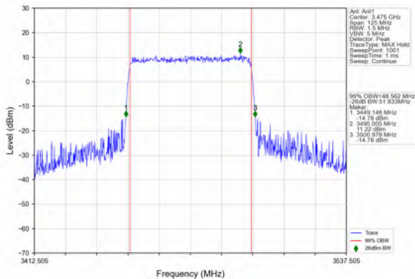
n78e_15kHz_SISO_NTNV_50MHz_CP-OFDM_QPSK_3475.005MHz_Outer_Full
