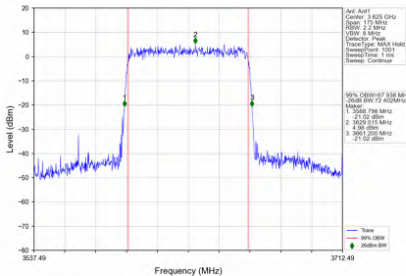
n78d_30kHz_SISO_NTNV_70MHz_CP-OFDM_256_QAM_3624.99MHz_Outer_Full
