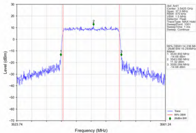
n78e_15kHz_SISO_NTNV_15MHz_CP-OFDM QPSK_3542.49MHz_Outer_Full
