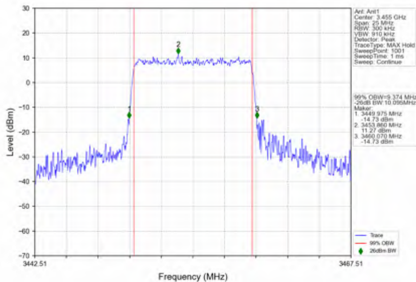
n78e_15kHz_SISO_NTNV_10MHz_CP-OFDM QPSK_3455.01MHz_Outer_Full
