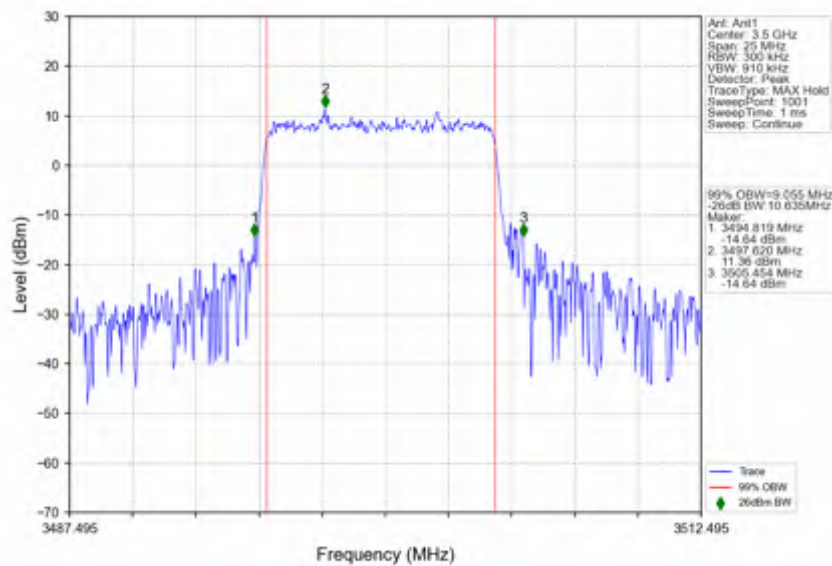
n78e_15kHz_SISO_NTNV_10MHz_DFT-s-OFDM PI/2 BPSK_3499.995MHz_Outer_Full
