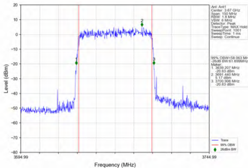
n78d_30kHz_SISO_NTNV_60MHz_CP-OFDM 64 QAM_3669.99MHz_Outer_Full
