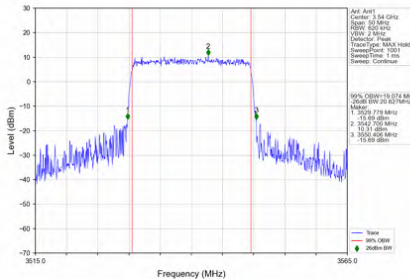
n78e_15kHz_SISO_NTNV_20MHz_CP-OFDM 64 QAM_3540MHz_Outer_Full
