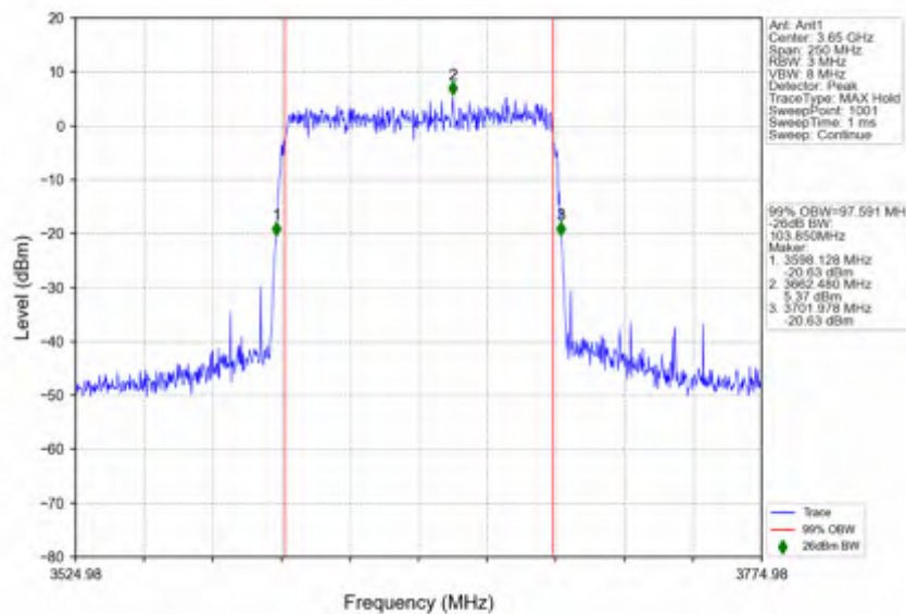
n78d_30kHz_SISO_NTNV_100MHz_CP-OFDM QPSK_3649.98MHz_Outer_Full
