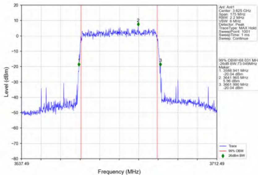
n78d_30kHz_SISO_NTNV_70MHz_CP-OFDM 16 QAM_3624.99MHz_Outer_Full
