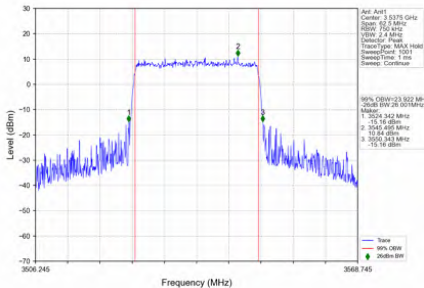
n78e_15kHz_SISO_NTNV_25MHz_CP-OFDM_64_QAM_3537.495MHz_Outer_Full
