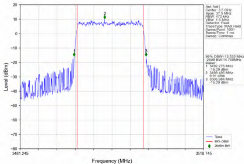
n78e_15kHz_SISO_NTNV_15MHz_DFT-s-OFDM_256_QAM_3499.995MHz_Outer_Full
