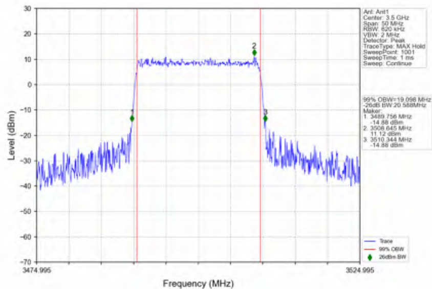
n78e_15kHz_SISO_NTNV_20MHz_CP-OFDM_16_QAM_3499.995MHz_Outer_Full
