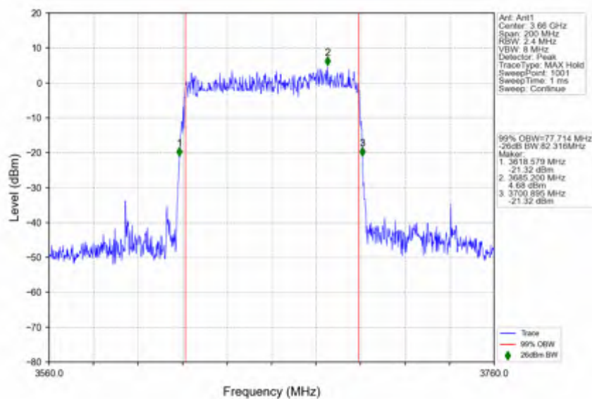
n78d 30kHz SISO NTNv 80MHz DFT-s-OFDM QPSK 3660MHz Outer Full
