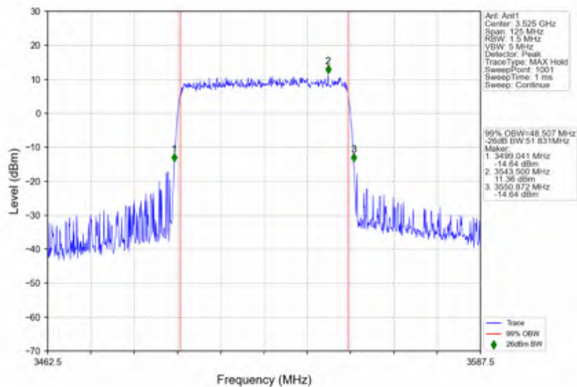
n78e_15kHz_SISO_NTNV_50MHz_DFT-s-OFDM 64 QAM_3525MHz_Outer_Full
