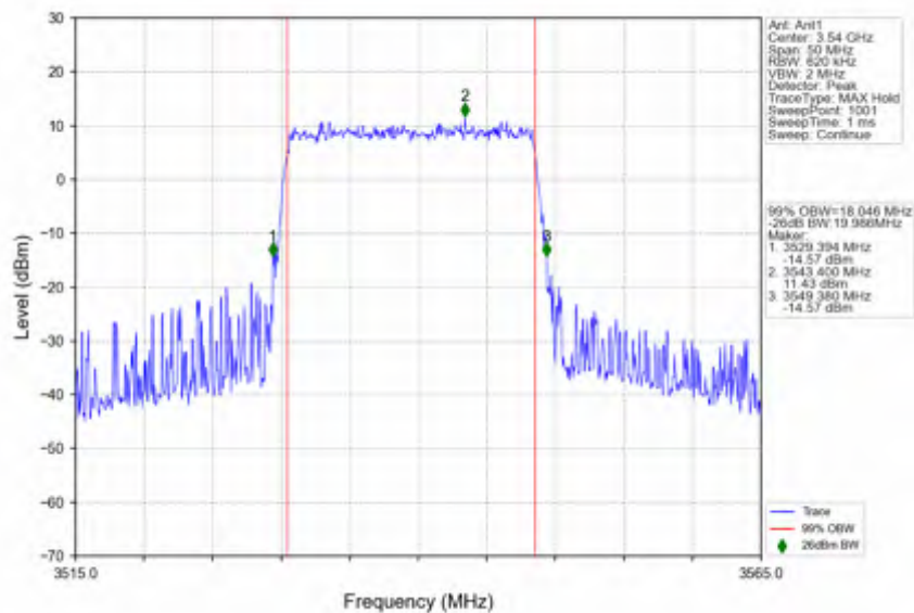
n78e_15kHz_SISO_NTNV_20MHz_DFT-s-OFDM_64_QAM_3540MHz_Outer_Full
