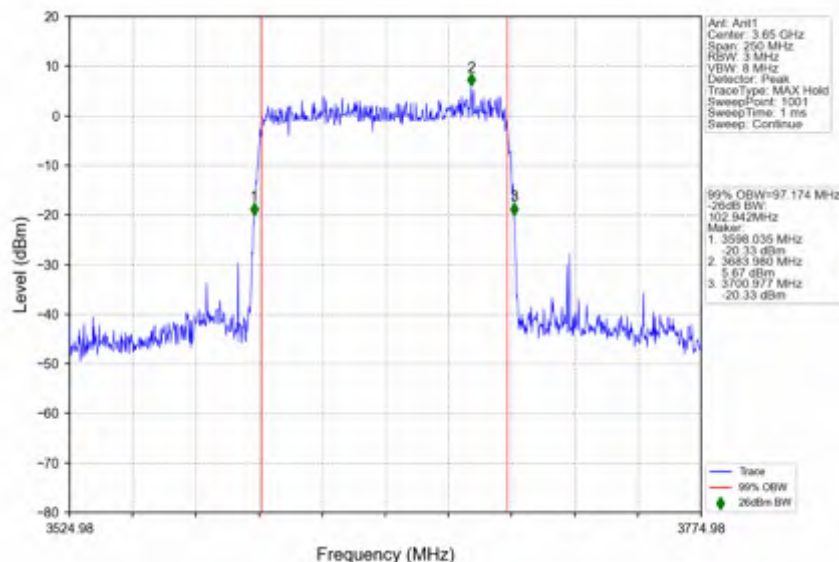
n78d_30kHz_SISO_NTNV_100MHz_DFT-s-OFDM QPSK_3649.98MHz_Outer_Full
