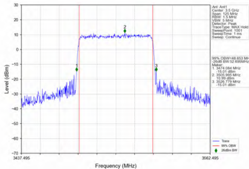
n78e_15kHz_SISO_NTNV_50MHz_CP-OFDM_16_QAM_3499.995MHz_Outer_Full
