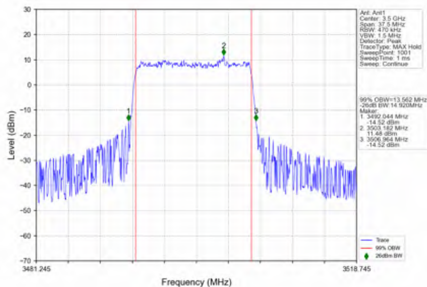
n78e_15kHz_SISO_NTNV_15MHz_DFT-s-OFDM_PI/2_BPSK_3499.995MHz_Outer_Full
