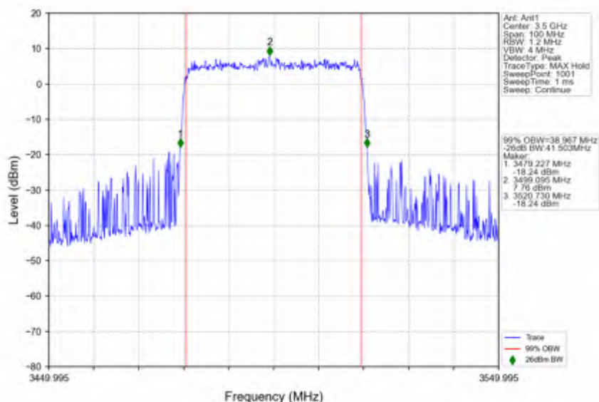
n78e 15kHz SISO NTNV 40MHz CP-OFDM 256 QAM 3499.995MHz Outer Full
