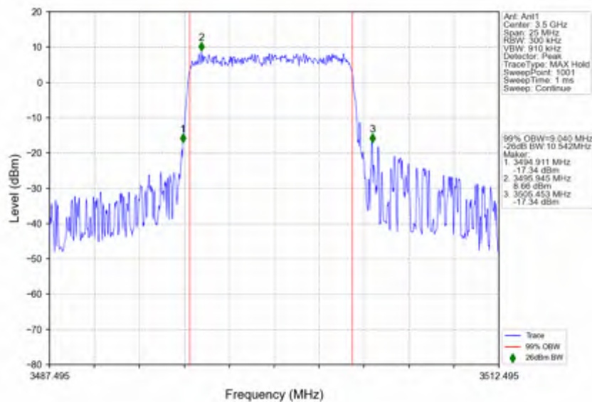
n78e_15kHz_SISO_NTNV_10MHz_DFT-s-OFDM_256_QAM_3499.995MHz_Outer_Full
