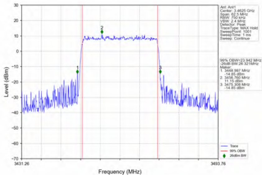
n78e_15kHz_SISO_NTNV_25MHz_CP-OFDM_64_QAM_3462.51MHz_Outer_Full
