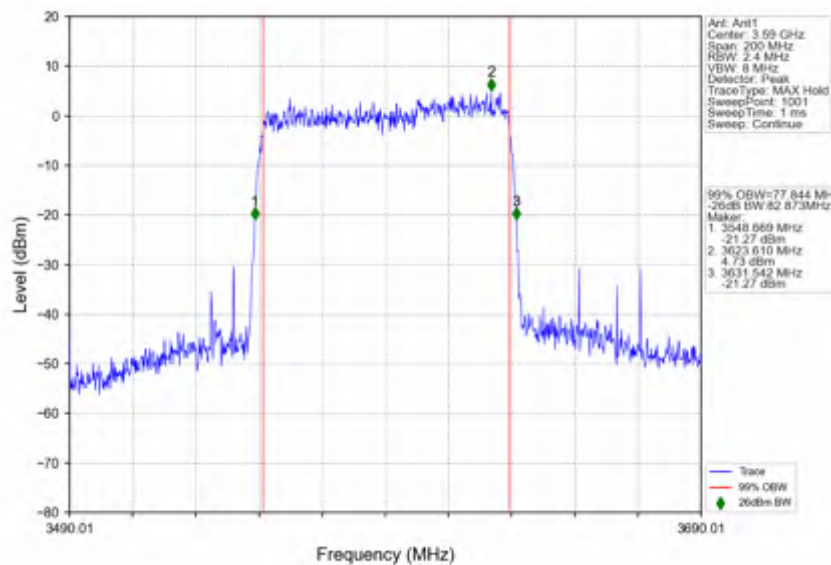
n78d_30kHz_SISO_NTNV_80MHz_CP-OFDM 64 QAM_3590.01MHz_Outer_Full
