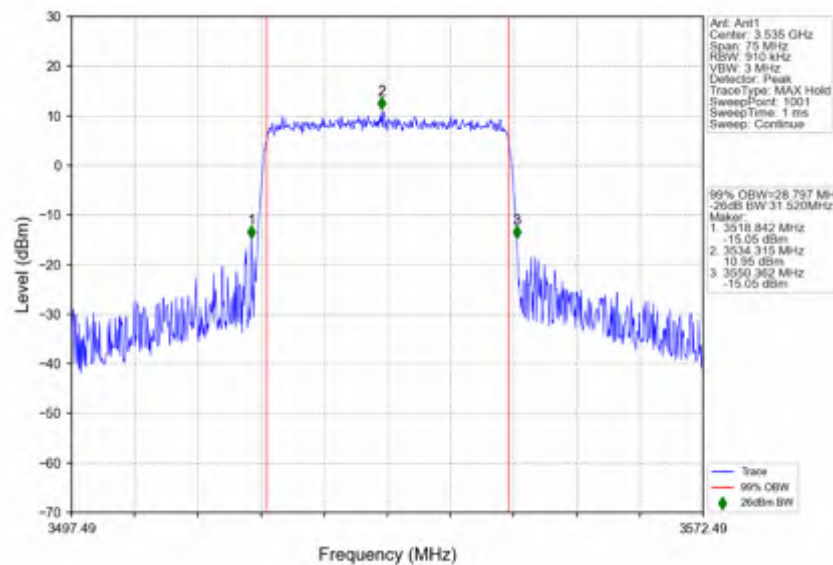
n78e_15kHz_SISO_NTNV_30MHz_CP-OFDM 64 QAM_3534.99MHz_Outer_Full
