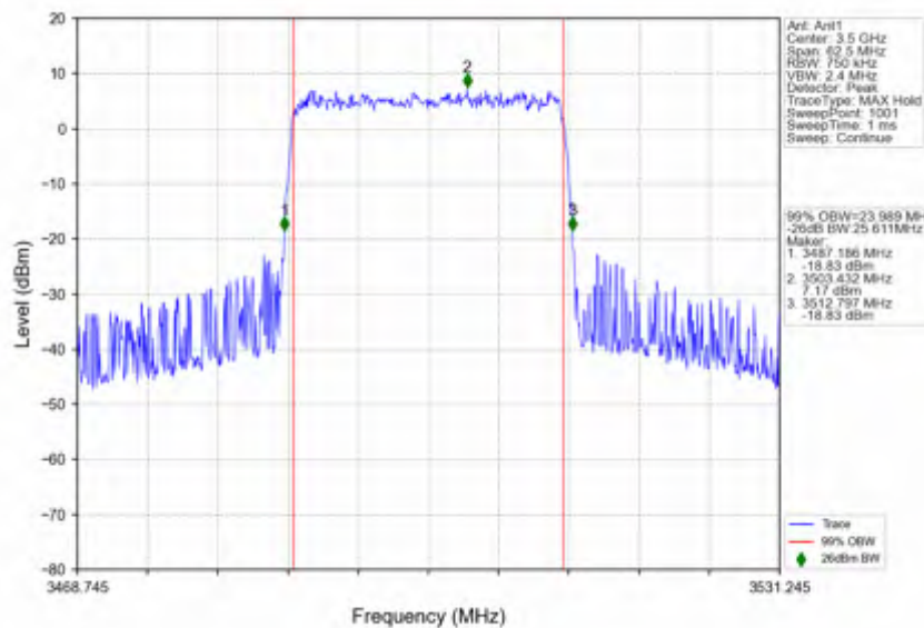
n78e_15kHz_SISO_NTNV_25MHz_CP-OFDM_256_QAM_3499.995MHz_Outer_Full
