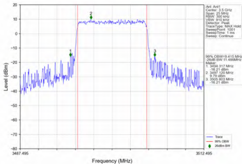
n78e_15kHz_SISO_NTNV_10MHz_CP-OFDM_16_QAM_3499.995MHz_Outer_Full
