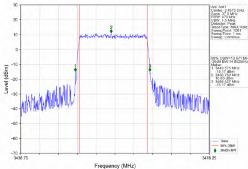
n78e_15kHz_SISO_NTNV_15MHz_DFT-s-OFDM QPSK_3457.5MHz_Outer_Full
