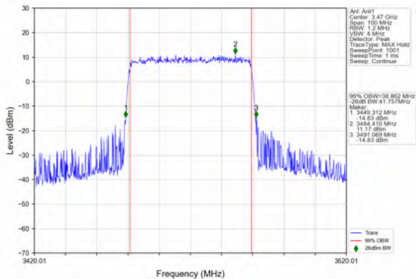
n78e_15kHz_SISO_NTNV_40MHz_DFT-s-OFDM 64 QAM_3470.01MHz_Outer_Full
