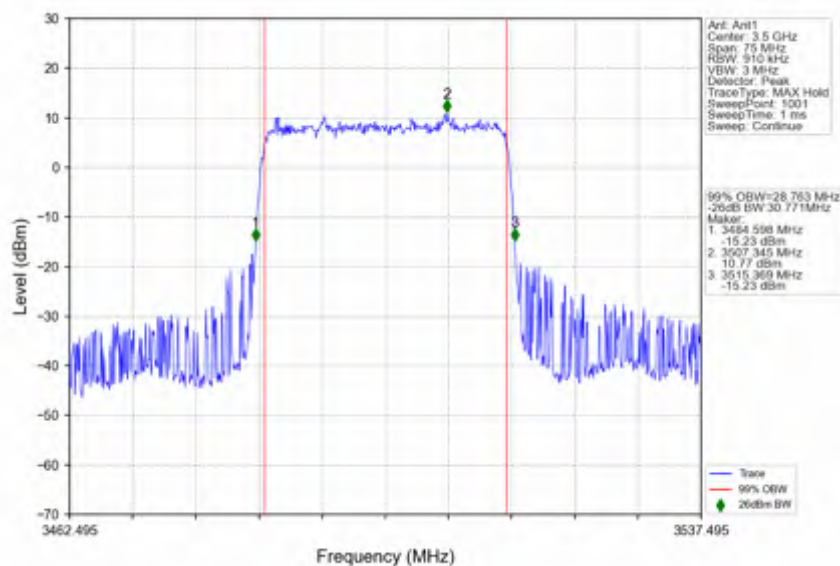
n78e_15kHz_SISO_NTNV_30MHz_DFT-s-OFDM_PI/2_BPSK_3499.995MHz_Outer_Full
