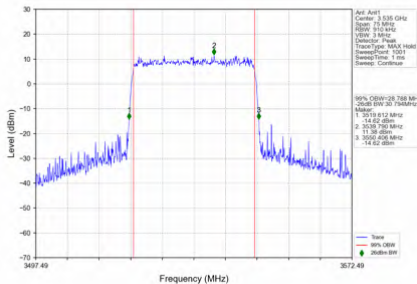
n78e_15kHz_SISO_NTNV_30MHz_CP-OFDM QPSK_3534.99MHz_Outer_Full
