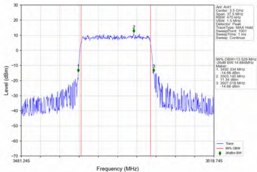
n78e_15kHz_SISO_NTNV_15MHz_DFT-s-OFDM_16_QAM_3499.995MHz_Outer_Full
