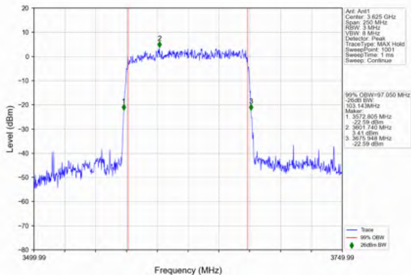
n78d_30kHz_SISO_NTNV_100MHz_DFT-s-OFDM_PI/2_BPSK_3624.99MHz_Outer_Full
