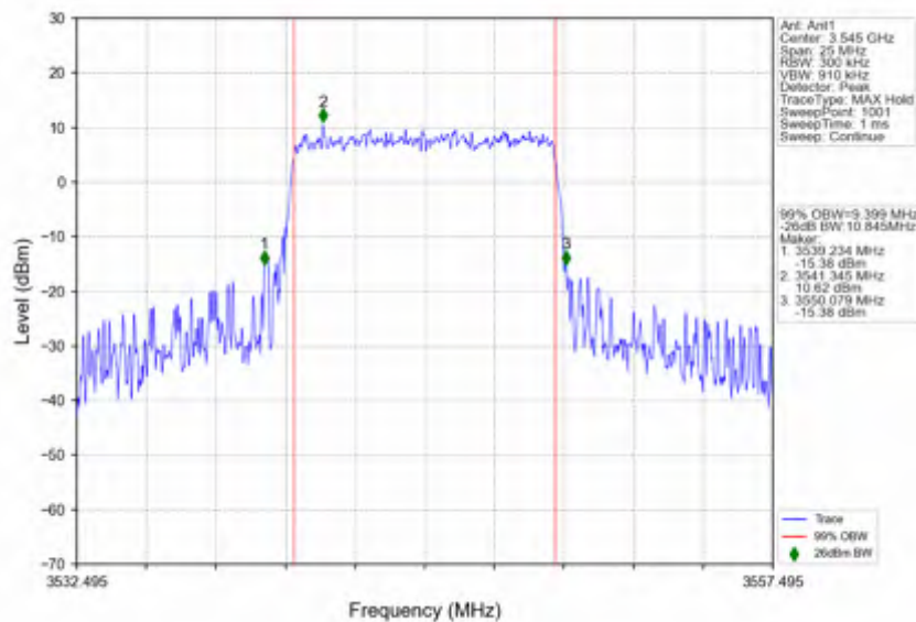
n78e_15kHz_SISO_NTNV_10MHz_CP-OFDM 64 QAM_3544.995MHz_Outer_Full
