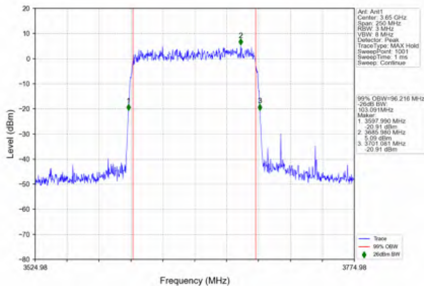
n78d_30kHz_SISO_NTNV_100MHz_DFT-s-OFDM 64 QAM_3649.98MHz_Outer_Full
