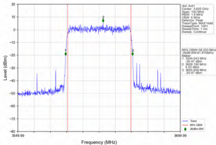
n78d_30kHz_SISO_NTNV_60MHz_CP-OFDM_256_QAM_3624.99MHz_Outer_Full
