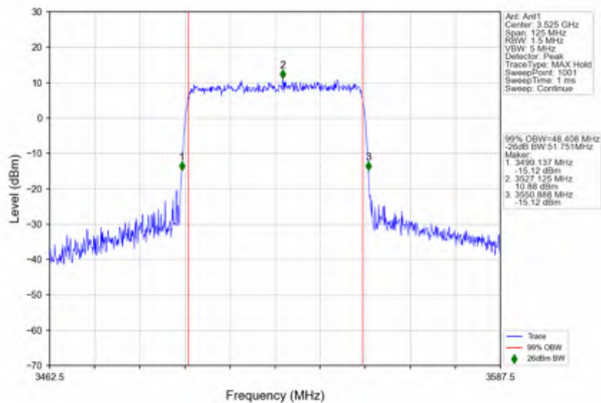
n78e_15kHz_SISO_NTNV_50MHz_CP-OFDM 64 QAM_3525MHz_Outer_Full
