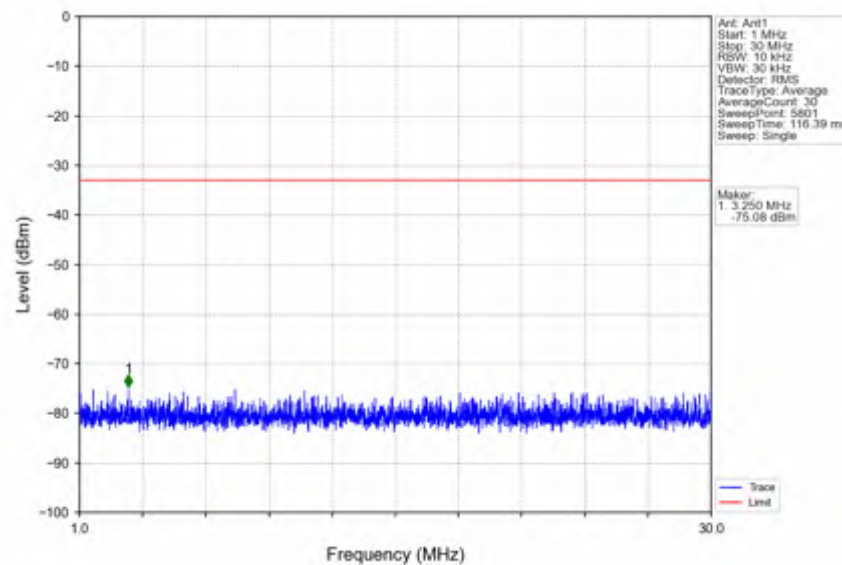
n66_15kHz_SISO_NTNV_25MHz_CP-OFDM QPSK_1767.5MHz_Edge_1RB_Right
