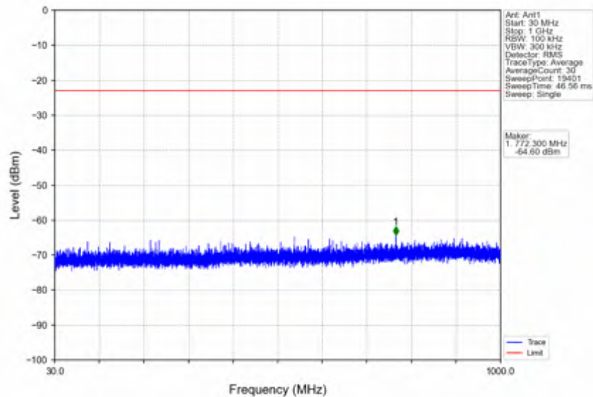
n66_15kHz_SISO_NTNV_30MHz_DFT-s-OFDM QPSK_1765MHz_Inner_1RB_Right
