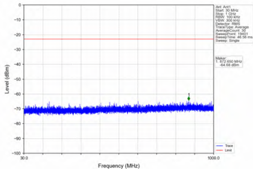
n66_15kHz_SISO_NTNV_15MHz_CP-OFDM QPSK_1772.5MHz_Outer_Full
