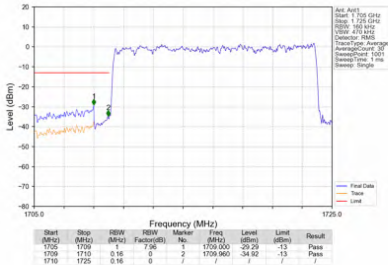
n66_15kHz_SISO_NTNV_15MHz_DFT-s-OFDM_QPSK_1717.5MHz_Outer_Full
