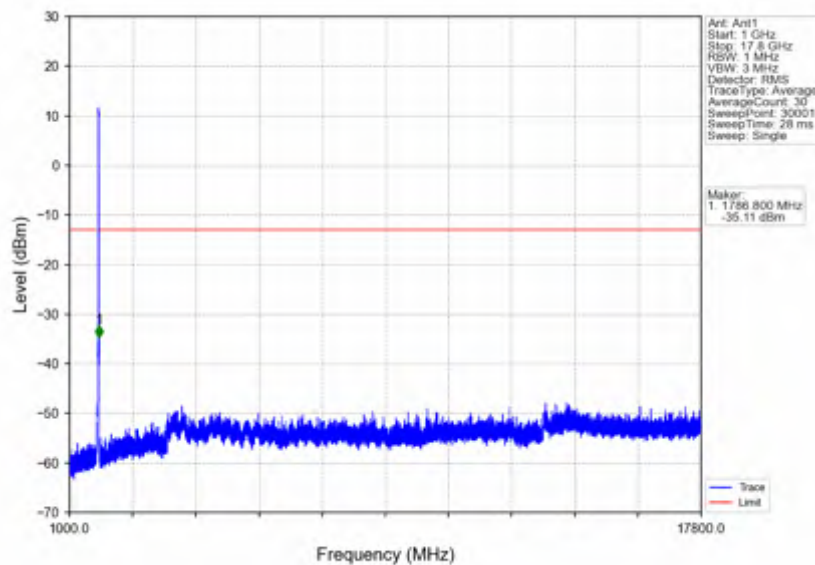
n66_15kHz_SISO_NTNV_20MHz_DFT-s-OFDM_PI/2_BPSK_1770MHz_Outer_Full
