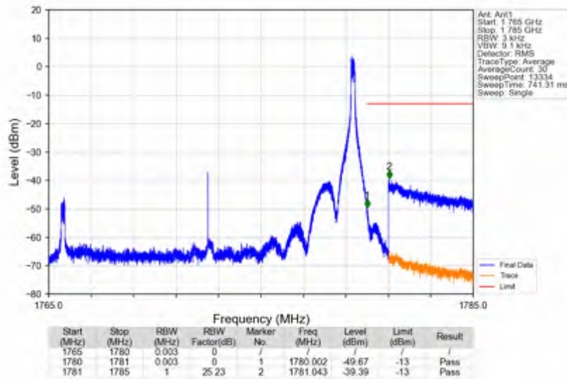
n66_15kHz_SISO_NTNV_15MHz_CP-OFDM_QPSK_1772.5MHz_Inner_1RB_Right
