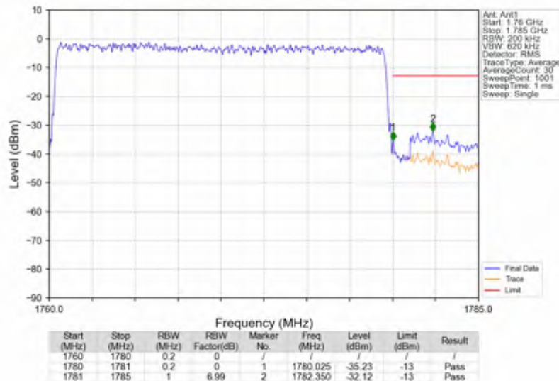
n66_15kHz_SISO_NTNV_20MHz_CP-OFDM QPSK_1770MHz_Outer_Full
