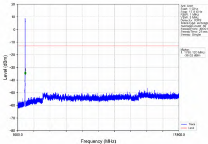
n66_15kHz_SISO_NTNV_30MHz_DFT-s-OFDM QPSK_1765MHz_Inner_1RB_Right
