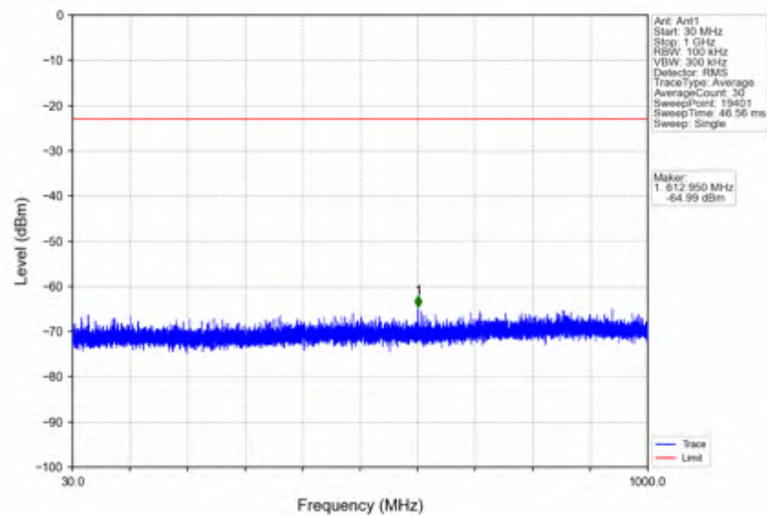
n66_15kHz_SISO_NTV_30MHz_CP-OFDM_QPSK_1725MHz_Outer_Full
