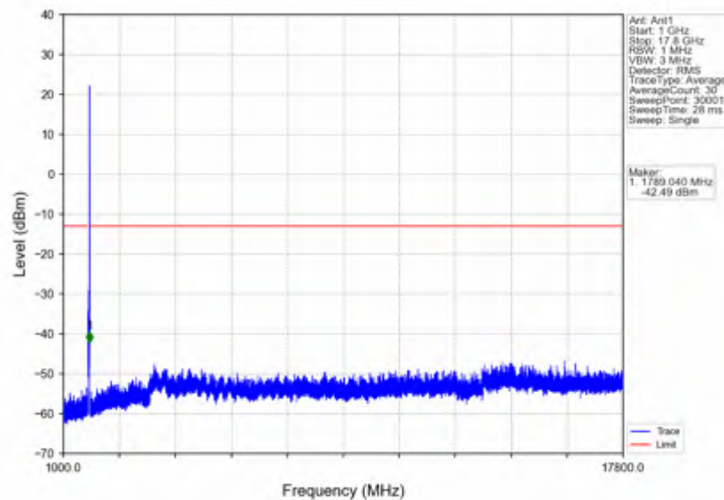
n66_15kHz_SISO_NTNV_20MHz_DFT-s-OFDM_QPSK_1770MHz_Edge_1RB_Right
