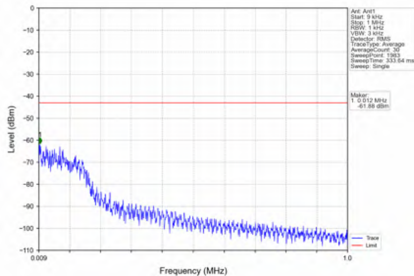
n66_15kHz_SISO_NTNV_20MHz_CP-OFDM_QPSK_1745MHz_Edge_1RB_Left
