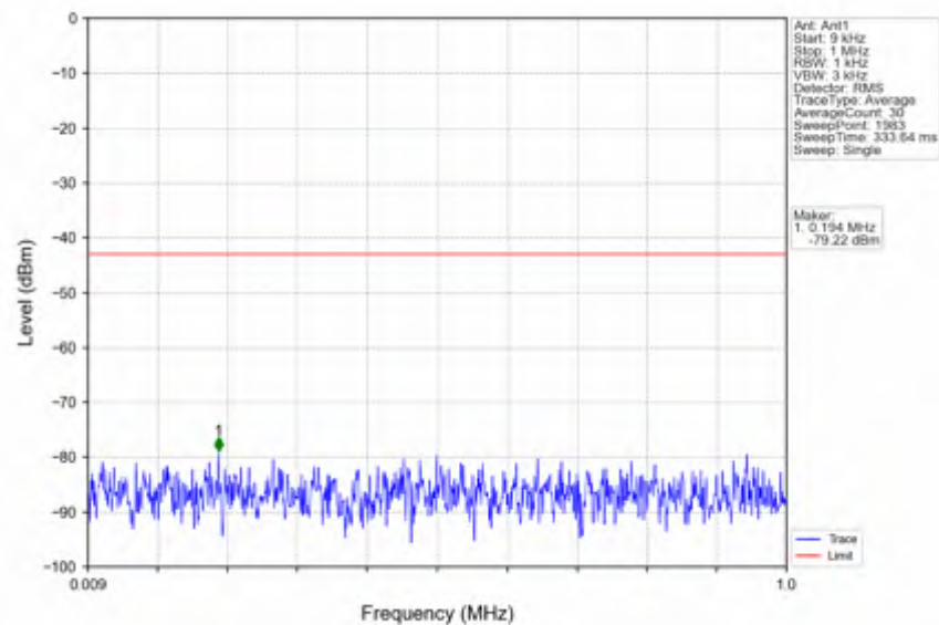
n66_15kHz_SISO_NTNV_20MHz_CP-OFDM_QPSK_1720MHz_Outer_Full
