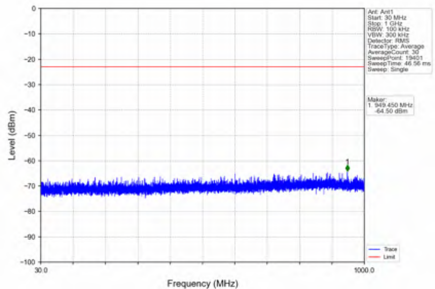
n66_15kHz_SISO_NTNV_25MHz_DFT-s-OFDM_QPSK_1722.5MHz_Outer_Full
