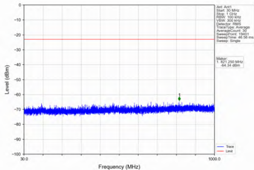
n66_15kHz_SISO_NTNV_15MHz_DFT-s-OFDM_QPSK_1772.5MHz_Outer_Full
