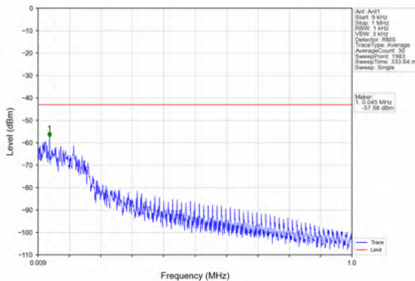
n66_15kHz_SISO_NTNV_15MHz_CP-OFDM_QPSK_1772.5MHz_Inner_1RB_Right
