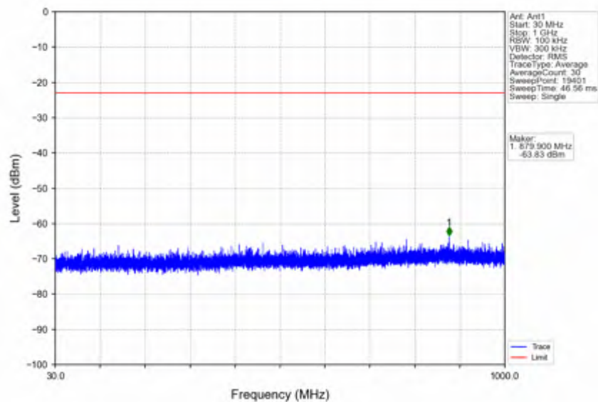
n66_15kHz_SISO_NTNV_20MHz_CP-OFDM_QPSK_1770MHz_Outer_Full
