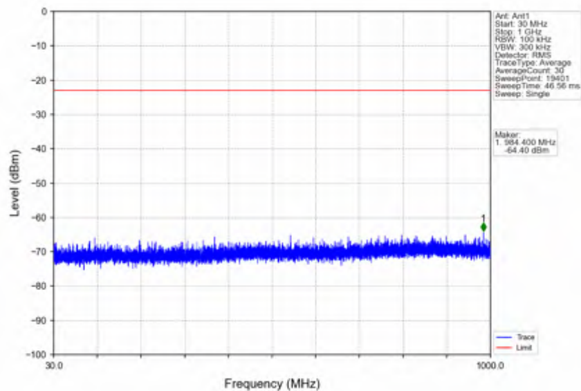
n66_15kHz_SISO_NTNV_20MHz_DFT-s-OFDM_PI/2_BPSK_1770MHz_Outer_Full
