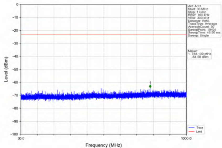
n66_15kHz_SISO_NTNV_30MHz_DFT-s-OFDM QPSK_1725MHz_Outer_Full
