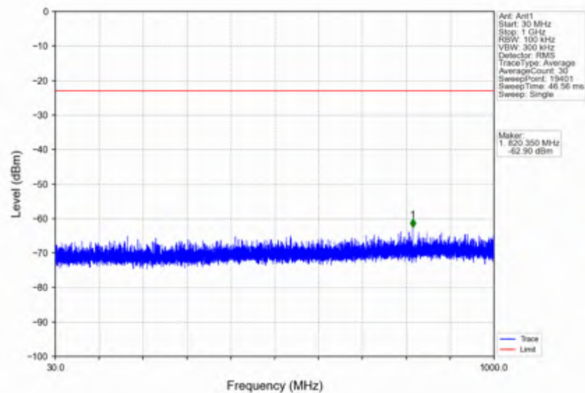
n66_15kHz_SISO_NTNV_20MHz_DFT-s-OFDM_QPSK_1770MHz_Edge_1RB_Right
