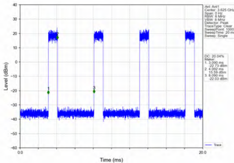
n78d_15kHz_SISO_NTNV_10MHz_CP-OFDM 64 QAM_3625.005MHz_Inner_Full
