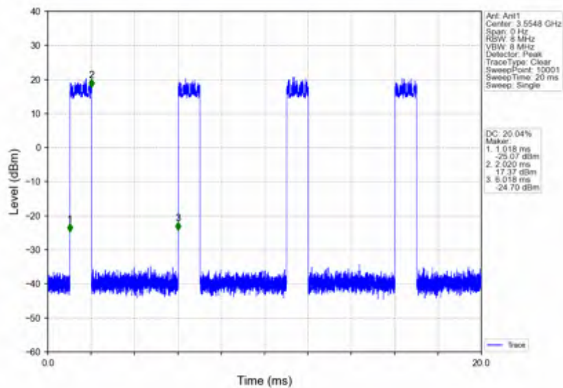
n78d_15kHz_SISO_NTNV_10MHz_DFT-s-OFDM_256_QAM_3555MHz_Inner_Full
