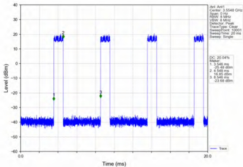
n78d_15kHz_SISO_NTNV_10MHz_DFT-s-OFDM 64 QAM_3555MHz_Inner_Full
