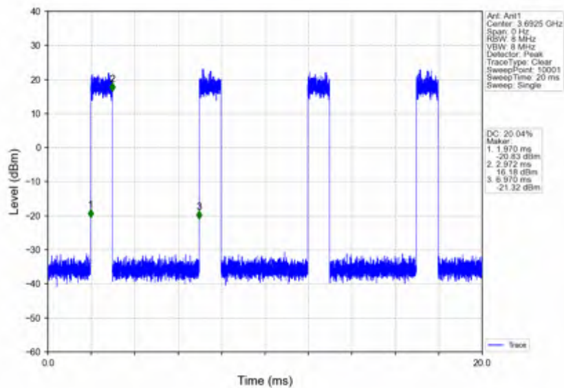
n78d_15kHz_SISO_NTNV_15MHz_CP-OFDM_256_QAM_3692.49MHz_Inner_Full
