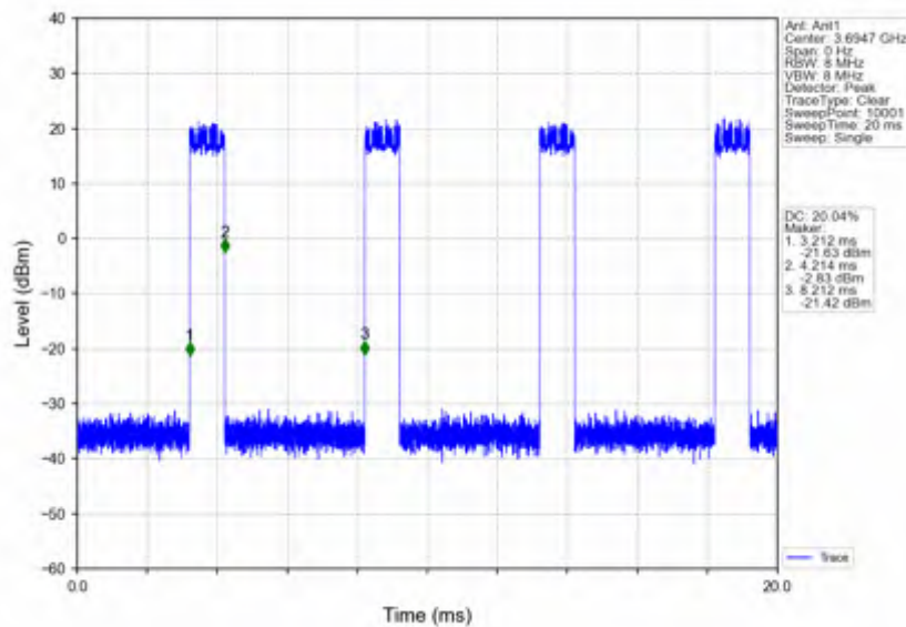
n78d_15kHz_SISO_NTNV_10MHz_DFT-s-OFDM 64 QAM_3694.995MHz_Inner_Full
