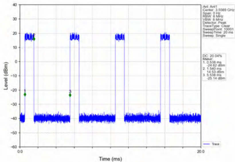
n78d_15kHz_SISO_NTNV_15MHz_DFT-s-OFDM 256 QAM_3557.505MHz_Inner_Full
