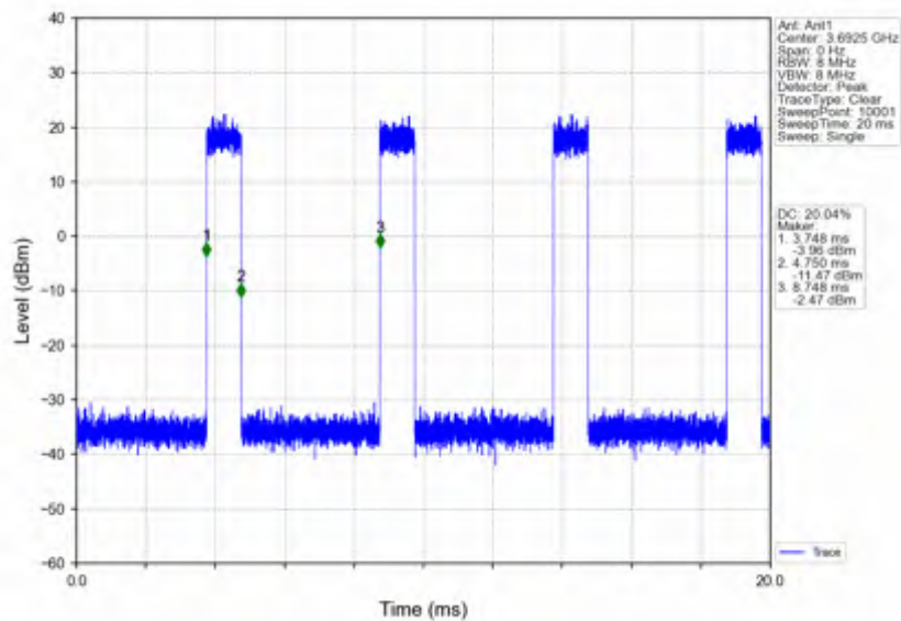
n78d_15kHz_SISO_NTNV_15MHz_CP-OFDM 64 QAM_3692.49MHz_Inner_Full
