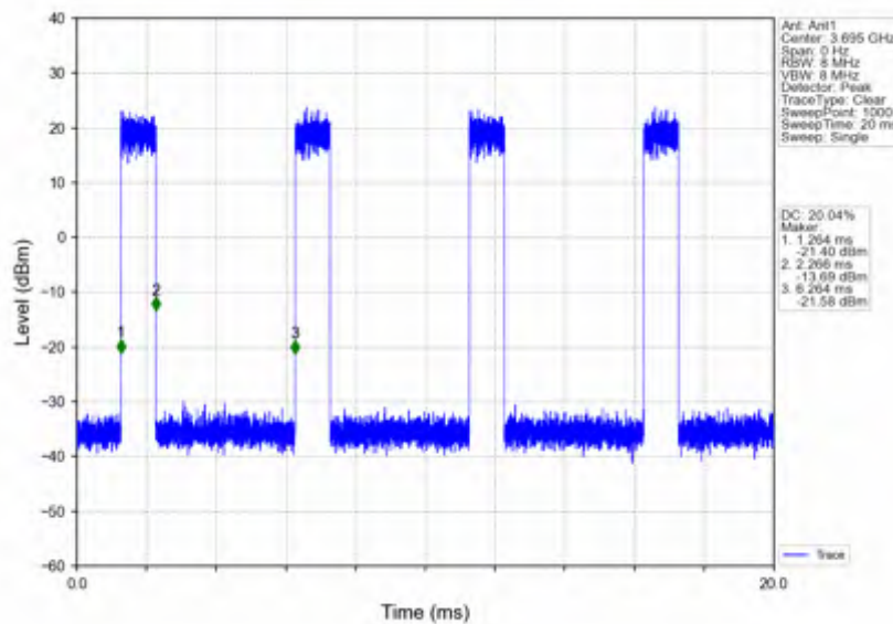
n78d_15kHz_SISO_NTNV_10MHz_CP-OFDM QPSK_3694.995MHz_Inner_Full
