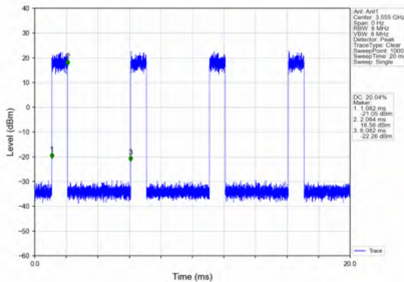
n78d_15kHz_SISO_NTNV_10MHz_CP-OFDM_16 QAM_3555MHz_Inner_Full
