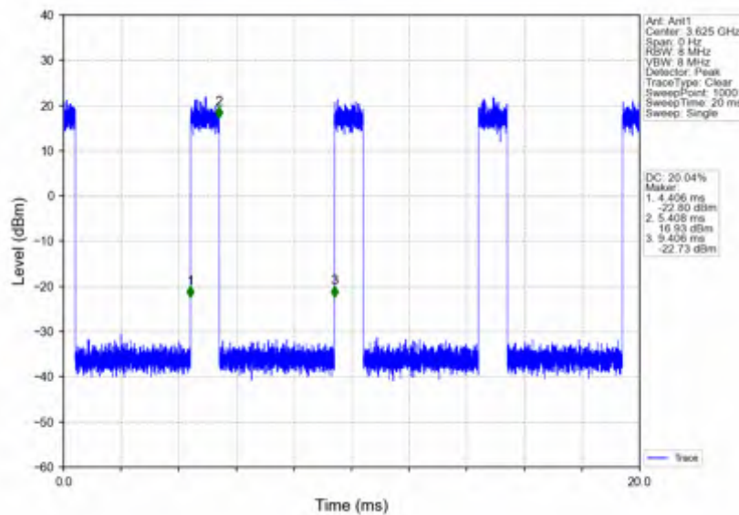
n78d_15kHz_SISO_NTNV_15MHz_CP-OFDM_64_QAM_3625.005MHz_Inner_Full
