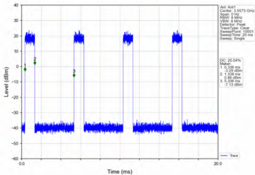
n78d_15kHz_SISO_NTNV_15MHz_CP-OFDM_64_QAM_3557.505MHz_Inner_Full
