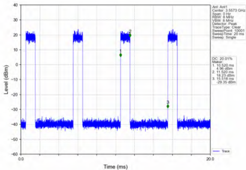
n78d_15kHz_SISO_NTNV_15MHz_CP-OFDM_QPSK_3557.505MHz_Inner_Full
