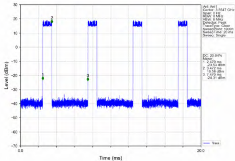
n78d_15kHz_SISO_NTNV_10MHz_DFT-s-OFDM_QPSK_3555MHz_Inner_Full
