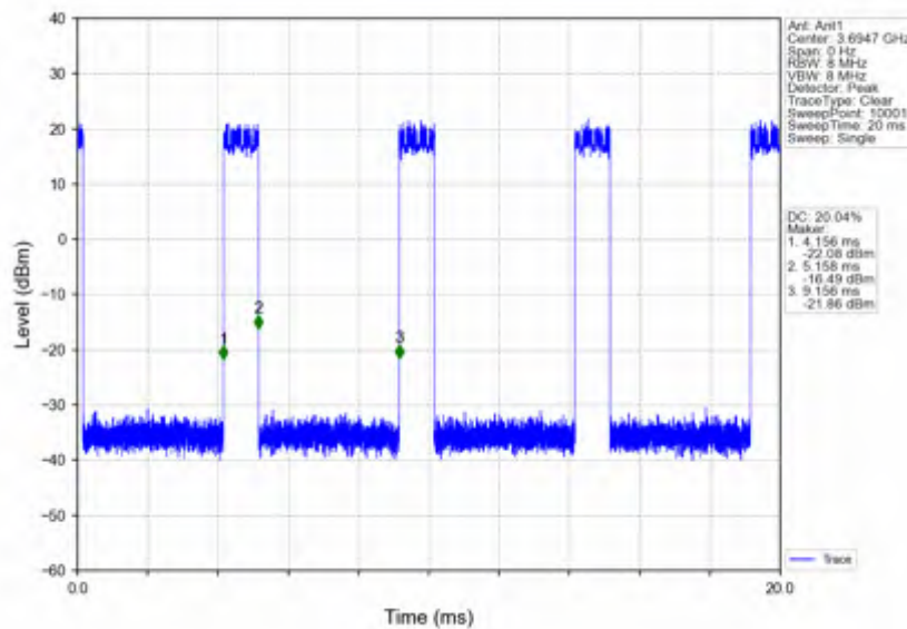
n78d_15kHz_SISO_NTNV_10MHz_DFT-s-OFDM_16_QAM_3694.995MHz_Inner_Full
