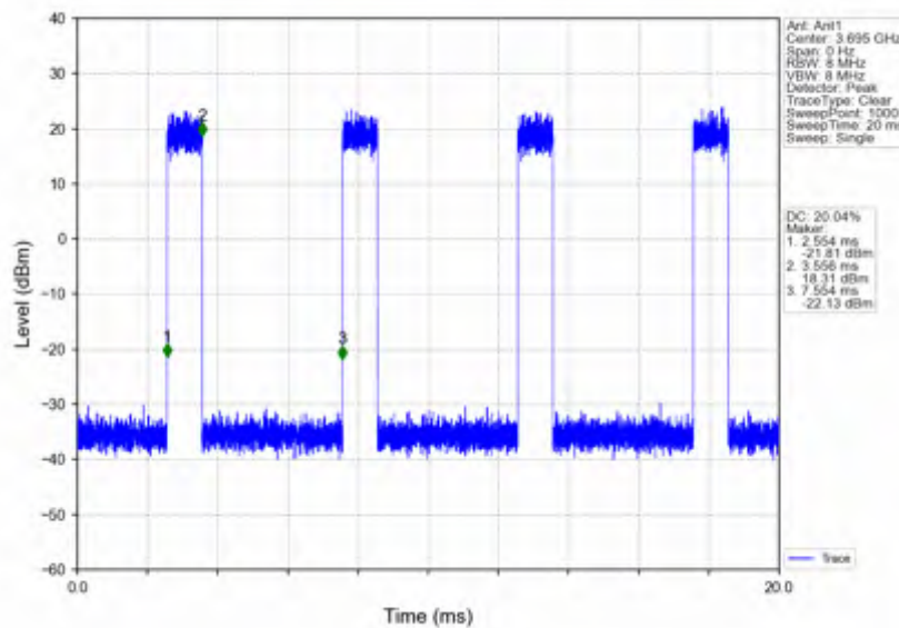
n78d_15kHz_SISO_NTNV_10MHz_CP-OFDM 64 QAM_3694.995MHz_Inner_Full
