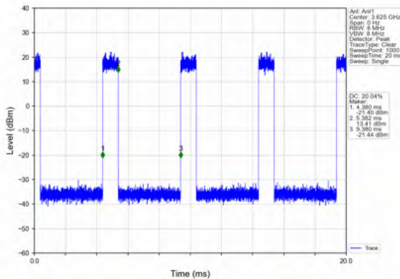
n78d_15kHz_SISO_NTNV_15MHz_CP-OFDM_16_QAM_3625.005MHz_Inner_Full
