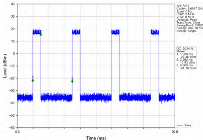
n78d_15kHz_SISO_NTNV_10MHz_DFT-s-OFDM QPSK_3694.995MHz_Inner_Full
