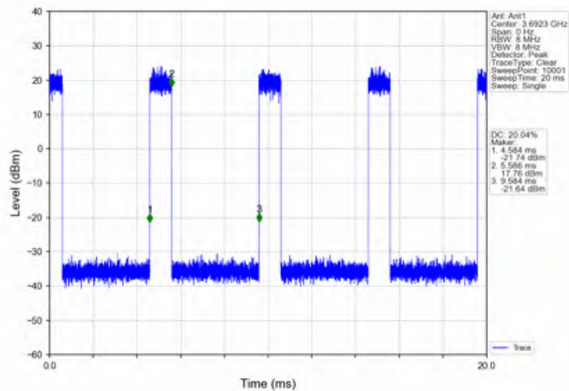
n78d_15kHz_SISO_NTNV_15MHz_CP-OFDM_QPSK_3692.49MHz_Inner_Full
