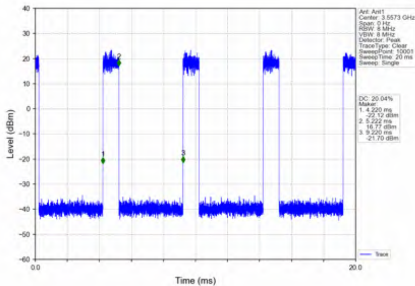
n78d_15kHz_SISO_NTNV_15MHz_CP-OFDM_16_QAM_3557.505MHz_Inner_Full
