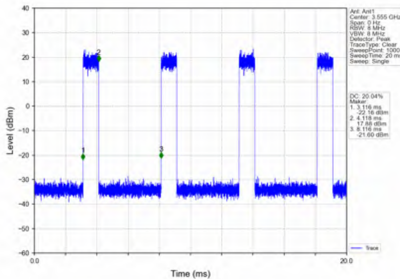
n78d_15kHz_SISO_NTNV_10MHz_CP-OFDM 64 QAM_3555MHz_Inner_Full
