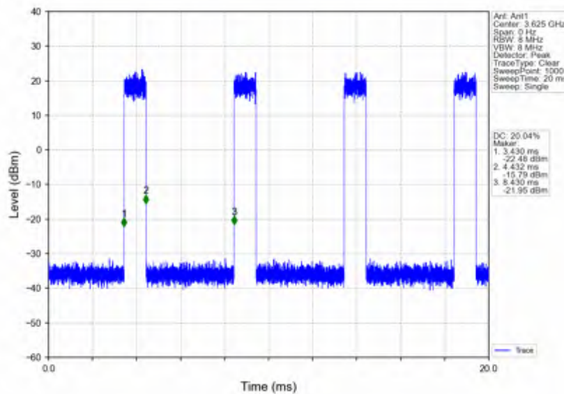
n78d_15kHz_SISO_NTNV_10MHz_CP-OFDM_16_QAM_3625.005MHz_Inner_Full
