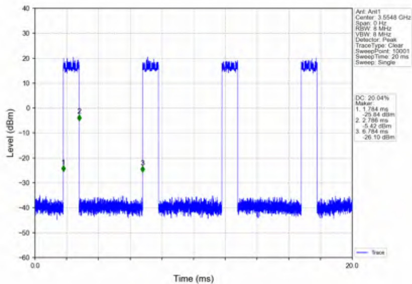
n78d_15kHz_SISO_NTNV_10MHz_DFT-s-OFDM_16_QAM_3555MHz_Inner_Full
