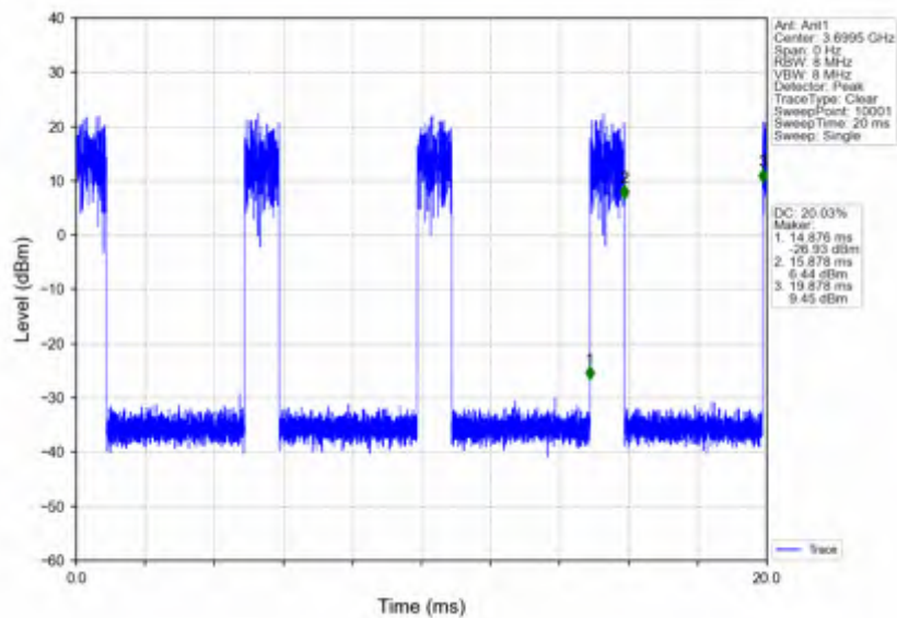
n78d_15kHz_SISO_NTNV_15MHz_CP-OFDM 64 QAM_3692.49MHz_Edge_1RB_Right
