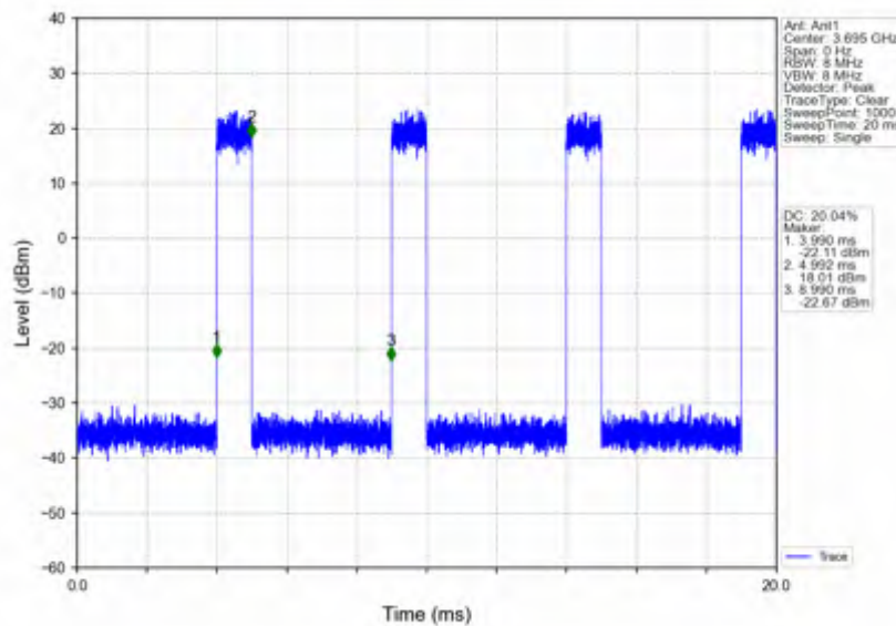
n78d_15kHz_SISO_NTNV_10MHz_CP-OFDM_16_QAM_3694.995MHz_Inner_Full
