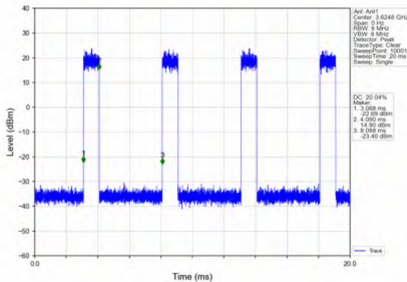
n78d_15kHz_SISO_NTNV_15MHz_CP-OFDM_64_QAM_3625.005MHz_Inner_Full
