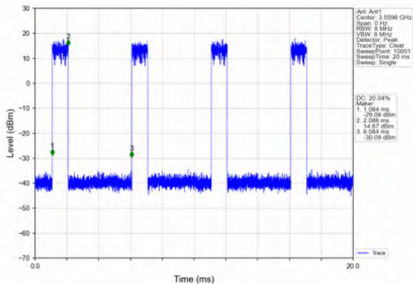
n78d_15kHz_SISO_NTNV_10MHz_DFT-s-OFDM_PI/2_BPSK_3555MHz_Edge_1RB_Right
