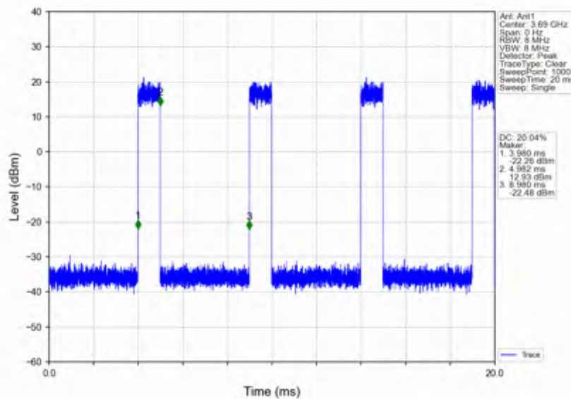
n78d_15kHz_SISO_NTNV_20MHz_CP-OFDM_16 QAM_3690MHz_Inner_Full
