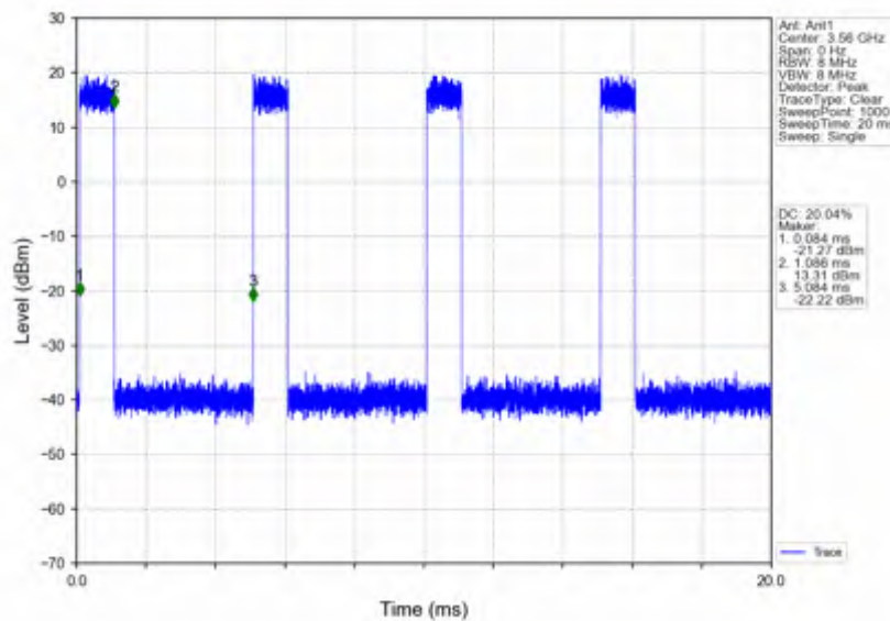
n78d_15kHz_SISO_NTNV_20MHz_CP-OFDM_256_QAM_3560.01MHz_Inner_Full
