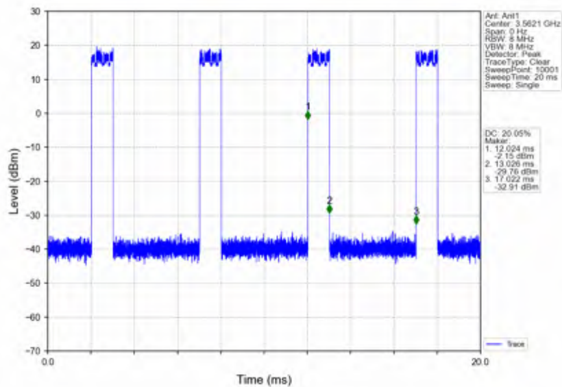
n78d_15kHz_SISO_NTNV_25MHz_DFT-s-OFDM_16_QAM_3562.5MHz_Inner_Full
