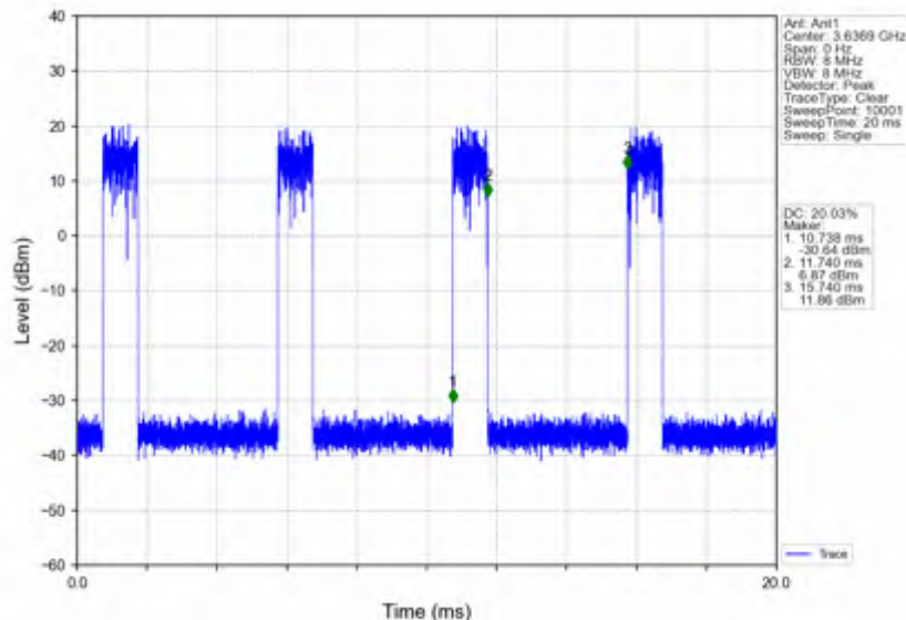
n78d_15kHz_SISO_NTNV_25MHz_DFT-s-OFDM_256_QAM_3625.005MHz_Edge_1RB_Right
