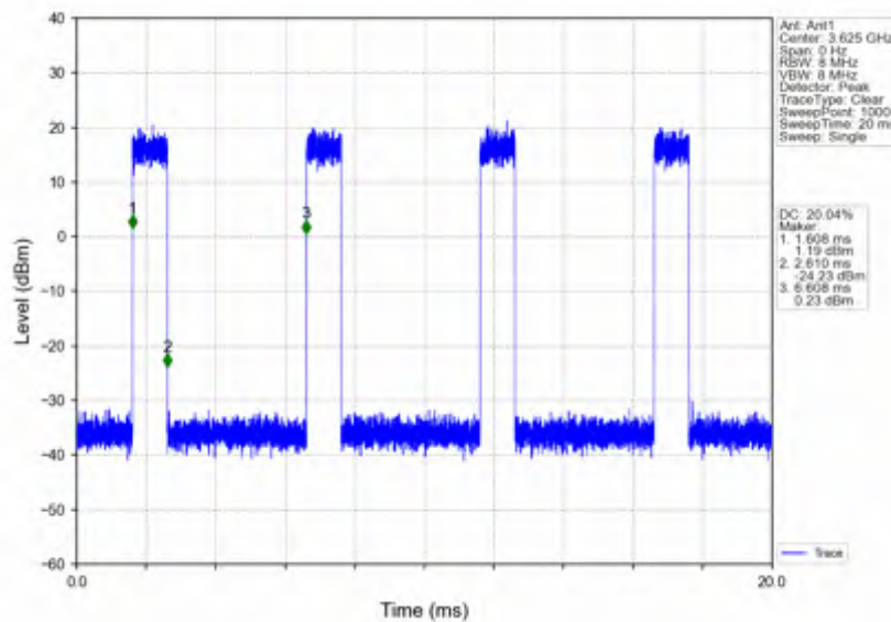
n78d_15kHz_SISO_NTNV_20MHz_CP-OFDM_QPSK_3625.005MHz_Inner_Full
