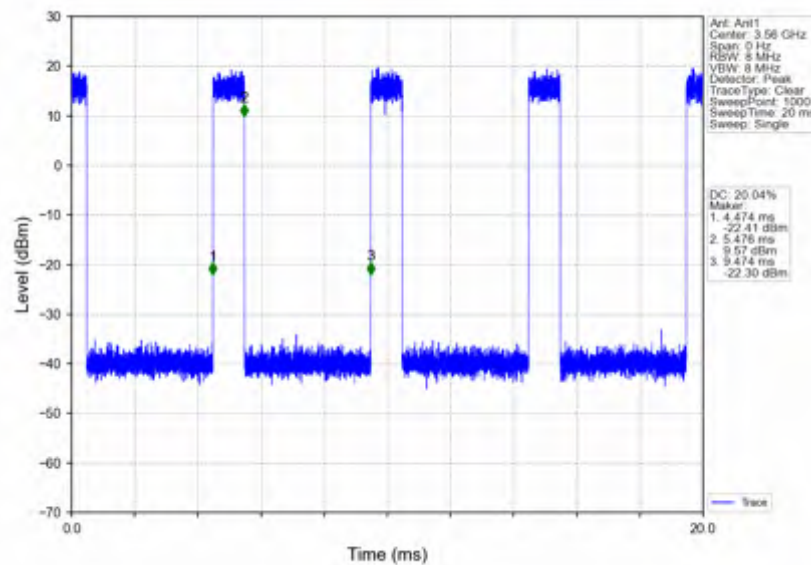
n78d_15kHz_SISO_NTNV_20MHz_CP-OFDM_QPSK_3560.01MHz_Inner_Full
