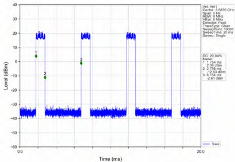
n78d_15kHz_SISO_NTNV_20MHz_DFT-s-OFDM_256_QAM_3690MHz_Inner_Full
