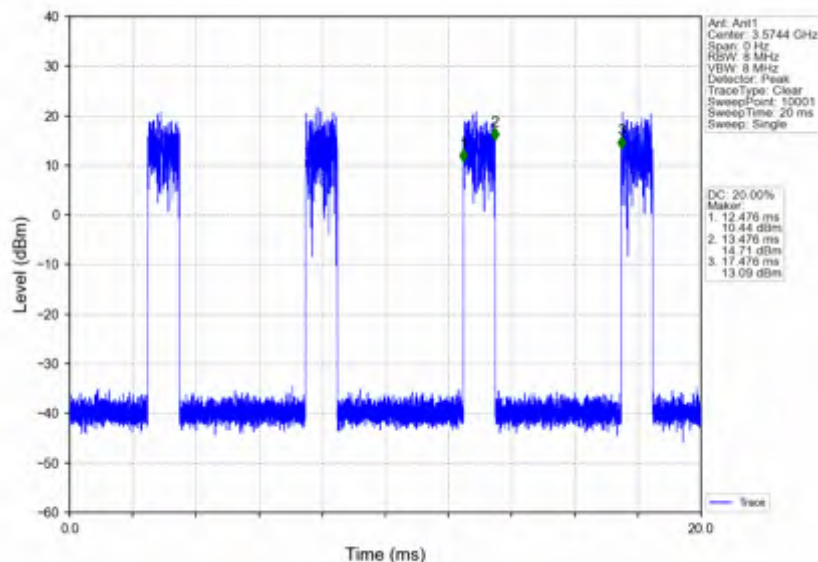
n78d_15kHz_SISO_NTNV_25MHz_CP-OFDM 16 QAM 3562.5MHz_Edge_1RB_Right
