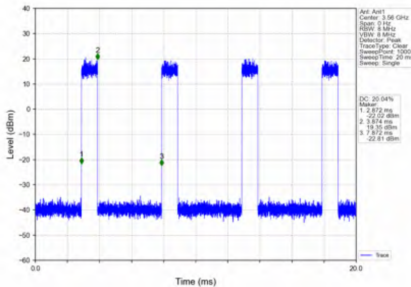
n78d_15kHz_SISO_NTNV_20MHz_CP-OFDM_16_QAM_3560.01MHz_Inner_Full
