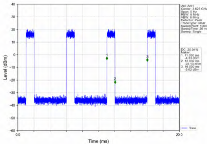
n78d_15kHz_SISO_NTNV_20MHz_CP-OFDM 256 QAM_3625.005MHz_Inner_Full
