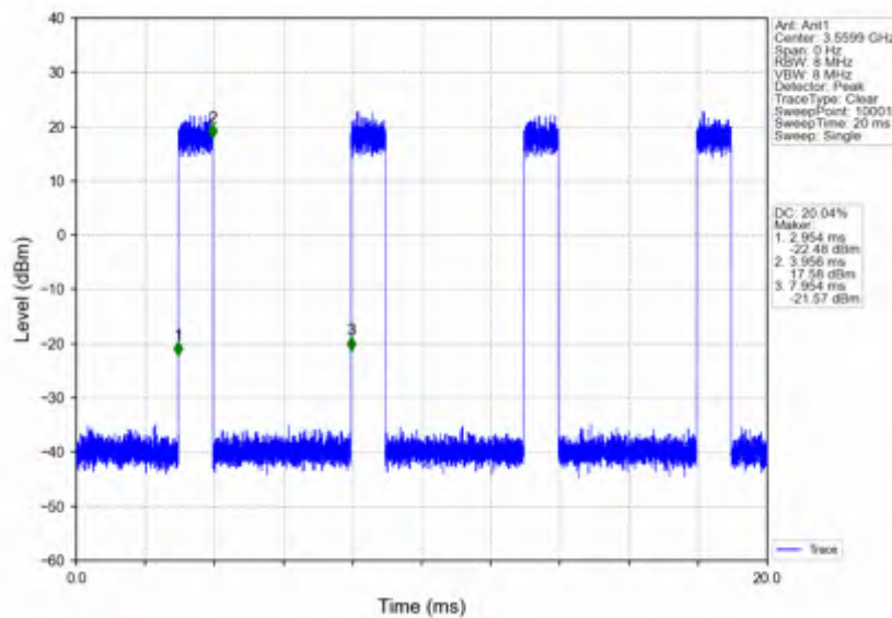
n78d_15kHz_SISO_NTNV_20MHz_CP-OFDM_256_QAM_3560.01MHz_Inner_Full
