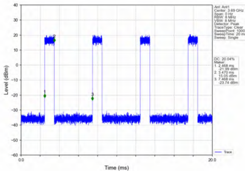
n78d_15kHz_SISO_NTNV_20MHz_CP-OFDM_QPSK_3690MHz_Inner_Full
