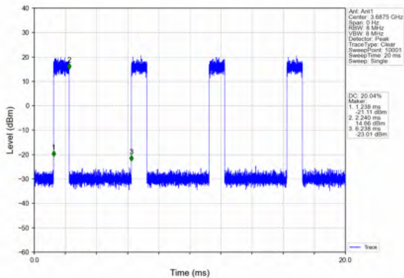
n78d_15kHz_SISO_NTNV_25MHz_CP-OFDM_16_QAM_3687.495MHz_Inner_Full
