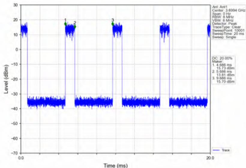
n78d_15kHz_SISO_NTNV_20MHz_DFT-s-OFDM PI/2 BPSK_3690MHz_Edge_1RB_Right
