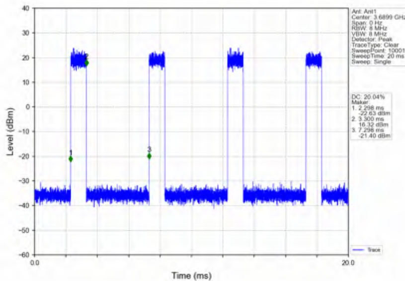
n78d_15kHz_SISO_NTNV_20MHz_CP-OFDM_16 QAM_3690MHz_Inner_Full
