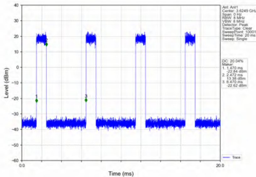
n78d_15kHz_SISO_NTNV_20MHz_CP-OFDM_QPSK_3625.005MHz_Inner_Full
