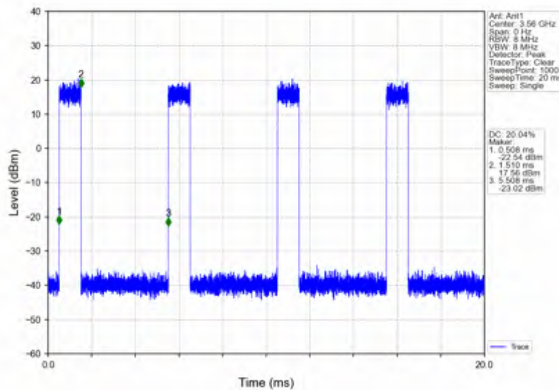
n78d_15kHz_SISO_NTNV_20MHz_CP-OFDM 64 QAM_3560.01MHz_Inner_Full
