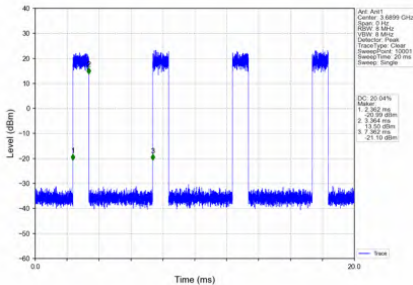
n78d_15kHz_SISO_NTNV_20MHz_CP-OFDM_QPSK_3690MHz_Inner_Full
