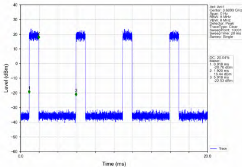
n78d_15kHz_SISO_NTNV_20MHz_CP-OFDM_256_QAM_3690MHz_Inner_Full
