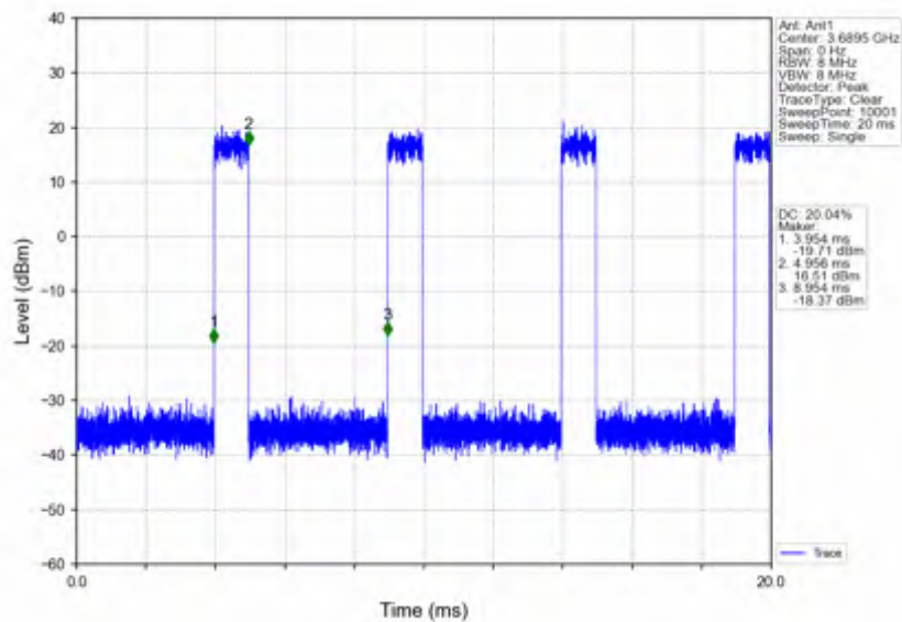
n78d_15kHz_SISO_NTNV_20MHz_DFT-s-OFDM_16_QAM_3690MHz_Inner_Full
