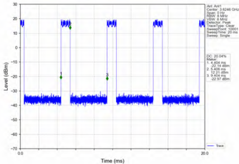
n78d_15kHz_SISO_NTNV_25MHz_DFT-s-OFDM_16_QAM_3625.005MHz_Inner_Full
