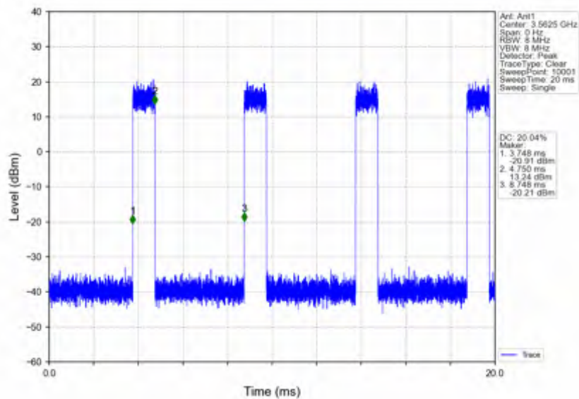
n78d_15kHz_SISO_NTNV_25MHz_CP-OFDM 256 QAM_3562.5MHz_Inner_Full
