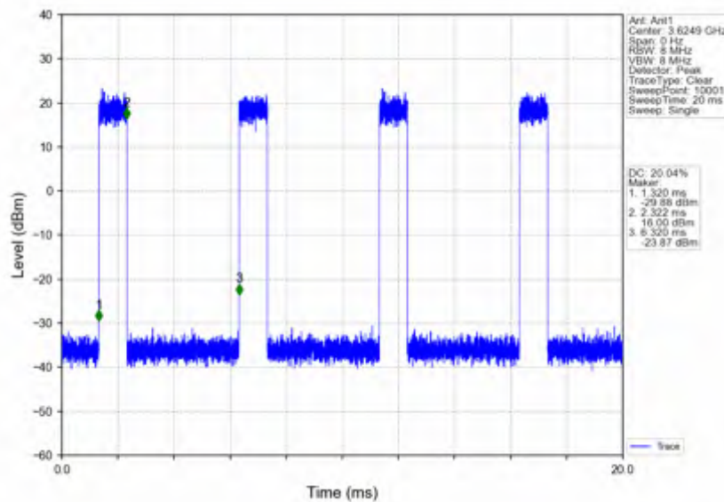
n78d_15kHz_SISO_NTNV_20MHz_CP-OFDM 256 QAM_3625.005MHz_Inner_Full
