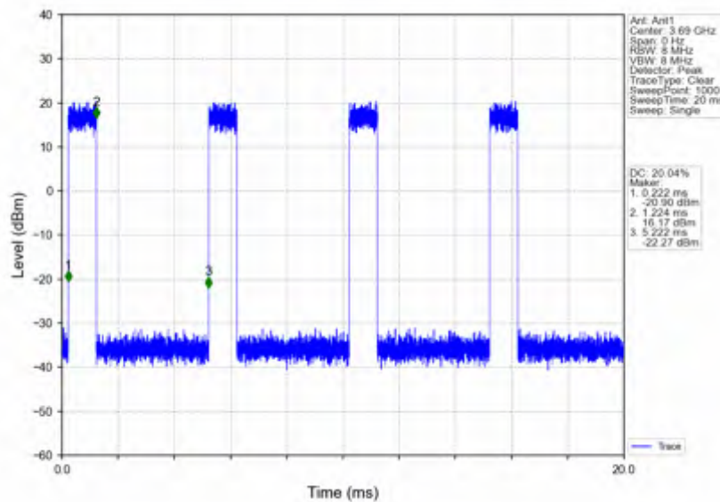
n78d_15kHz_SISO_NTNV_20MHz_CP-OFDM 64 QAM_3690MHz_Inner_Full
