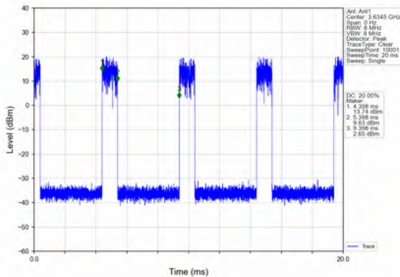
n78d_15kHz_SISO_NTNV_20MHz_DFT-s-OFDM_256_QAM_3625.005MHz_Edge_1RB_Right
