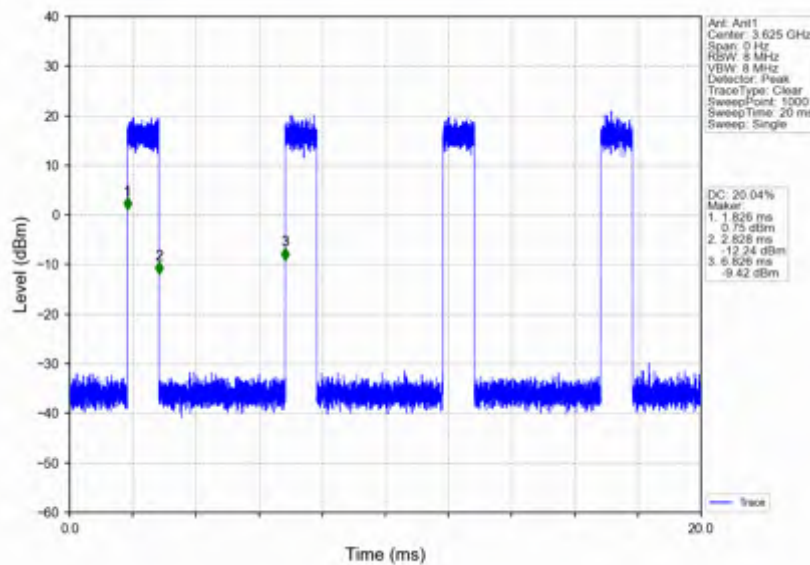
n78d_15kHz_SISO_NTNV_20MHz_CP-OFDM 64 QAM_3625.005MHz_Inner_Full
