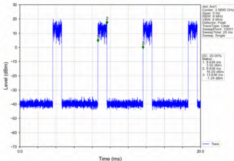
n78d_15kHz_SISO_NTNV_20MHz_DFT-s-OFDM_16_QAM_3560.01MHz_Edge_1RB_Right
