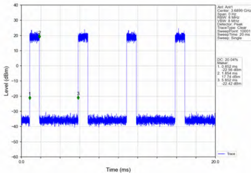
n78d_15kHz_SISO_NTNV_20MHz_CP-OFDM 64 QAM_3690MHz_Inner_Full
