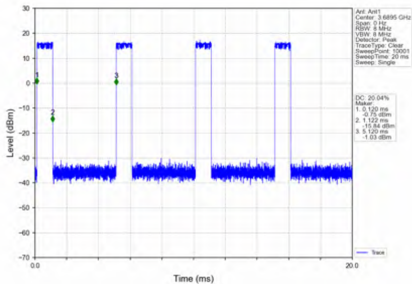
n78d_15kHz_SISO_NTNV_20MHz_DFT-s-OFDM_QPSK_3690MHz_Inner_Full
