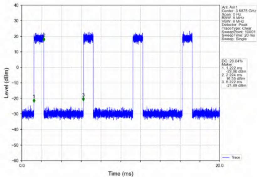
n78d_15kHz_SISO_NTNV_25MHz_CP-OFDM 64 QAM_3687.495MHz_Inner_Full
