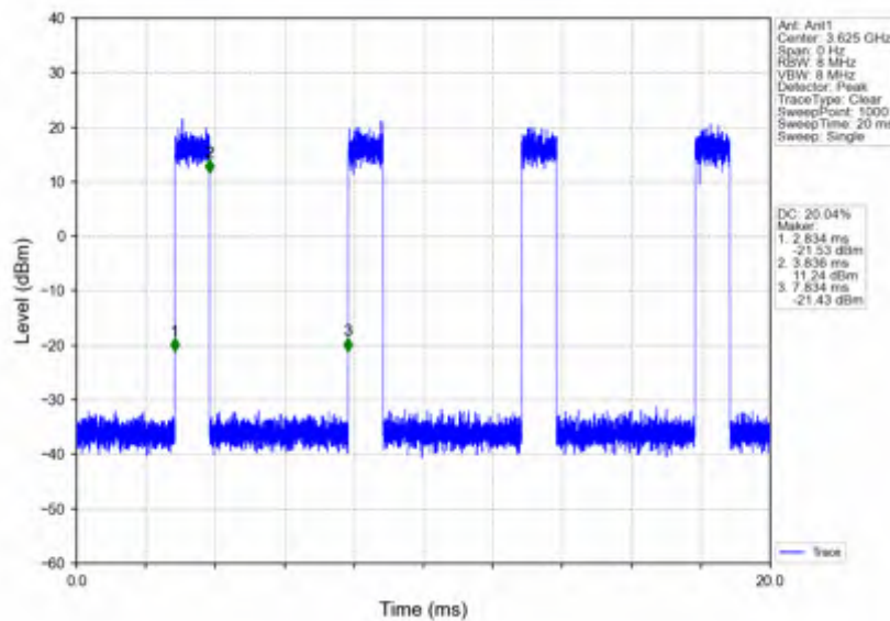
n78d_15kHz_SISO_NTNV_20MHz_CP-OFDM_16_QAM_3625.005MHz_Inner_Full
