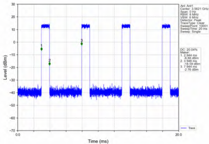
n78d_15kHz_SISO_NTNV_25MHz_DFT-s-OFDM PI/2 BPSK_3562.5MHz_Inner_Full
