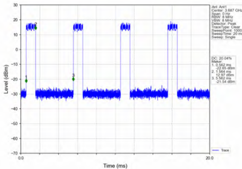
n78d_15kHz_SISO_NTNV_25MHz_DFT-s-OFDM 64 QAM_3687.495MHz_Inner_Full
