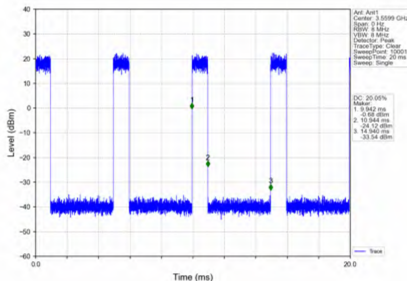
n78d_15kHz_SISO_NTNV_20MHz_CP-OFDM_QPSK_3560.01MHz_Inner_Full
