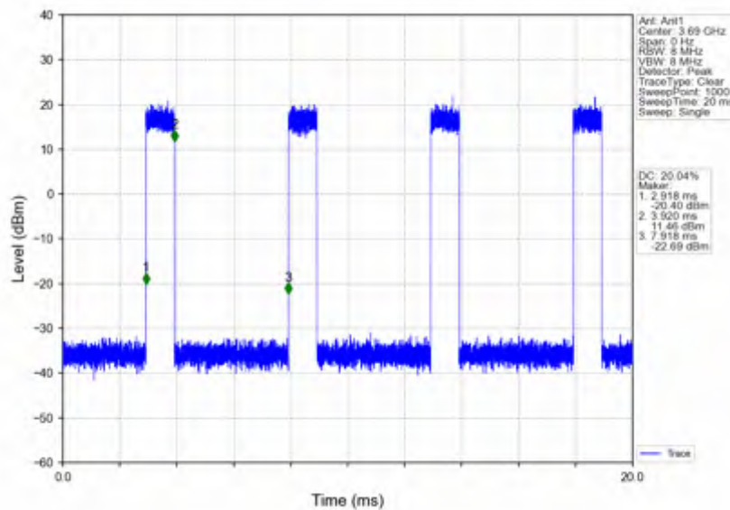
n78d_15kHz_SISO_NTNV_20MHz_CP-OFDM_256_QAM_3690MHz_Inner_Full
