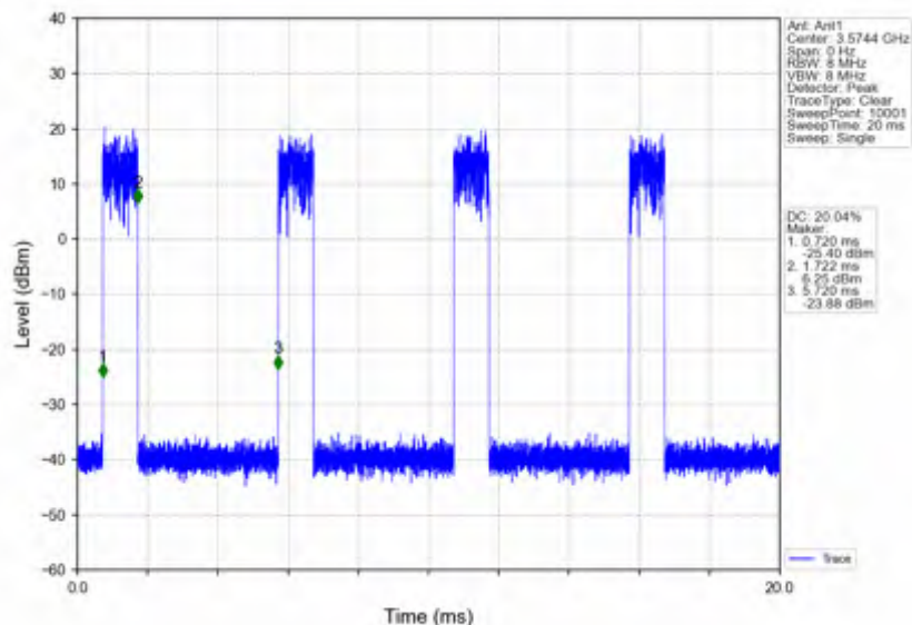
n78d_15kHz_SISO_NTNV_25MHz_DFT-s-OFDM_16_QAM_3562.5MHz_Edge_1RB_Right
