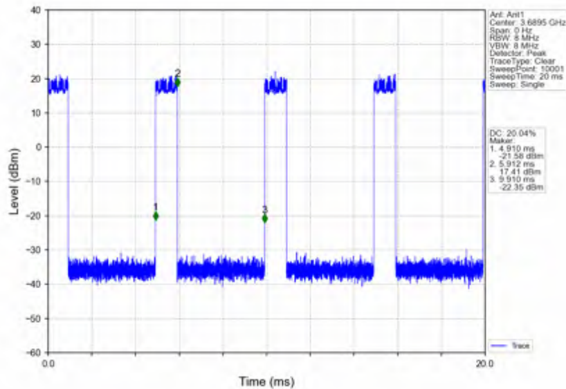
n78d_15kHz_SISO_NTNV_20MHz_DFT-s-OFDM 64 QAM_3690MHz_Inner_Full
