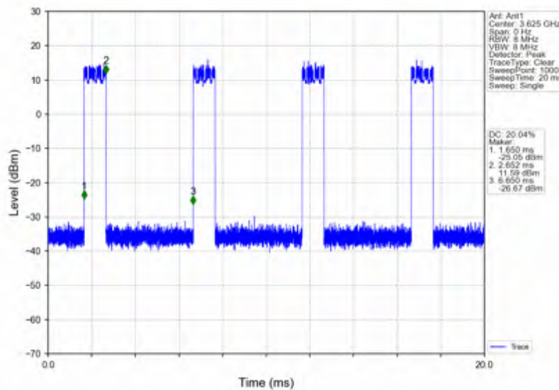
n78d_15kHz_SISO_NTNV_50MHz_DFT-s-OFDM QPSK_3625.005MHz_Inner_Full
