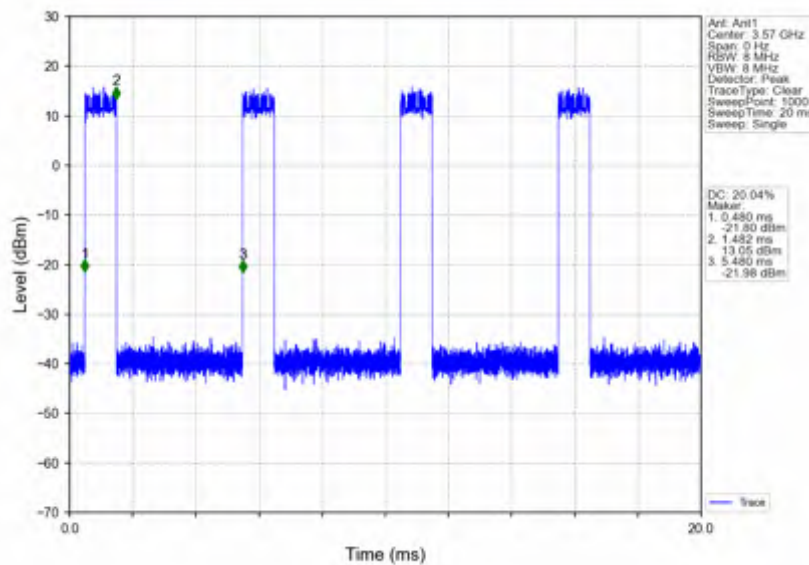
n78d_15kHz_SISO_NTNV_40MHz_DFT-s-OFDM_16_QAM_3570MHz_Inner_Full
