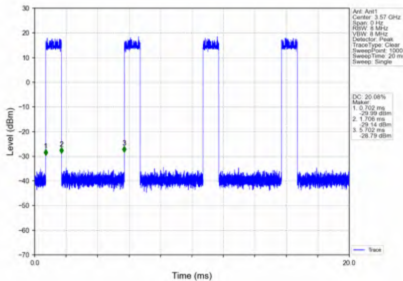
n78d_15kHz_SISO_NTNV_40MHz_DFT-s-OFDM_256_QAM_3570MHz_Inner_Full
