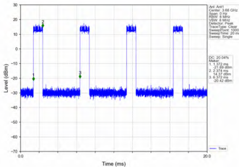
n78d_15kHz_SISO_NTNV_40MHz_DFT-s-OFDM_16_QAM_3679.995MHz_Inner_Full
