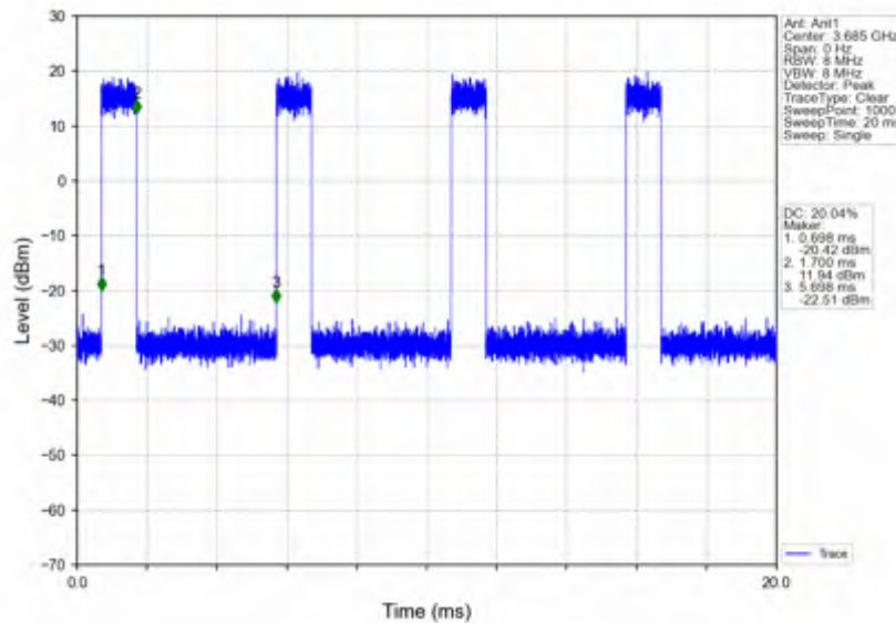
n78d_15kHz_SISO_NTNV_30MHz_CP-OFDM_256_QAM_3684.99MHz_Inner_Full
