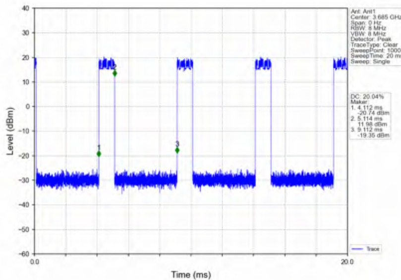
n78d_15kHz_SISO_NTNV_30MHz_DFT-s-OFDM 64 QAM_3684.99MHz_Inner_Full
