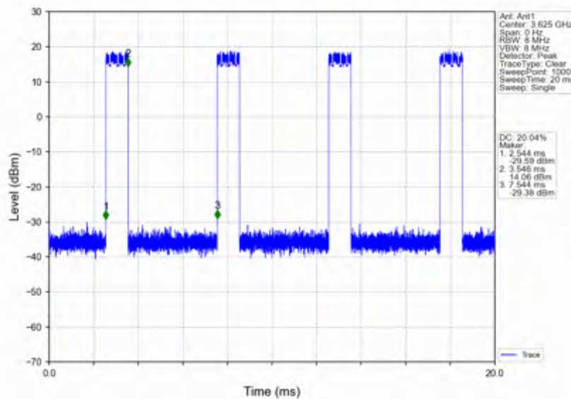
n78d_15kHz_SISO_NTNV_30MHz_DFT-s-OFDM_16_QAM_3625.005MHz_Inner_Full
