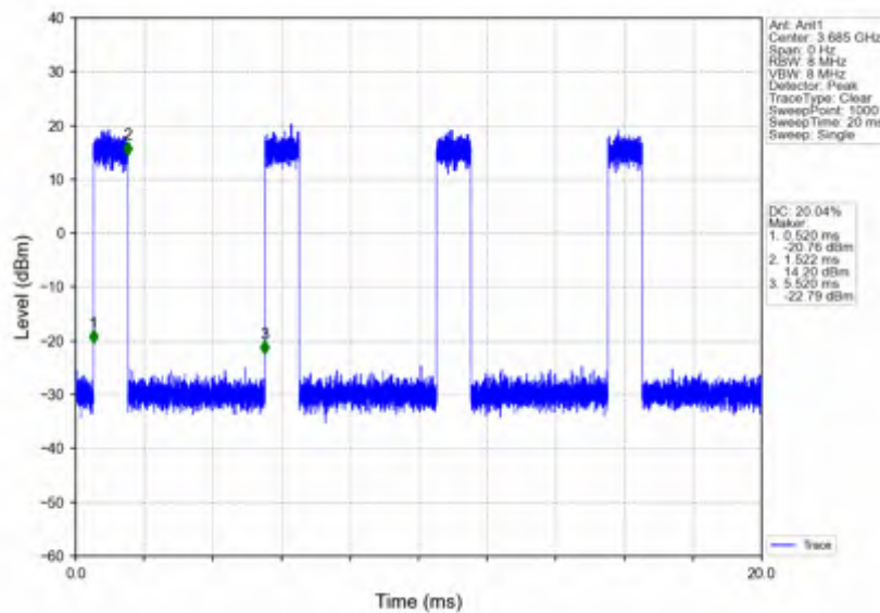
n78d_15kHz_SISO_NTNV_30MHz_CP-OFDM 64 QAM_3684.99MHz_Inner_Full
