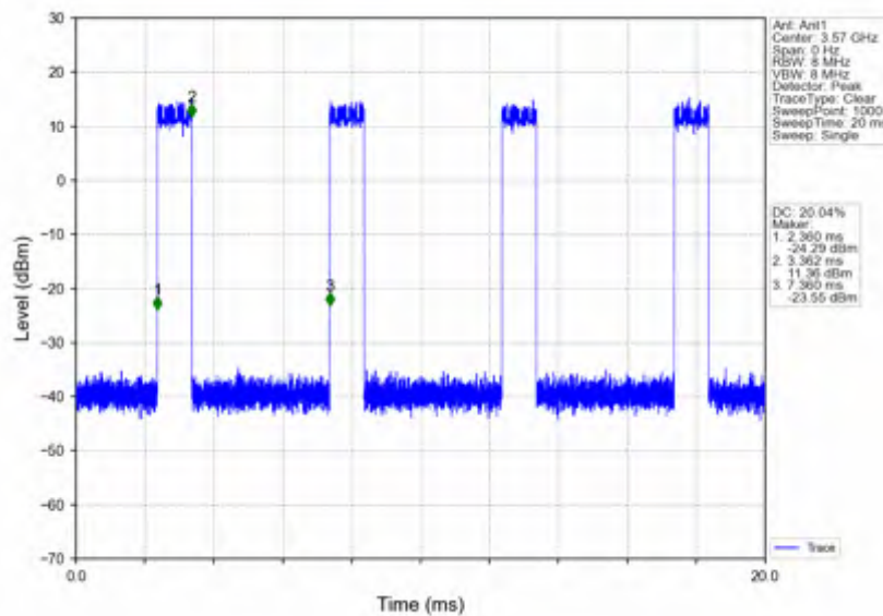
n78d_15kHz_SISO_NTNV_40MHz_DFT-s-OFDM_QPSK_3570MHz_Inner_Full
