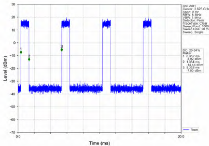
n78d_15kHz_SISO_NTNV_30MHz_CP-OFDM_16_QAM_3625.005MHz_Inner_Full
