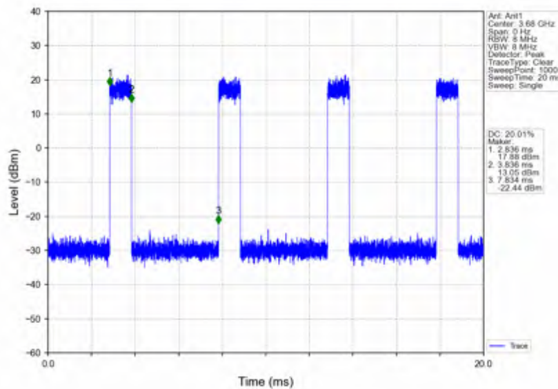
n78d_15kHz_SISO_NTNV_40MHz_CP-OFDM 64 QAM_3679.995MHz_Inner_Full
