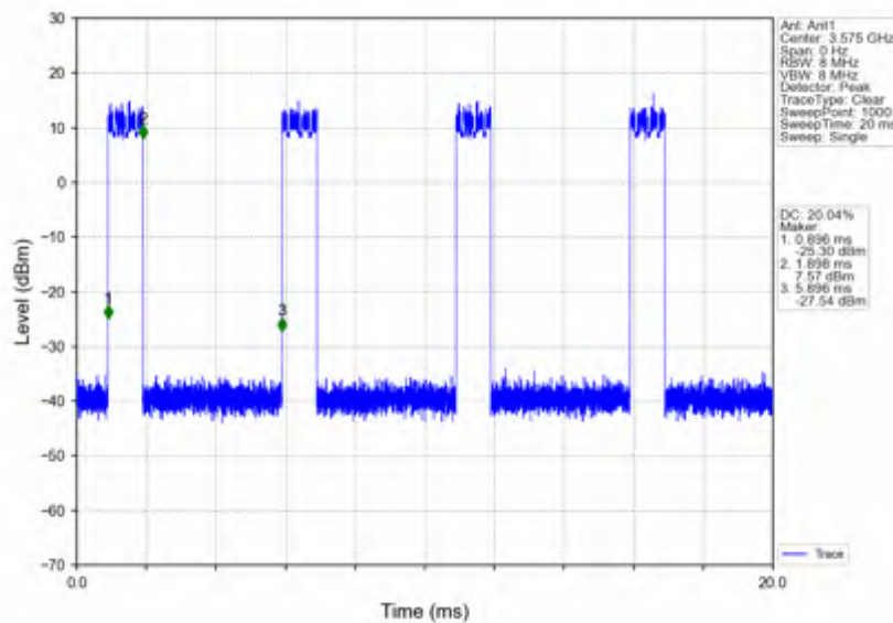
n78d_15kHz_SISO_NTNV_50MHz_DFT-s-OFDM_QPSK_3575.01MHz_Inner_Full
