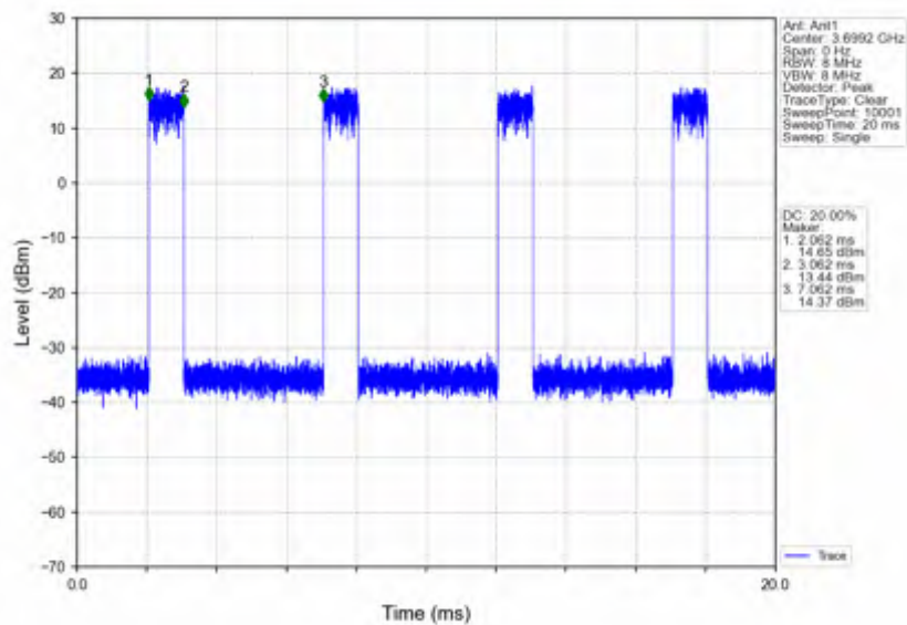
n78d_15kHz_SISO_NTNV_50MHz_DFT-s-OFDM PI/2 BPSK_3675MHz_Edge_1RB_Right
