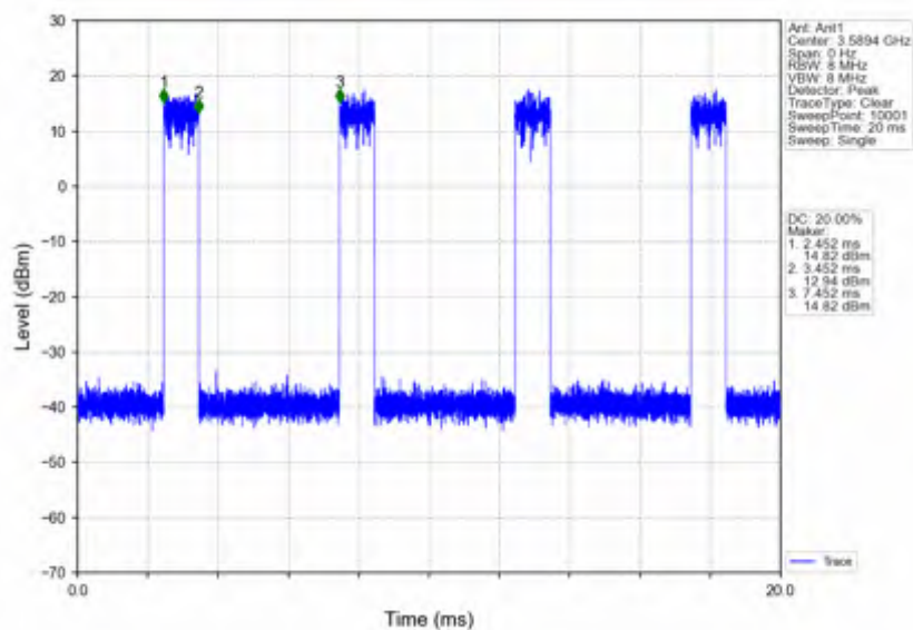
n78d_15kHz_SISO_NTNV_40MHz_DFT-s-OFDM_PI/2_BPSK_3570MHz_Edge_1RB_Right
