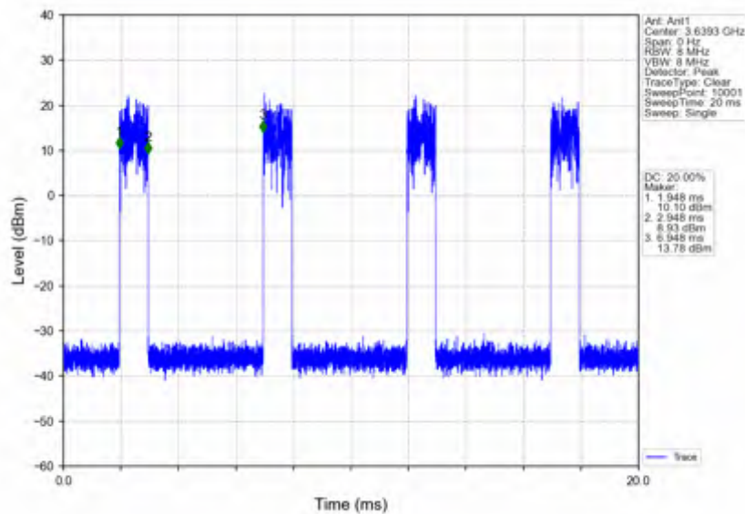
n78d_15kHz_SISO_NTNV_30MHz_CP-OFDM_256_QAM_3625.005MHz_Edge_1RB_Right
