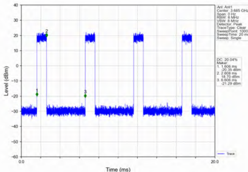
n78d_15kHz_SISO_NTNV_30MHz_CP-OFDM QPSK_3684.99MHz_Inner_Full
