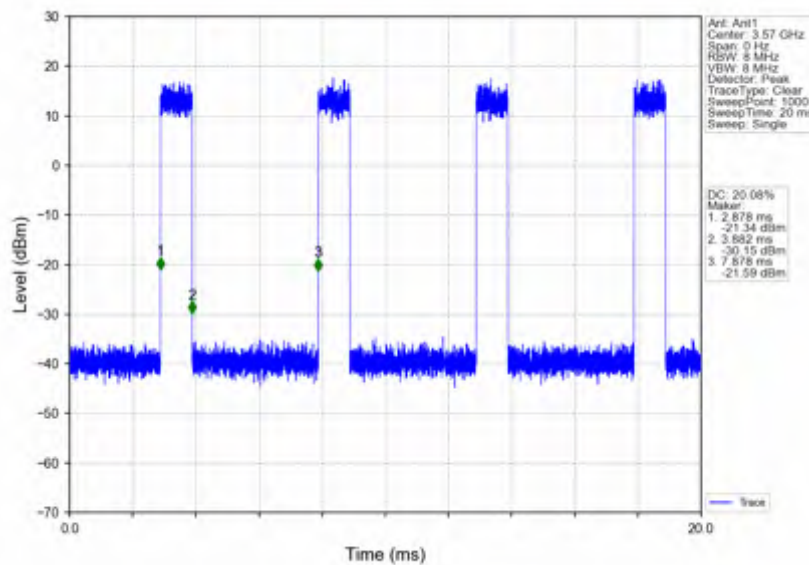
n78d_15kHz_SISO_NTNV_40MHz_CP-OFDM 64 QAM_3570MHz_Inner_Full
