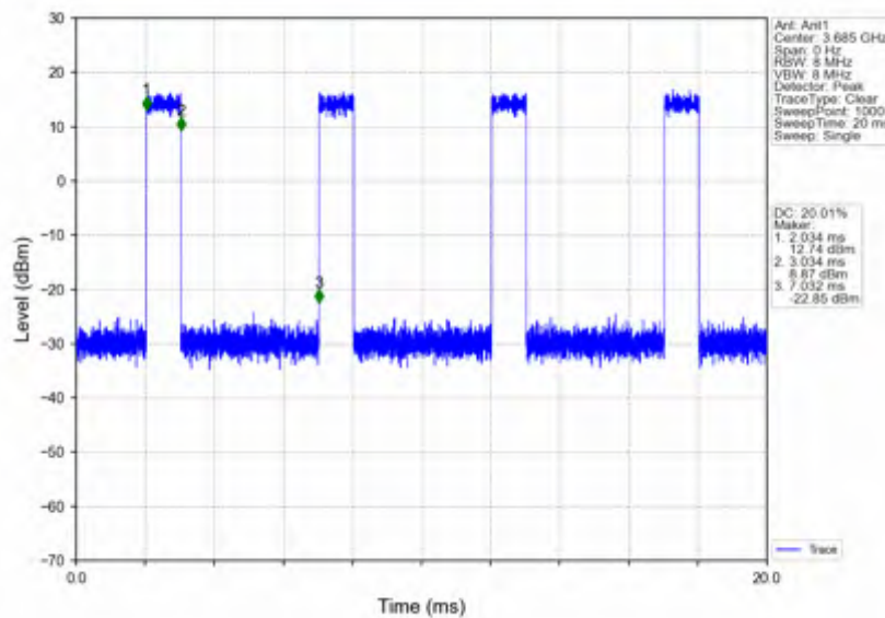
n78d_15kHz_SISO_NTNV_30MHz_DFT-s-OFDM_QPSK_3684.99MHz_Inner_Full
