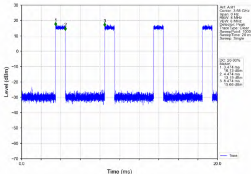
n78d_15kHz_SISO_NTNV_40MHz_DFT-s-OFDM QPSK_3679.995MHz_Inner_Full
