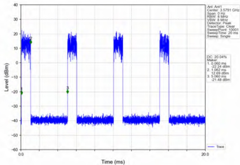
n78d_15kHz_SISO_NTNV_30MHz_CP-OFDM_256_QAM_3565.005MHz_Inner_1RB_Right
