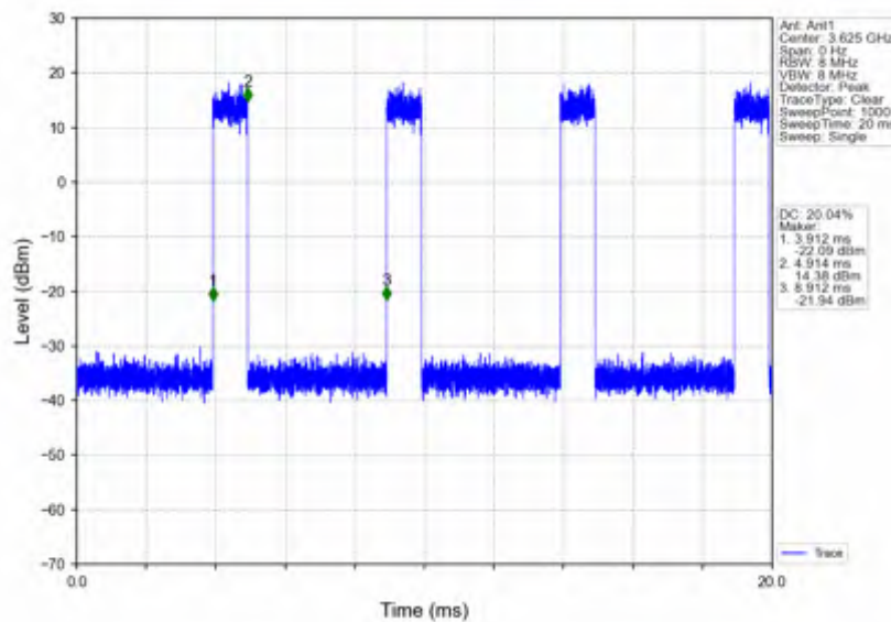
n78d_15kHz_SISO_NTNV_40MHz_CP-OFDM 64 QAM_3625.005MHz_Inner_Full
