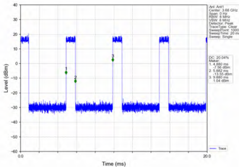
n78d_15kHz_SISO_NTNV_40MHz_DFT-s-OFDM 64 QAM_3679.995MHz_Inner_Full
