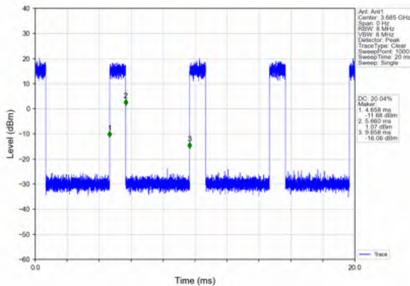
n78d_15kHz_SISO_NTNV_30MHz_CP-OFDM_16_QAM_3684.99MHz_Inner_Full
