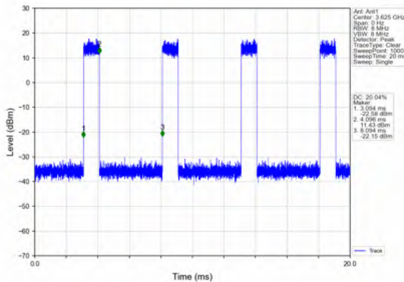
n78d_15kHz_SISO_NTNV_40MHz_CP-OFDM_16_QAM_3625.005MHz_Inner_Full
