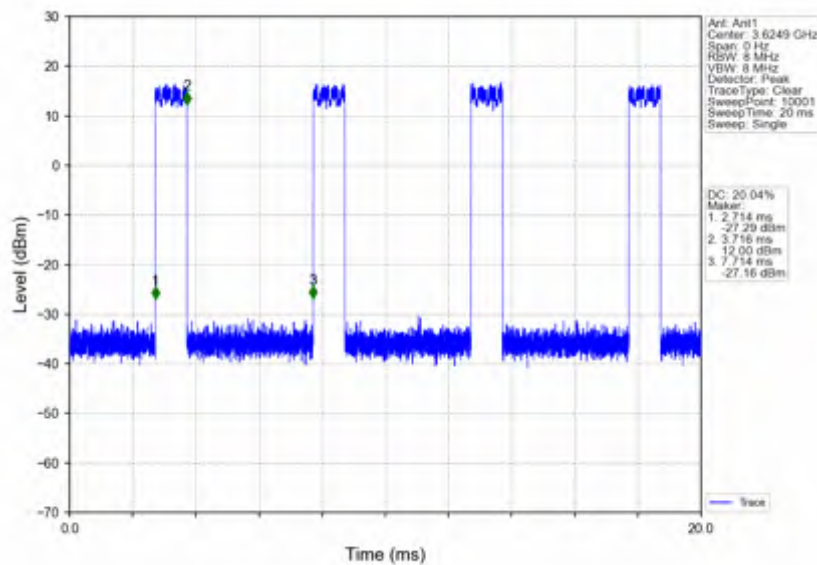
n78d_15kHz_SISO_NTNV_50MHz_DFT-s-OFDM QPSK_3625.005MHz_Inner_Full
