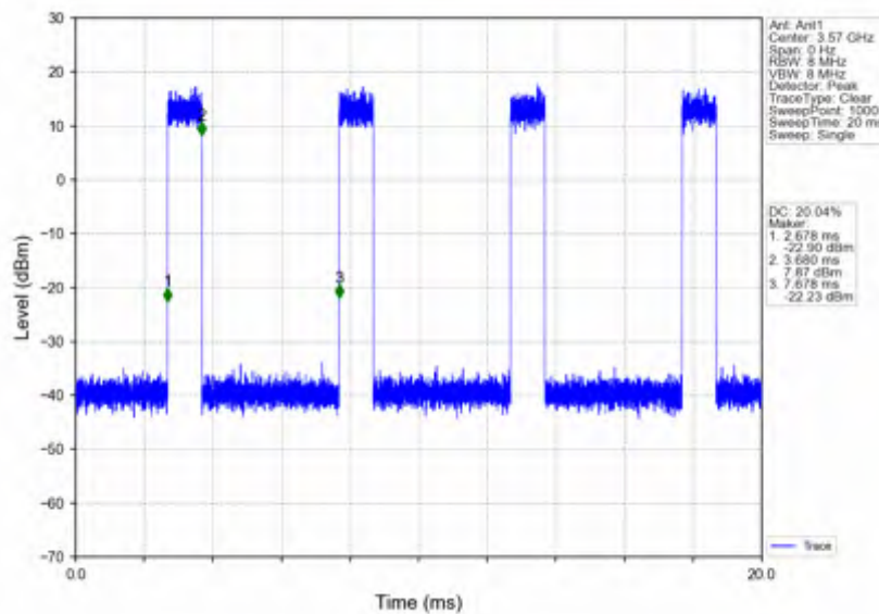
n78d_15kHz_SISO_NTNV_40MHz_CP-OFDM_QPSK_3570MHz_Inner_Full
