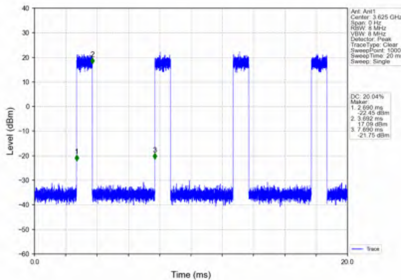
n78d_15kHz_SISO_NTNV_30MHz_CP-OFDM 64 QAM_3625.005MHz_Inner_Full
