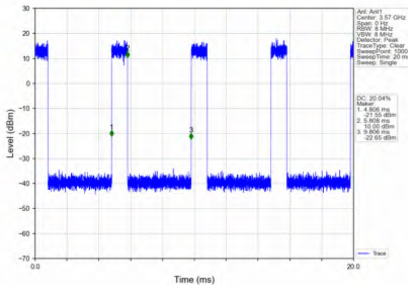
n78d_15kHz_SISO_NTNV_40MHz_CP-OFDM_16 QAM_3570MHz_Inner_Full
