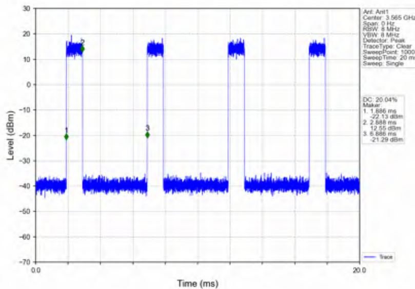
n78d_15kHz_SISO_NTNV_30MHz_CP-OFDM_64_QAM_3565.005MHz_Inner_Full
