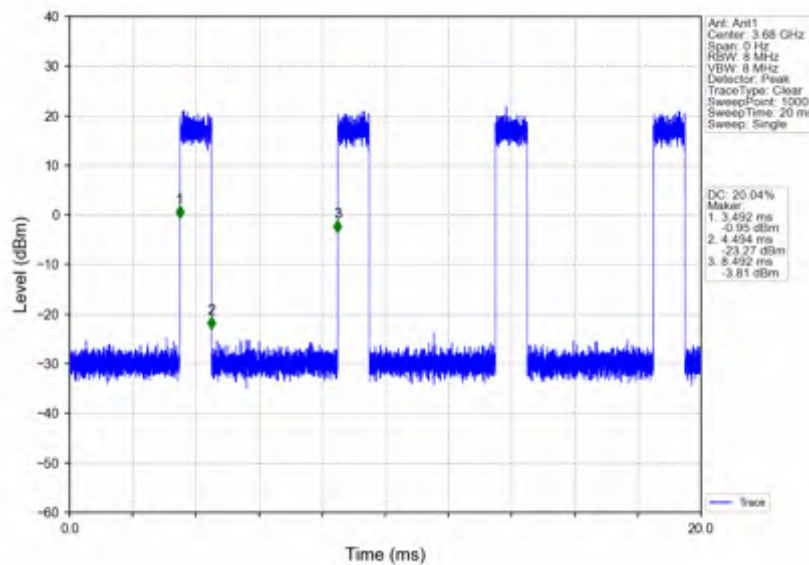
n78d_15kHz_SISO_NTNV_40MHz_CP-OFDM_16_QAM_3679.995MHz_Inner_Full
