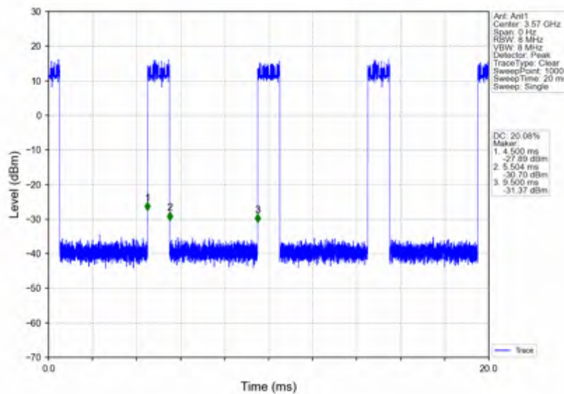
n78d_15kHz_SISO_NTNV_40MHz_DFT-s-OFDM 64 QAM_3570MHz_Inner_Full
