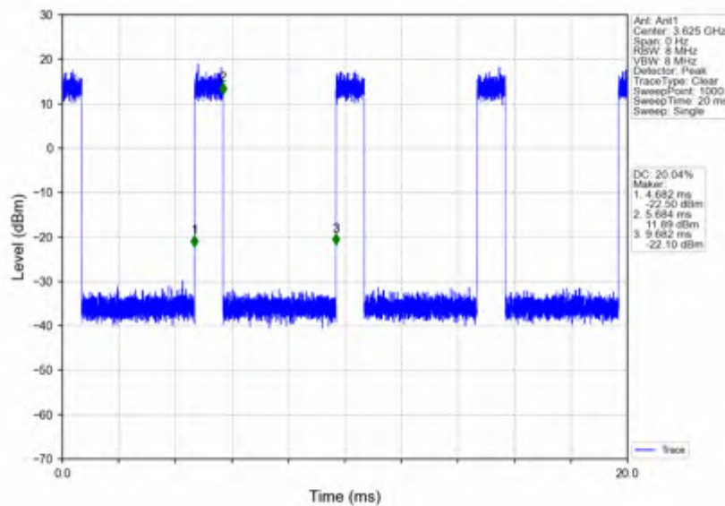
n78d_15kHz_SISO_NTNV_40MHz_CP-OFDM QPSK_3625.005MHz_Inner_Full
