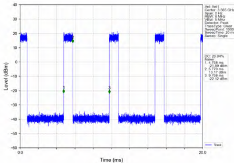
n78d_15kHz_SISO_NTNV_30MHz_CP-OFDM_16_QAM_3565.005MHz_Inner_Full
