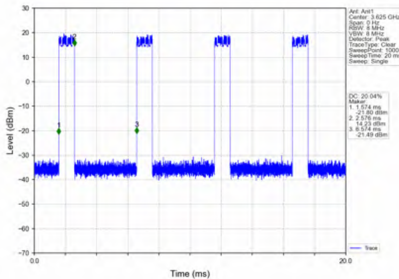
n78d_15kHz_SISO_NTNV_30MHz_DFT-s-OFDM 64 QAM_3625.005MHz_Inner_Full
