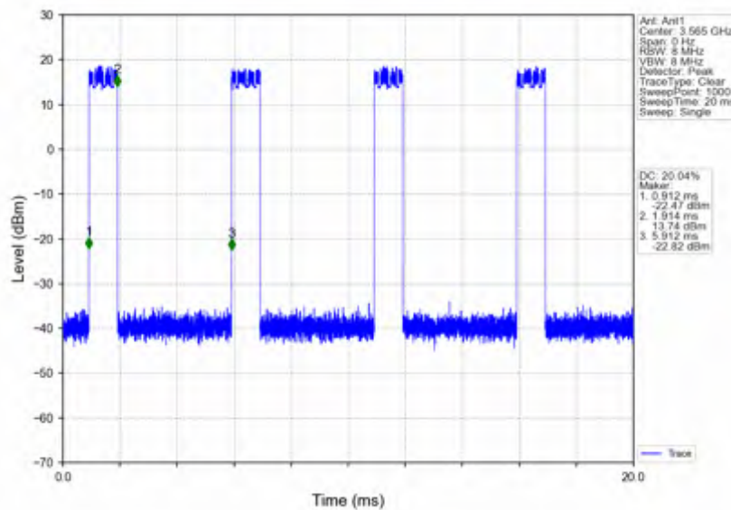
n78d_15kHz_SISO_NTNV_30MHz_DFT-s-OFDM 64 QAM_3565.005MHz_Inner_Full
