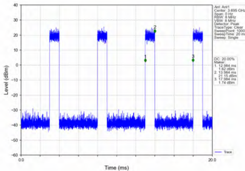
n78d_30kHz_SISO_NTNV_10MHz_CP-OFDM_16_QAM_3694.98MHz_Inner_Full
