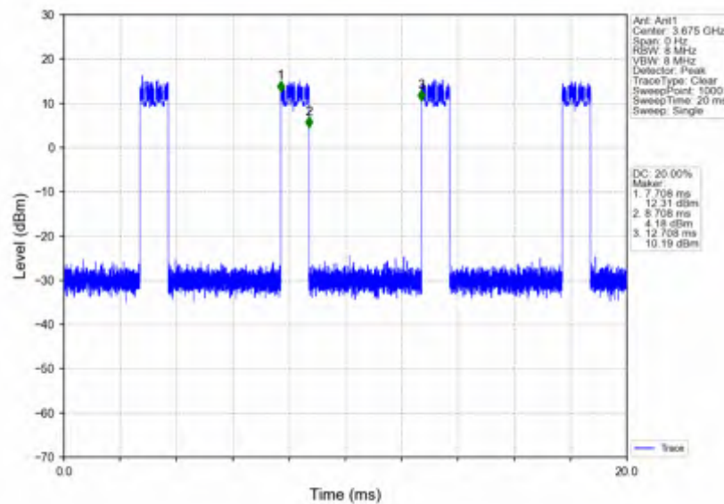
n78d_15kHz_SISO_NTNV_50MHz_DFT-s-OFDM_QPSK_3675MHz_Inner_Full
