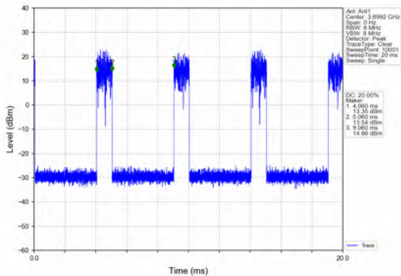
n78d_15kHz_SISO_NTNV_50MHz_CP-OFDM_16 QAM_3675MHz_Edge_1RB_Right
