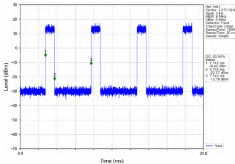
n78d_15kHz_SISO_NTNV_50MHz_CP-OFDM_QPSK_3675MHz_Inner_Full
