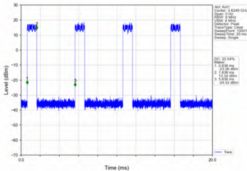
n78d_15kHz_SISO_NTNV_50MHz_DFT-s-OFDM 64 QAM_3625.005MHz_Inner_Full
