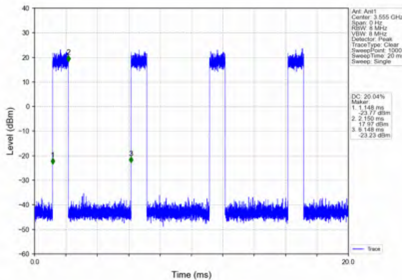
n78d_30kHz_SISO_NTNV_10MHz_CP-OFDM_QPSK_3555MHz_Inner_Full
