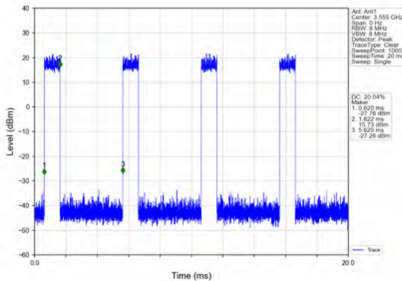
n78d_30kHz_SISO_NTNV_10MHz_DFT-s-OFDM 64 QAM_3555MHz_Inner_Full
