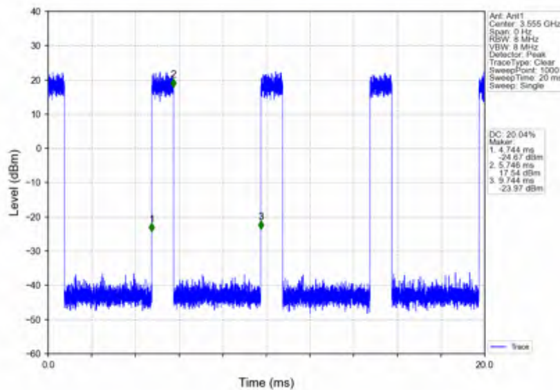
n78d_30kHz_SISO_NTNV_10MHz_CP-OFDM_16 QAM_3555MHz_Inner_Full
