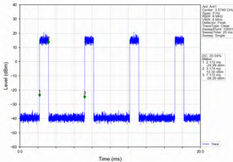
n78d_15kHz_SISO_NTNV_50MHz_CP-OFDM_QPSK_3575.01MHz_Inner_Full
