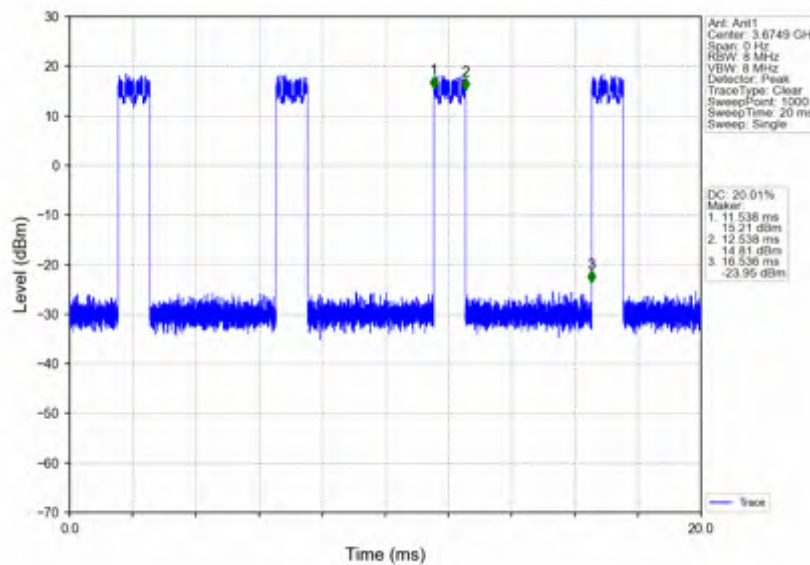
n78d_15kHz_SISO_NTNV_50MHz_DFT-s-OFDM 64 QAM_3675MHz_Inner_Full
