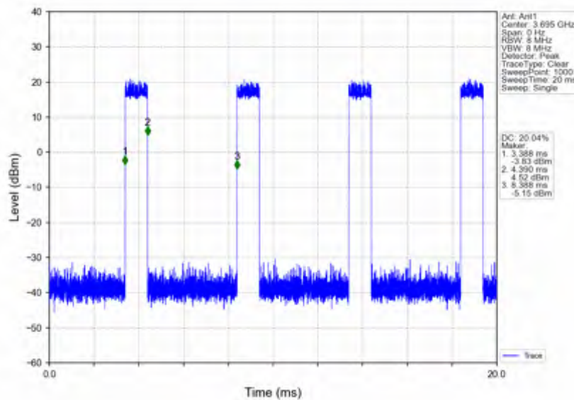
n78d_30kHz_SISO_NTNV_10MHz_DFT-s-OFDM_QPSK_3694.98MHz_Inner_Full
