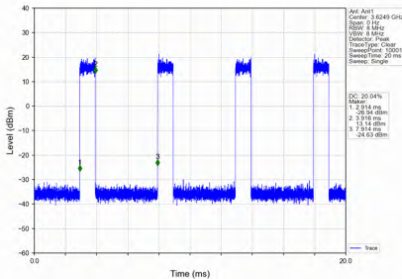
n78d_15kHz_SISO_NTNV_50MHz_CP-OFDM_16_QAM_3625.005MHz_Inner_Full
