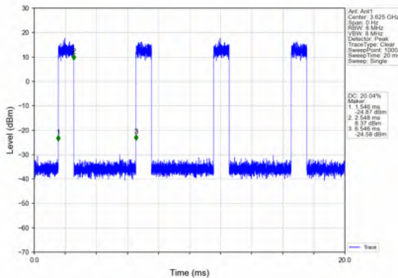
n78d_15kHz_SISO_NTNV_50MHz_CP-OFDM 64 QAM_3625.005MHz_Inner_Full
