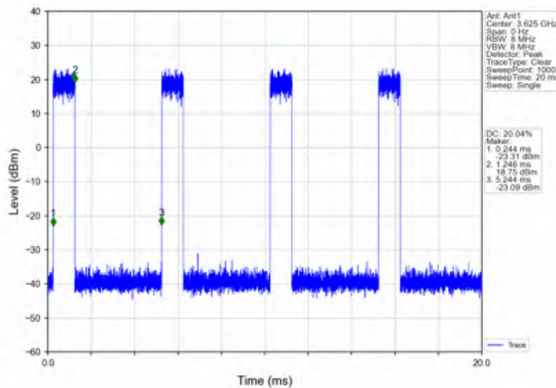
n78d_30kHz_SISO_NTNV_10MHz_CP-OFDM_QPSK_3624.99MHz_Inner_Full
