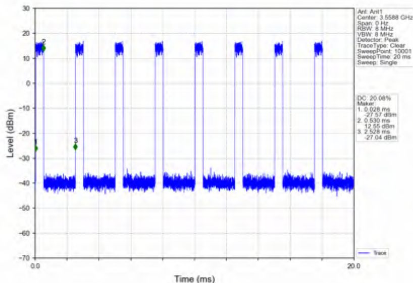
n78d_30kHz_SISO_NTNV_10MHz_DFT-s-OFDM PI/2 BPSK_3555MHz_Inner_1RB_Right
