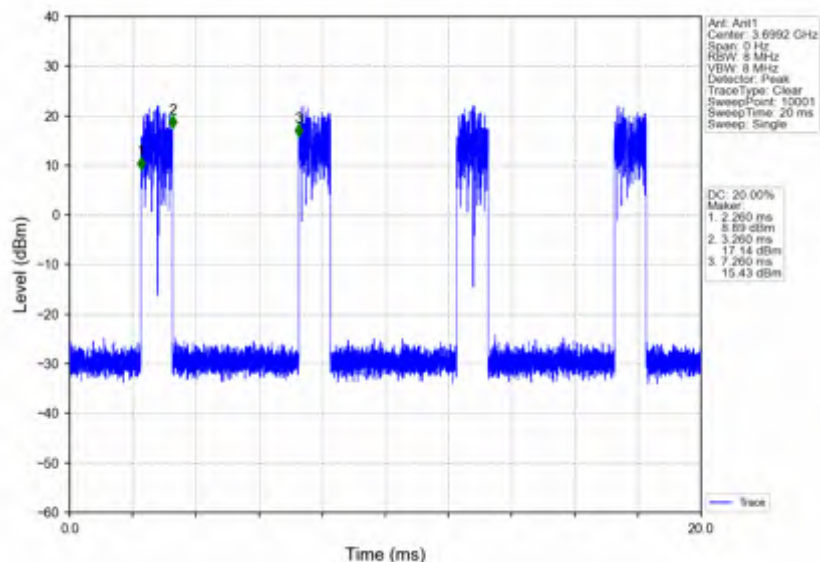
n78d_15kHz_SISO_NTNV_50MHz_CP-OFDM 64 QAM_3675MHz_Edge_1RB_Right
