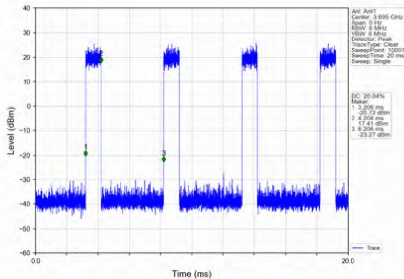
n78d_30kHz_SISO_NTNV_10MHz_CP-OFDM_QPSK_3694.98MHz_Inner_Full
