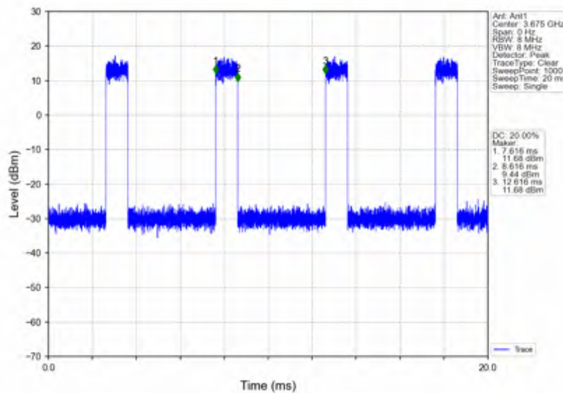
n78d_15kHz_SISO_NTNV_50MHz_CP-OFDM 64 QAM_3675MHz_Inner_Full
