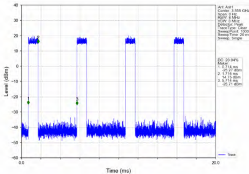
n78d_30kHz_SISO_NTNV_10MHz_DFT-s-OFDM_QPSK_3555MHz_Inner_Full
