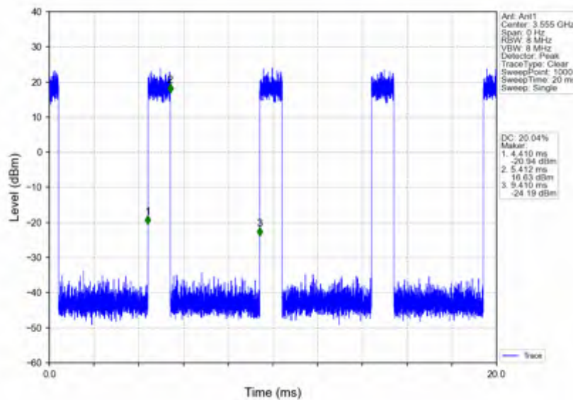
n78d_30kHz_SISO_NTNV_10MHz_CP-OFDM 64 QAM_3555MHz_Inner_Full
