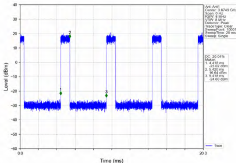
n78d_15kHz_SISO_NTNV_50MHz_CP-OFDM 64 QAM_3675MHz_Inner_Full
