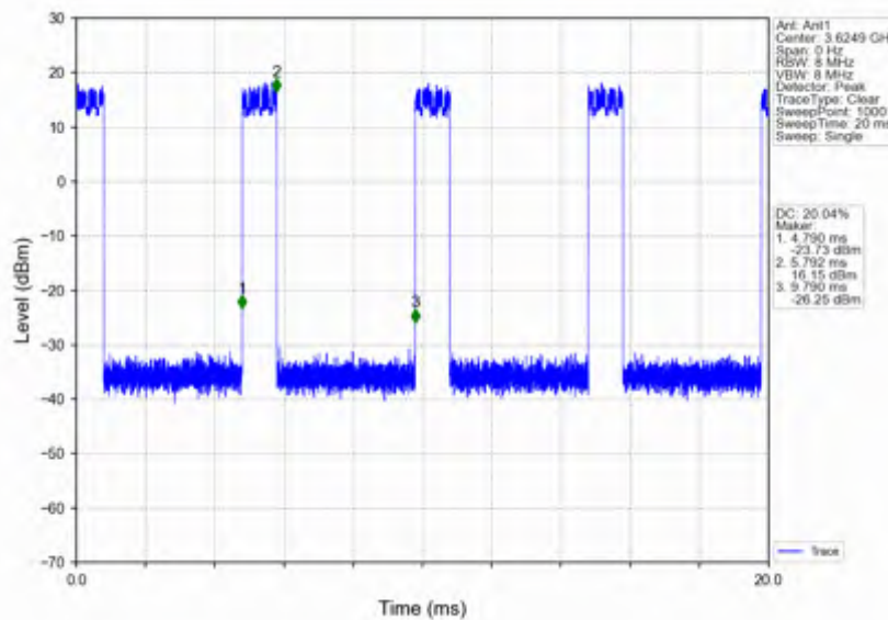
n78d_15kHz_SISO_NTNV_50MHz_DFT-s-OFDM_16_QAM_3625.005MHz_Inner_Full
