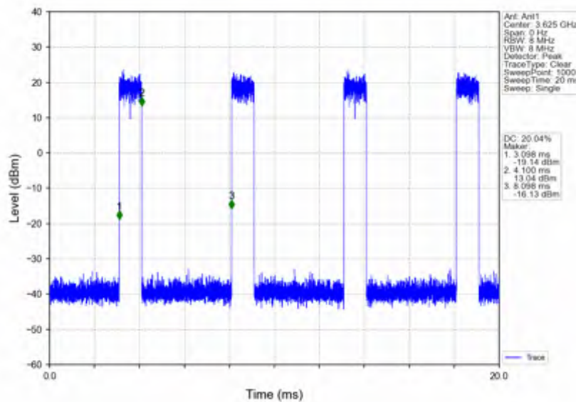
n78d_30kHz_SISO_NTNV_10MHz_CP-OFDM_256_QAM_3624.99MHz_Inner_Full
