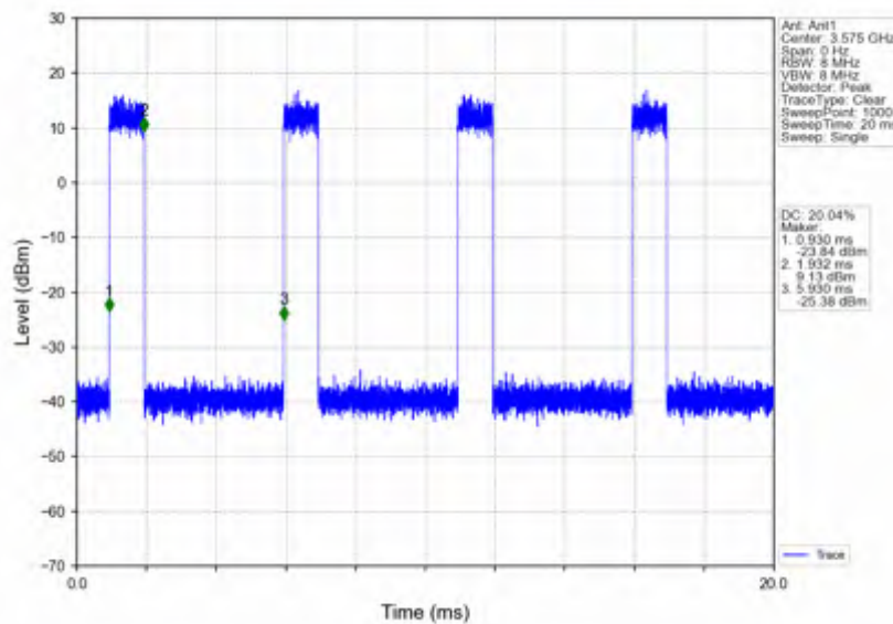
n78d_15kHz_SISO_NTNV_50MHz_CP-OFDM 64 QAM_3575.01MHz_Inner_Full
