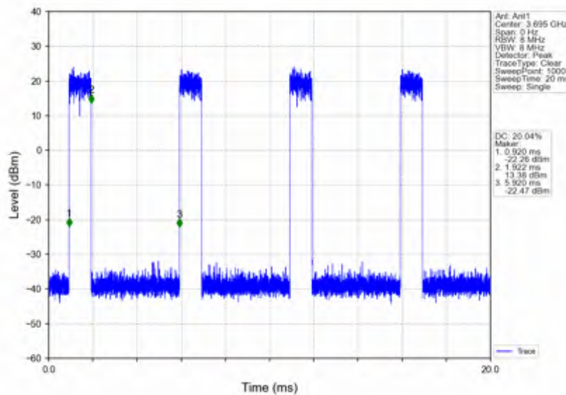
n78d_30kHz_SISO_NTNV_10MHz_CP-OFDM_256_QAM_3694.98MHz_Inner_Full
