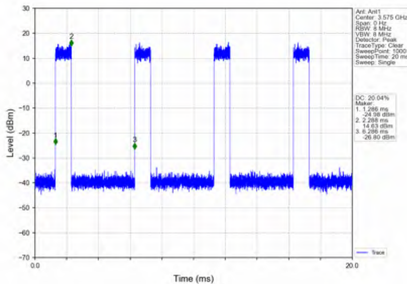
n78d_15kHz_SISO_NTNV_50MHz_CP-OFDM 16 QAM 3575.01MHz_Inner_Full
