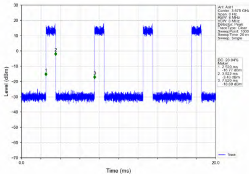
n78d_15kHz_SISO_NTNV_50MHz_CP-OFDM 256 QAM_3675MHz_Inner_Full
