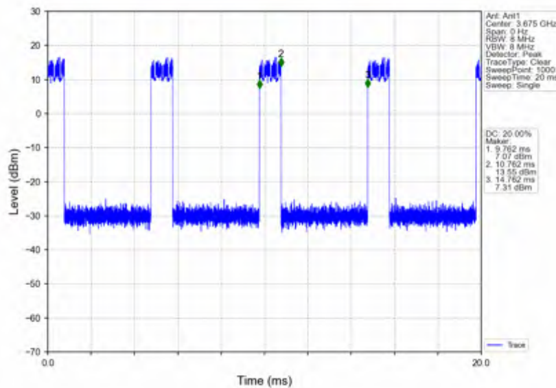
n78d_15kHz_SISO_NTNV_50MHz_DFT-s-OFDM_256_QAM_3675MHz_Inner_Full
