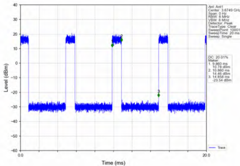
n78d_15kHz_SISO_NTNV_50MHz_CP-OFDM_QPSK_3675MHz_Inner_Full
