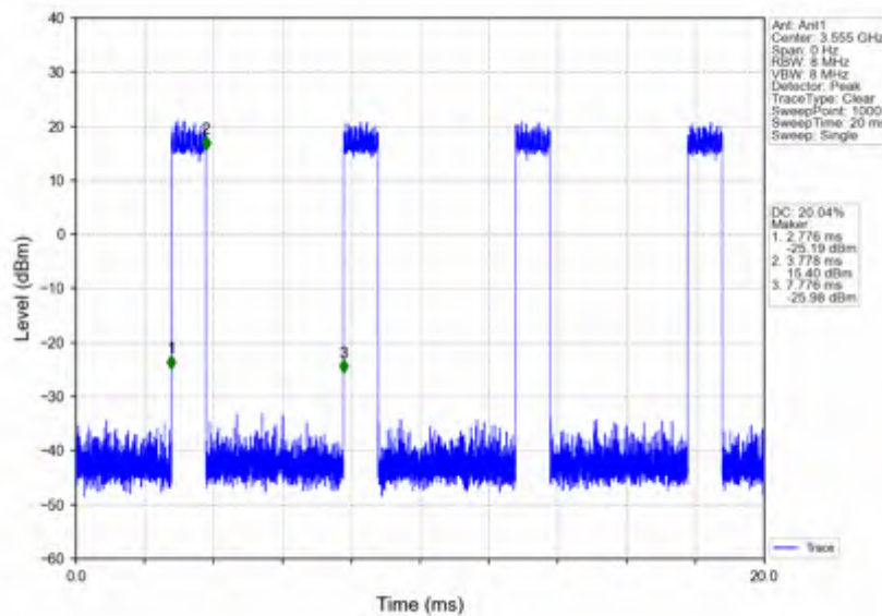
n78d_30kHz_SISO_NTNV_10MHz_DFT-s-OFDM 16 QAM_3555MHz_Inner_Full
