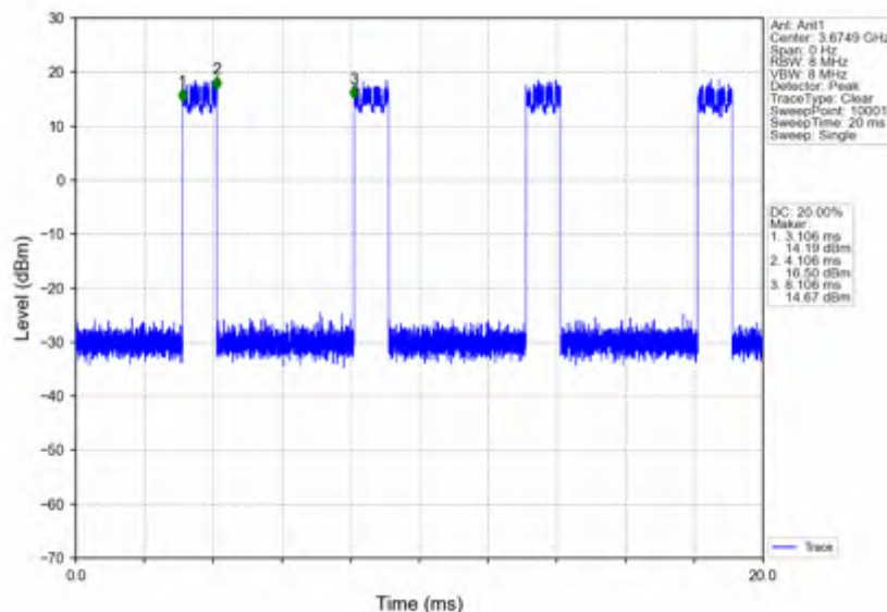
n78d_15kHz_SISO_NTNV_50MHz_DFT-s-OFDM 16 QAM_3675MHz_Inner_Full
