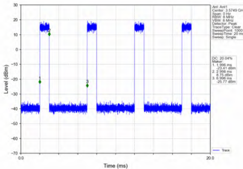
n78d_15kHz_SISO_NTNV_50MHz_CP-OFDM_256_QAM_3575.01MHz_Inner_Full
