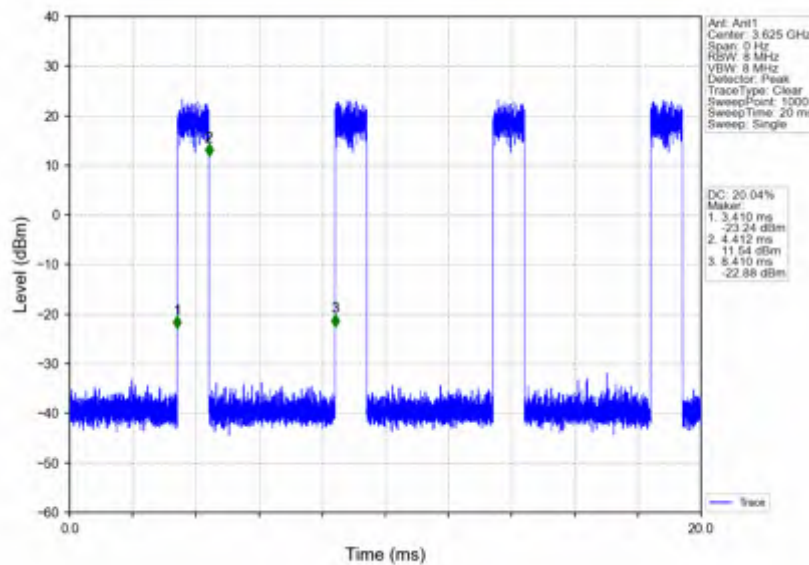
n78d_30kHz_SISO_NTNV_10MHz_CP-OFDM 16 QAM 3624.99MHz_Inner_Full
