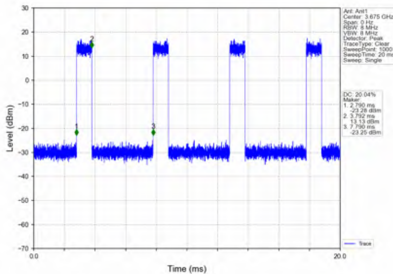
n78d_15kHz_SISO_NTNV_50MHz_CP-OFDM_16 QAM_3675MHz_Inner_Full
