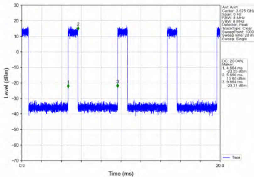
n78d_15kHz_SISO_NTNV_50MHz_CP-OFDM_16_QAM_3625.005MHz_Inner_Full
