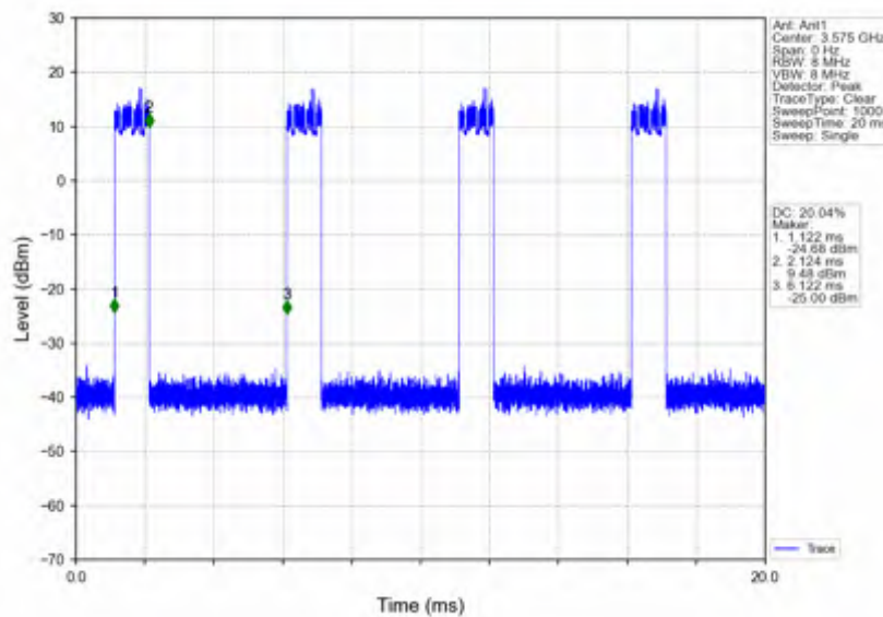
n78d_15kHz_SISO_NTNV_50MHz_DFT-s-OFDM_256_QAM_3575.01MHz_Inner_Full
