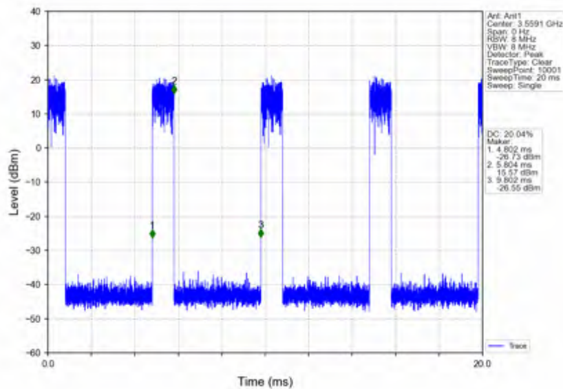
n78d_30kHz_SISO_NTNV_10MHz_CP-OFDM_QPSK_3555MHz_Edge_1RB_Right
