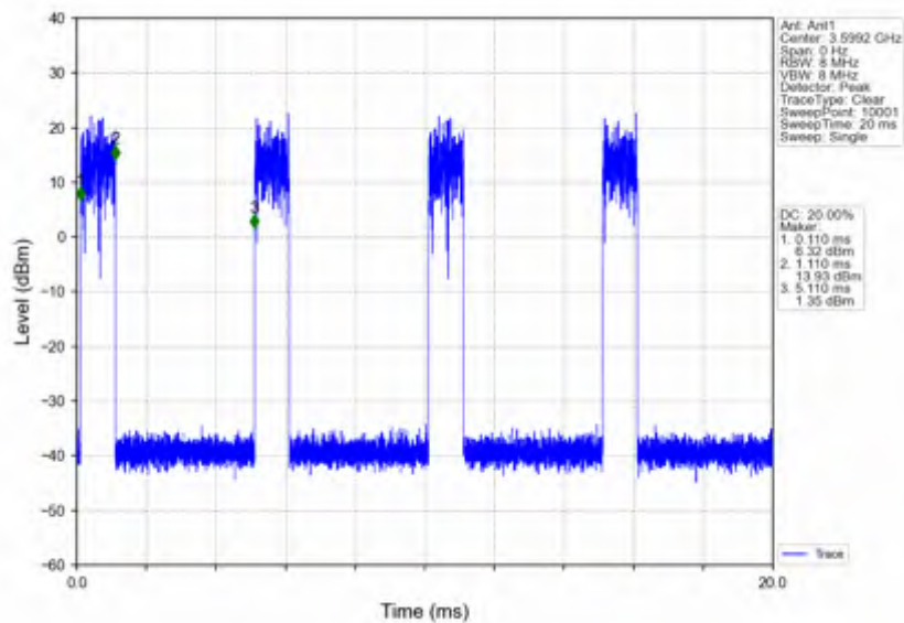
n78d_15kHz_SISO_NTNV_50MHz_CP-OFDM_16_QAM_3575.01MHz_Edge_1RB_Right
