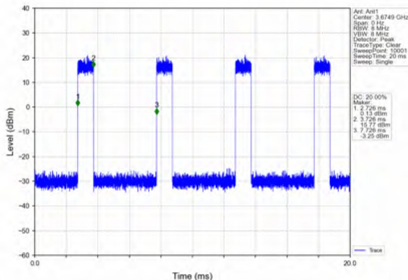
n78d_15kHz_SISO_NTNV_50MHz_CP-OFDM 256 QAM_3675MHz_Inner_Full
