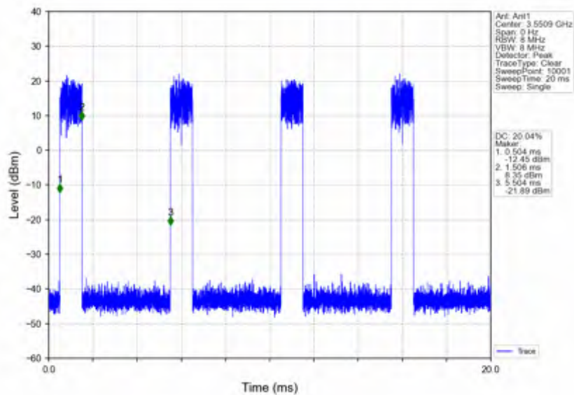
n78d_30kHz_SISO_NTNV_10MHz_CP-OFDM 64 QAM_3555MHz_Edge_1RB_Right
