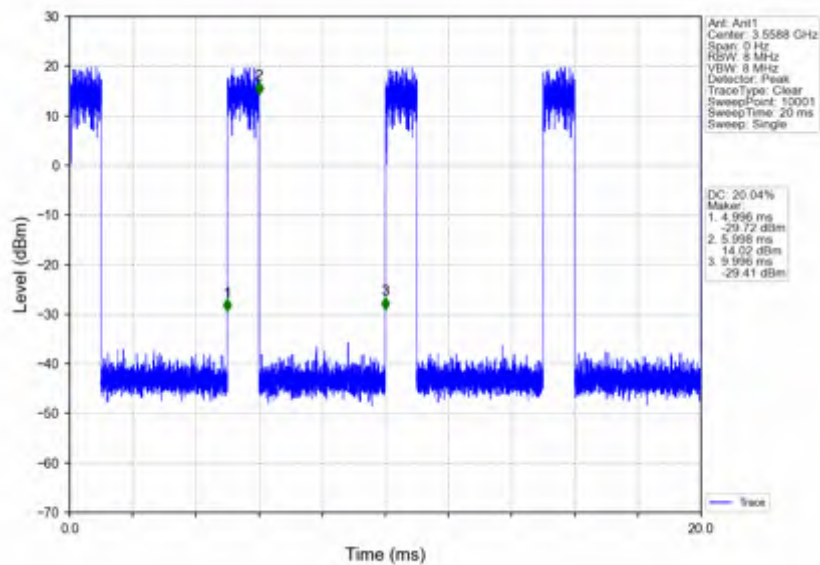
n78d_30kHz_SISO_NTNV_10MHz_DFT-s-OFDM 64 QAM_3555MHz_Inner_1RB_Right
