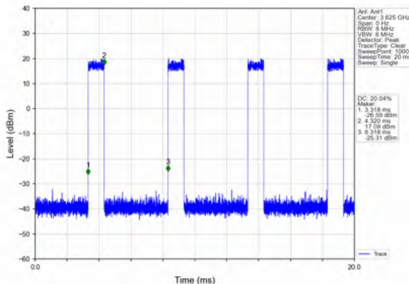
n78d 30kHz SISO NTNV 10MHz DFT-s-OFDM QPSK 3624.99MHz Inner Full
