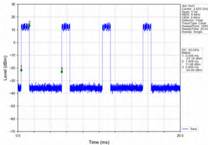
n78d_15kHz_SISO_NTNV_50MHz_DFT-s-OFDM 64 QAM_3625.005MHz_Inner_Full
