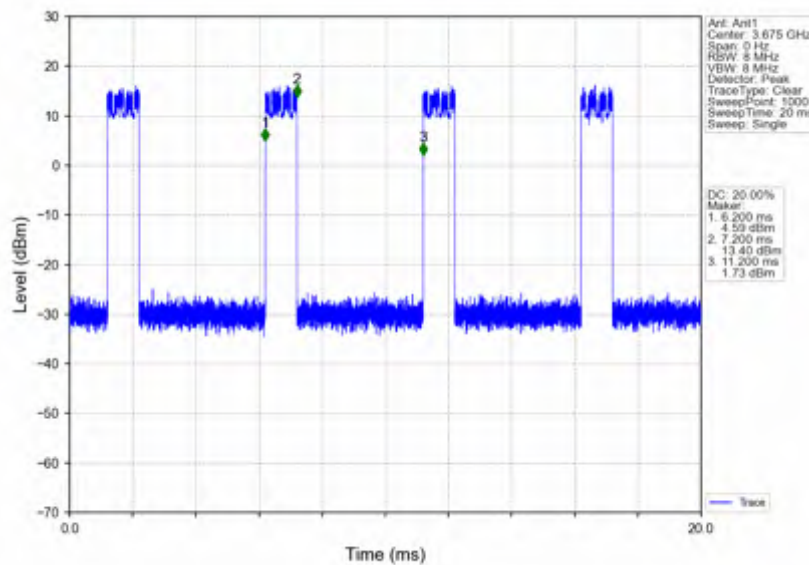
n78d_15kHz_SISO_NTNV_50MHz_DFT-s-OFDM 16 QAM_3675MHz_Inner_Full
