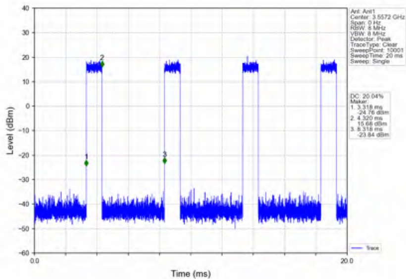
n78d_30kHz_SISO_NTNV_15MHz_DFT-s-OFDM_QPSK_3557.52MHz_Inner_Full
