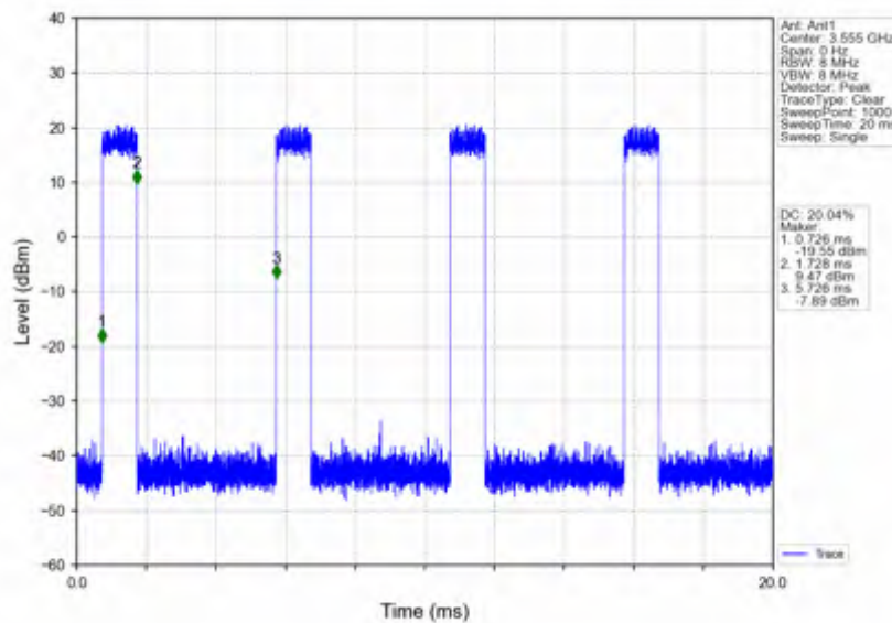
n78d_30kHz_SISO_NTNV_10MHz_DFT-s-OFDM_256_QAM_3555MHz_Inner_Full
