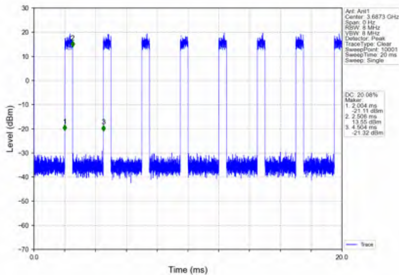
n78d_30kHz_SISO_NTNV_25MHz_DFT-s-OFDM_QPSK_3687.48MHz_Inner_Full
