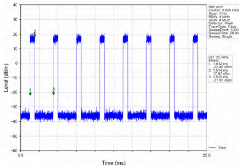
n78d_30kHz_SISO_NTNV_20MHz_CP-OFDM_256_QAM_3624.99MHz_Inner_Full
