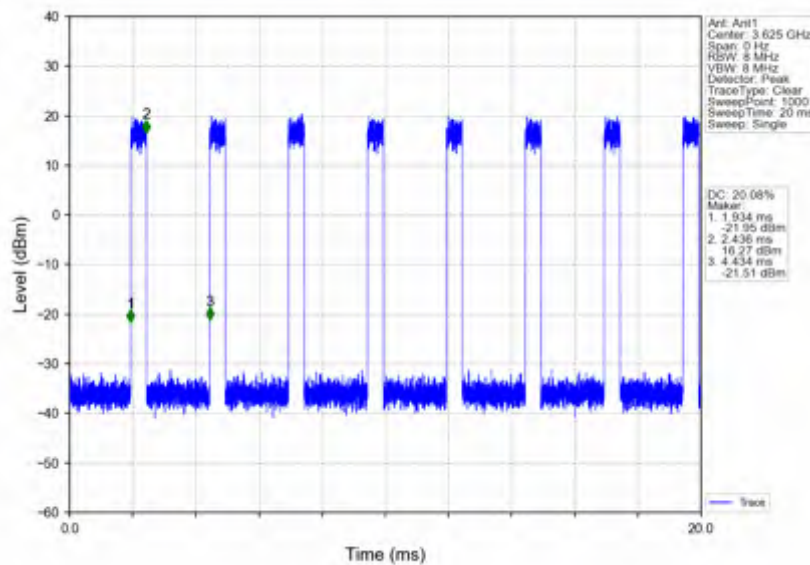
n78d_30kHz_SISO_NTNV_20MHz_CP-OFDM 64 QAM_3624.99MHz_Inner_Full
