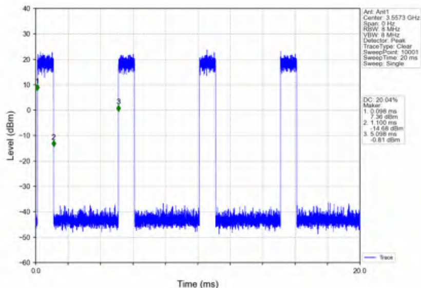
n78d_30kHz_SISO_NTNV_15MHz_CP-OFDM_16_QAM_3557.52MHz_Inner_Full
