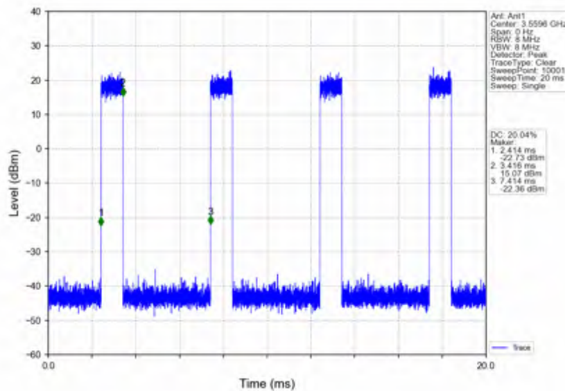
n78d_30kHz_SISO_NTNV_20MHz_CP-OFDM QPSK_3560.01MHz_Inner_Full
