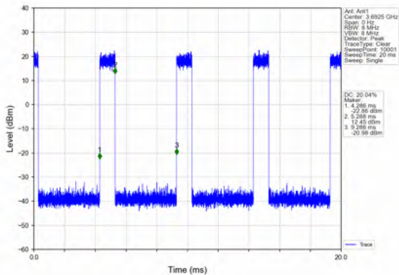
n78d_30kHz_SISO_NTNV_15MHz_CP-OFDM 64 QAM_3692.49MHz_Inner_Full
