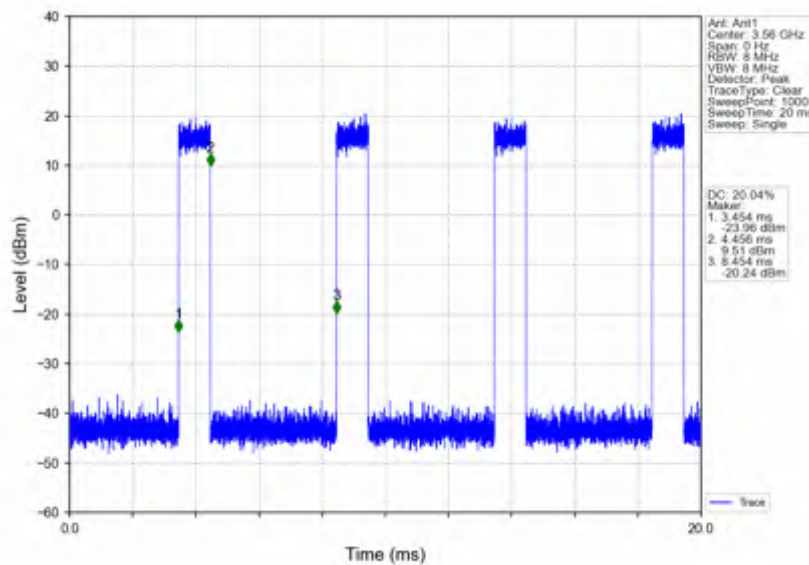
n78d_30kHz_SISO_NTNV_20MHz_CP-OFDM 64 QAM_3560.01MHz_Inner_Full
