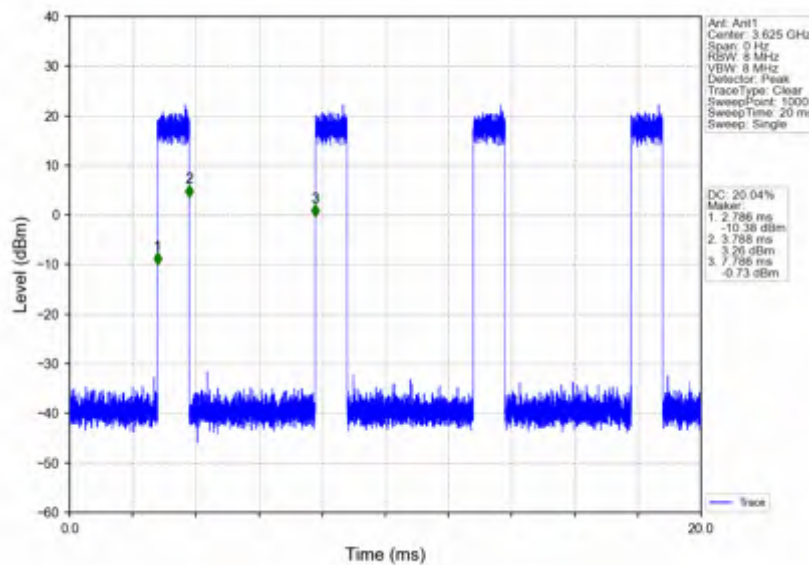
n78d_30kHz_SISO_NTNV_15MHz_CP-OFDM_QPSK_3624.99MHz_Inner_Full
