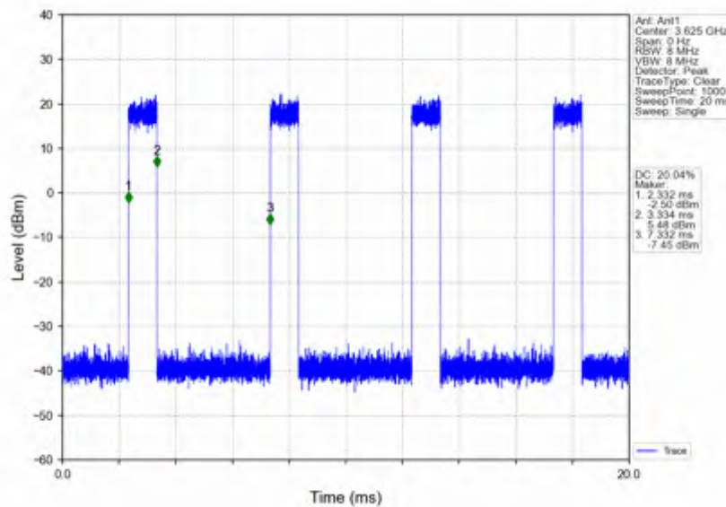
n78d_30kHz_SISO_NTNV_15MHz_CP-OFDM 64 QAM_3624.99MHz_Inner_Full
