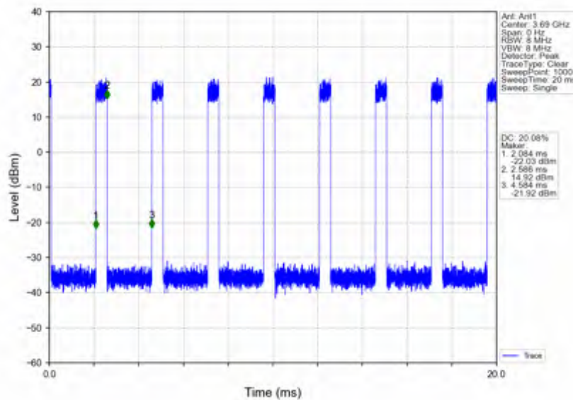
n78d_30kHz_SISO_NTNV_20MHz_CP-OFDM_256_QAM_3690MHz_Inner_Full
