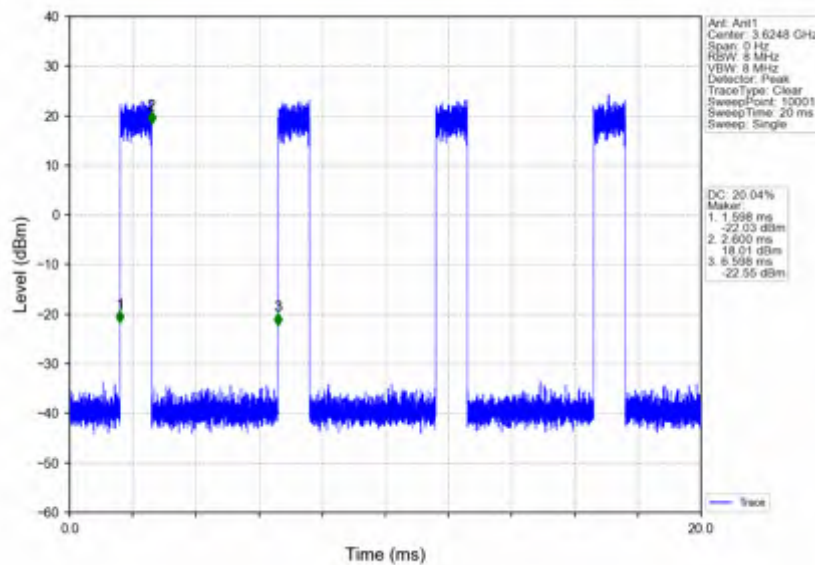
n78d_30kHz_SISO_NTNV_15MHz_CP-OFDM_QPSK_3624.99MHz_Inner_Full
