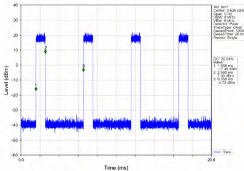
n78d_30kHz_SISO_NTNV_15MHz_CP-OFDM_256_QAM_3624.99MHz_Inner_Full
