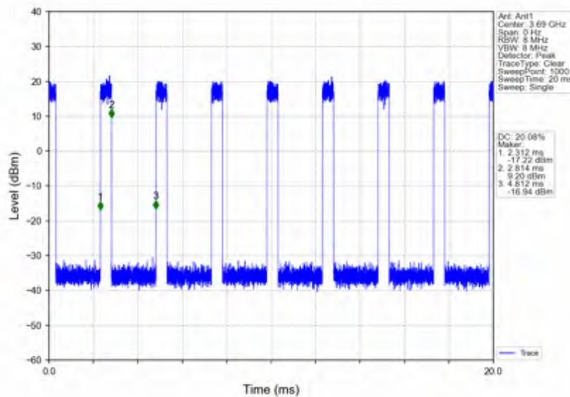
n78d_30kHz_SISO_NTNV_20MHz_CP-OFDM_QPSK_3690MHz_Inner_Full
