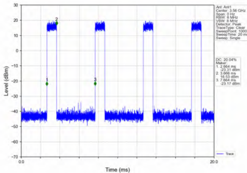
n78d_30kHz_SISO_NTNV_20MHz_CP-OFDM_16_QAM_3560.01MHz_Inner_Full
