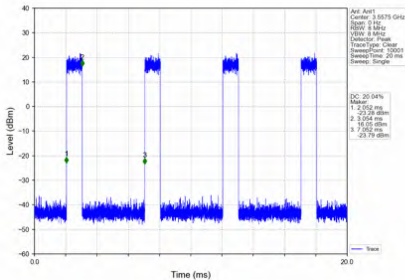
n78d_30kHz_SISO_NTNV_15MHz_CP-OFDM_QPSK_3557.52MHz_Inner_Full
