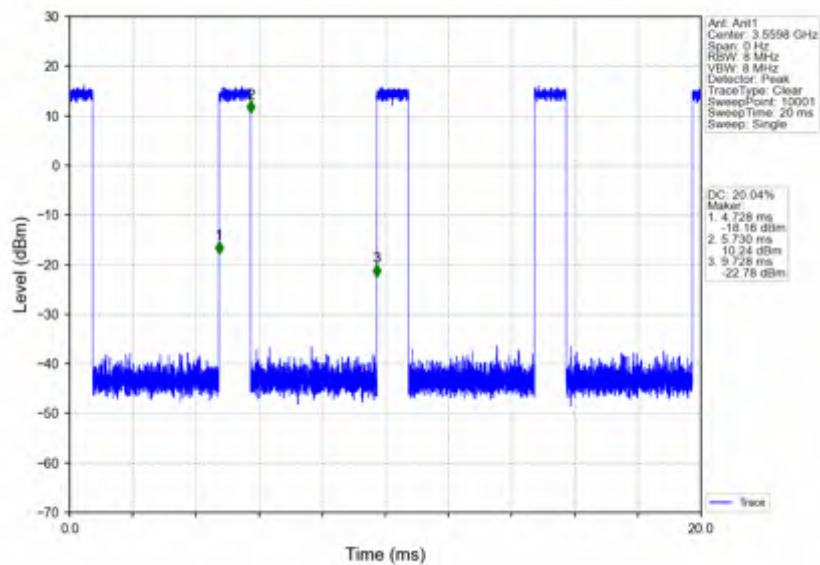
n78d_30kHz_SISO_NTNV_20MHz_DFT-s-OFDM_QPSK_3560.01MHz_Inner_Full
