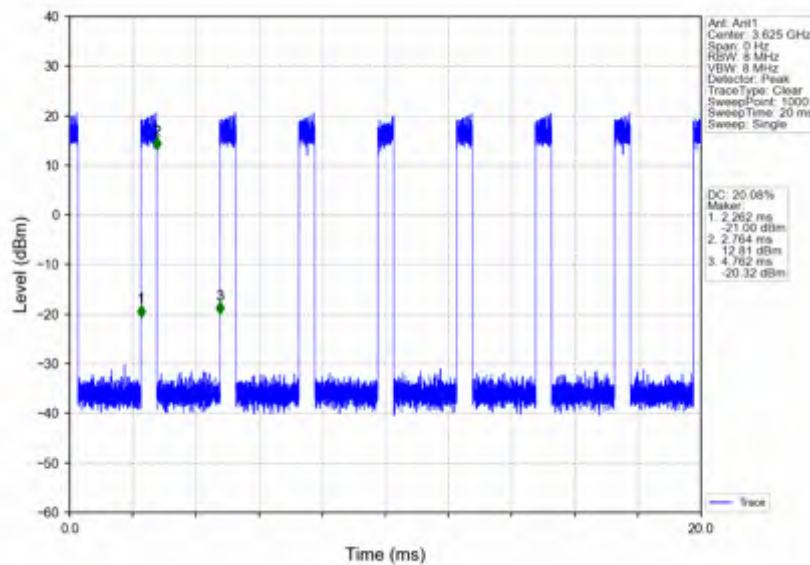
n78d_30kHz_SISO_NTNV_20MHz_CP-OFDM_16_QAM_3624.99MHz_Inner_Full
