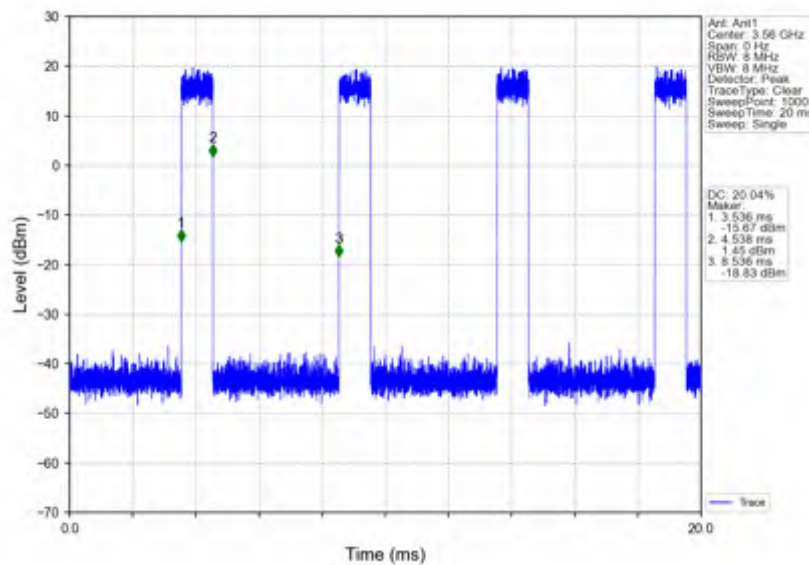
n78d_30kHz_SISO_NTNV_20MHz_CP-OFDM QPSK_3560.01MHz_Inner_Full
