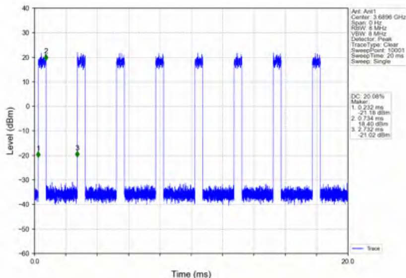
n78d_30kHz_SISO_NTNV_20MHz_DFT-s-OFDM 64 QAM_3690MHz_Inner_Full
