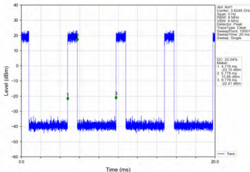
n78d_30kHz_SISO_NTNV_15MHz_CP-OFDM 64 QAM_3624.99MHz_Inner_Full
