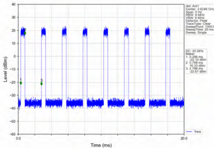
n78d_30kHz_SISO_NTNV_20MHz_CP-OFDM_QPSK_3624.99MHz_Inner_Full
