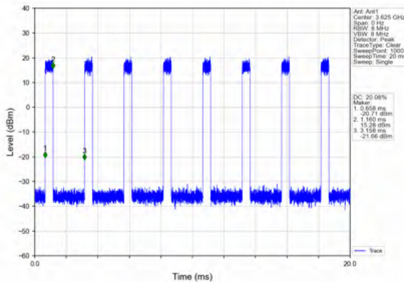
n78d_30kHz_SISO_NTNV_20MHz_CP-OFDM_QPSK_3624.99MHz_Inner_Full
