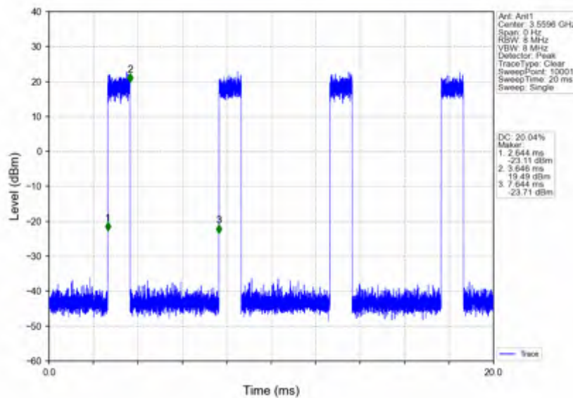
n78d_30kHz_SISO_NTNV_20MHz_CP-OFDM_256_QAM_3560.01MHz_Inner_Full
