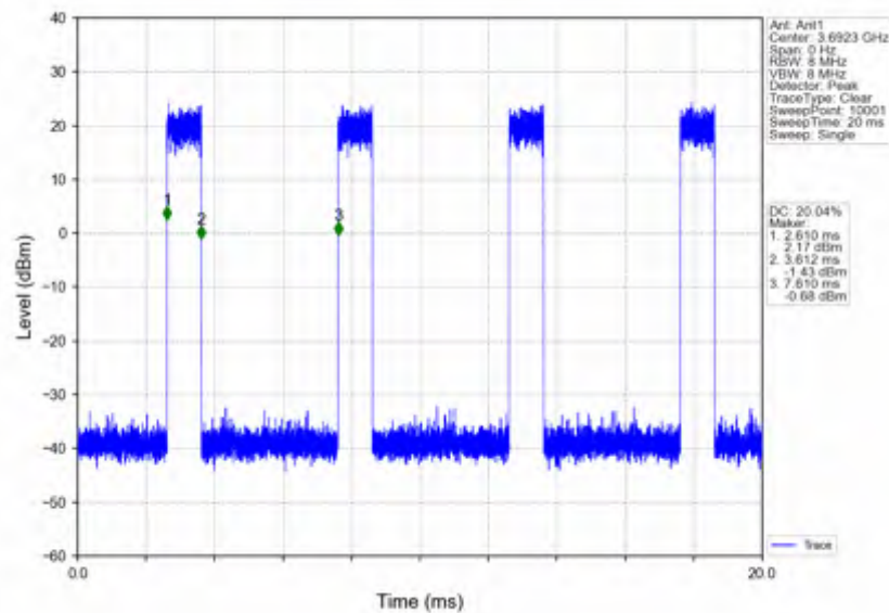
n78d_30kHz_SISO_NTNV_15MHz_CP-OFDM_QPSK_3692.49MHz_Inner_Full
