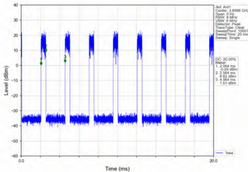
n78d_30kHz_SISO_NTNV_20MHz_CP-OFDM_QPSK_3690MHz_Inner_1RB_Right
