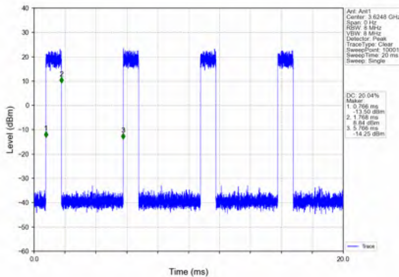
n78d_30kHz_SISO_NTNV_15MHz_CP-OFDM_256_QAM_3624.99MHz_Inner_Full
