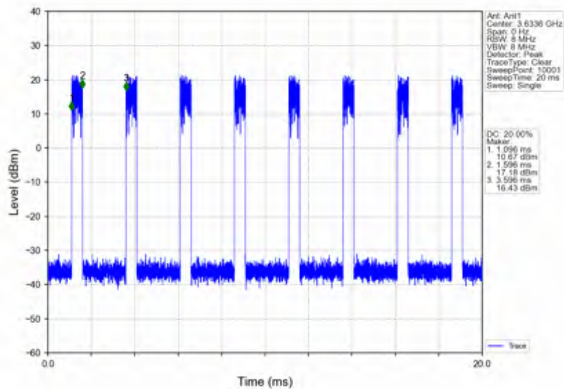
n78d_30kHz_SISO_NTNV_20MHz_CP-OFDM 64 QAM_3624.99MHz_Inner_1RB_Right
