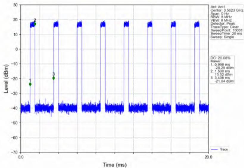
n78d_30kHz_SISO_NTNV_25MHz_DFT-s-OFDM_64_QAM_3562.5MHz_Inner_Full
