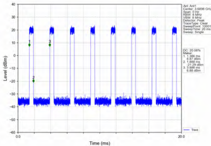
n78d_30kHz_SISO_NTNV_20MHz_CP-OFDM_256_QAM_3690MHz_Inner_Full
