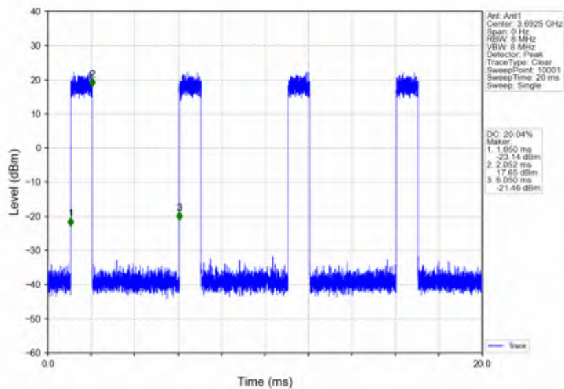
n78d_30kHz_SISO_NTNV_15MHz_CP-OFDM_256_QAM_3692.49MHz_Inner_Full
